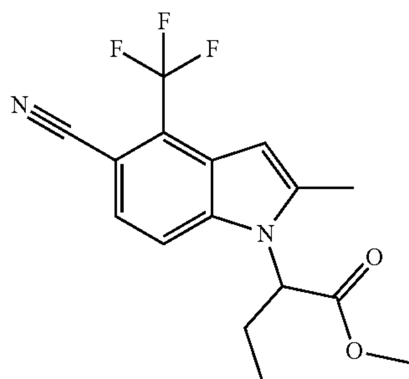
Methyl 2-[5-cyano-2-methyl-4-(trifluoromethyl)-1H-indol-1-yl]butanoate
