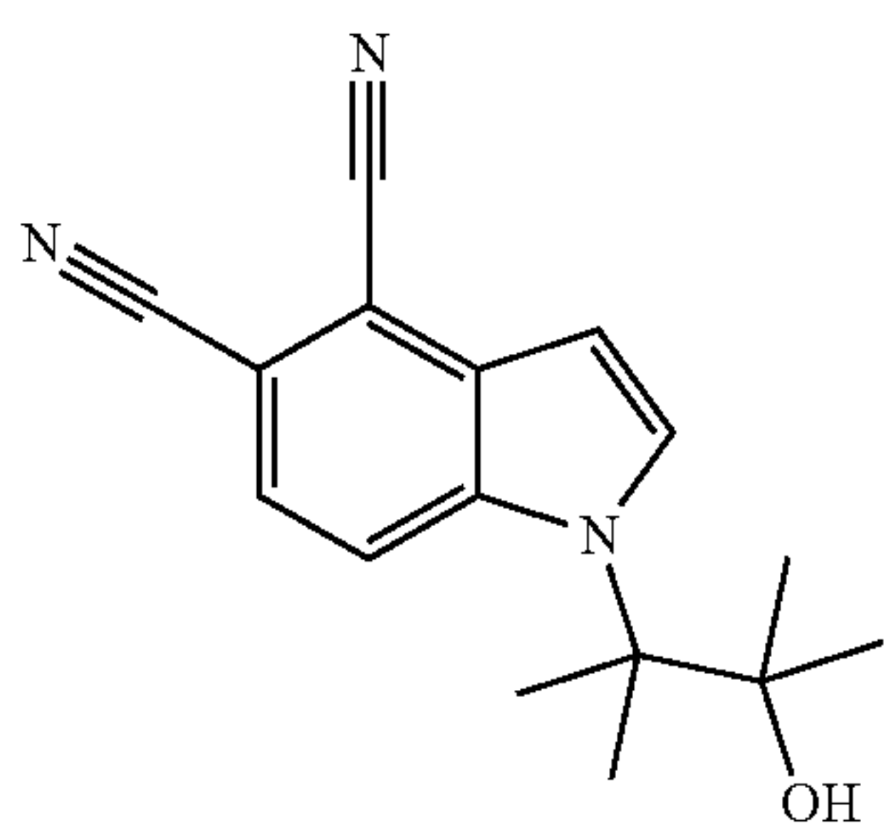
1-(3-Hydroxy-2,3-dimethylbutan-2-yl)-1H-indole-4,5-dicarbonitrile
