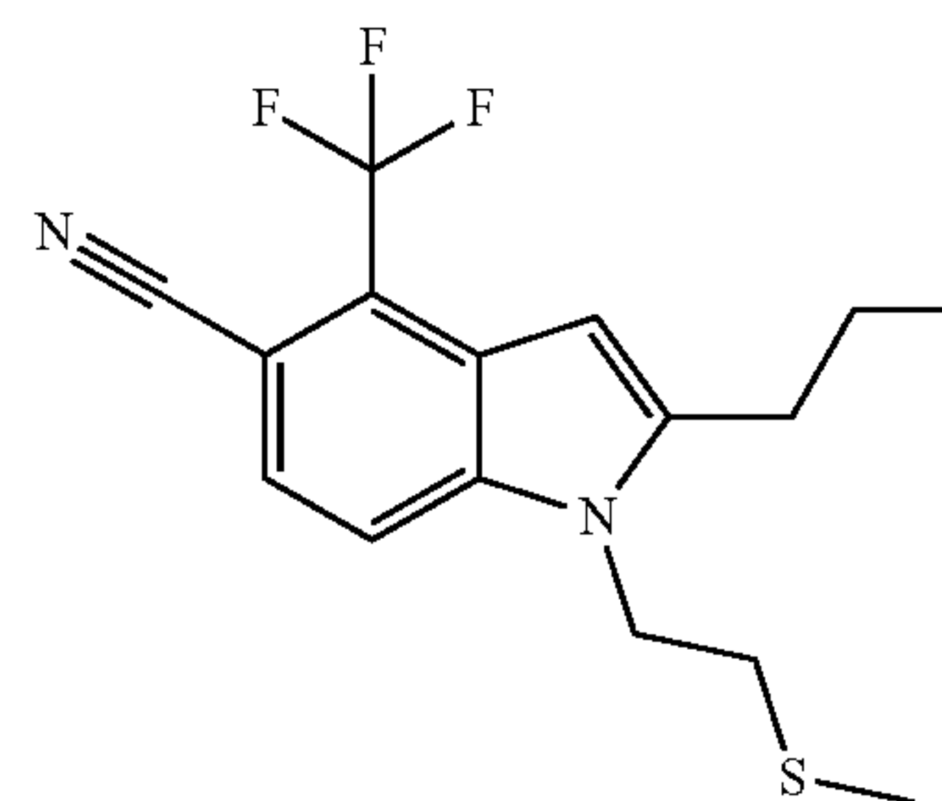
1-(2-(Methylthio)ethyl)-2-propyl-4-(trifluoromethyl)-1H-indole-5-carbonitrile
