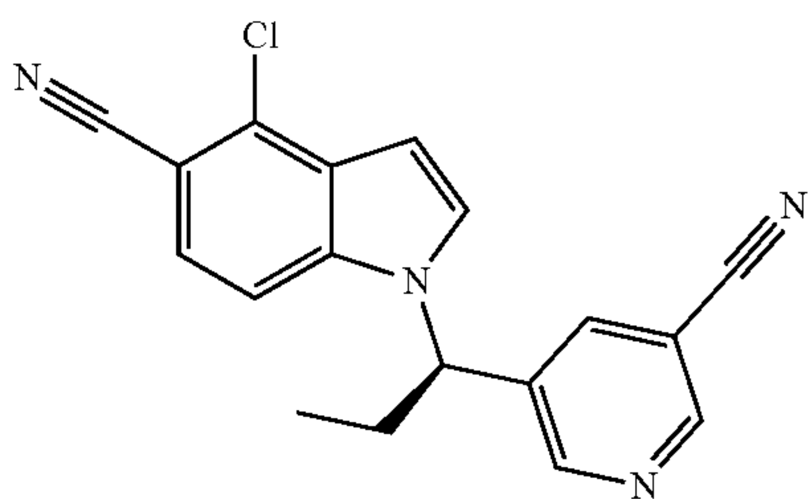
(R)-4-Chloro-1-(1-(5-cyanopyridin-3-yl)propyl)-1H-indole-5-carbonitrile
