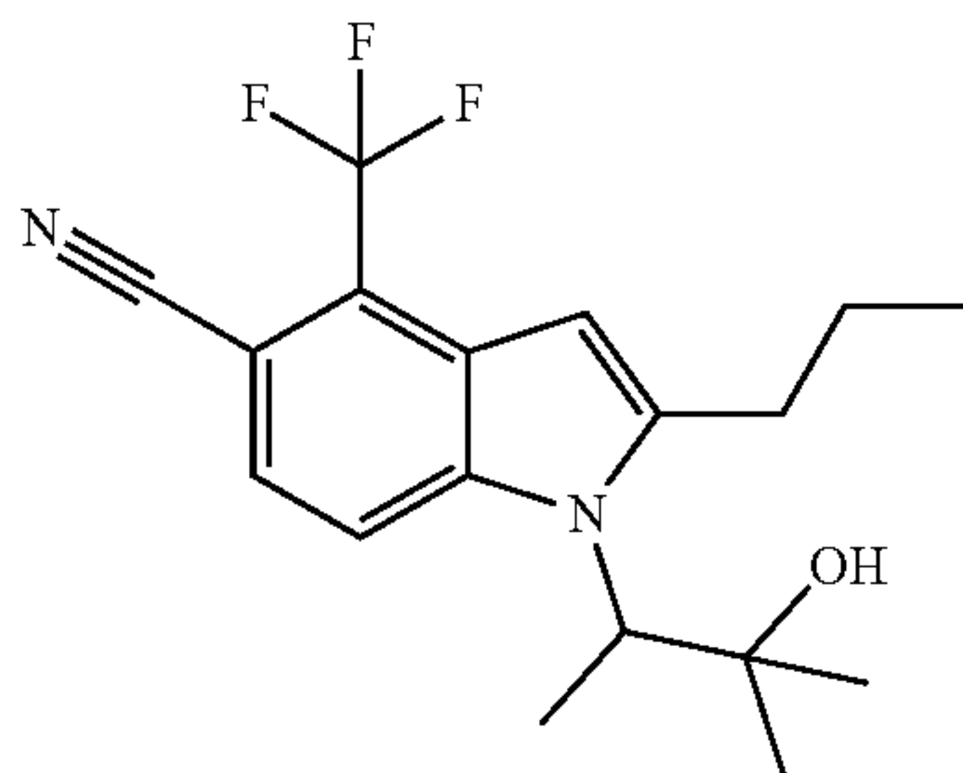
B. 1-(3-Hydroxy-3-methylbutan-2-yl)-2-propyl-4-(trifluoromethyl)-1H-indole-5-carbonitrile
