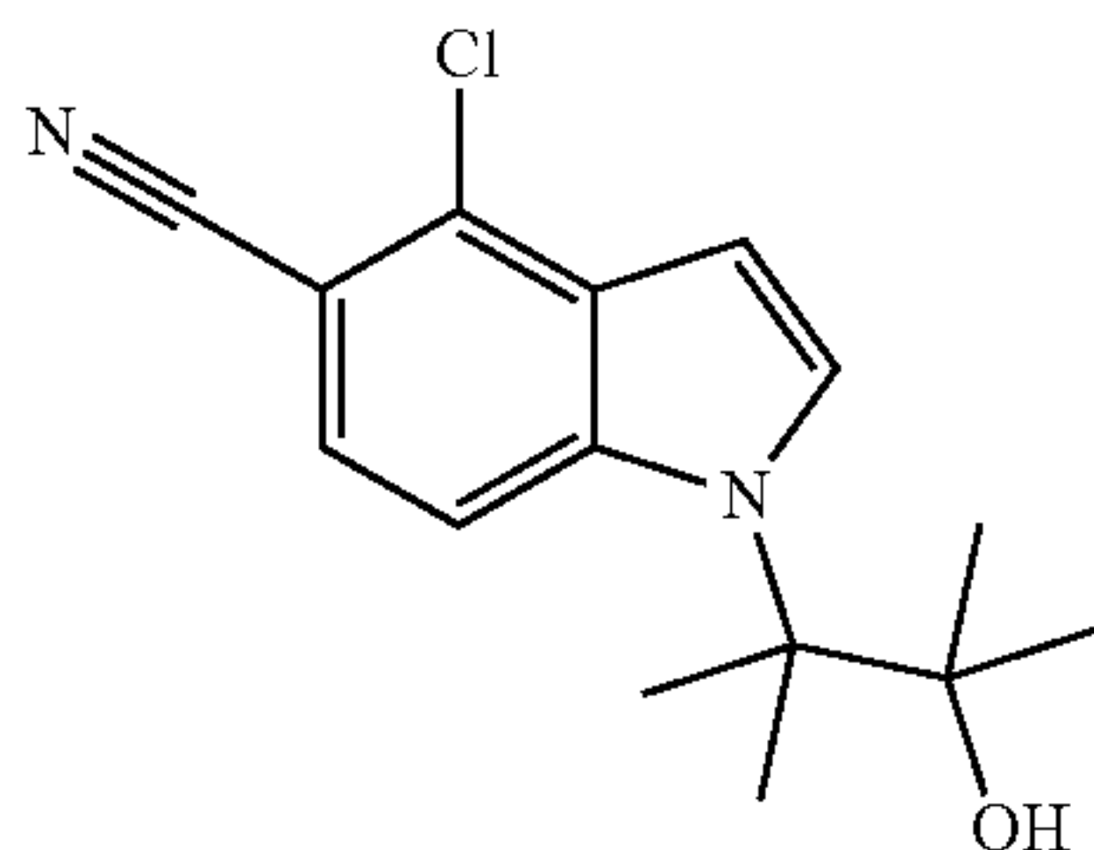
4-Chloro-1-(3-hydroxy-2,3-dimethylbutan-2-yl)-1H-indole-5-carbonitrile
