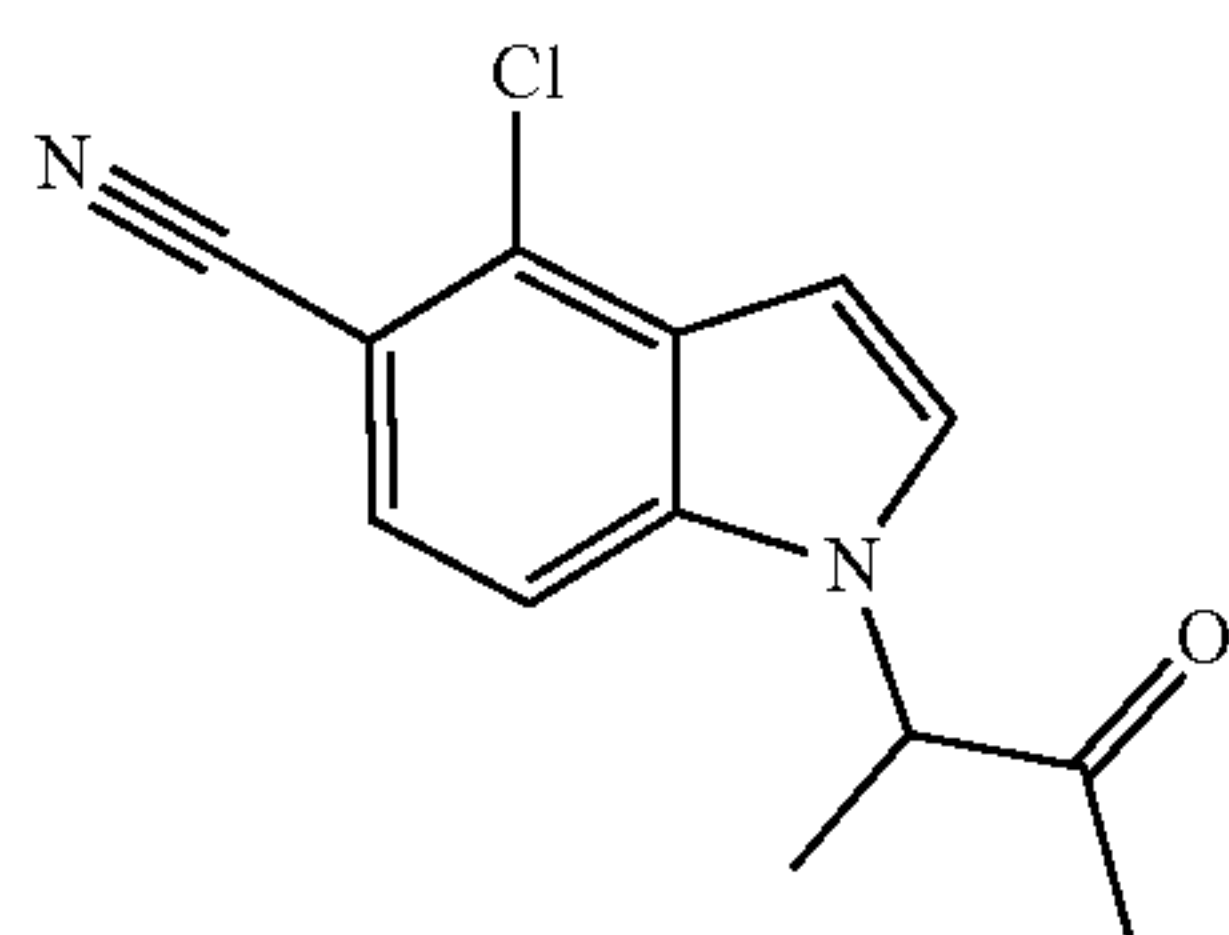
4-Chloro-1-(3-oxobutan-2-yl)-1H-indole-5-carbonitrile
