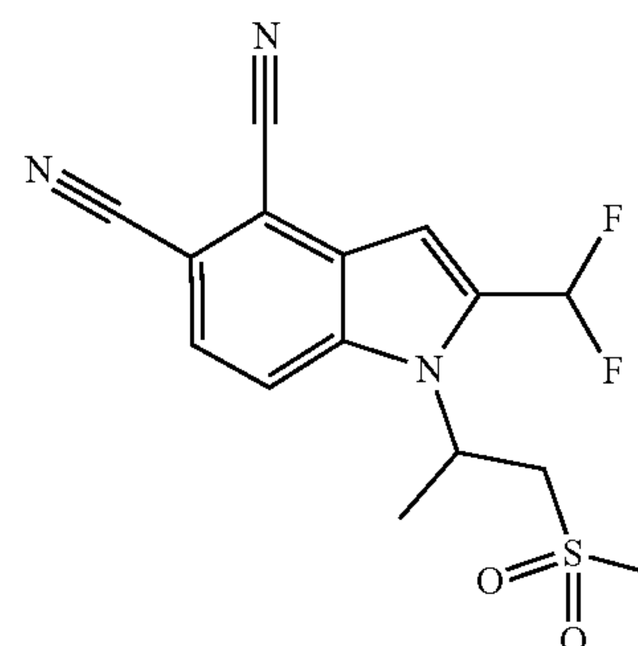
2-(Difluoromethyl)-1-(1-(methylsulfonyl)propan-2-yl)-1H-indole-4,5-dicarbonitrile
