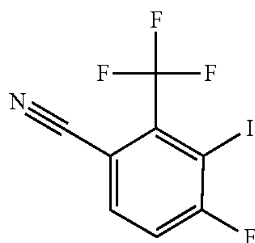
C. 4-Fluoro-3-iodo-2-(trifluoromethyl)benzonitrile
