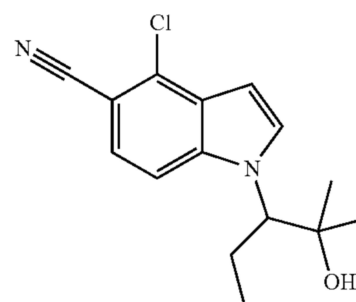
B. 4-Chloro-1-(2-hydroxy-2-methylpentan-3-yl)-1H-indole-5-carbonitrile
