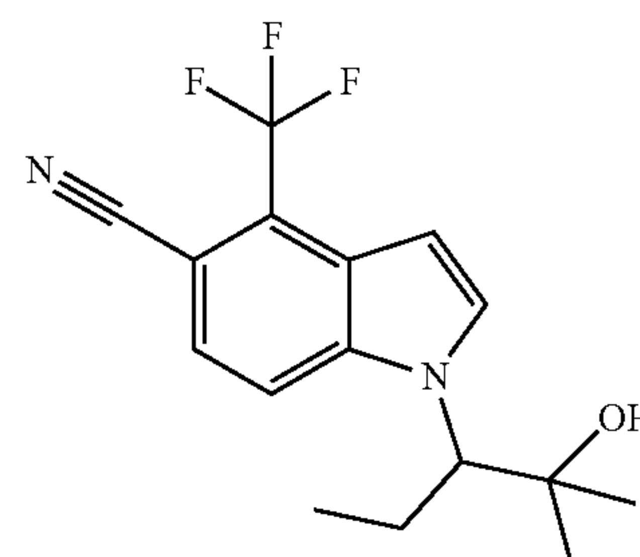
1-(2-Hydroxy-2-methylpentan-3-yl)-4-(trifluoromethyl)-1H-indole-5-carbonitrile
