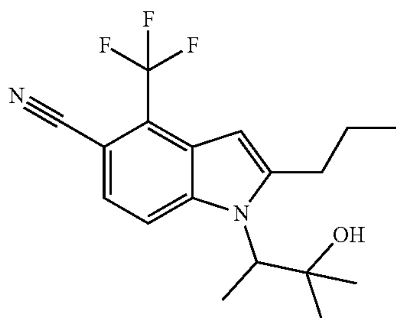
1-(3-Hydroxy-3-methylbutan-2-yl)-2-propyl-4-(trifluoromethyl)-1H-indole-5-carbonitrile
