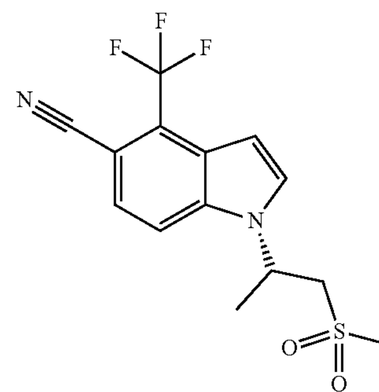
(S)-1-(1-(Methylsulfonyl)propan-2-yl)-4-(trifluoromethyl)-1H-indole-5-carbonitrile
