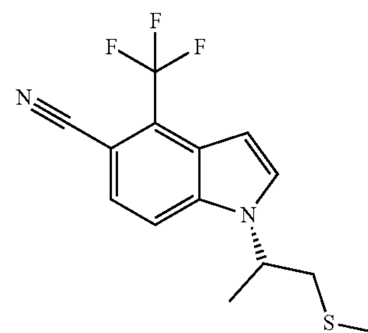
(S)-1-(1-(Methylthio)propan-2-yl)-4-(trifluoromethyl)-1H-indole-5-carbonitrile
