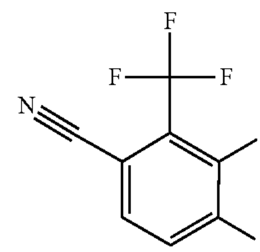
4-Fluoro-3-iodo-2-(trifluoromethyl)benzonitrile
