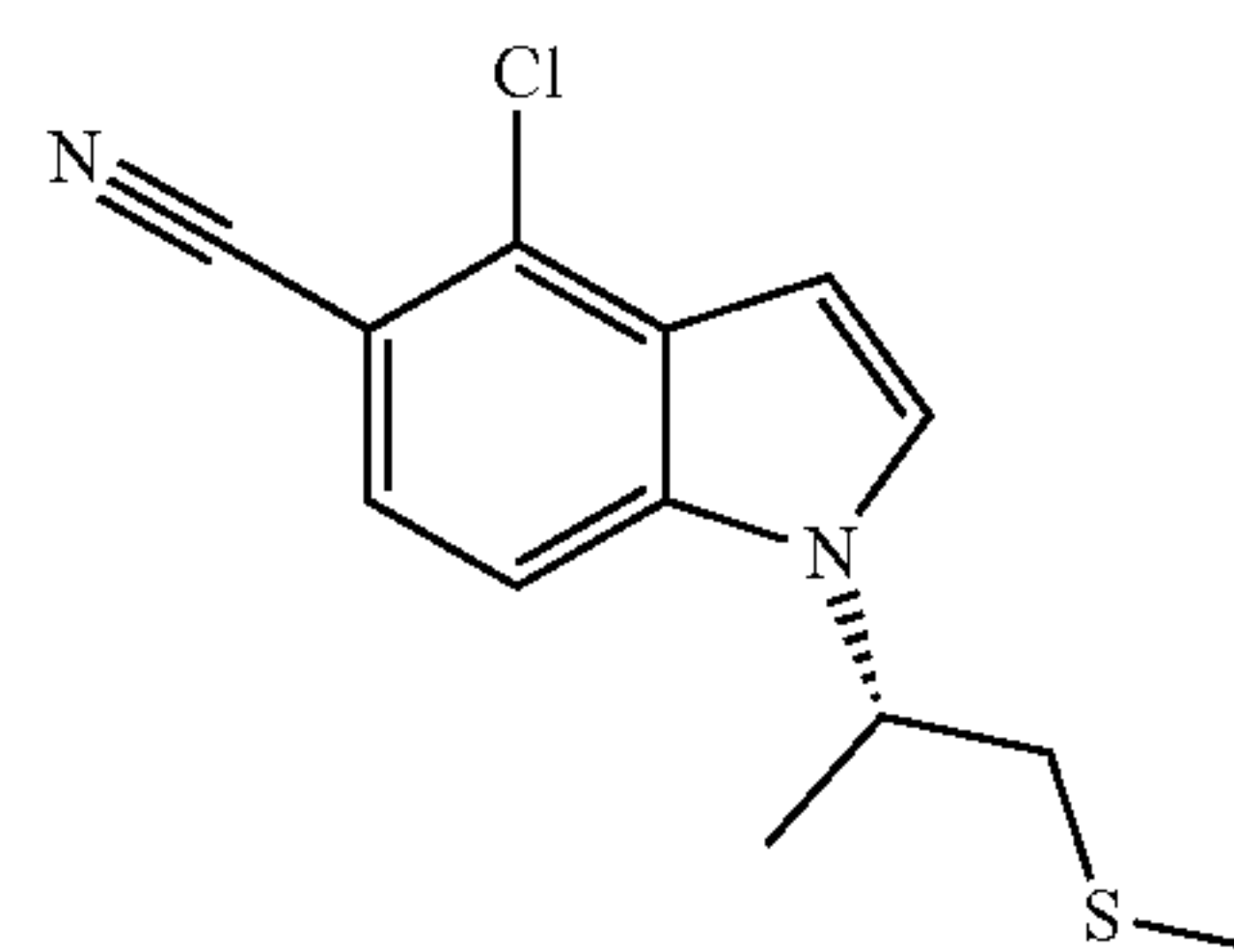
(S)-4-Chloro-1-(1-(methylthio)propan-2-yl)-1H-indole-5-carbonitrile
