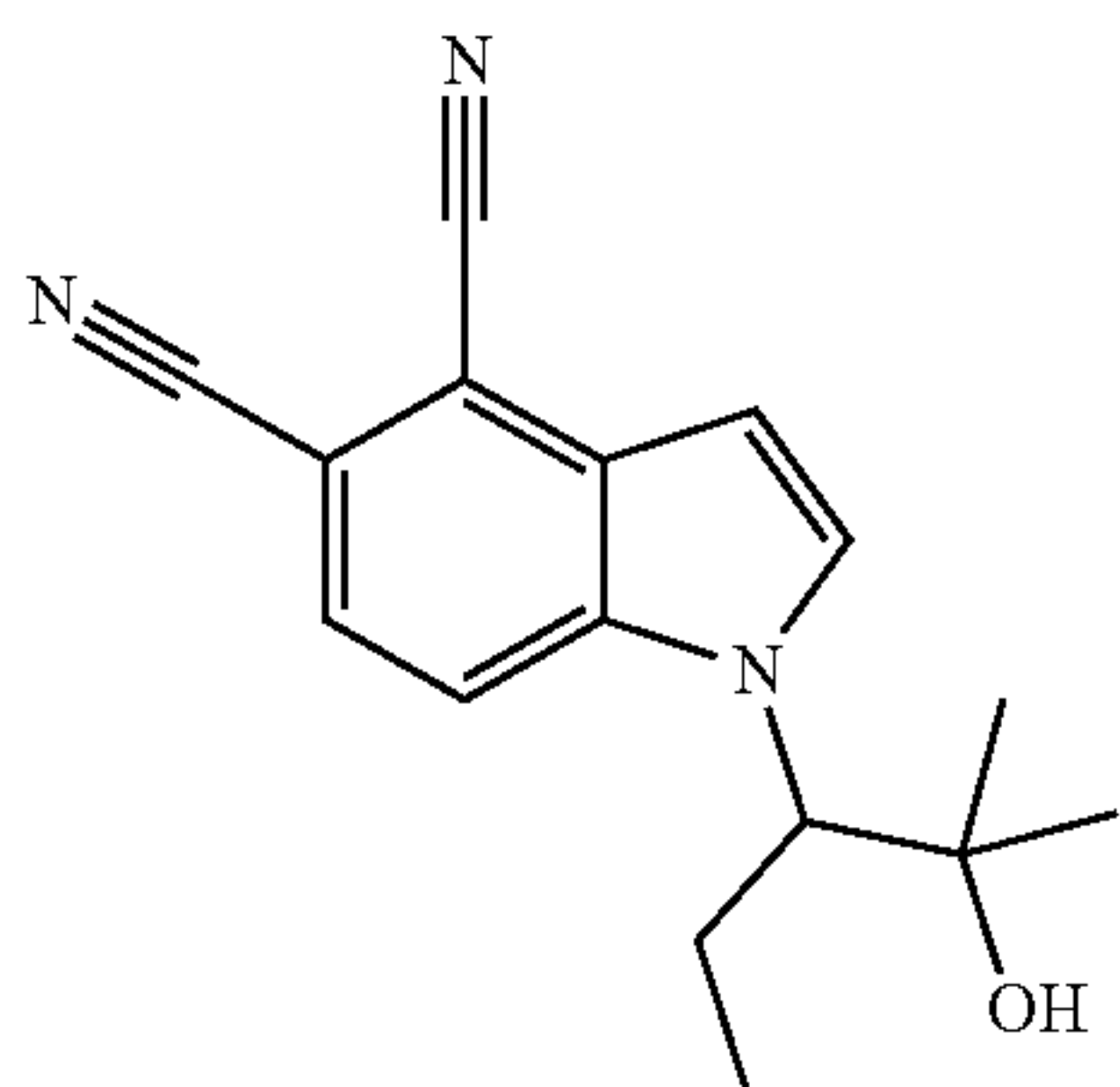
1-(2-Hydroxy-2-methylpentan-3-yl)-1H-indole-4,5-dicarbonitrile
