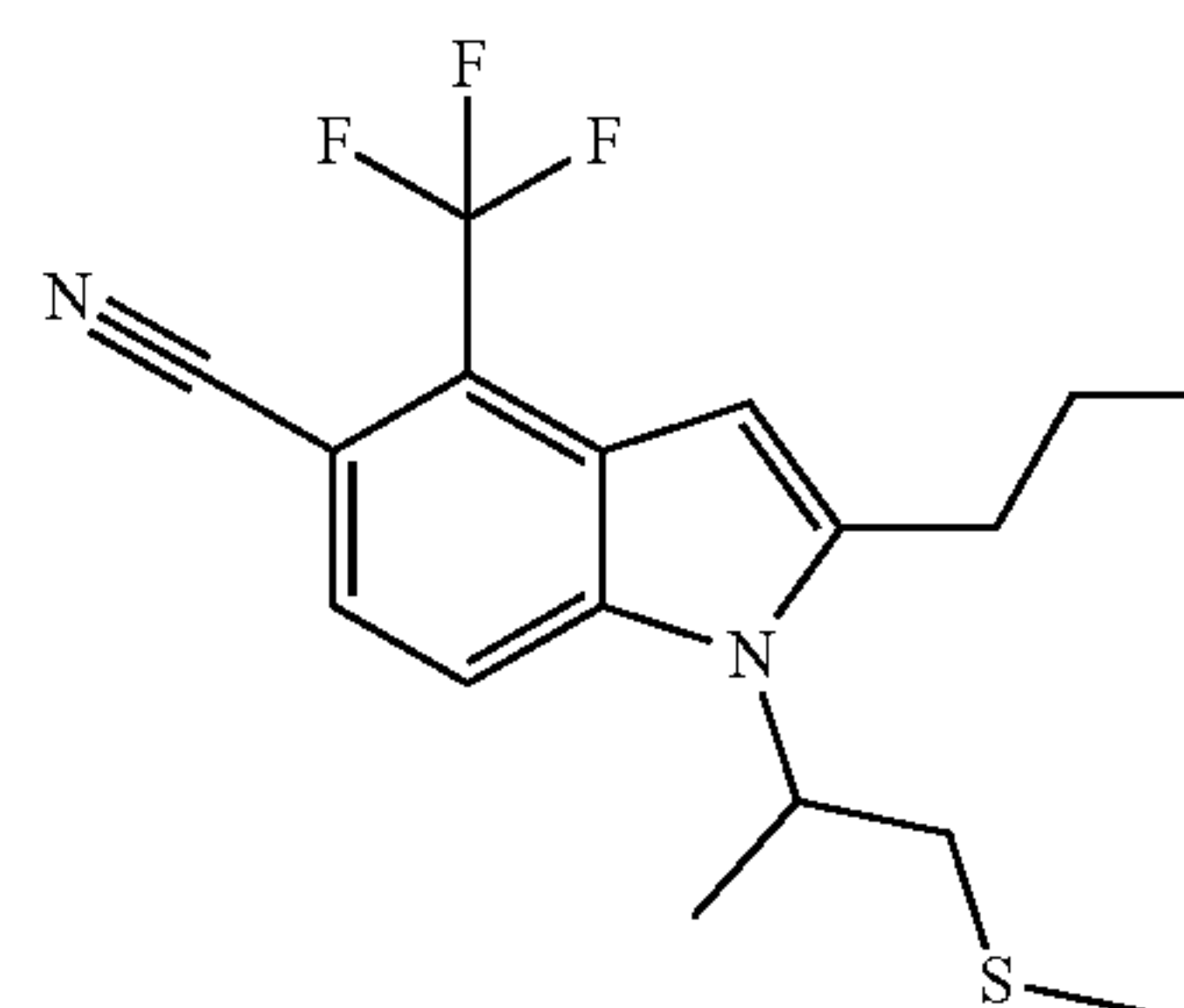
1-(1-(Methylthio)propan-2-yl)-2-propyl-4-(trifluoromethyl)-1H-indole-5-carbonitrile
