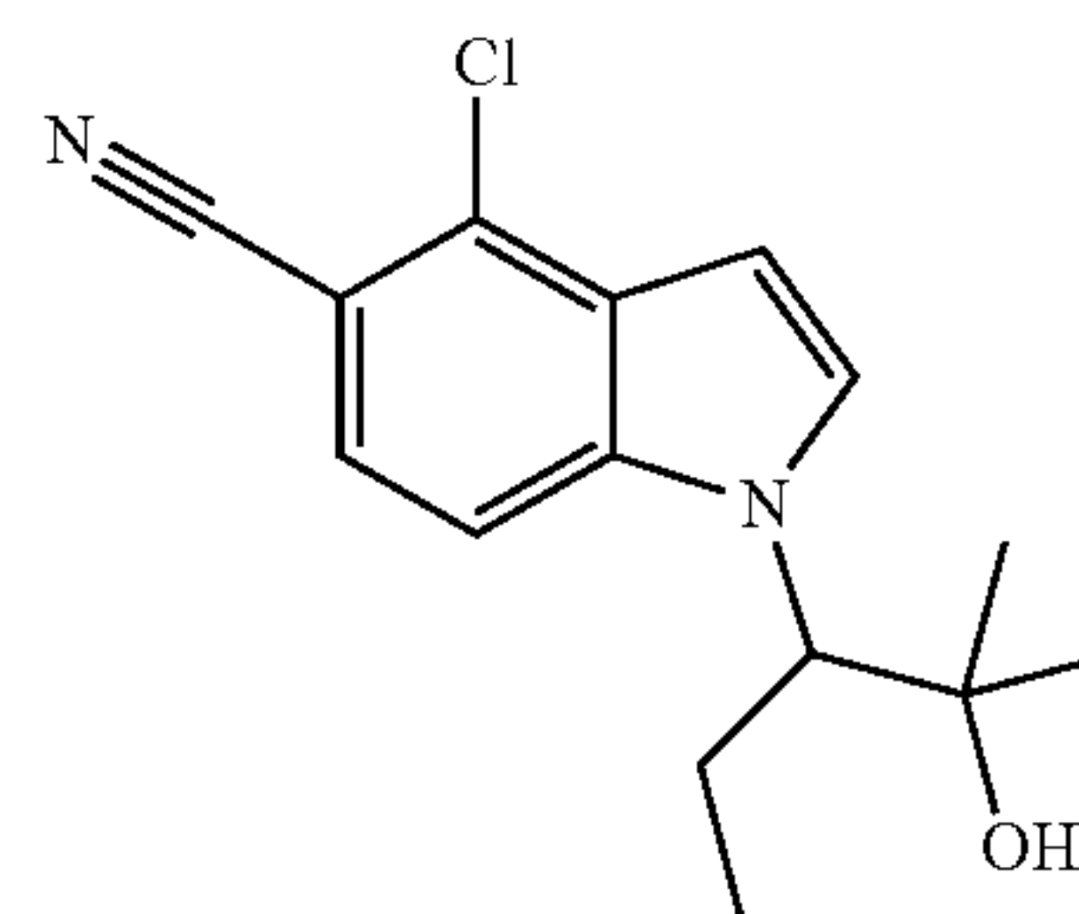
4-Chloro-1-(2-hydroxy-2-methylpentan-3-yl)-1H-indole-5-carbonitrile
