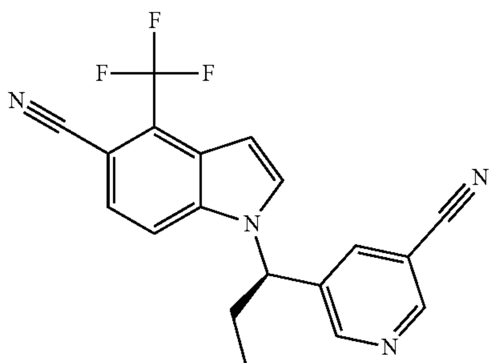
(R)-1-(1-(5-Cyanopyridin-3-yl)propyl)-4-(trifluoromethyl)-1H-indole-5-carbonitrile
