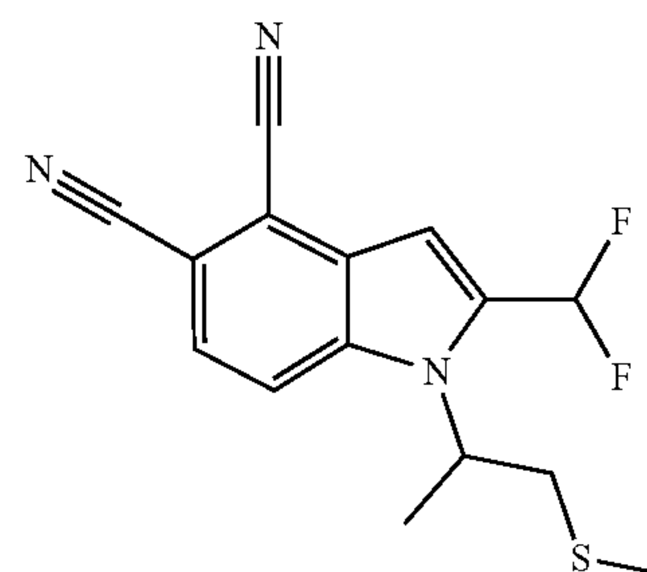
2-(Difluoromethyl)-1-(1-(methylthio)propan-2-yl)-1H-indole-4,5-dicarbonitrile
