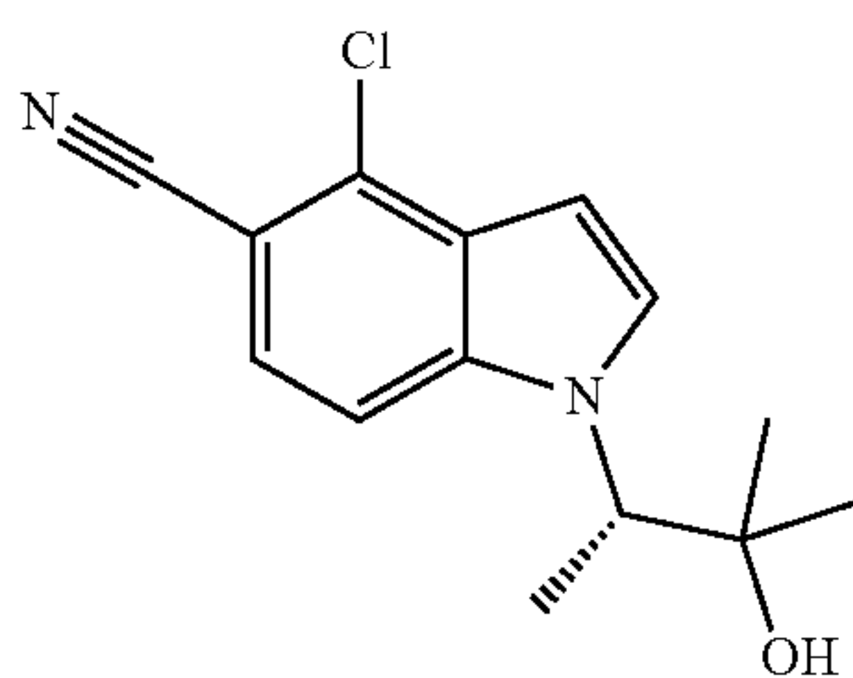
(S)-4-Chloro-1-(3-hydroxy-3-methylbutan-2-yl)-1H-indole-5-carbonitrile
