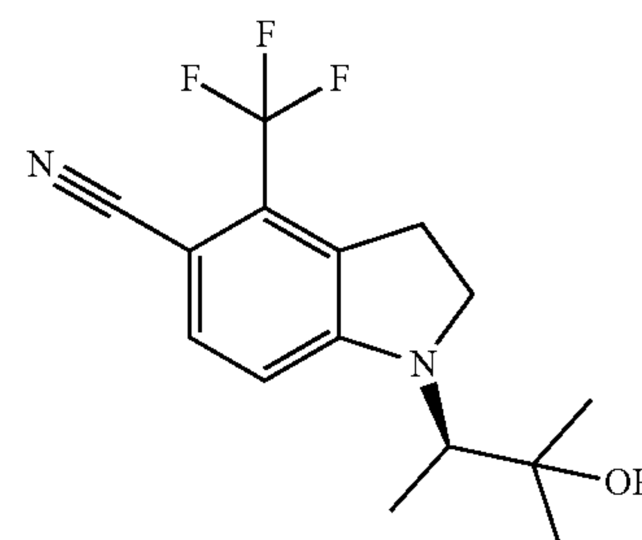
(R)-1-(3-Hydroxy-3-methylbutan-2-yl)-4-(trifluoromethyl)indoline-5-carbonitrile
