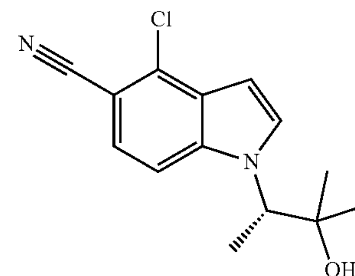
C. (S)-4-Chloro-1-(3-hydroxy-3-methylbutan-2-yl)-1H-indole-5-carbonitrile
