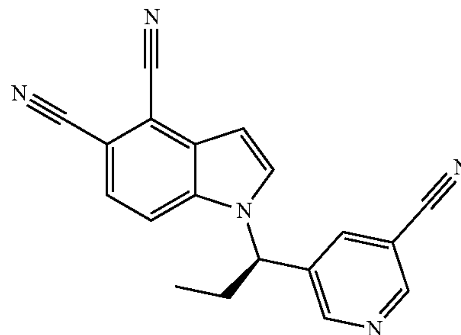
B. (R)-1-(1-(5-Cyanopyridin-3-yl)propyl)-1H-indole-4,5-dicarbonitrile
