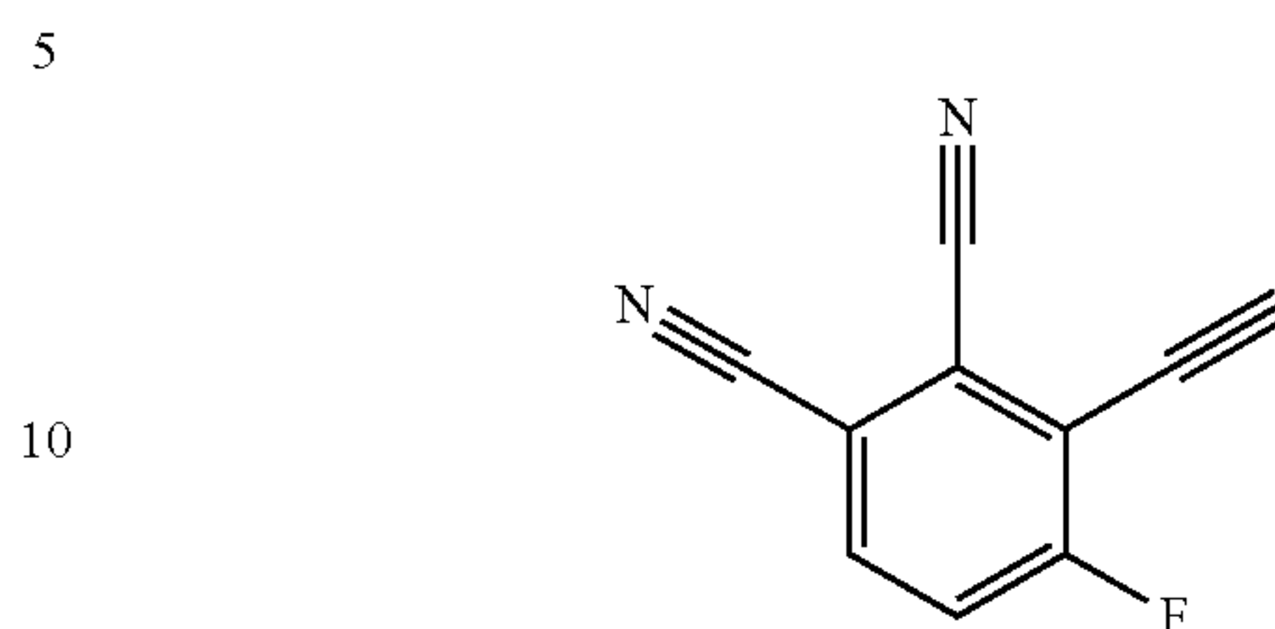
A. 3-Ethynyl-4-fluorophthalonitrile
