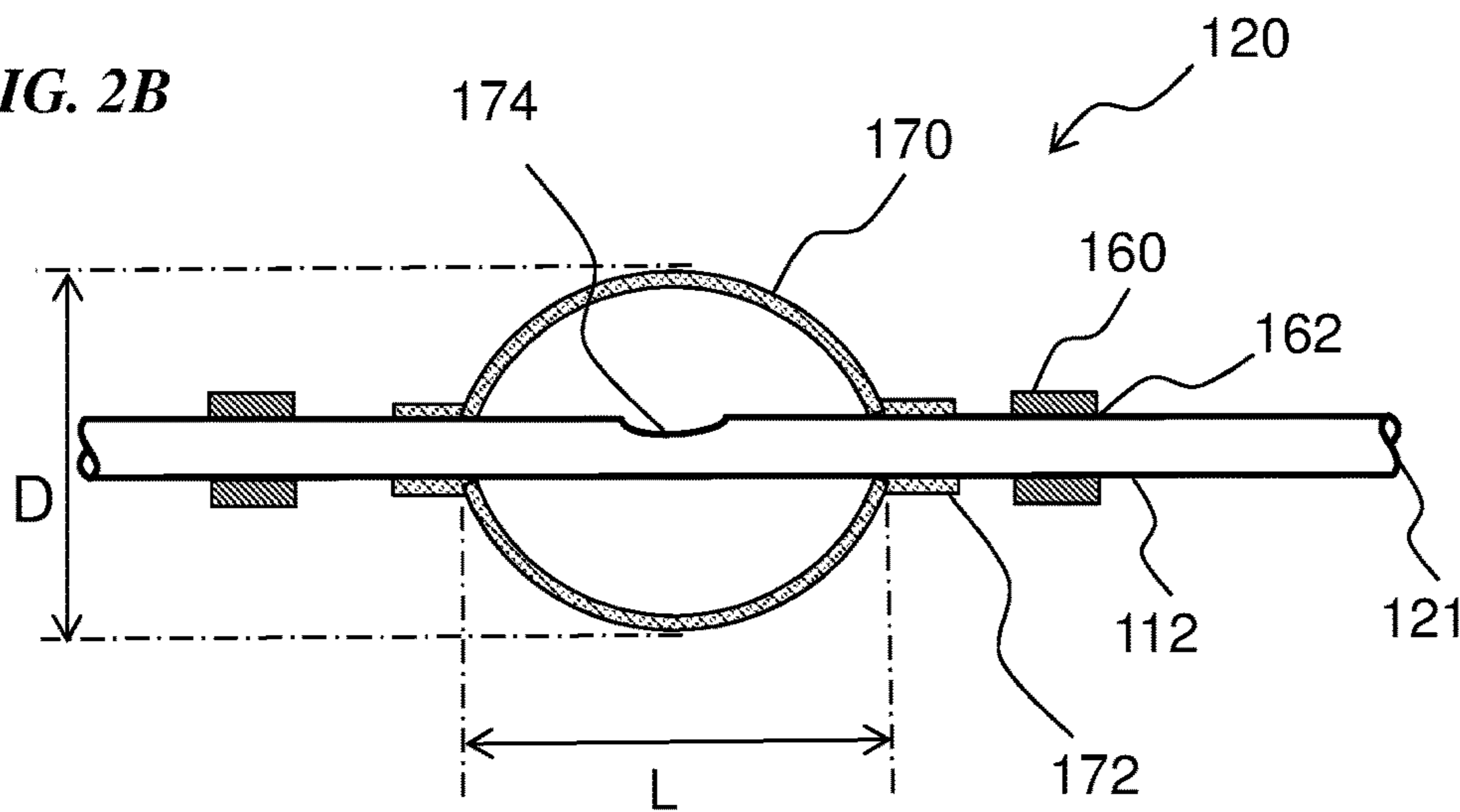
SECTION 2B-2B OF FIG. 1B
