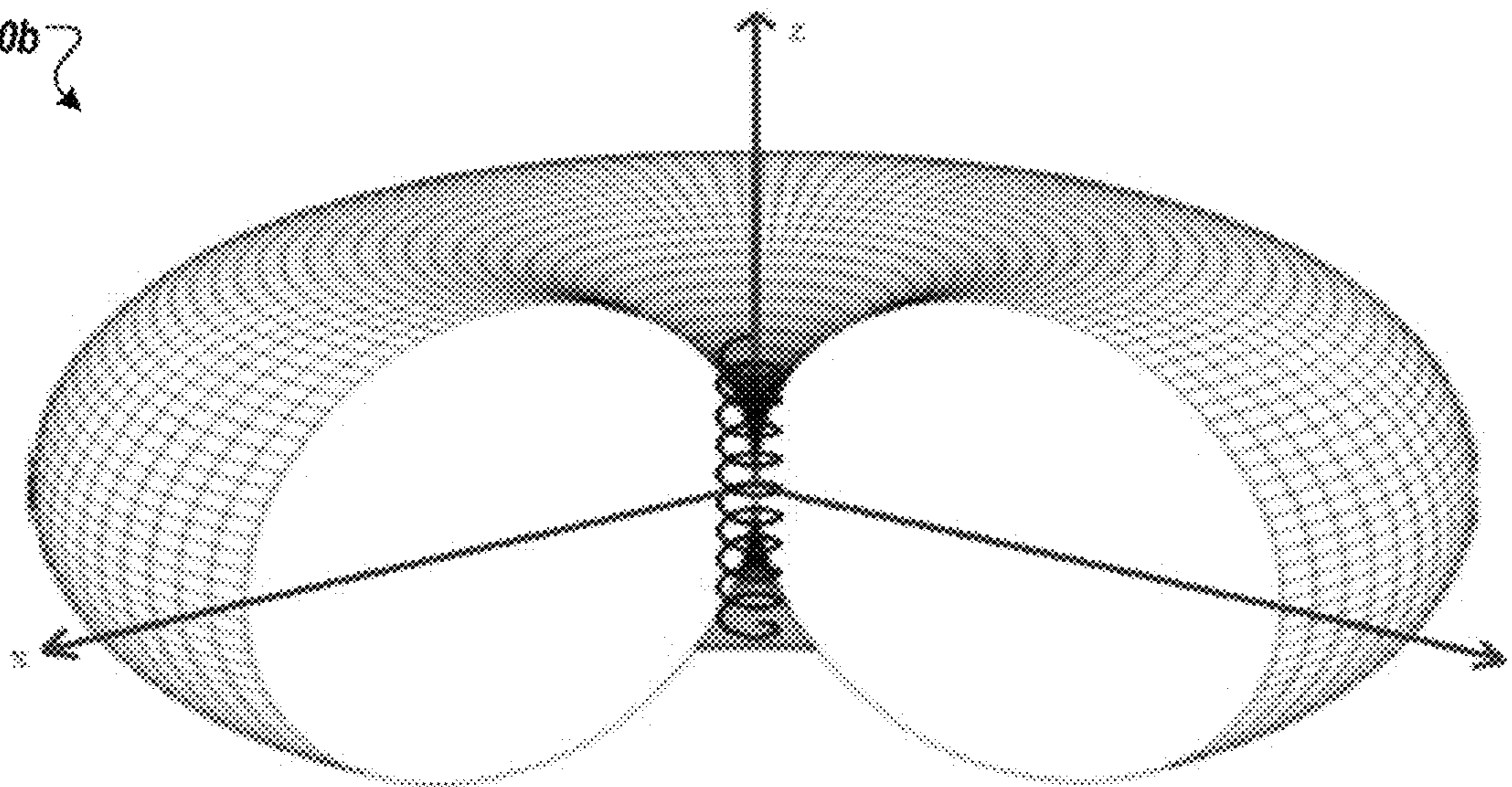
Helical antenna in normal mode
