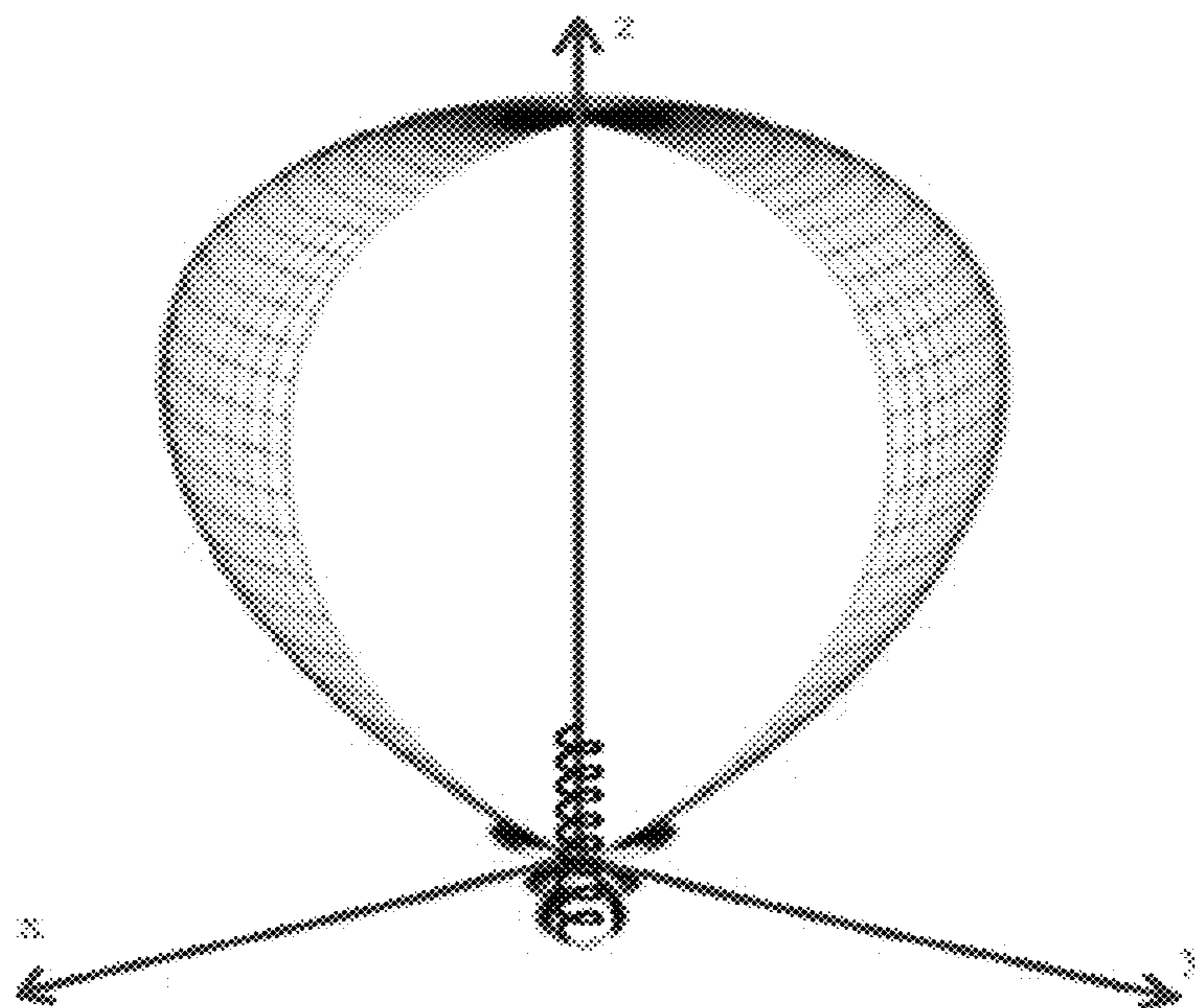
Helical antenna in endfire mode
