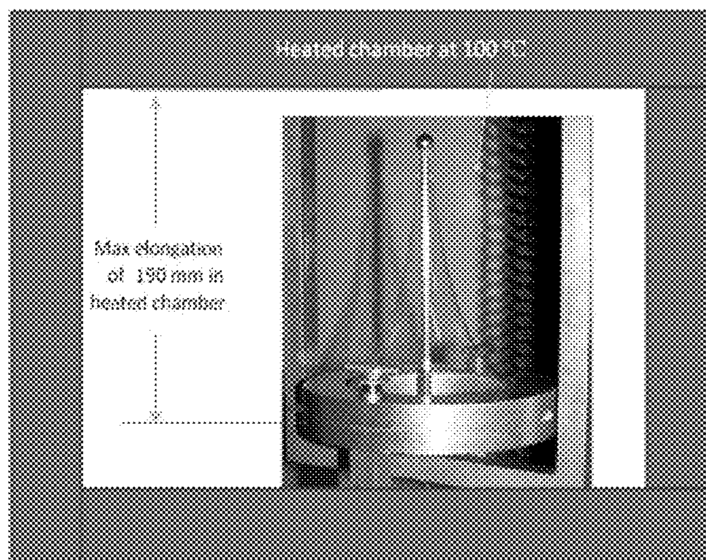
Puncture test at 100°C used to simulate high temperature deformation and film drawdown.
