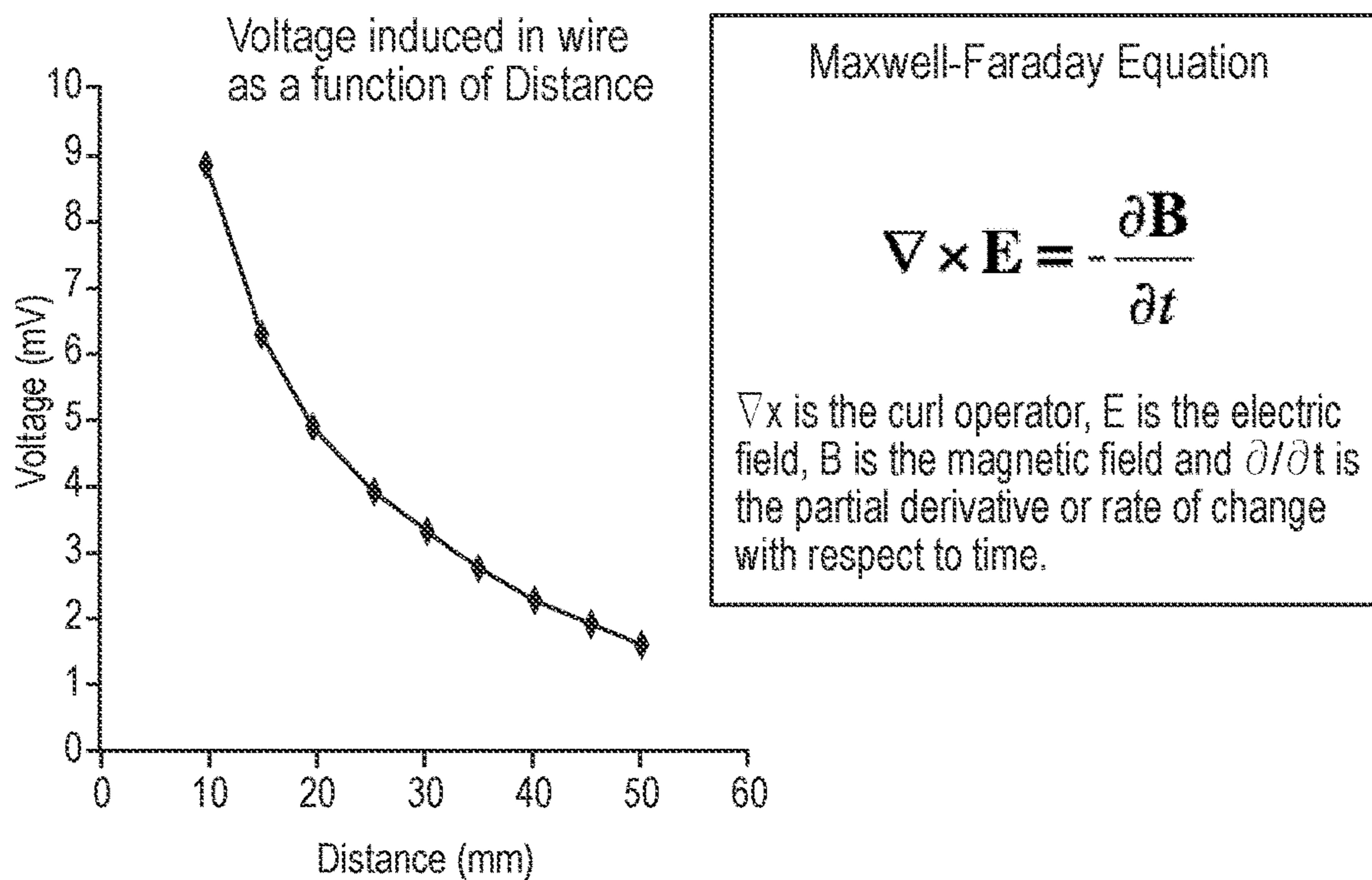
FIG. 4 (Prior Art)
