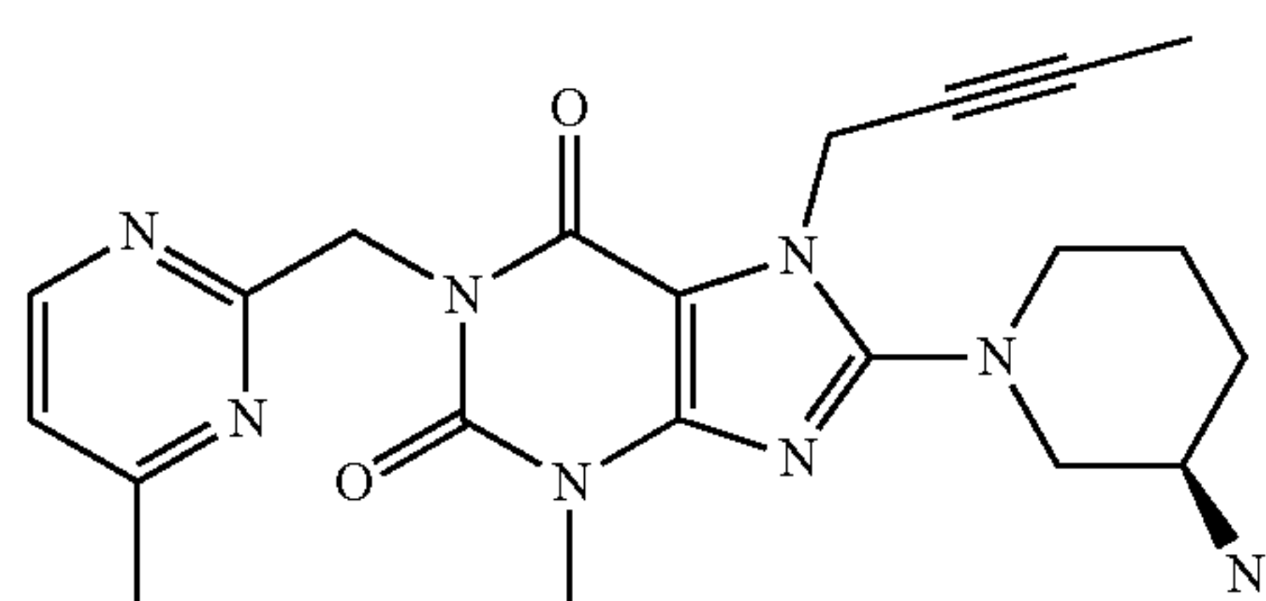
1-[(4,6-dimethyl-pyrimidin-2-yl)methyl]-3-methyl-7-(2-butyn-1-yl)-8-((R)-3-amino-piperidin-1-yl)-xanthine (cf. WO 2005/085246, Example 1(82)):
