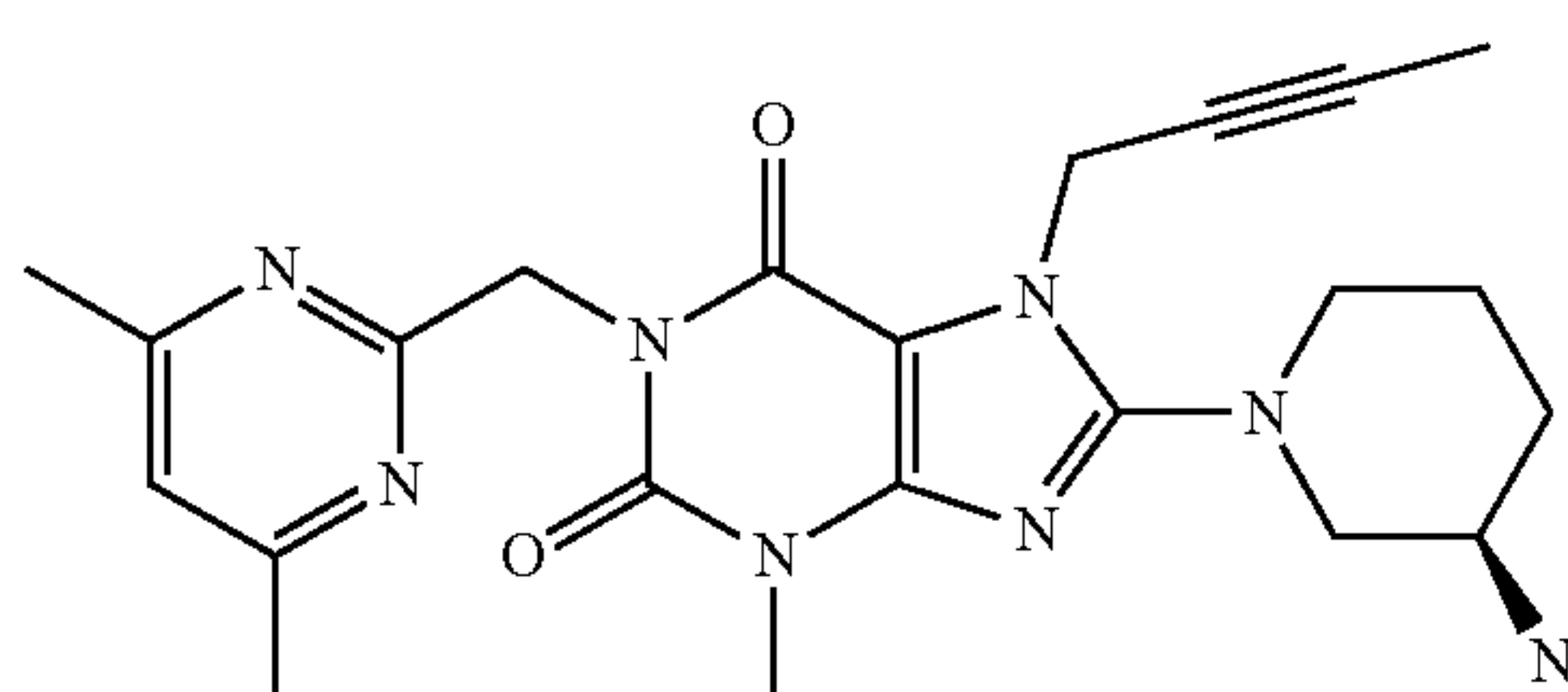
1-[(4,6-dimethyl-pyrimidin-2-yl)methyl]-3-methyl-7-(2-butyn-1-yl)-8-((R)-3-amino-piperidin-1-yl)-xanthine (cf. WO 2005/085246, Example 1(82)):
