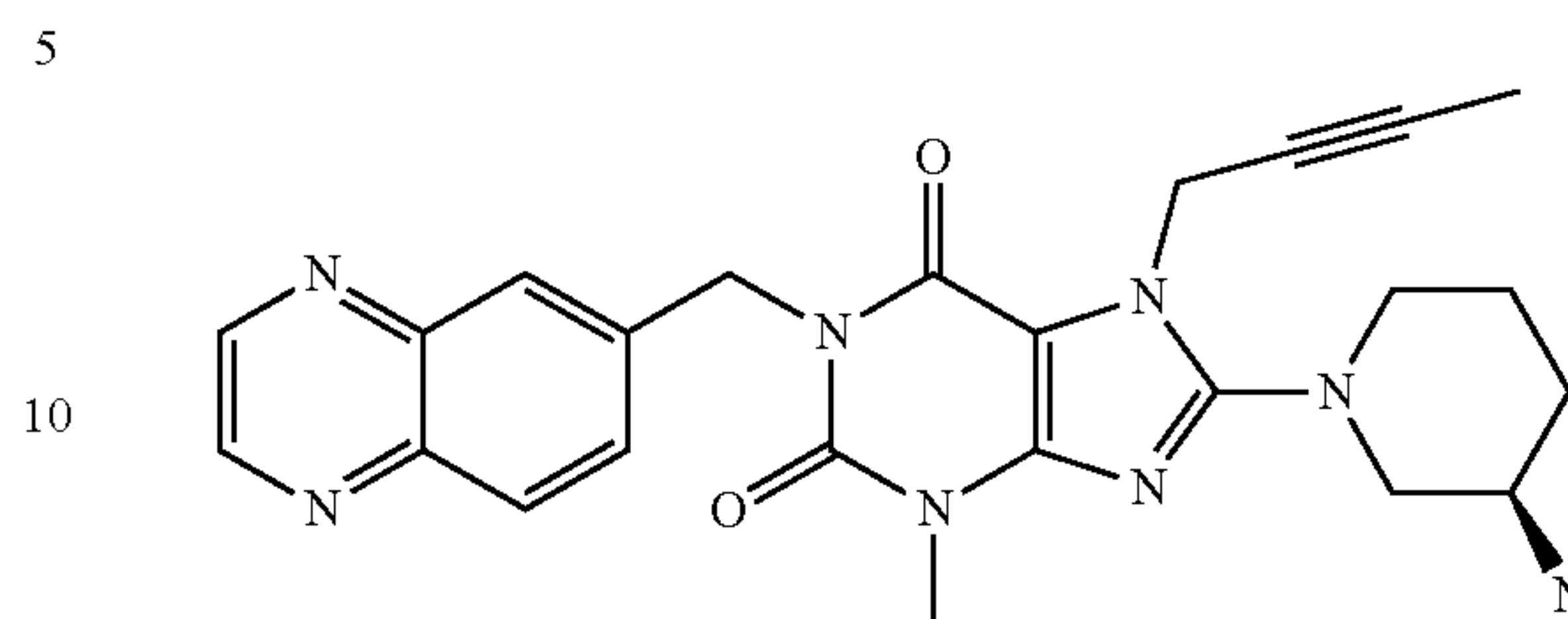
1-[(quinoxalin-6-yl)methyl]-3-methyl-7-(2-butyn-1-yl)-8-((R)-3-amino-piperidin-1-yl)-xanthine (cf. WO 2005/085246, Example 1(83)):
