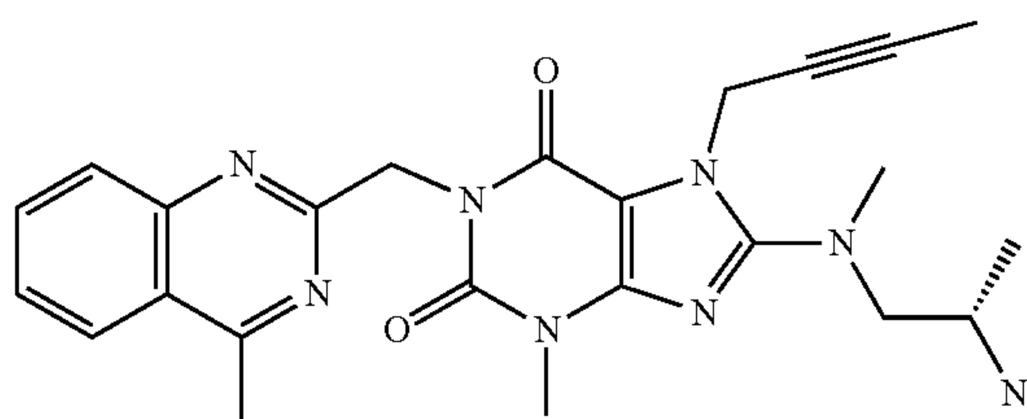
1-[(3-cyano-pyridin-2-yl)methyl]-3-methyl-7-(2-butyn-1-yl)-8-((R)-3-amino-piperidin-1-yl)-xanthine (cf. WO 2005/085246, Example 1(52)):
