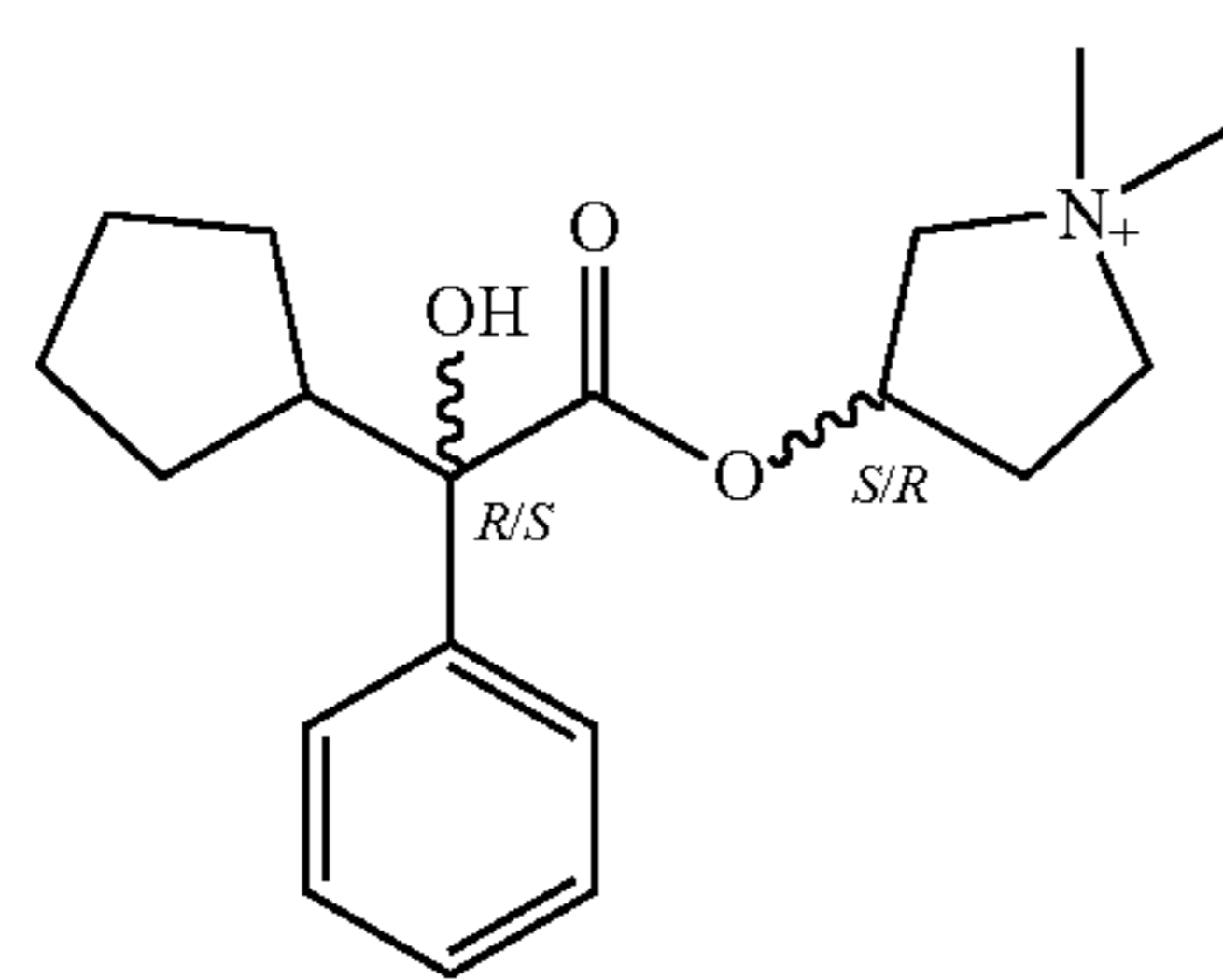
Glycopyrronium tosylate (threo pair) FW = 489.62
