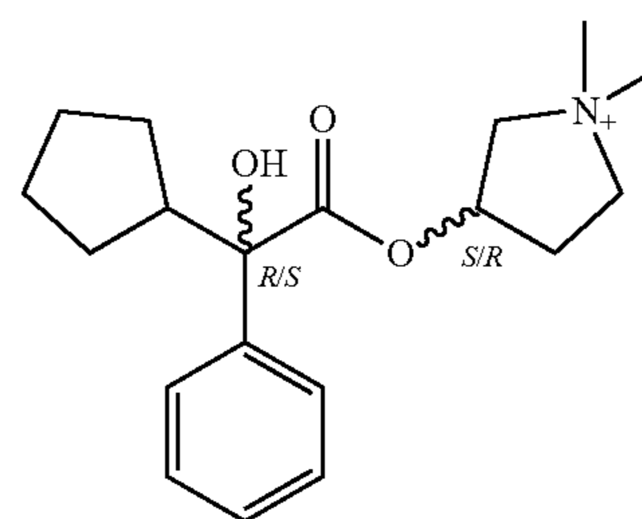
Glycopyrronium tosylate monohydrate (threo pair) FW = 507.64
