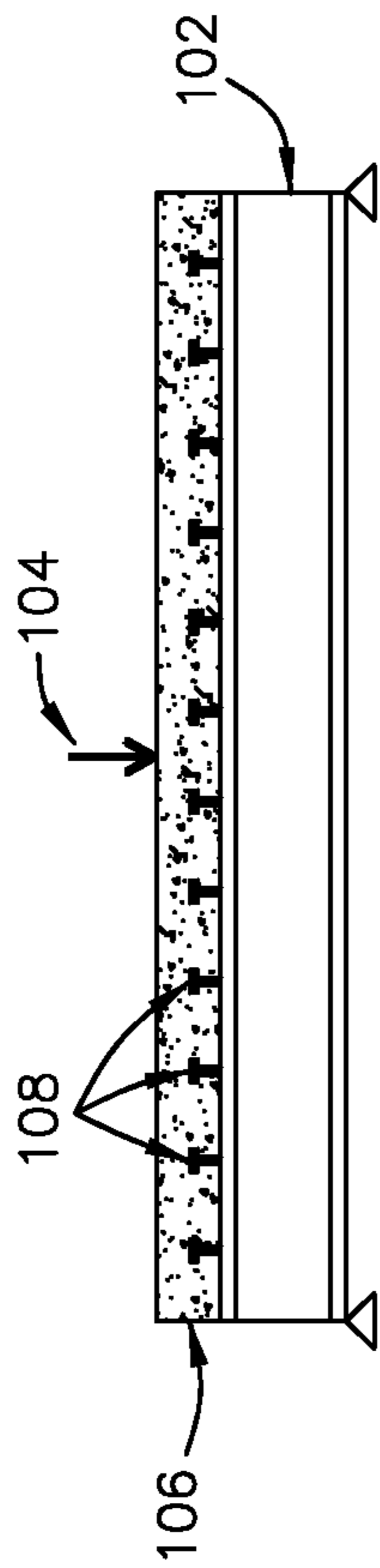
Fig. 1A (Prior Art)
