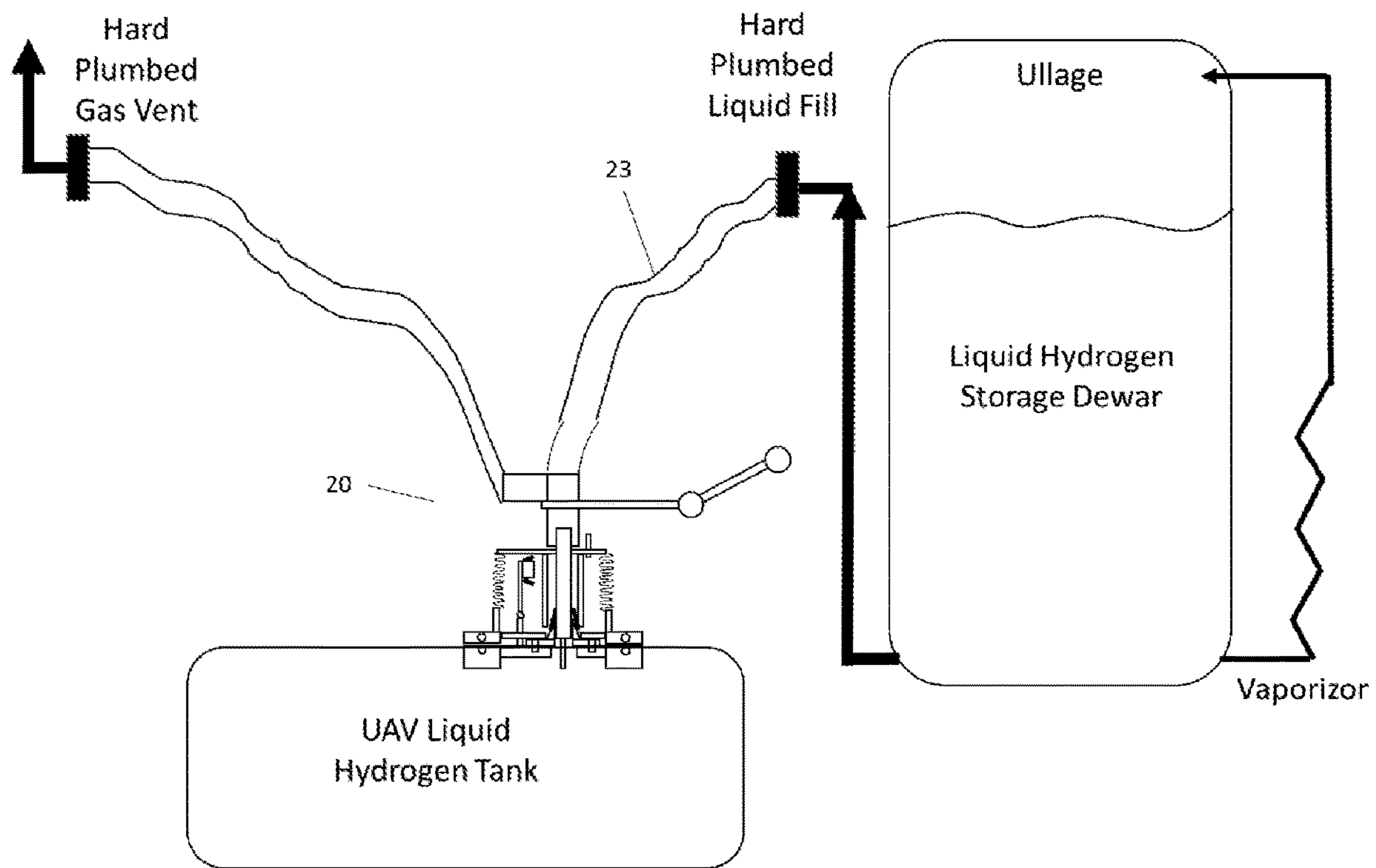
Nozzles Inserted into Tank Figure 13D
