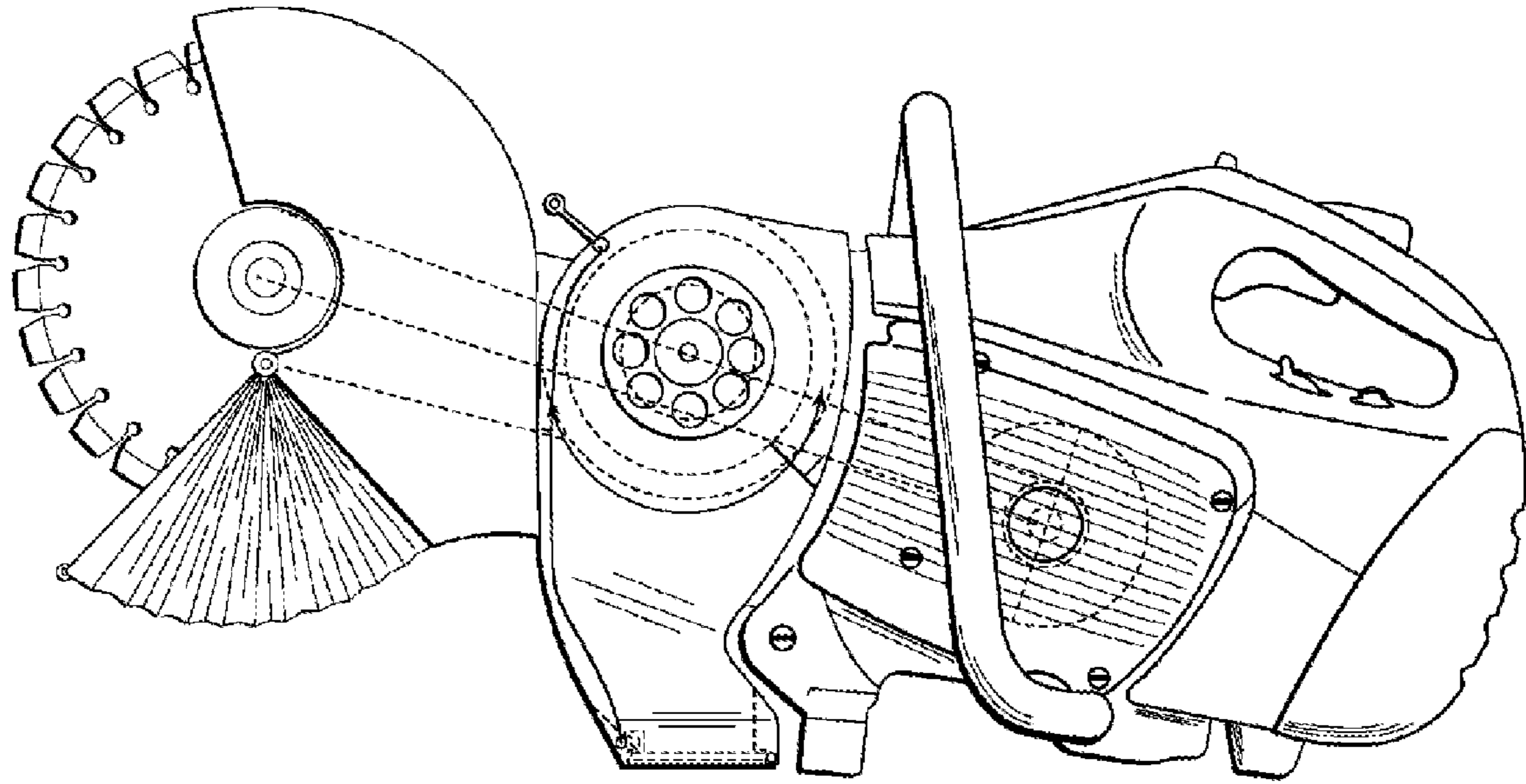
FIG. 1 (PRIOR ART)
