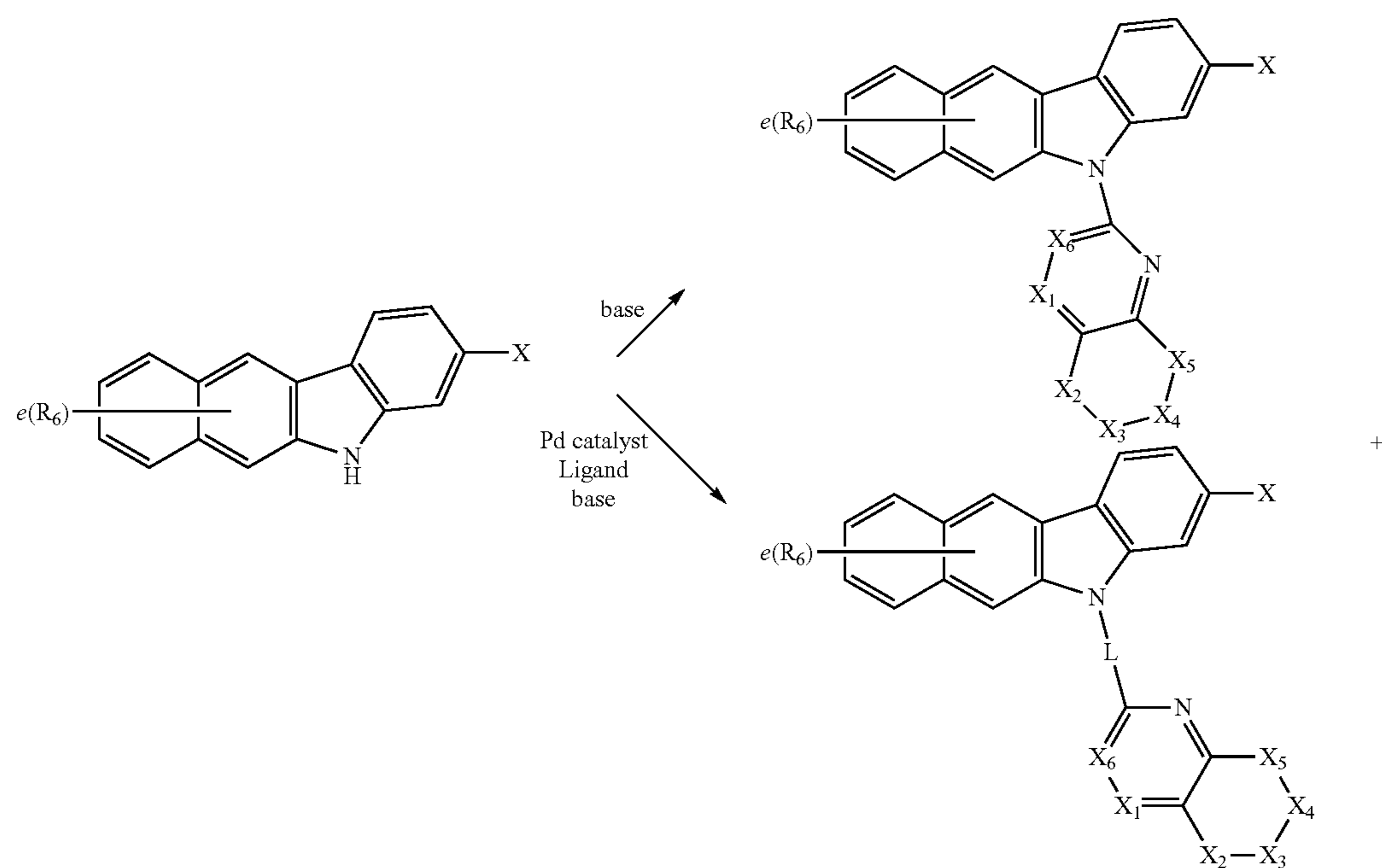
[Reaction Scheme 4]
