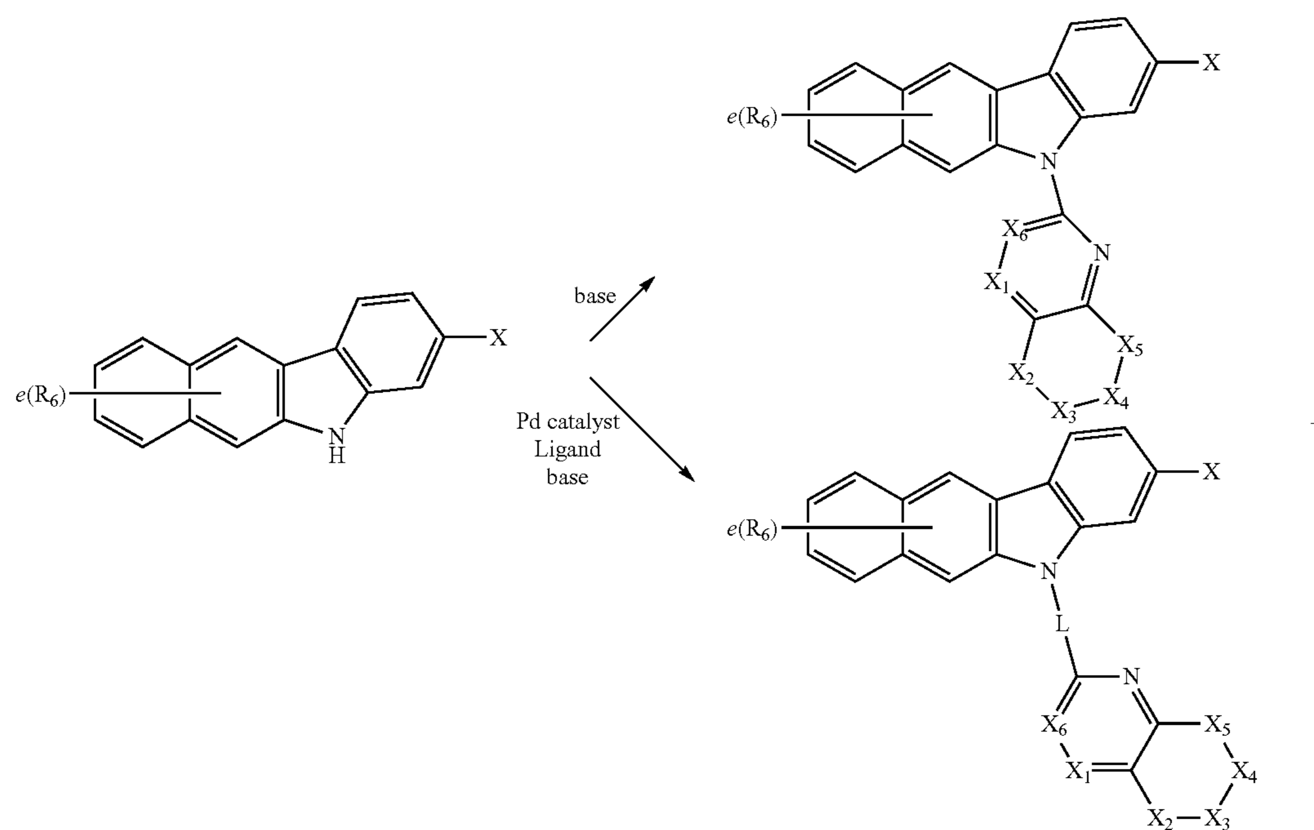
[Reaction Scheme 4]
