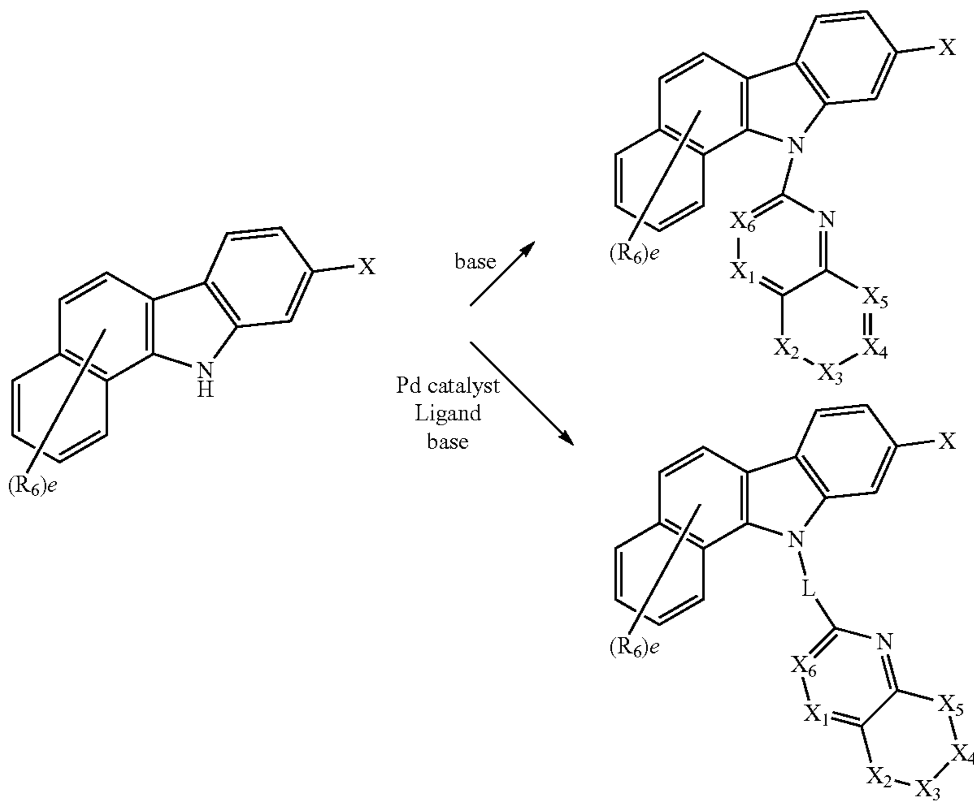
[Reaction Scheme 2]
