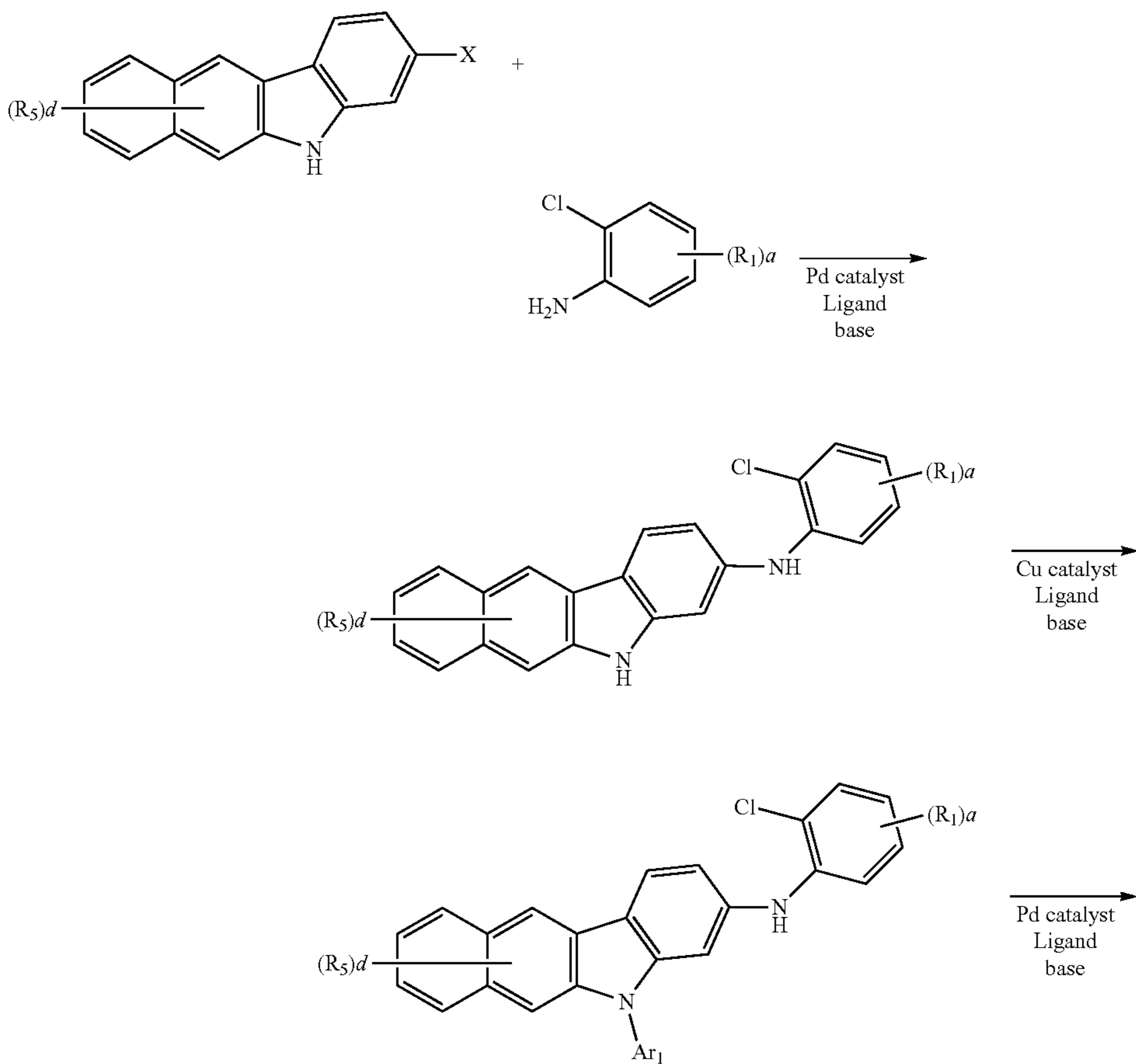
[Reaction Scheme 3]
