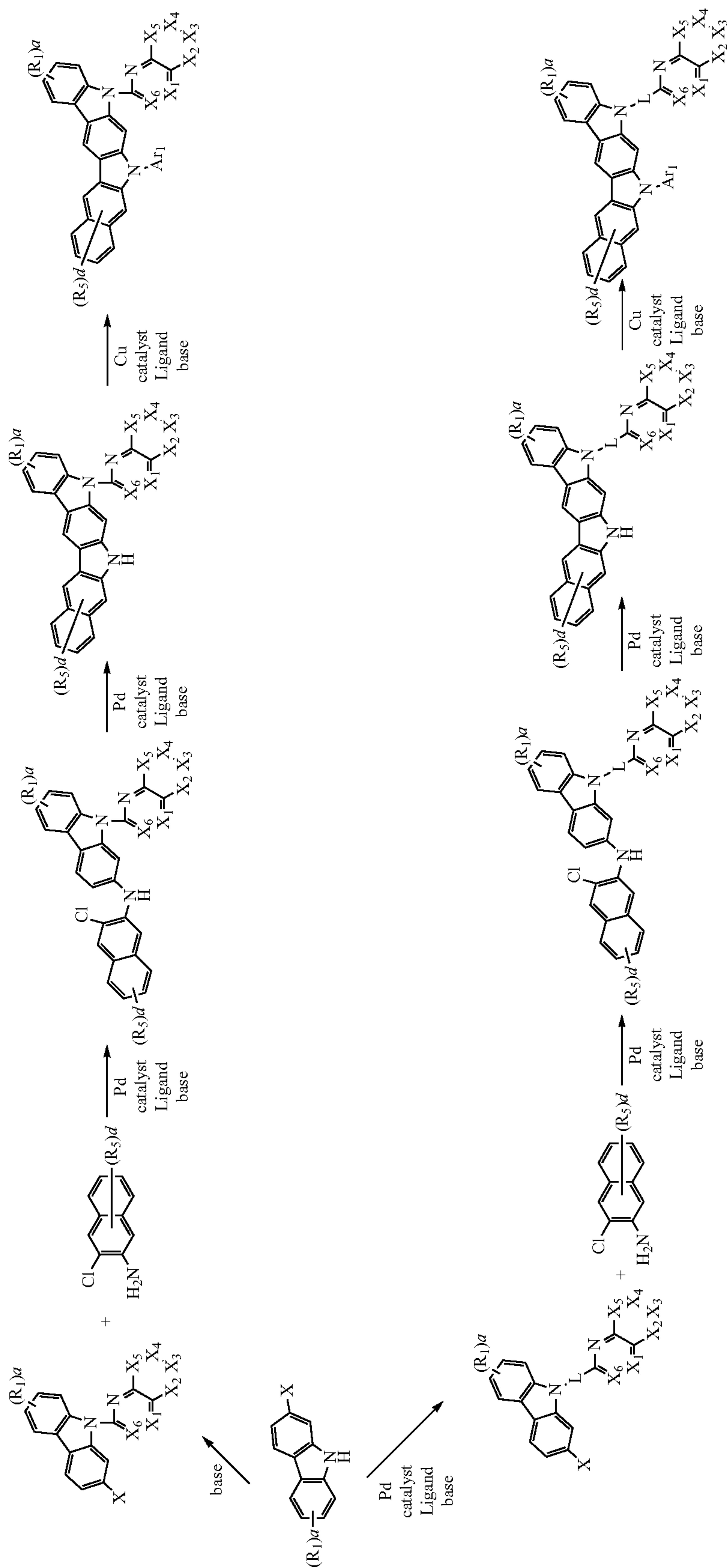
[Reaction Scheme 5]
