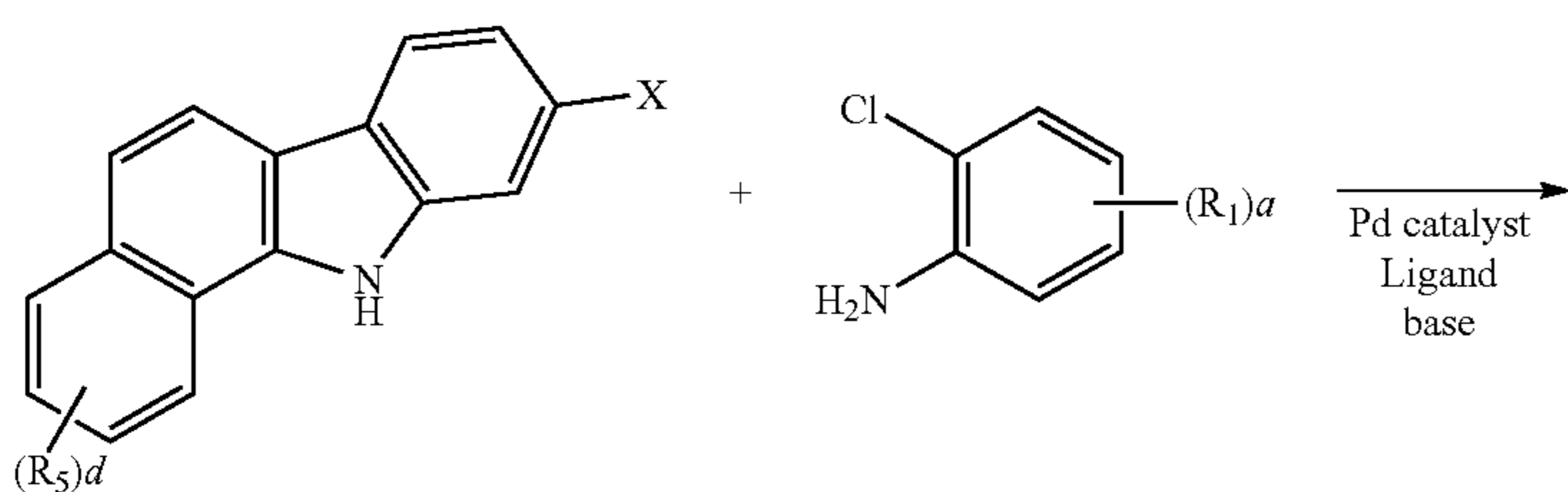
[Reaction Scheme 1]
