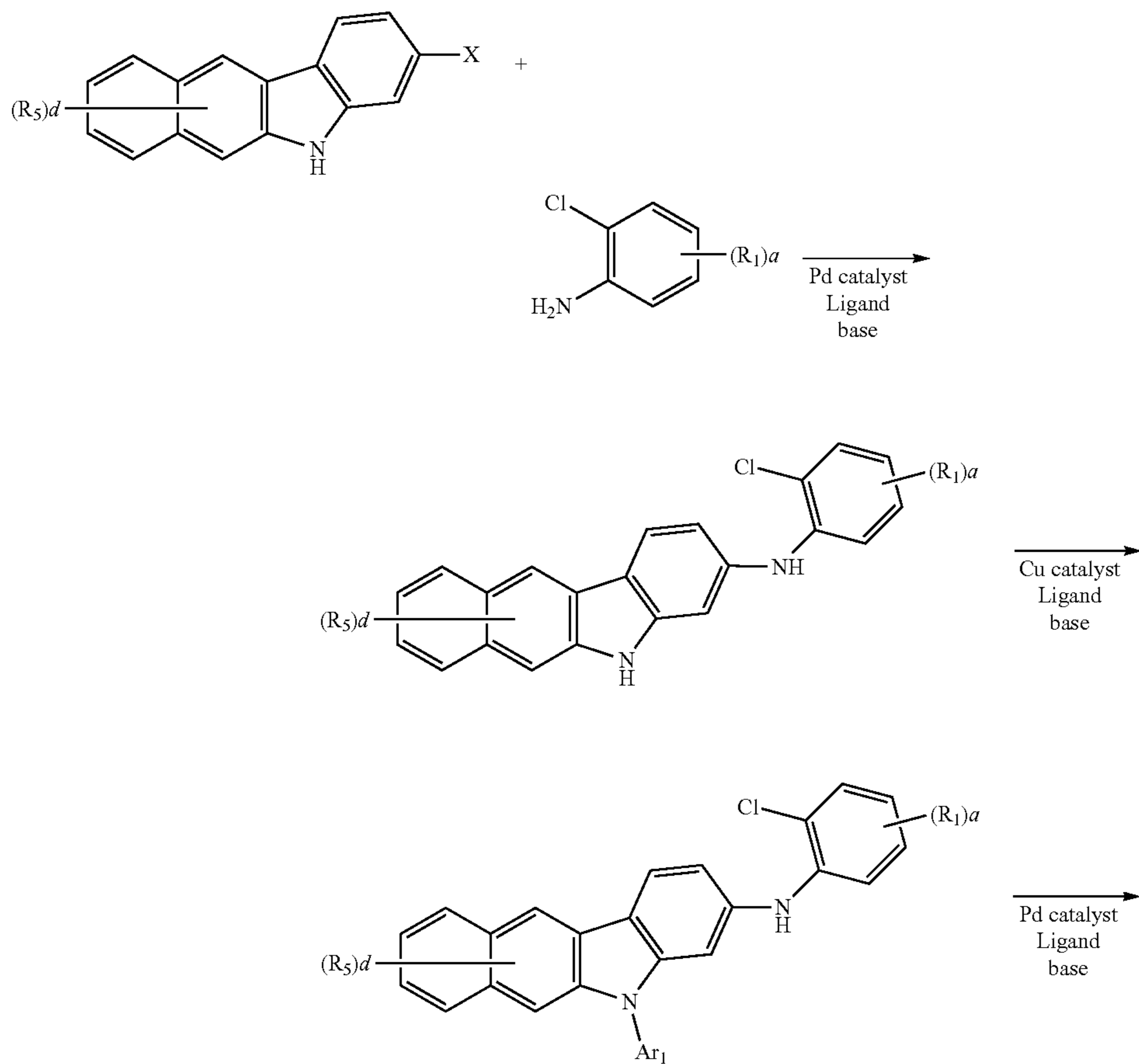
[Reaction Scheme 3]
