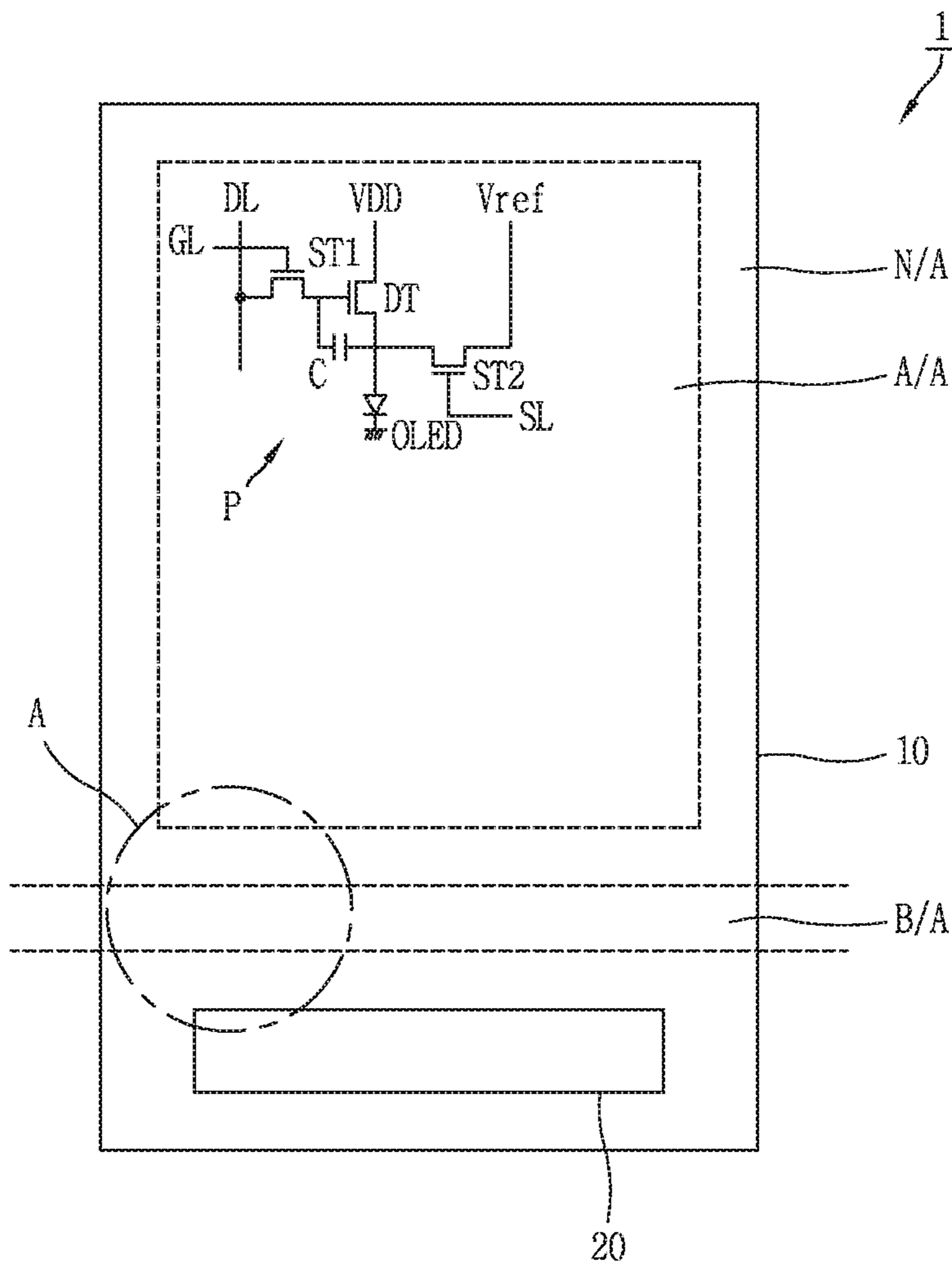
FIG. 1 RELATED ART
