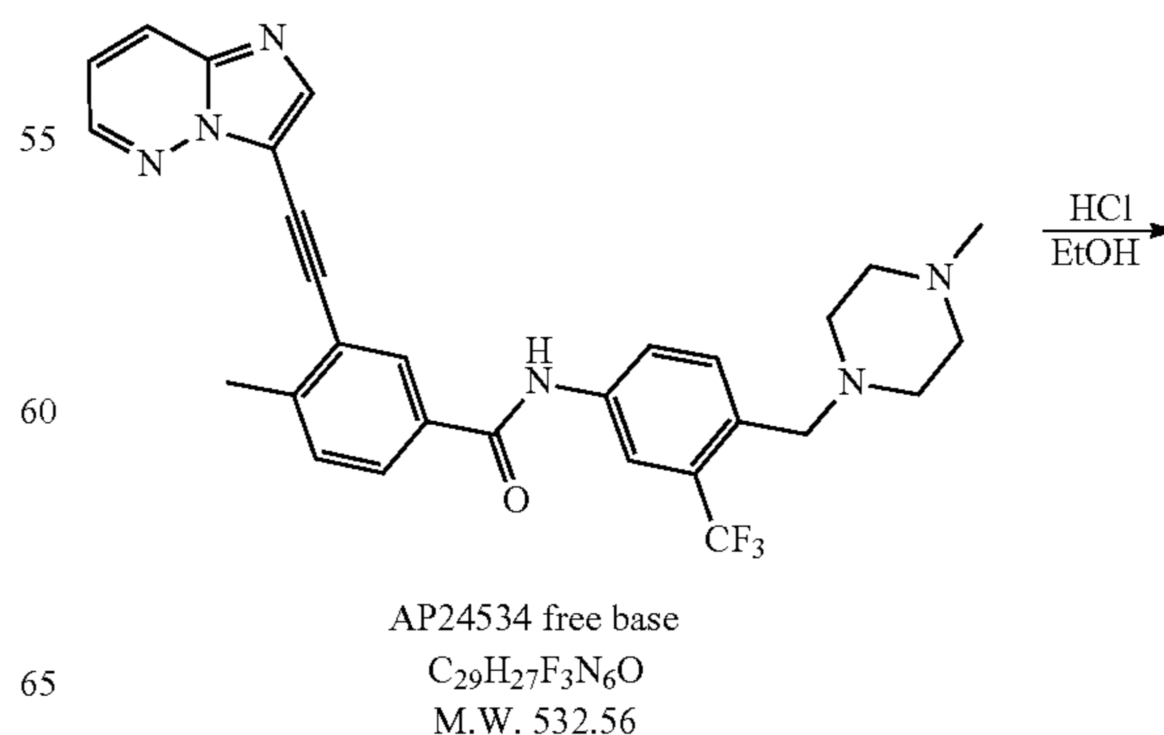
Scheme 5: Step 4 - Synthesis of Ponatinib HCl
