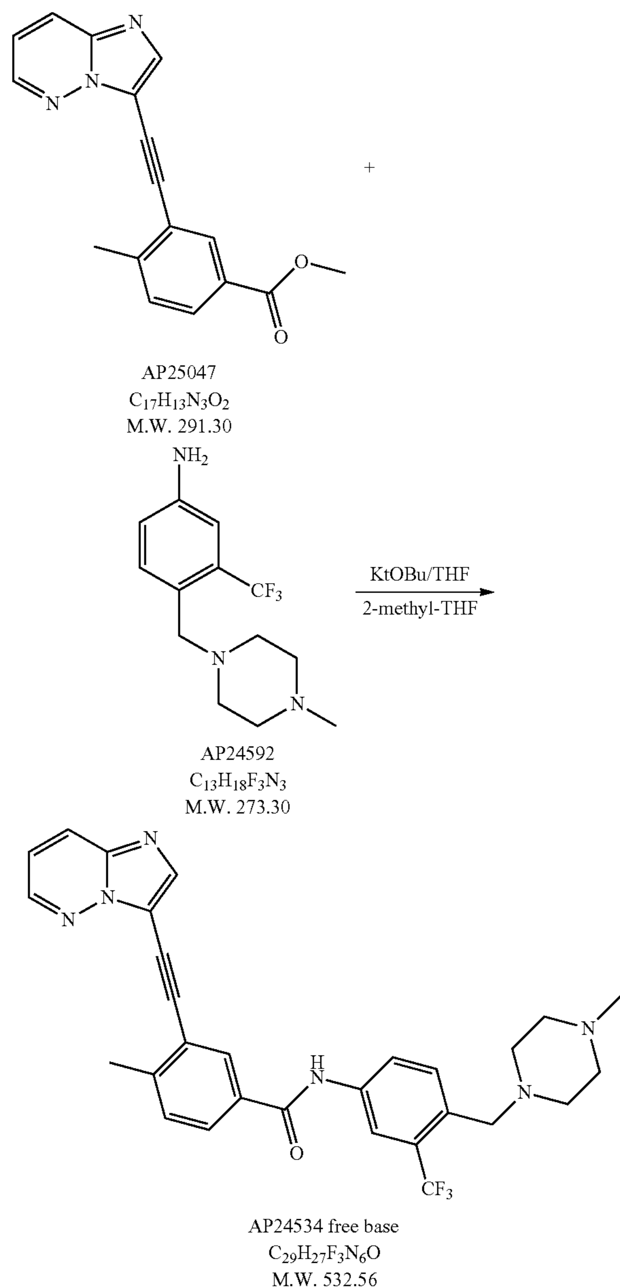
Scheme 4: Step 3-Synthesis of AP24534 Free Base
