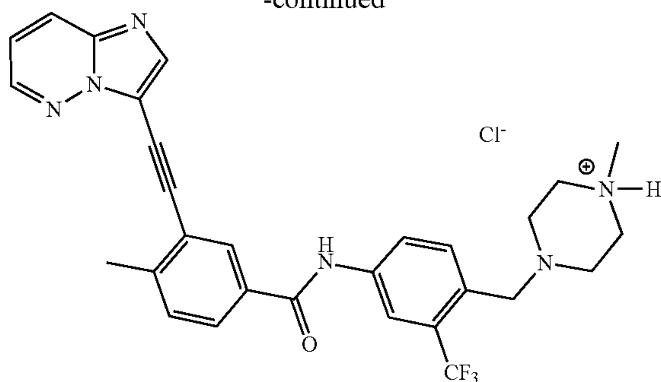
ponatinib HCl drug substance
