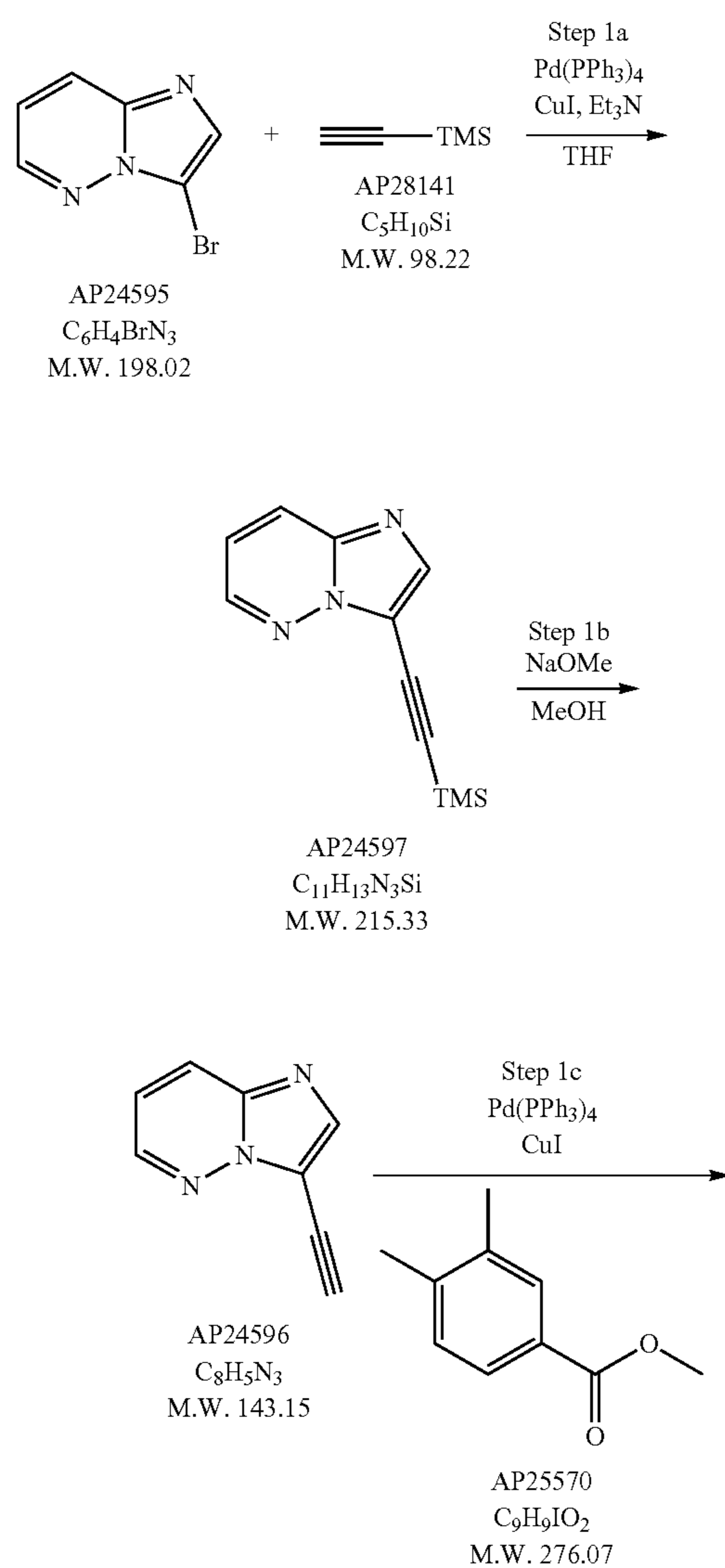
Scheme 2: Step 1-Synthesis of AP25047
