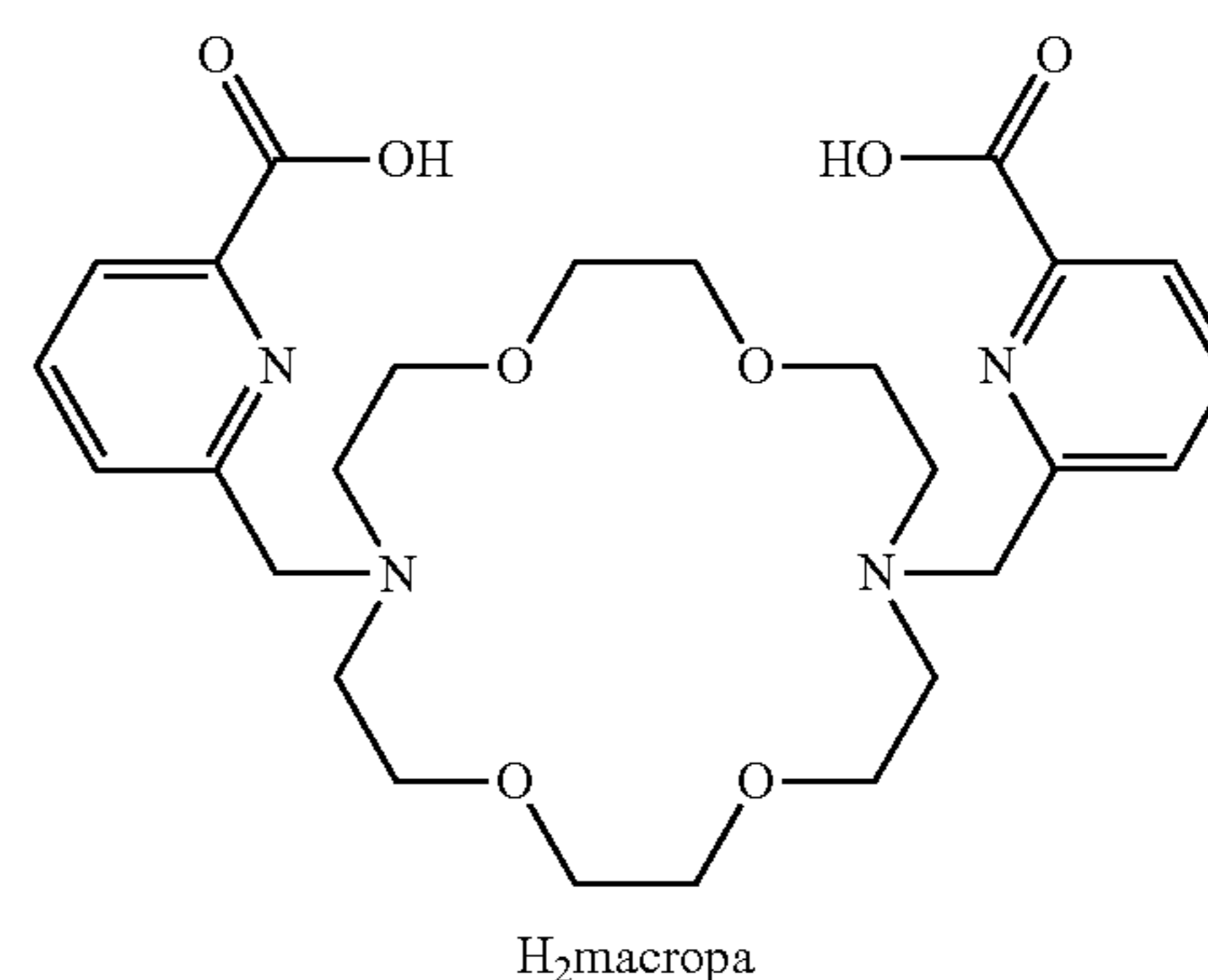
Scheme 1. Structures of \text{H}_2\text{macropa} , \text{H}_2\text{macropa-NCS} ("macropa-ncs"), and \text{macropa-(OCH}_2\text{CH}_2\text{)-Ph-NCS} .
