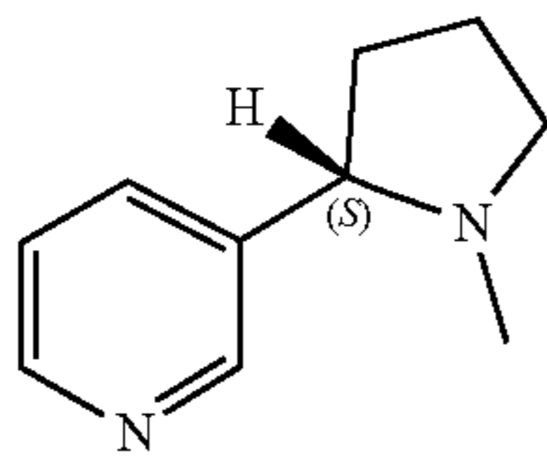
(S)-Nicotine
