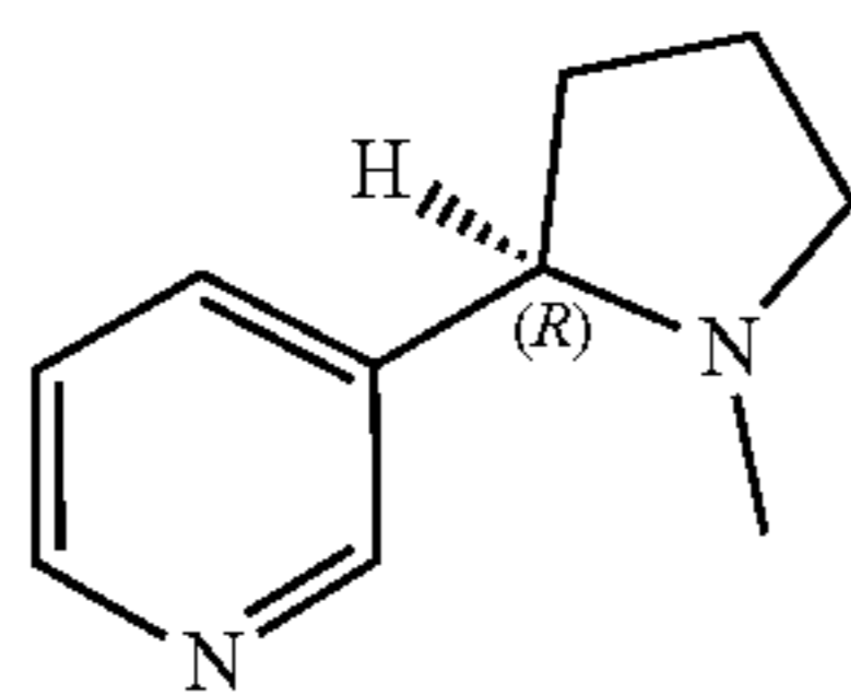
(R)-Nicotine
