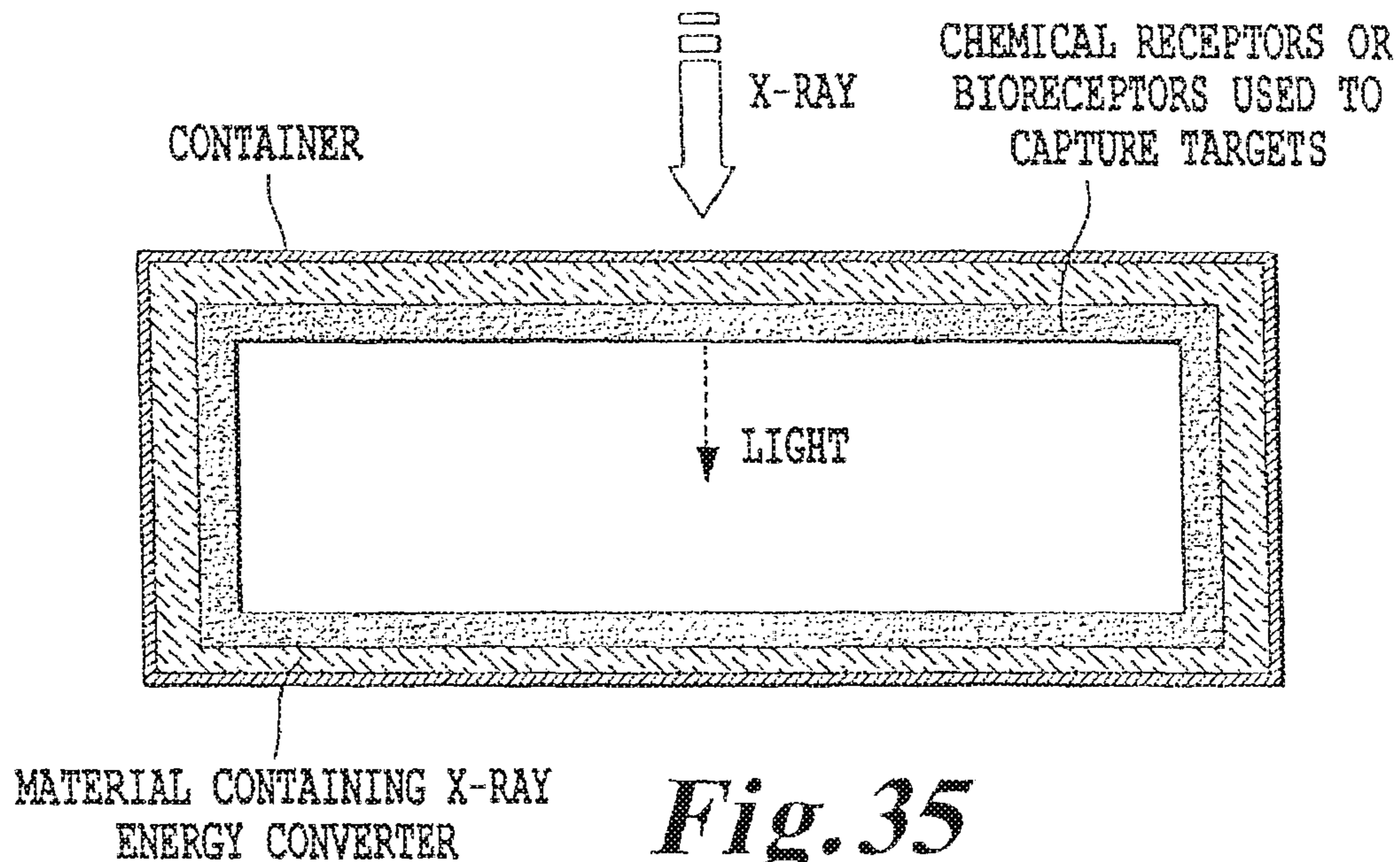
STERILIZATION SYSTEM 9 WITH CHEMICAL RECEPTORS OR BIORECEPTORS
