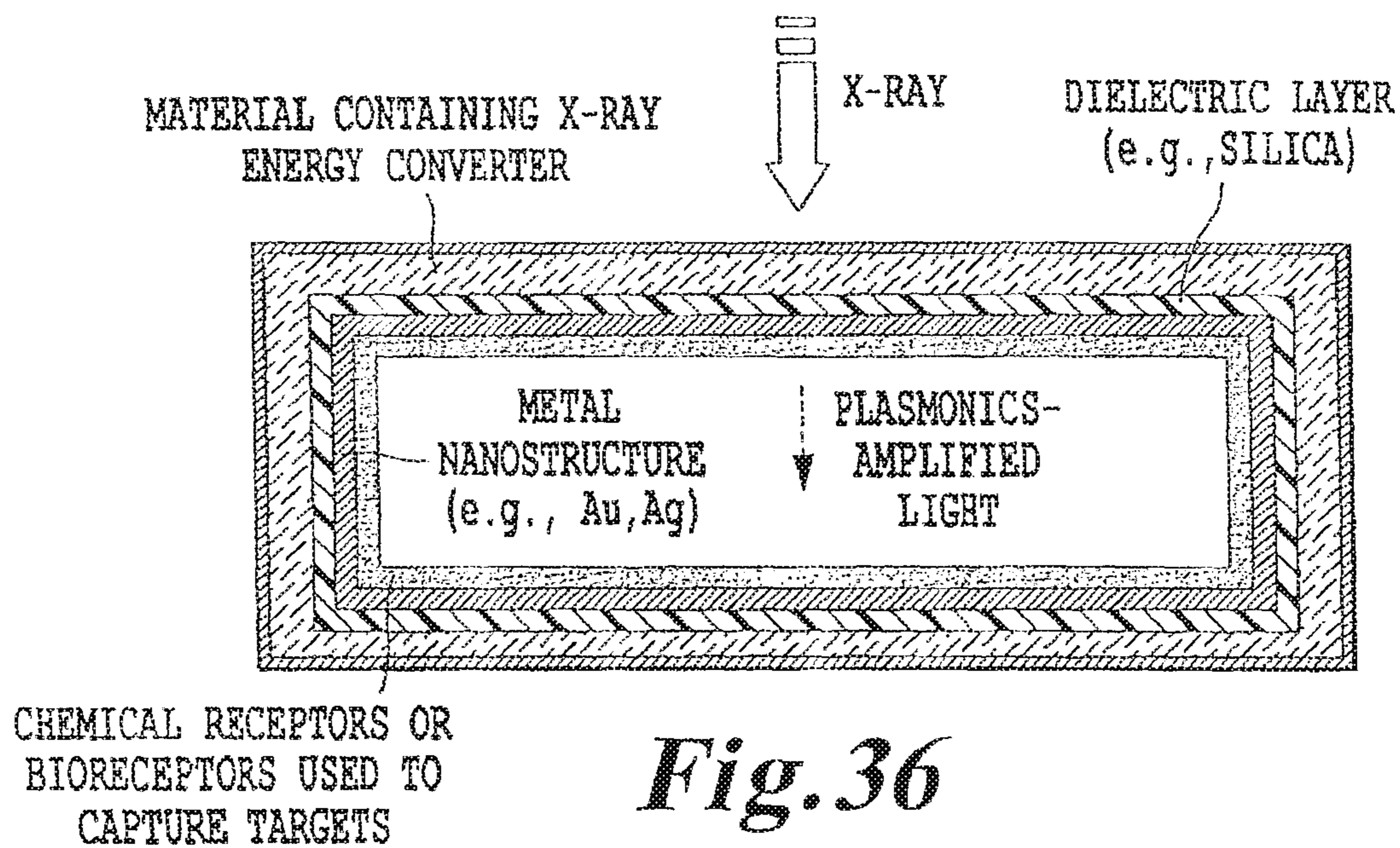
STERILIZATION SYSTEM 10 WITH PLASMONICS AND CHEMICAL RECEPTORS OR BIORECEPTORS
