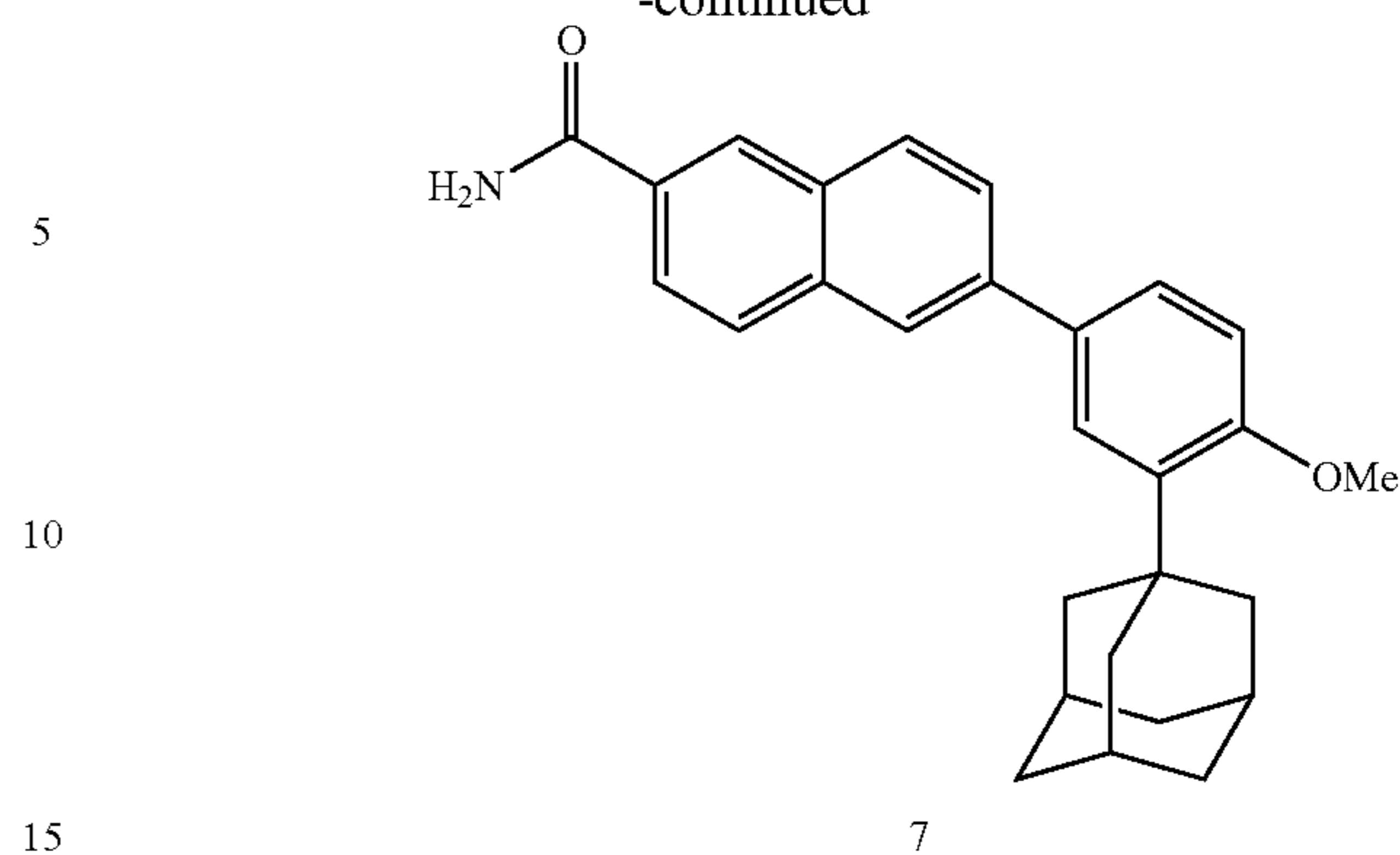
6-(3-(adamantan-1-yl)-4-methoxyphenyl)-2-naphthamide (7)
