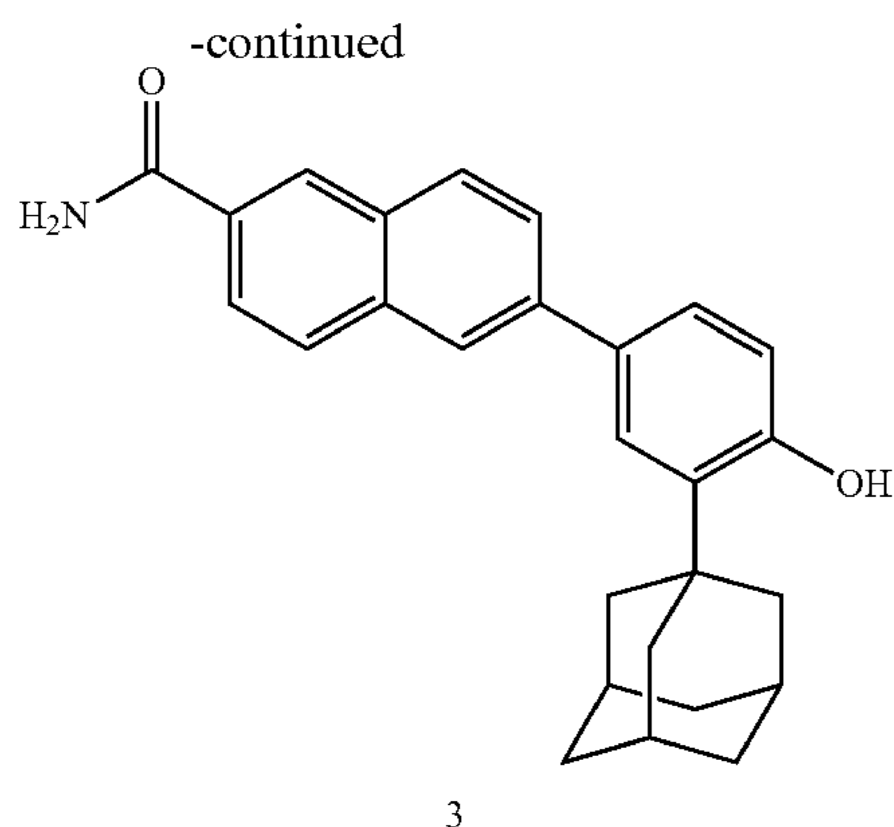
6-(3-(adamantan-1-yl)-4-hydroxyphenyl)-2-naphthamide (3)
