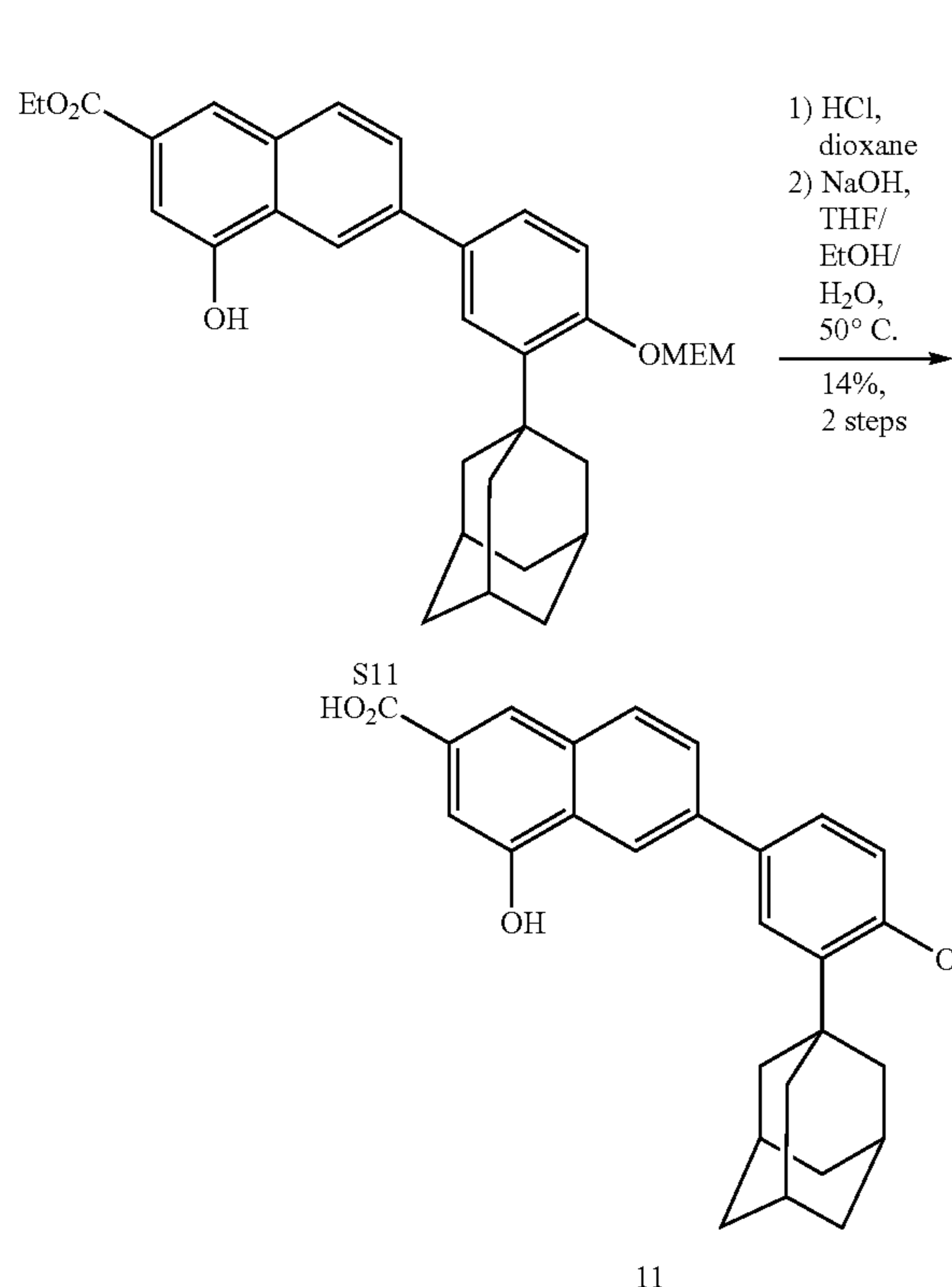
6-(3-(adamantan-1-yl)-4-hydroxyphenyl)-4-hydroxy-2-naphthoic acid (11)
