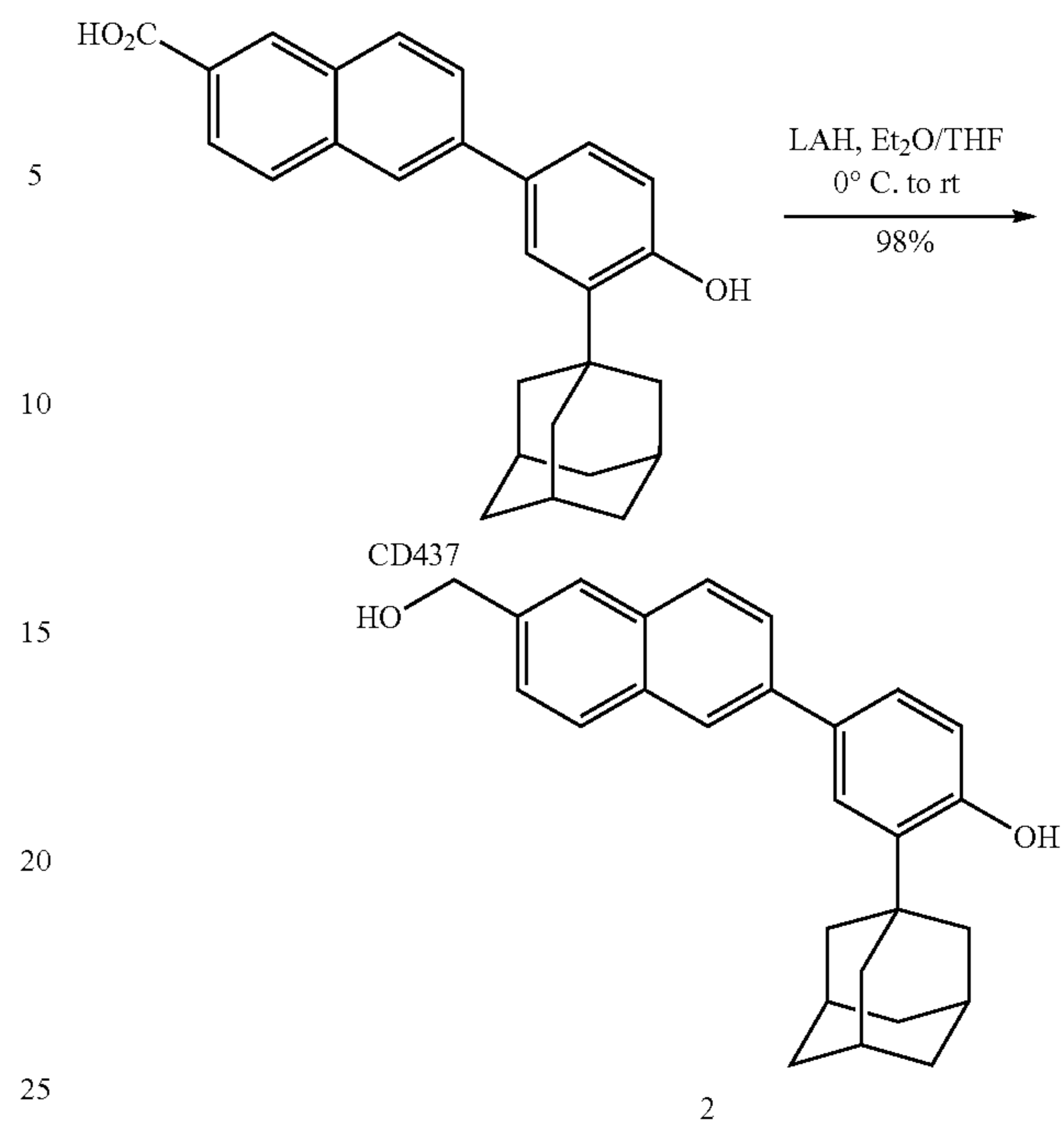
2-(adamantan-1-yl)-4-(6-(hydroxymethyl)naphthalen-2-yl)phenol (2)
