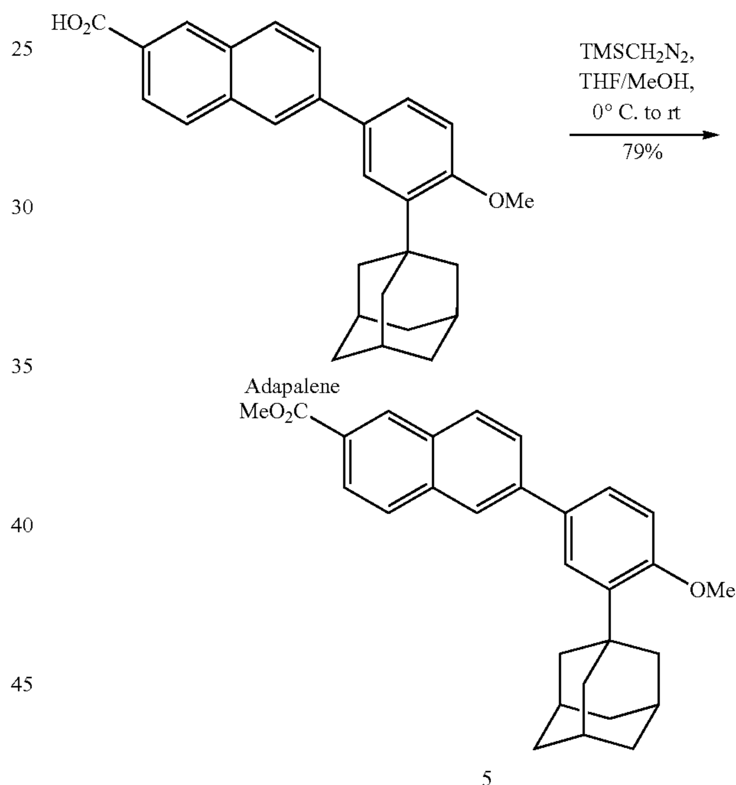
Methyl 6-(3-(adamantan-1-yl)-4-methoxyphenyl)-2-naphthoate (5)
