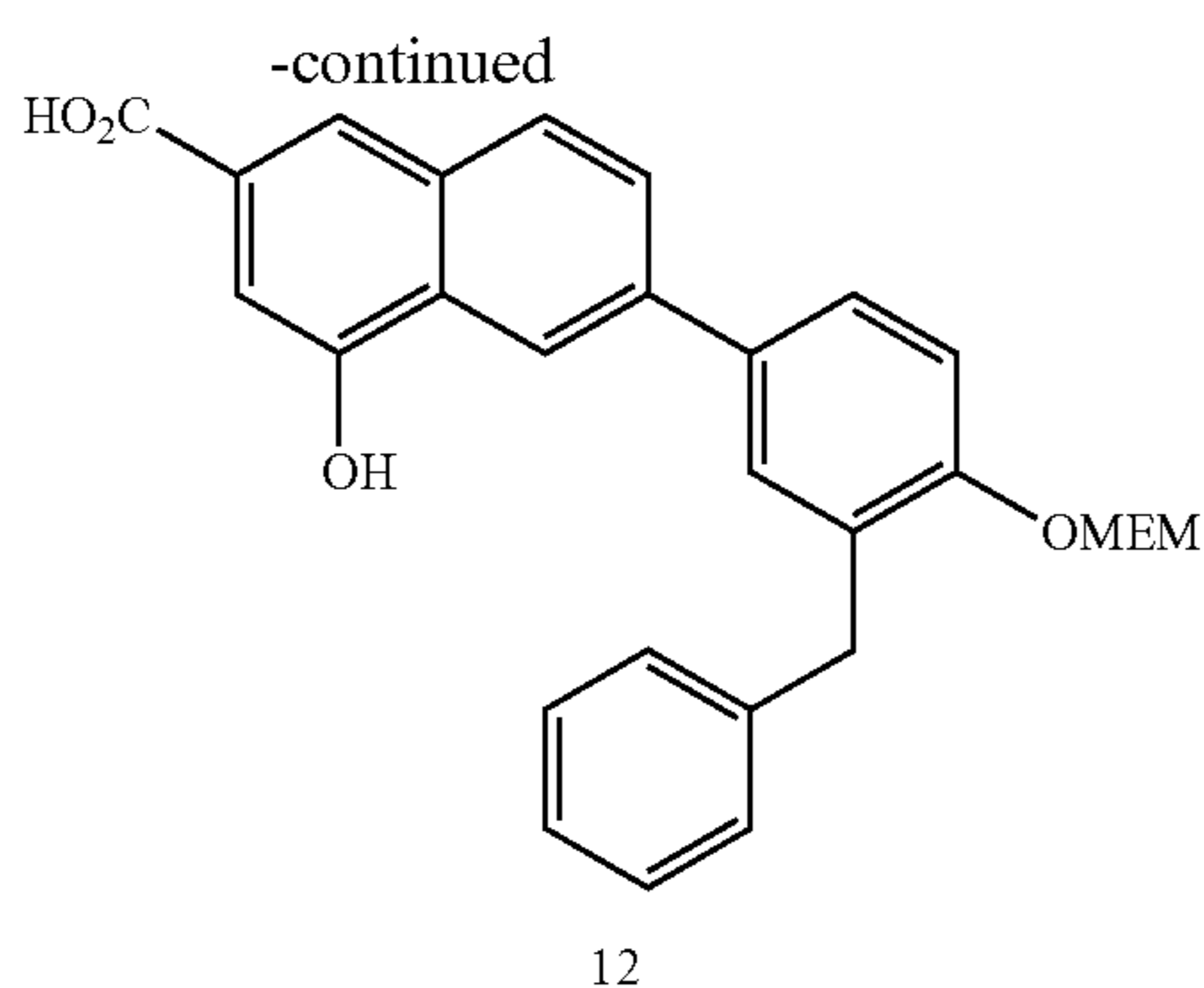
6-(3-benzyl-4-hydroxyphenyl)-4-hydroxy-2-naphthoic acid (12)
