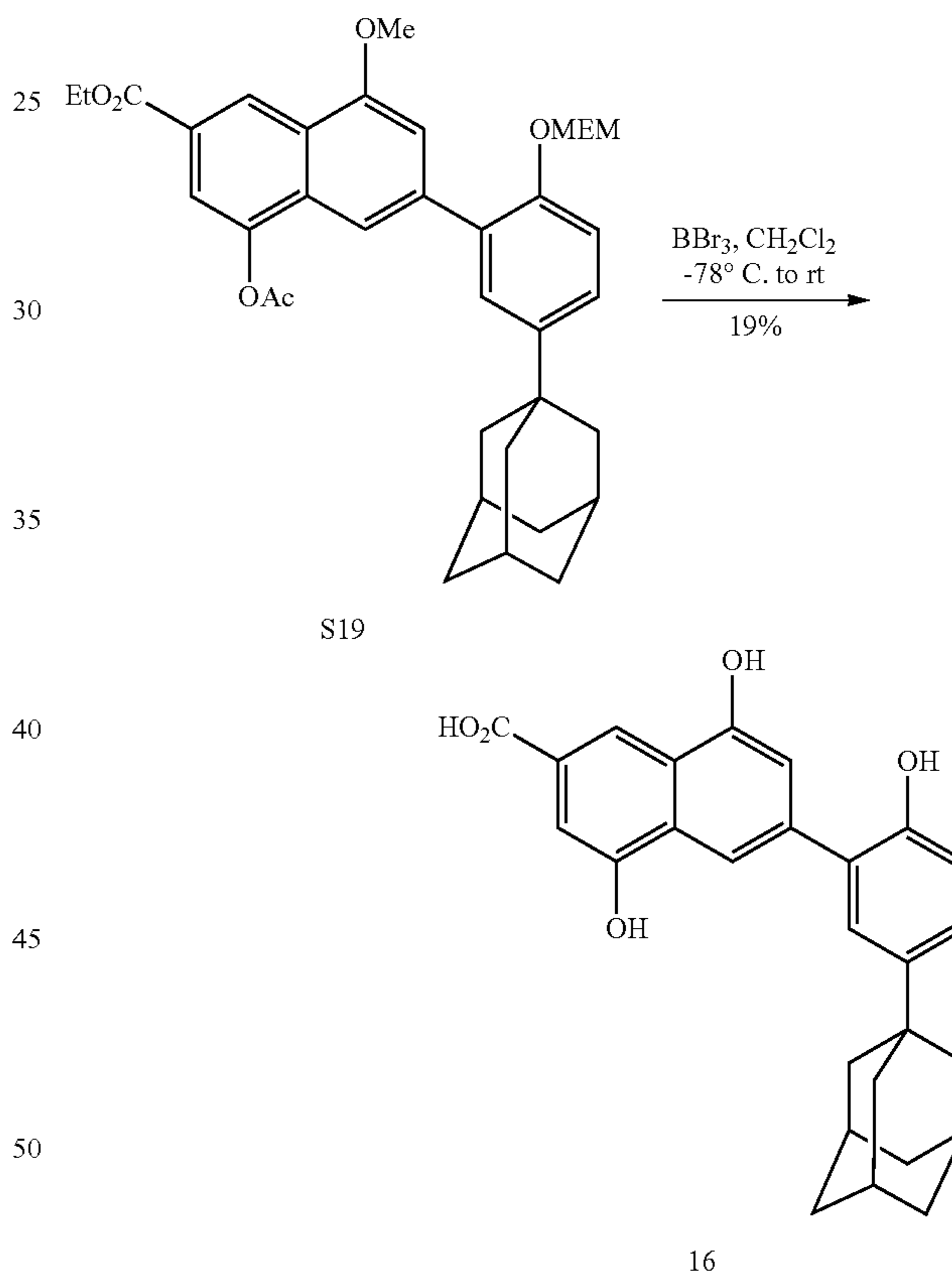
6-(5-(adamantan-1-yl)-2-hydroxyphenyl)-4,8-dihydroxy-2-naphthoic acid (16)
