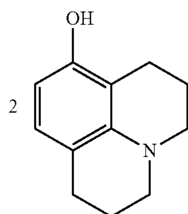
8-hydroxyjulolidine
