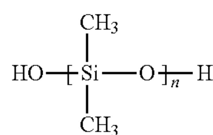
PDMS-hydroxy
