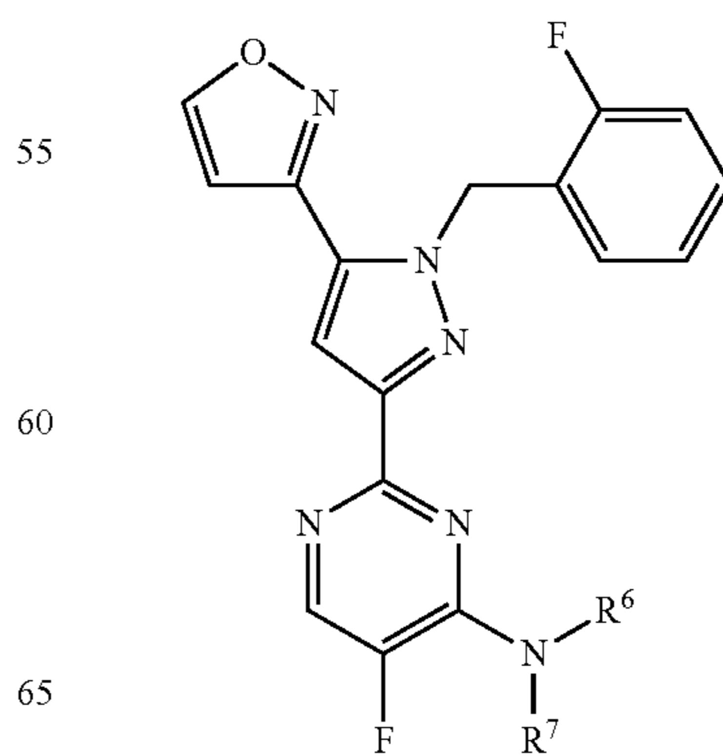
Formula IV
