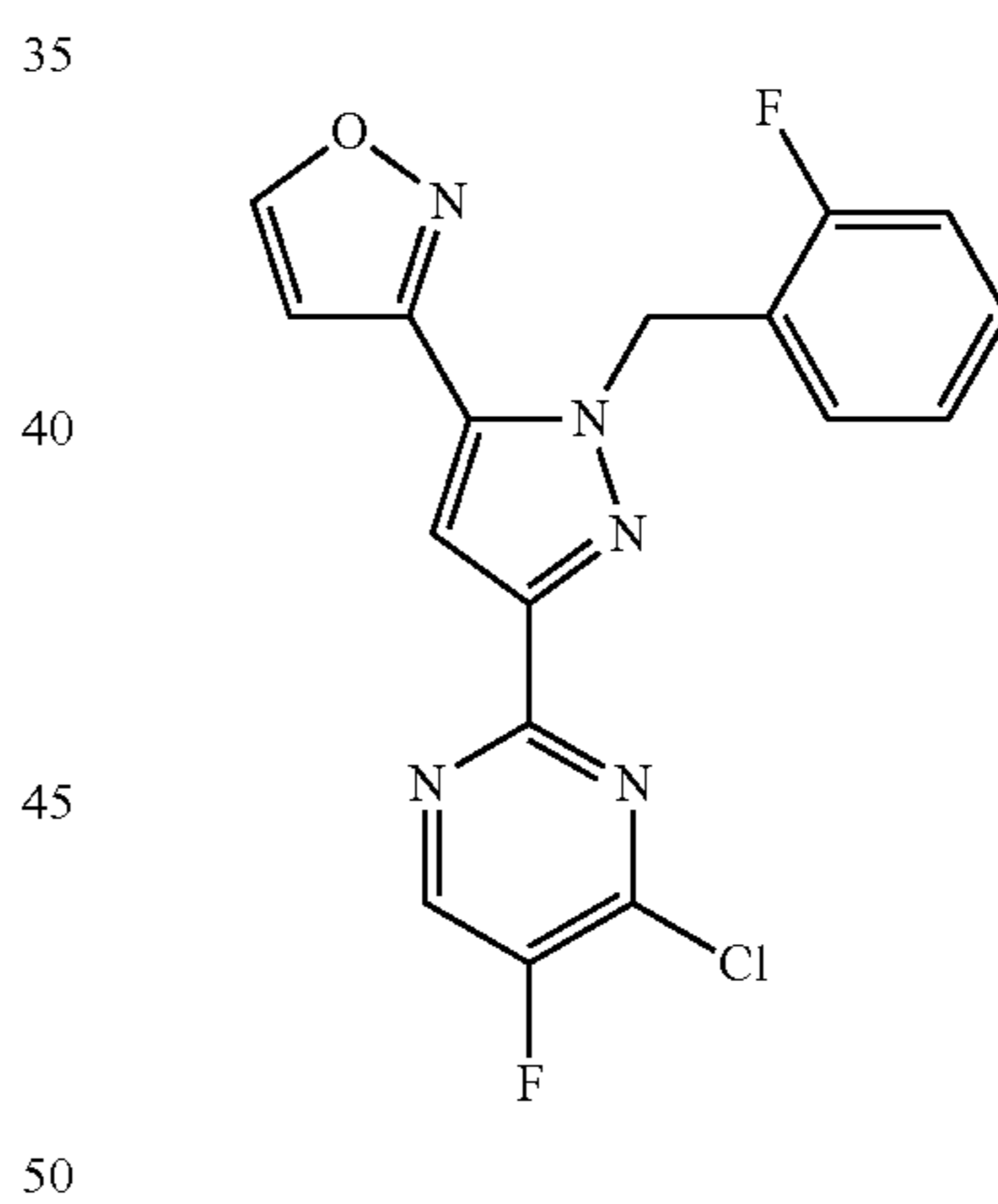
Formula III
