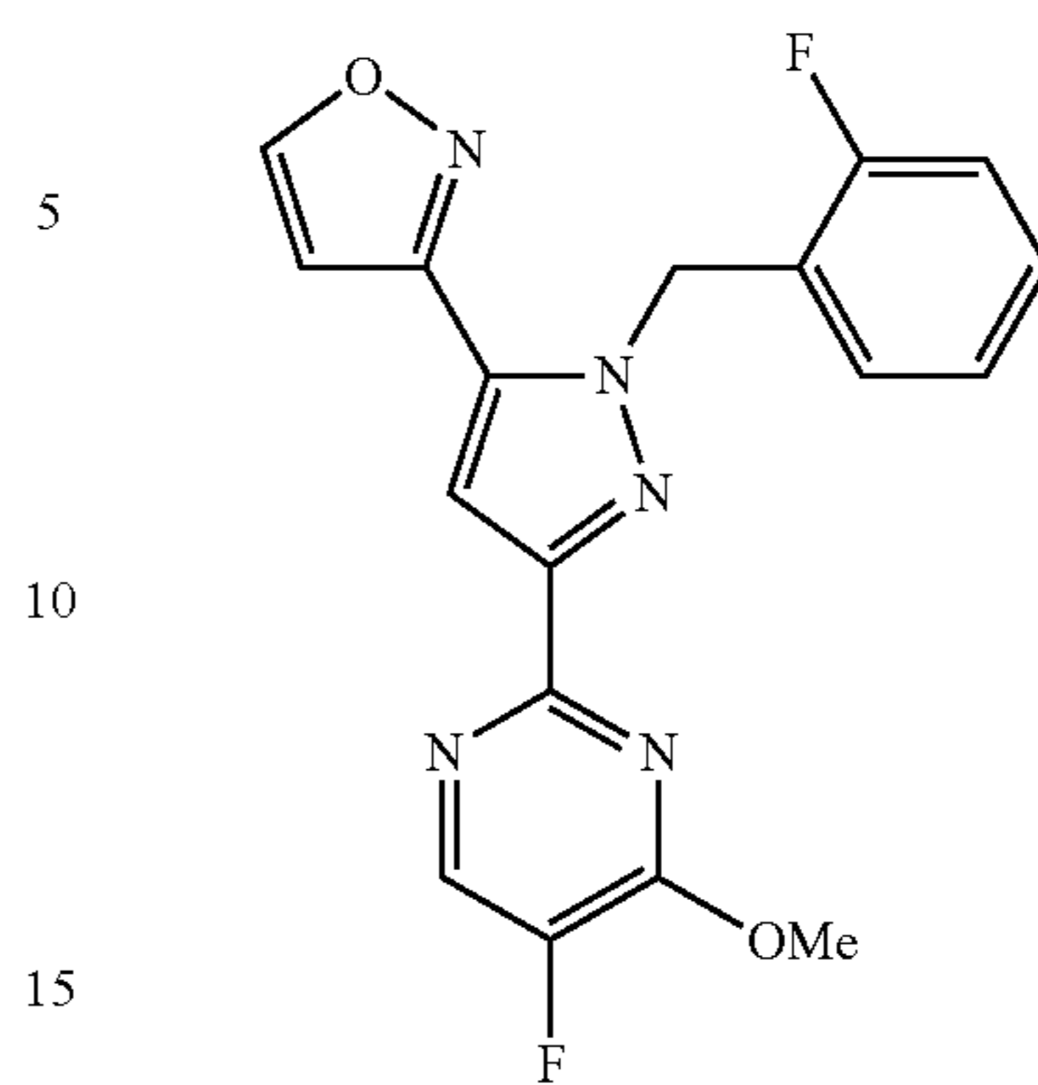
Formula II
