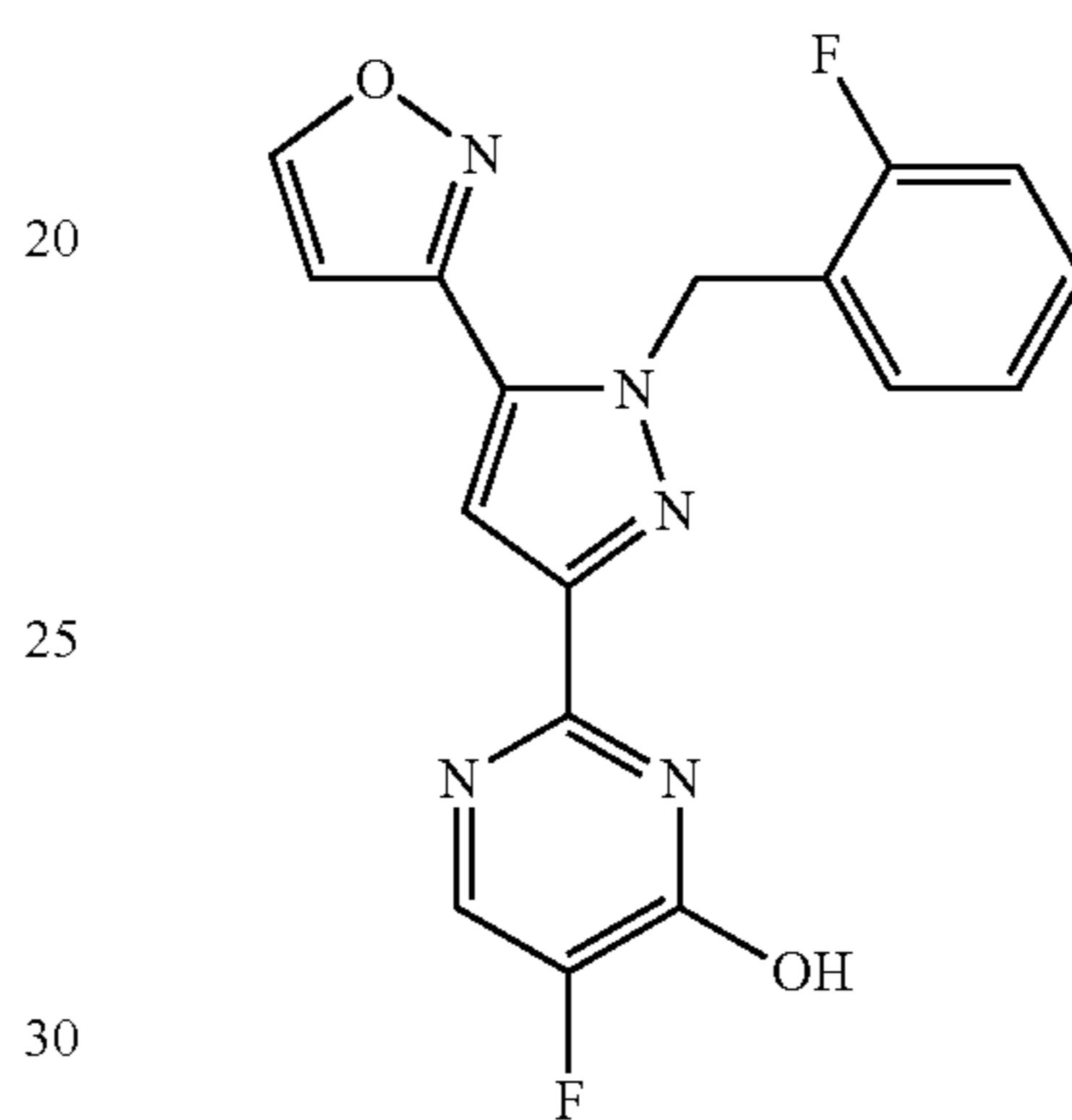
Compound 9
