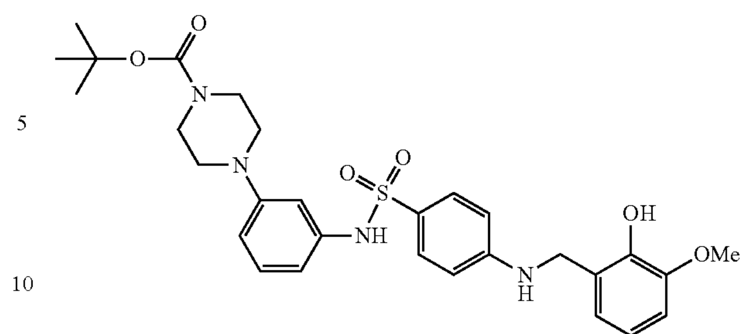
tert-butyl 4-(3-(4-((2-hydroxy-3-methoxybenzyl)amino)phenyl)sulfonamido)phenyl)piperidine-1-carboxylate (65)
