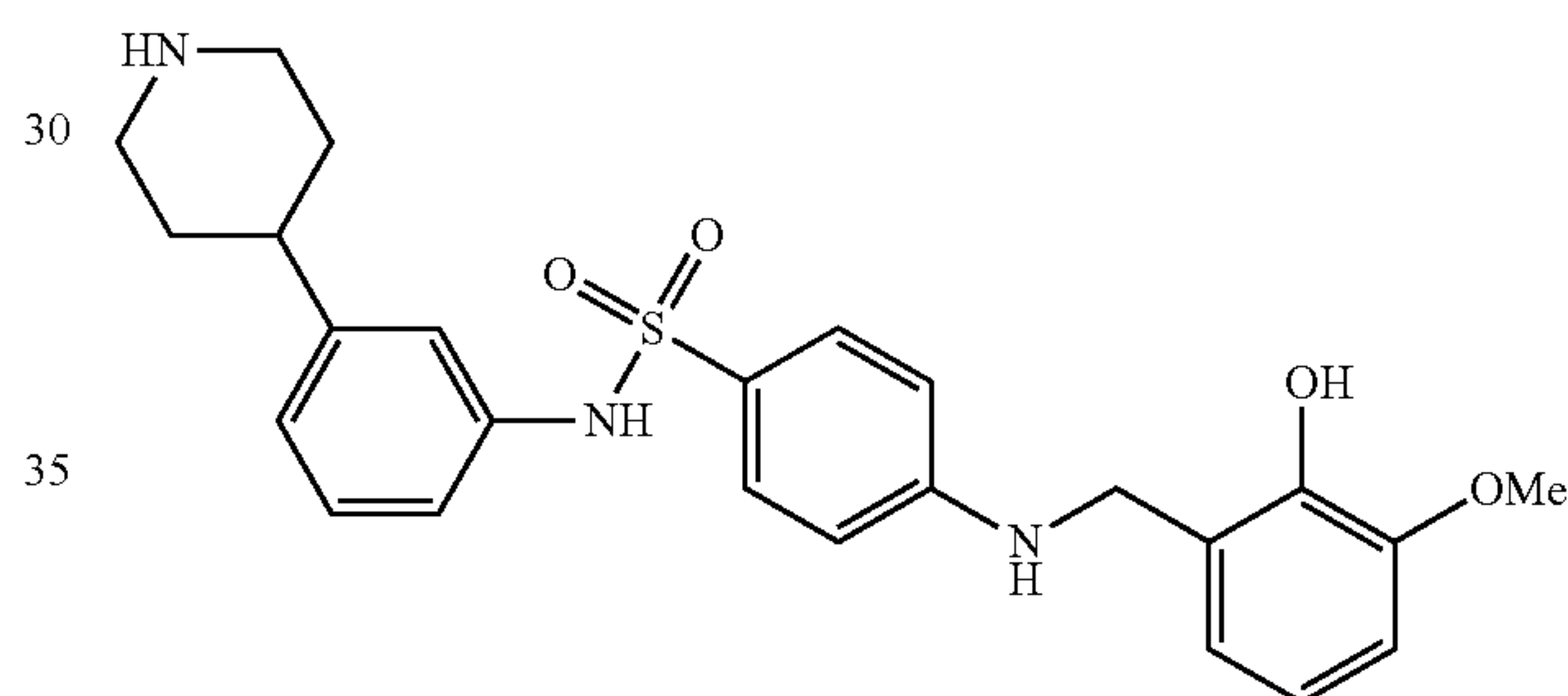
4-((2-hydroxy-3-methoxybenzyl)amino)-N-(3-(piperidin-4-yl)phenyl)benzenesulfonamide, TFA (66)
