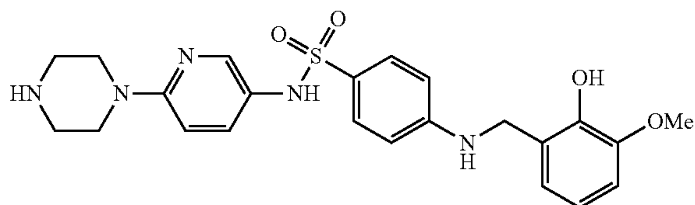
4-(2-hydroxy-3-methoxybenzylamino)-N-(6-(piperazin-1-yl)pyridin-3-yl)benzenesulfonamide (56)
