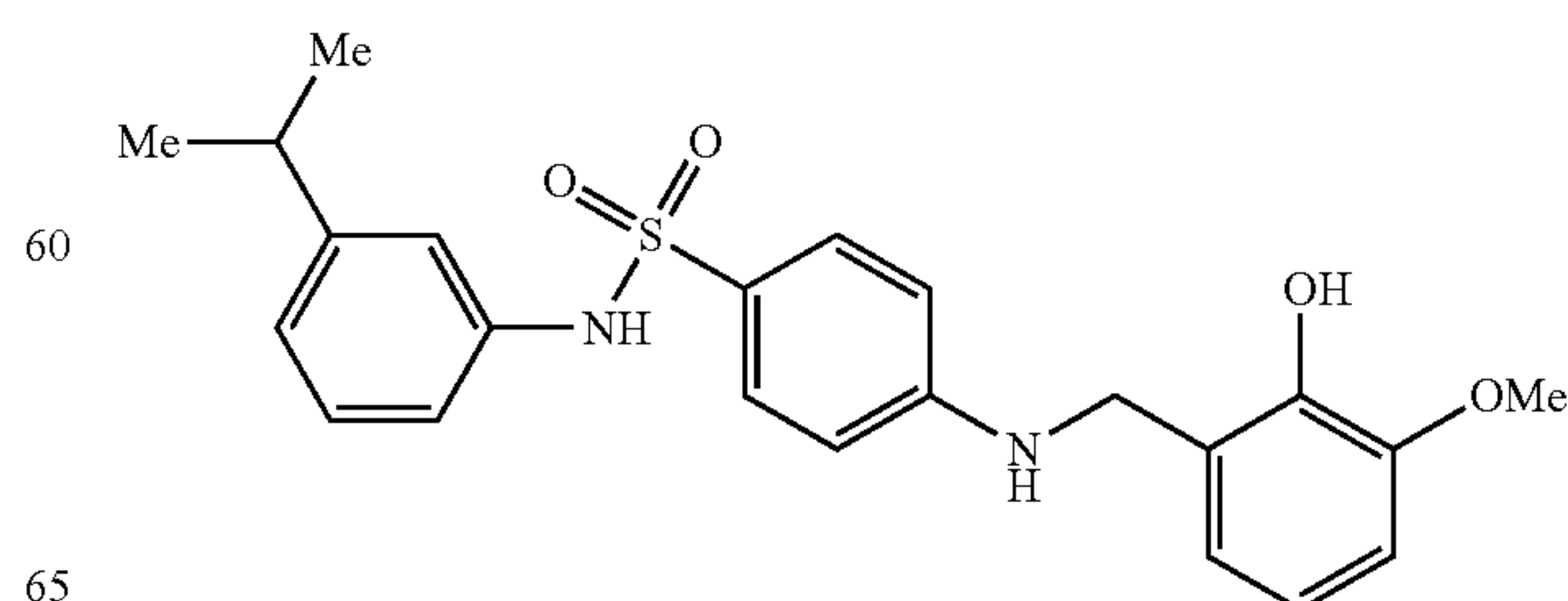
4-((2-hydroxy-3-methoxybenzyl)amino)-N-(3-morpholinophenyl)benzenesulfonamide, TFA (64)
