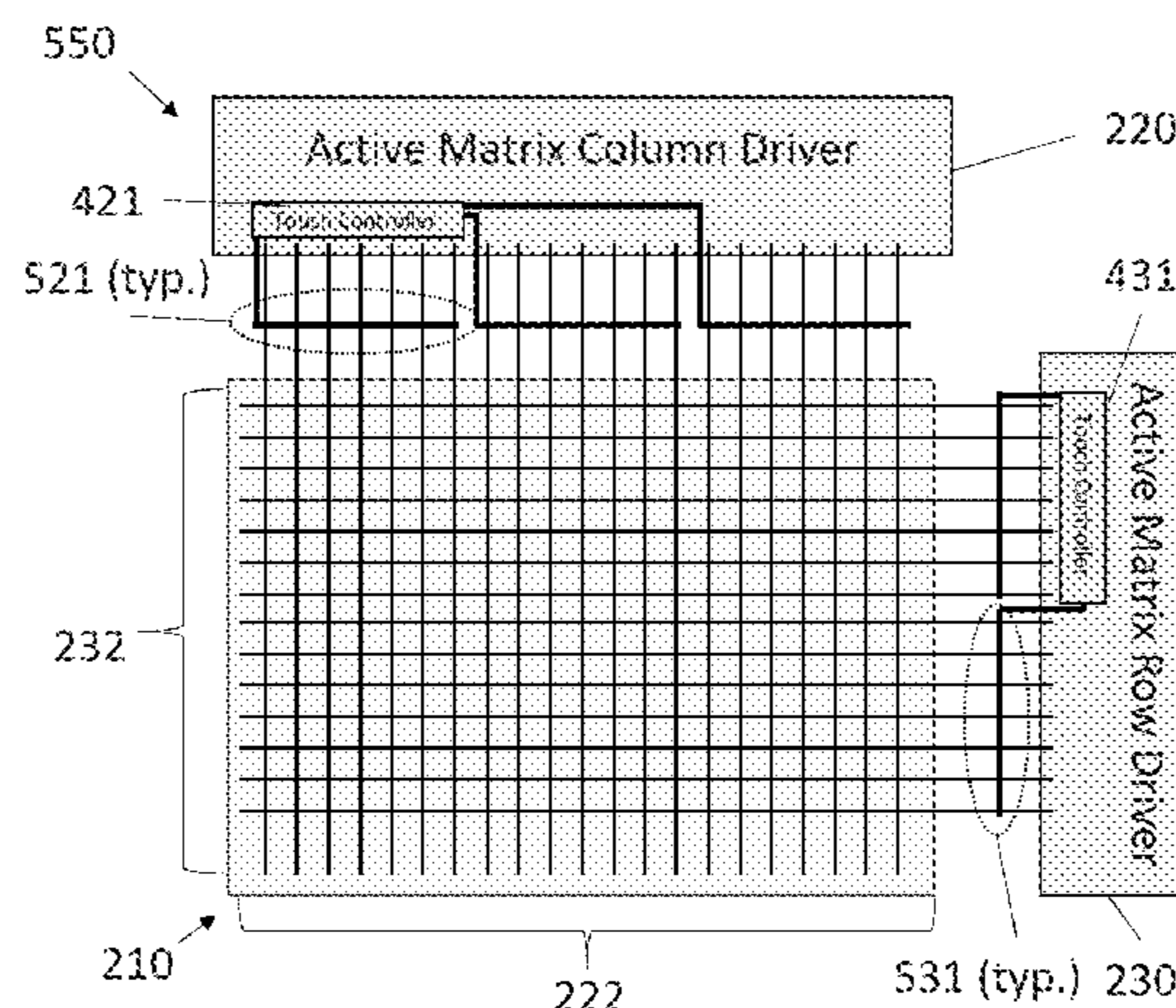
Touch controller channels capacitively coupled to selected Active Matrix rows and columns.
