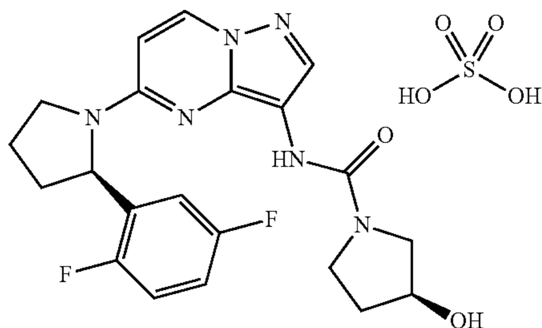
(S)—N-(5-((R)-2-(2,5-difluorophenyl)pyrrolidin-1-yl)pyrazolo[1,5-a]pyrimidin-3-yl)-3-hydroxypyrrolidine-1-carboxamide sulfate
