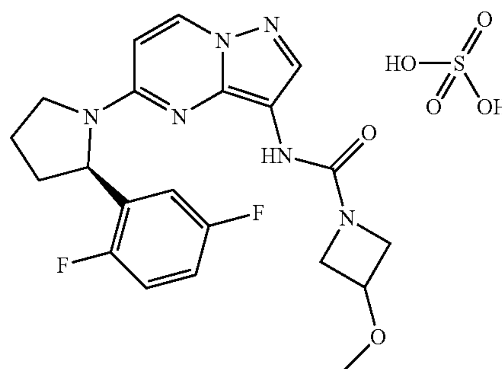
(R)—N-(5-(2-(2,5-difluorophenyl)pyrrolidin-1-yl)pyrazolo[1,5-a]pyrimidin-3-yl)-3-methoxyazetidine-1-carboxamide sulfate
