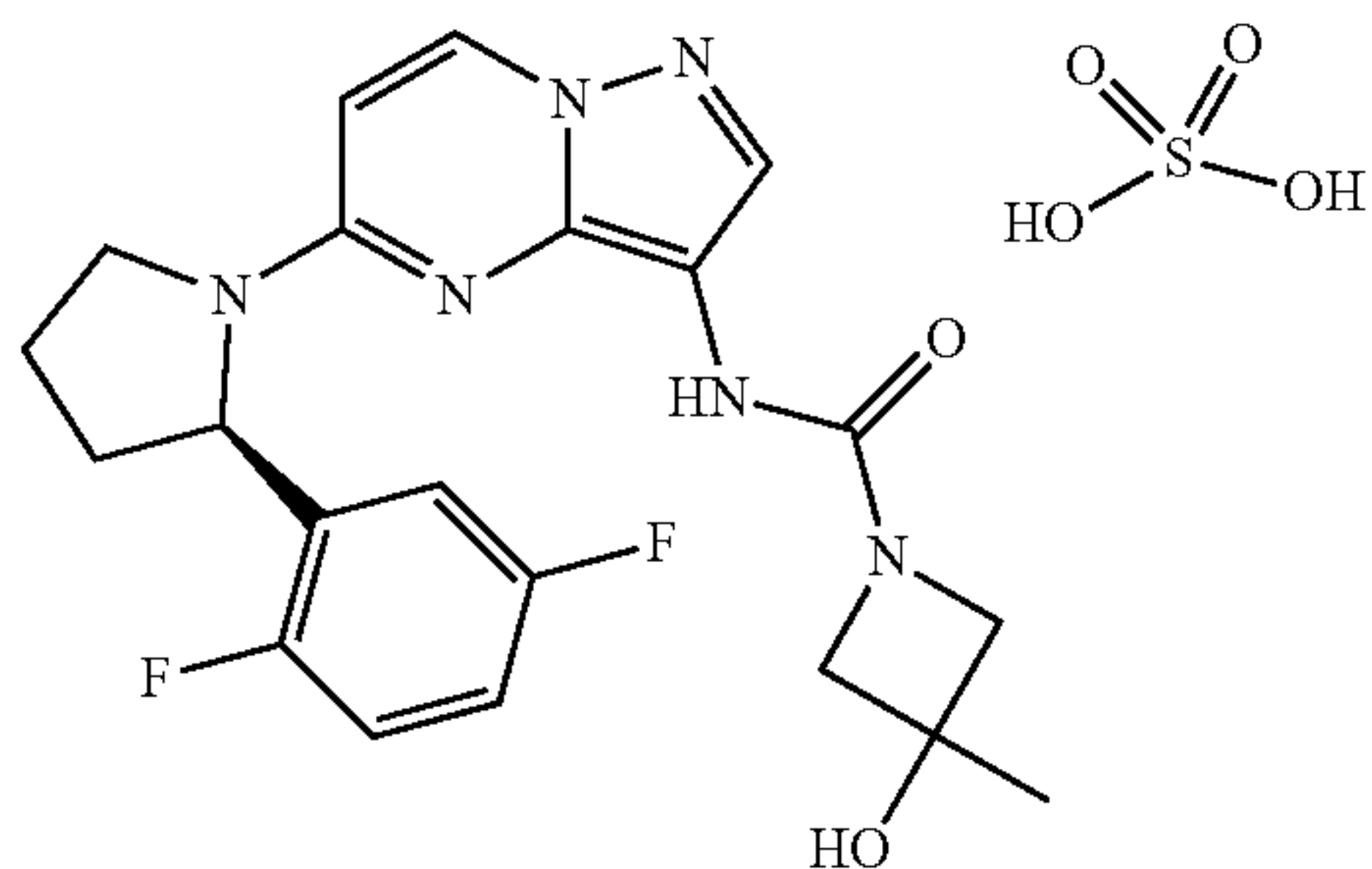
(R)—N-(5-(2-(2,5-difluorophenyl)pyrrolidin-1-yl)pyrazolo[1,5-a]pyrimidin-3-yl)-3-hydroxy-3-methylazetidine-1-carboxamide sulfate
