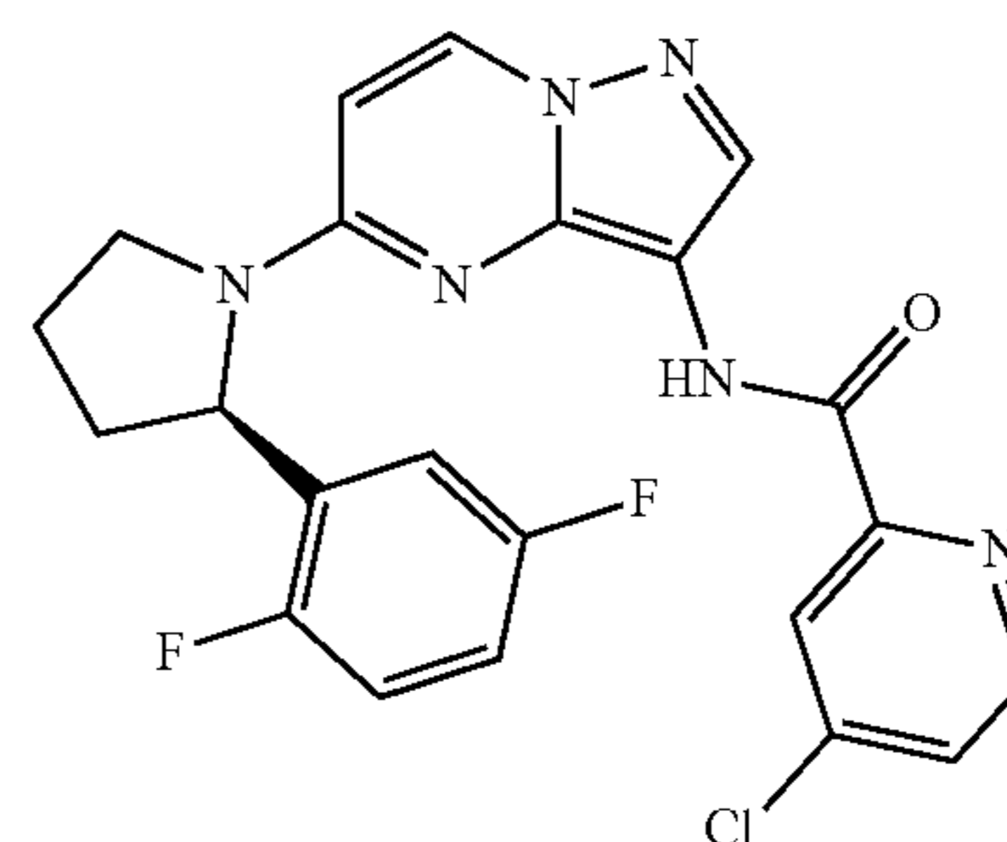
(R)-4-chloro-N-(5-(2-(2,5-difluorophenyl)pyrrolidin-1-yl)pyrazolo[1,5-a]pyrimidin-3-yl)picolinamide
