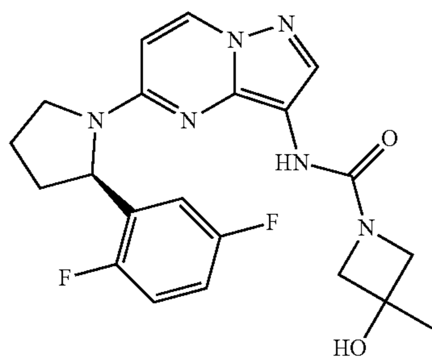
(R)—N-(5-(2-(2,5-difluorophenyl)pyrrolidin-1-yl)pyrazolo[1,5-a]pyrimidin-3-yl)-3-hydroxy-3-methylazetidide-1-carboxamide
