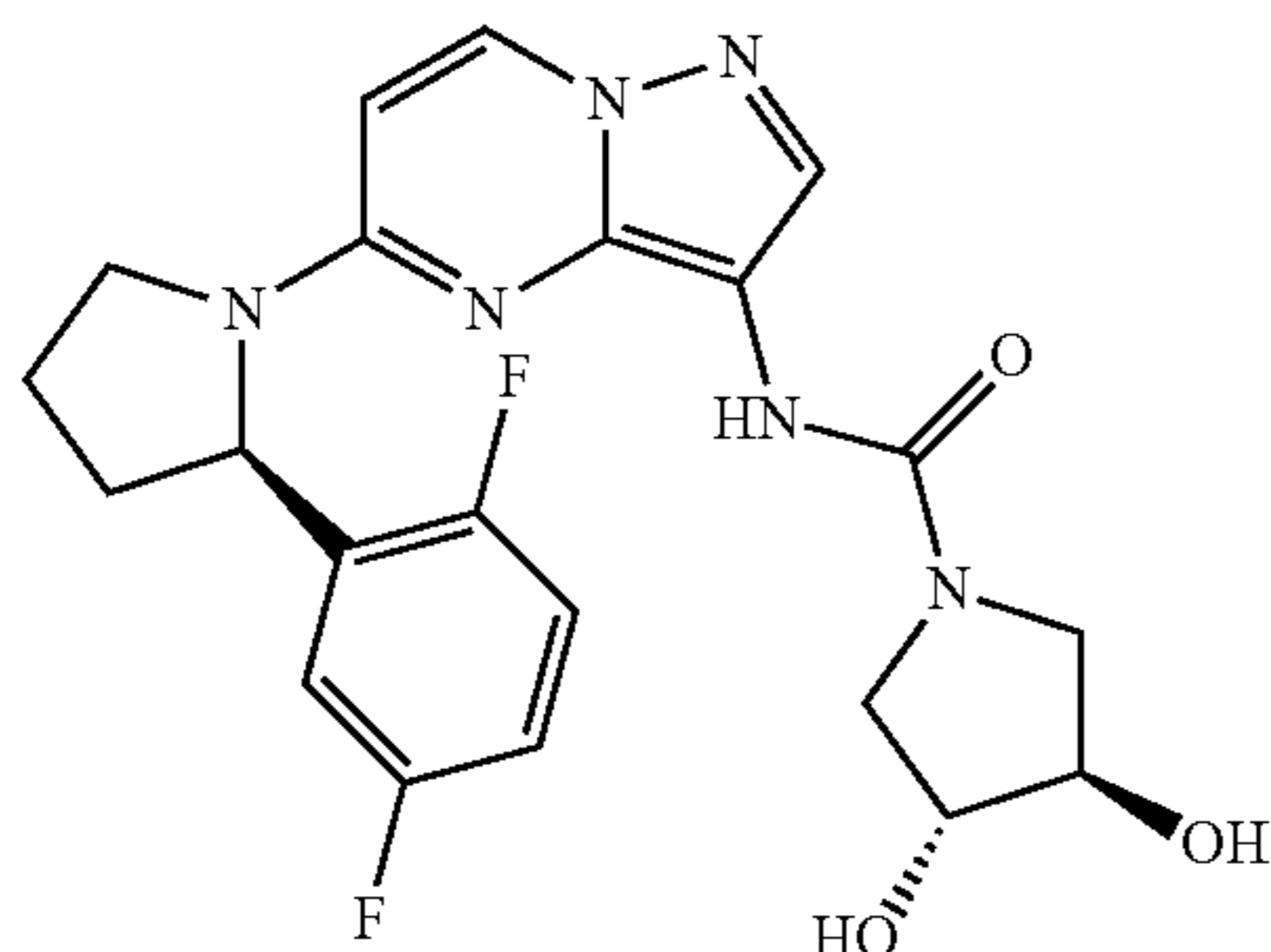
(3R,4R)—N-(5-((R)-2-(2,5-difluorophenyl)pyrrolidin-1-yl)pyrazolo[1,5-a]pyrimidin-3-yl)-3,4-dihydroxypyrrolidine-1-carboxamide
