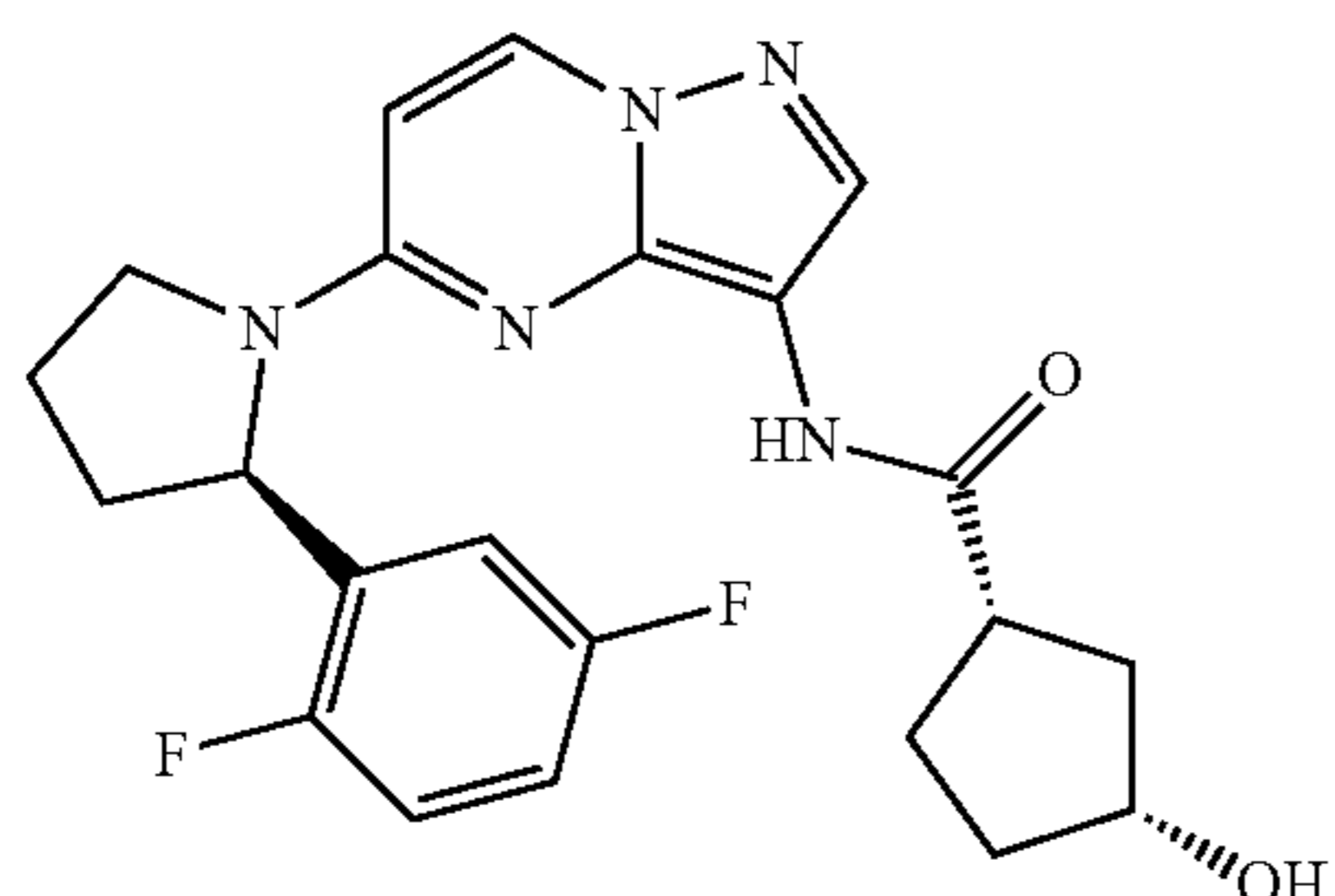
(1S,3R)—N-(5-((R)-2-(2,5-difluorophenyl)pyrrolidin-1-yl)pyrazolo[1,5-a]pyrimidin-3-yl)-3-hydroxycyclopentanecarboxamide
