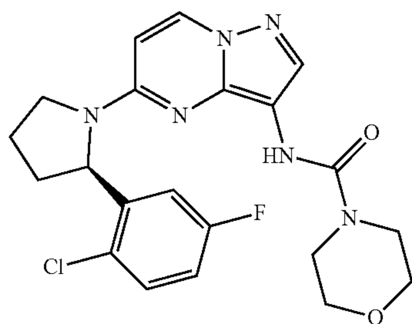
(R)—N-(5-(2-(2-chloro-5-fluorophenyl)pyrrolidin-1-yl)pyrazolo[1,5-a]pyrimidin-3-yl)morpholine-4-carboxamide
