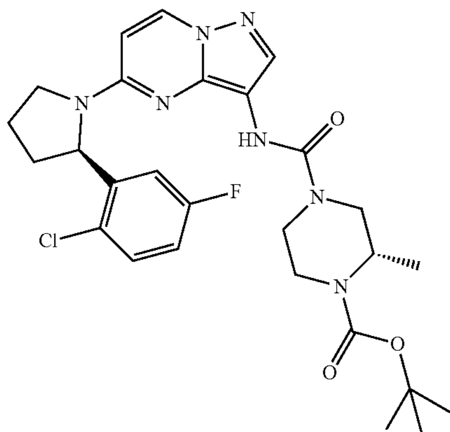
(S)-tert-butyl 4-(5-(2-(2-chloro-5-fluorophenyl)pyrrolidin-1-yl)pyrazolo[1,5-a]pyrimidin-3-yl)carbamoyl-2-methylpiperazine-1-carboxylate
