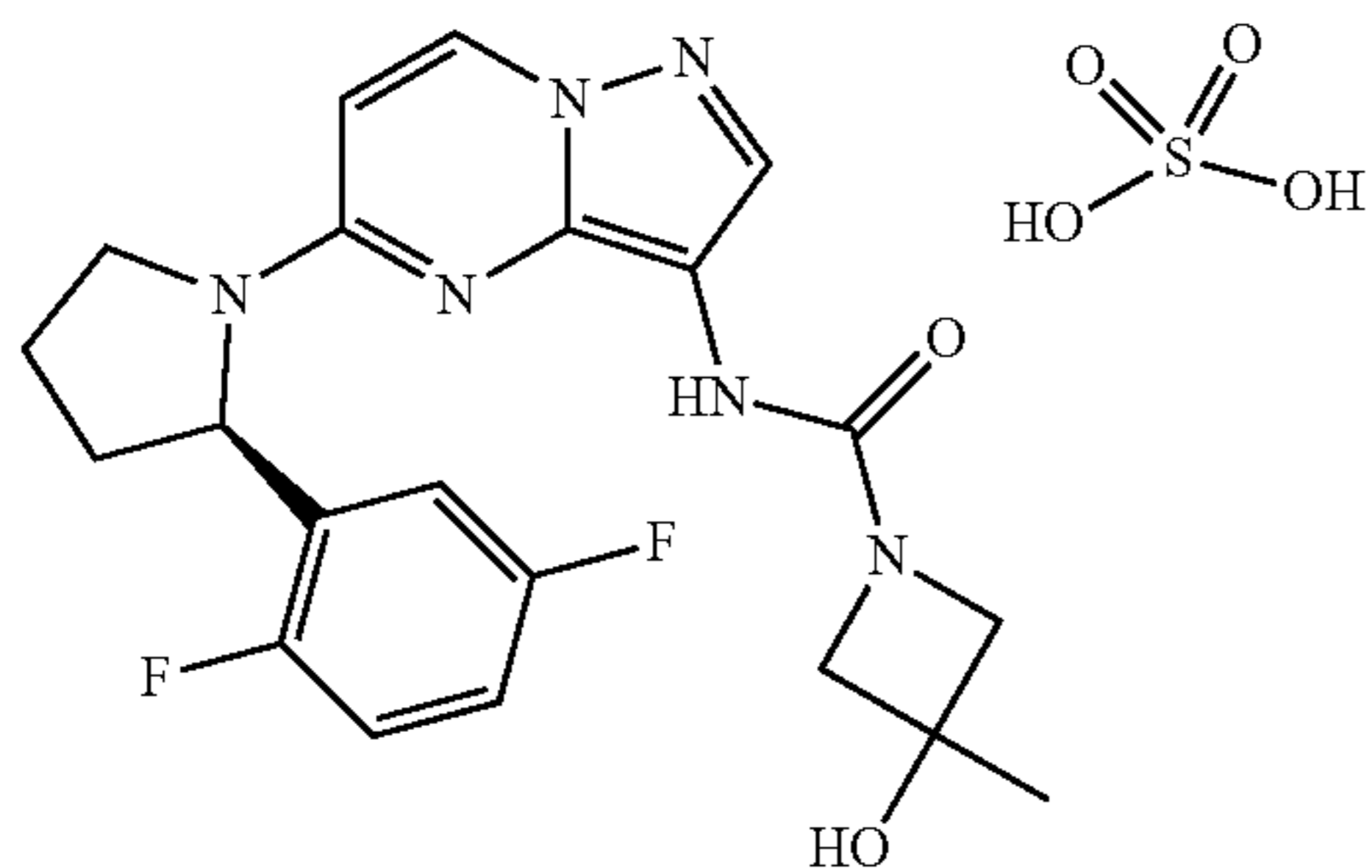
(R)—N-(5-(2-(2,5-difluorophenyl)pyrrolidin-1-yl)pyrazolo[1,5-a]pyrimidin-3-yl)-3-hydroxy-3-methylazetidide-1-carboxamide sulfate
