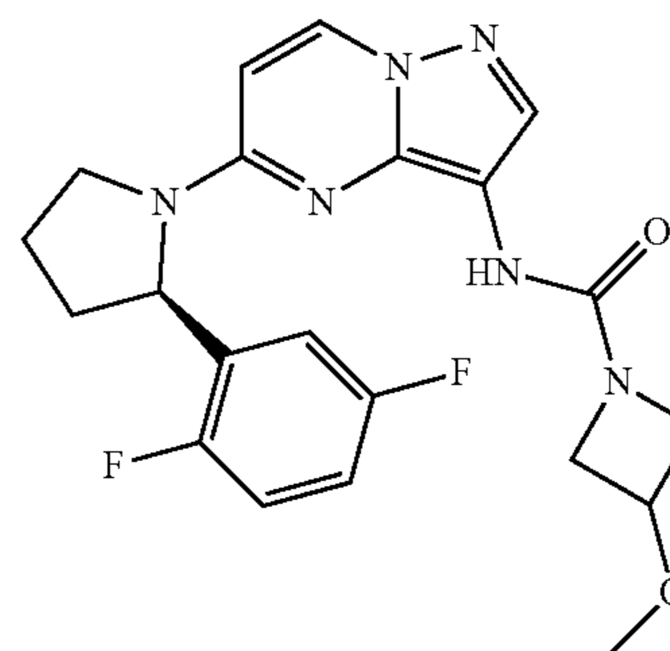
(R)—N-(5-(2-(2,5-difluorophenyl)pyrrolidin-1-yl)pyrazolo[1,5-a]pyrimidin-3-yl)-3-methoxyazetidene-1-carboxamide
