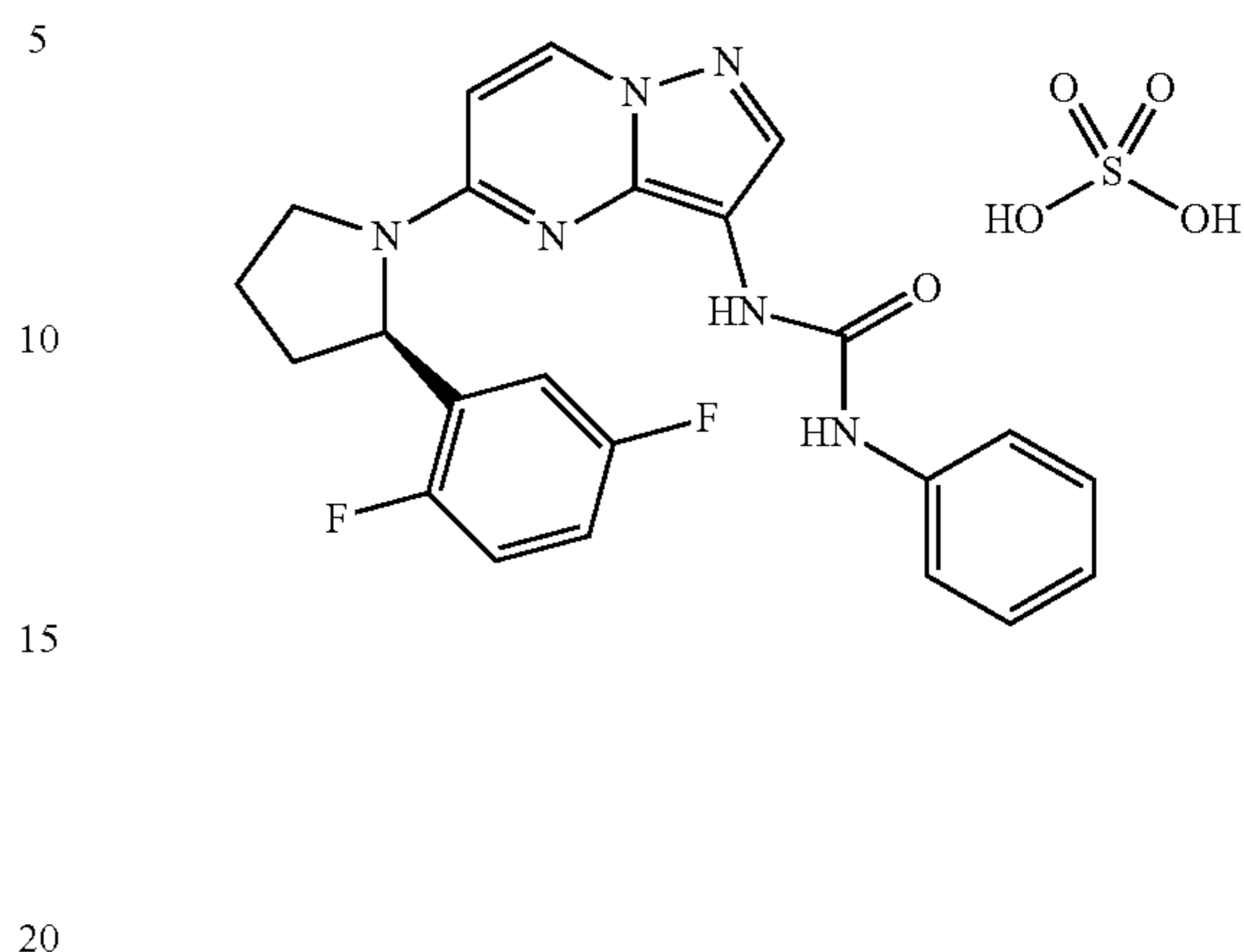
(R)-1-(5-(2-(2,5-difluorophenyl)pyrrolidin-1-yl)pyrazolo[1,5-a]pyrimidin-3-yl)-3-phenylurea sulfate
