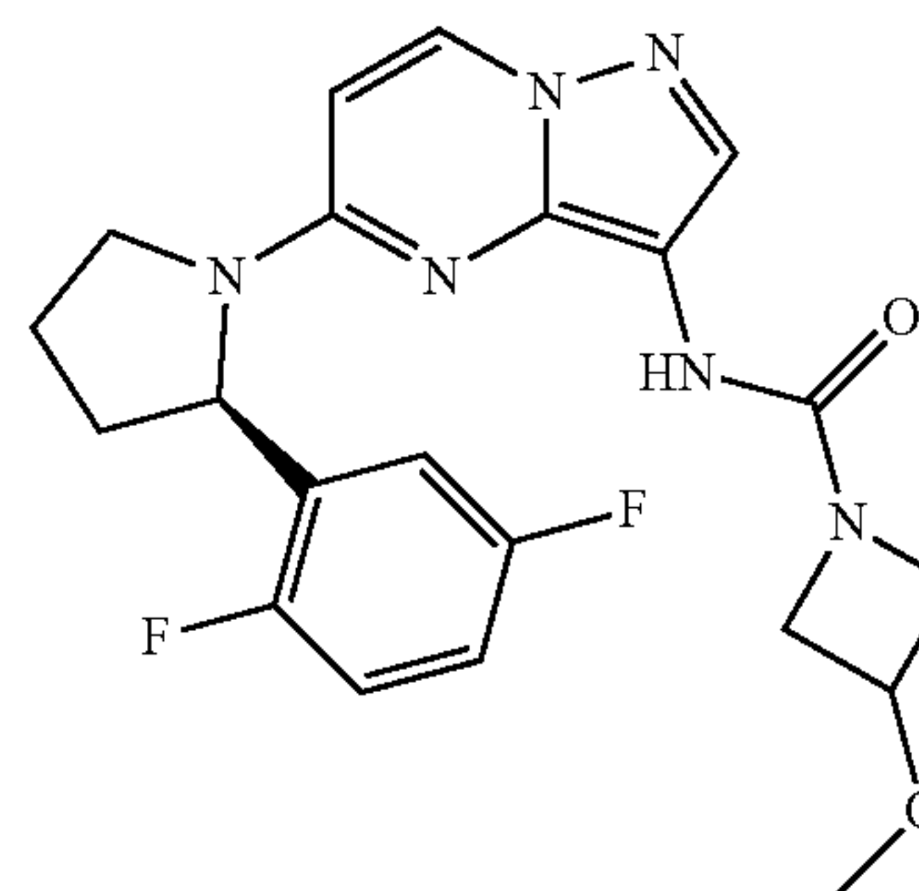
(R)—N-(5-(2-(2,5-difluorophenyl)pyrrolidin-1-yl)pyrazolo[1,5-a]pyrimidin-3-yl)-3-methoxyazetidine-1-carboxamide
