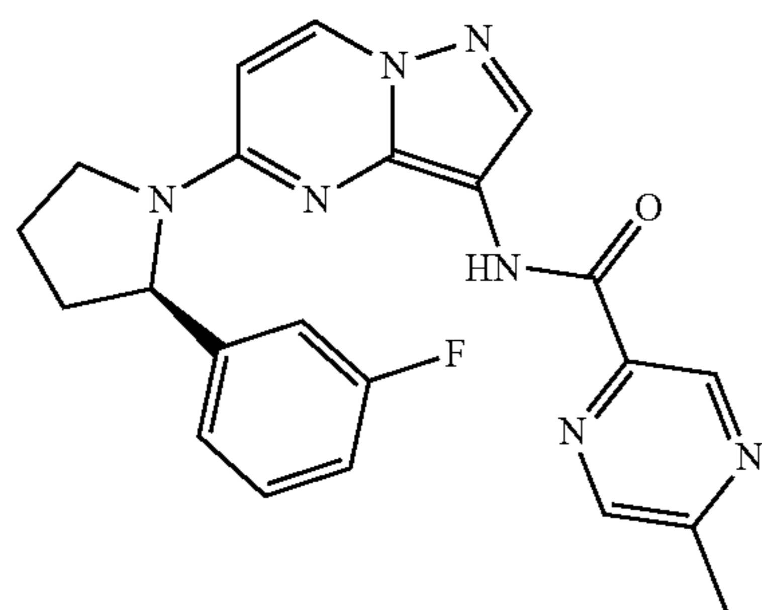
(R)—N-(5-(2-(3-fluorophenyl)pyrrolidin-1-yl)pyrazolo[1,5-a]pyrimidin-3-yl)-5-methylpyrazine-2-carboxamide
