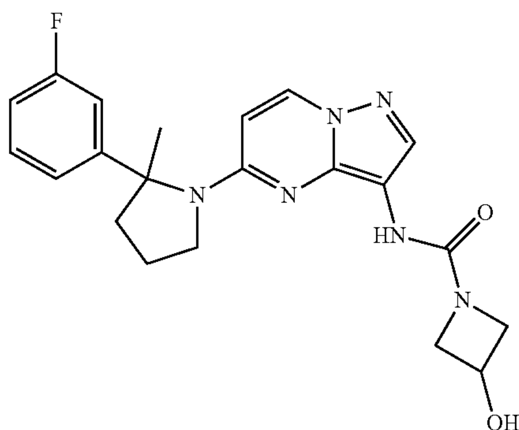
N-(5-(2-(3-fluorophenyl)-2-methylpyrrolidin-1-yl)pyrazolo[1,5-a]pyrimidin-3-yl)-3-hydroxyazetidine-1-carboxamide
