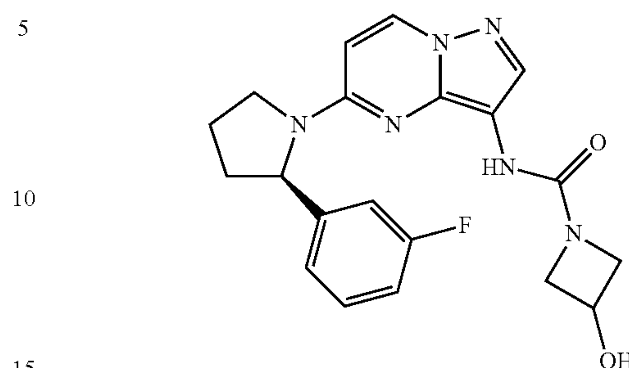
(R)-N-(5-(2-(3-fluorophenyl)pyrrolidin-1-yl)pyrazolo[1,5-a]pyrimidin-3-yl)-3-hydroxyazetidine-1-carboxamide
