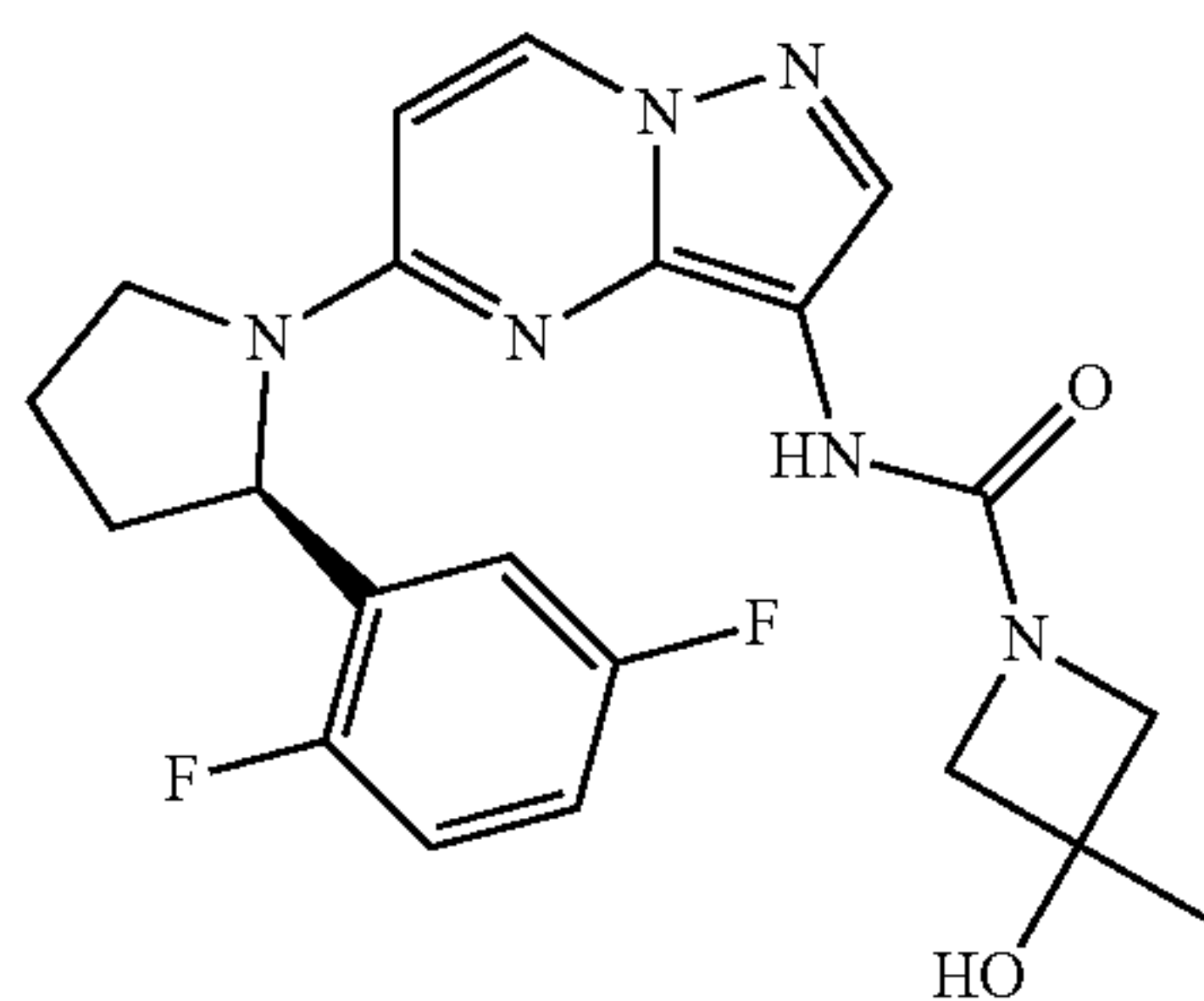
(R)—N-(5-(2-(2,5-difluorophenyl)pyrrolidin-1-yl)pyrazolo[1,5-a]pyrimidin-3-yl)-3-hydroxy-3-methylazetidine-1-carboxamide
