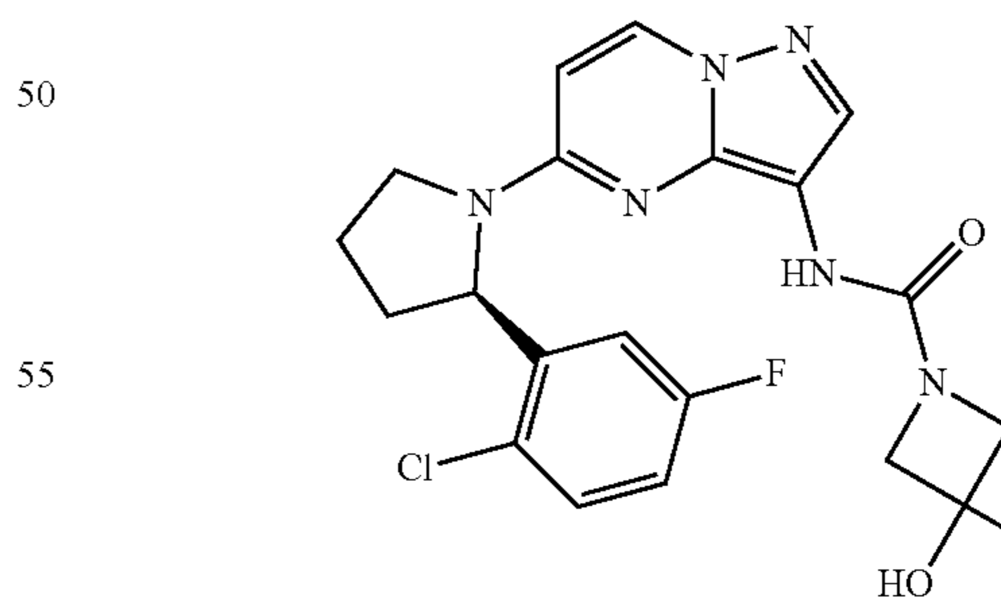
(R)-N-(5-(2-(2-chloro-5-fluorophenyl)pyrrolidin-1-yl)pyrazolo[1,5-a]pyrimidin-3-yl)-3-hydroxy-3-methylazetidine-1-carboxamide
