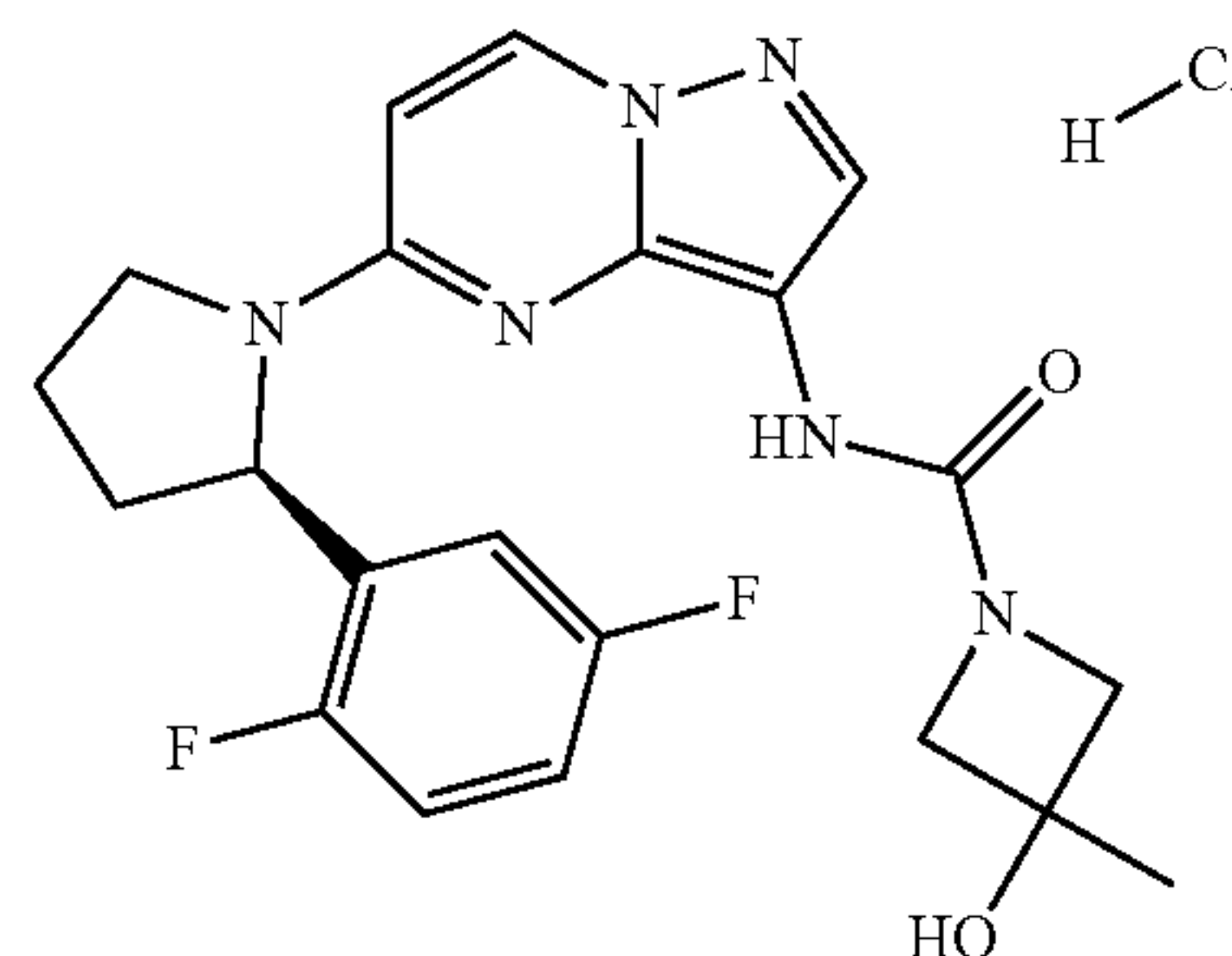
(R)—N-(5-(2-(2,5-difluorophenyl)pyrrolidin-1-yl)pyrazolo[1,5-a]pyrimidin-3-yl)-3-hydroxy-3-methylazetidine-1-carboxamide hydrochloride
