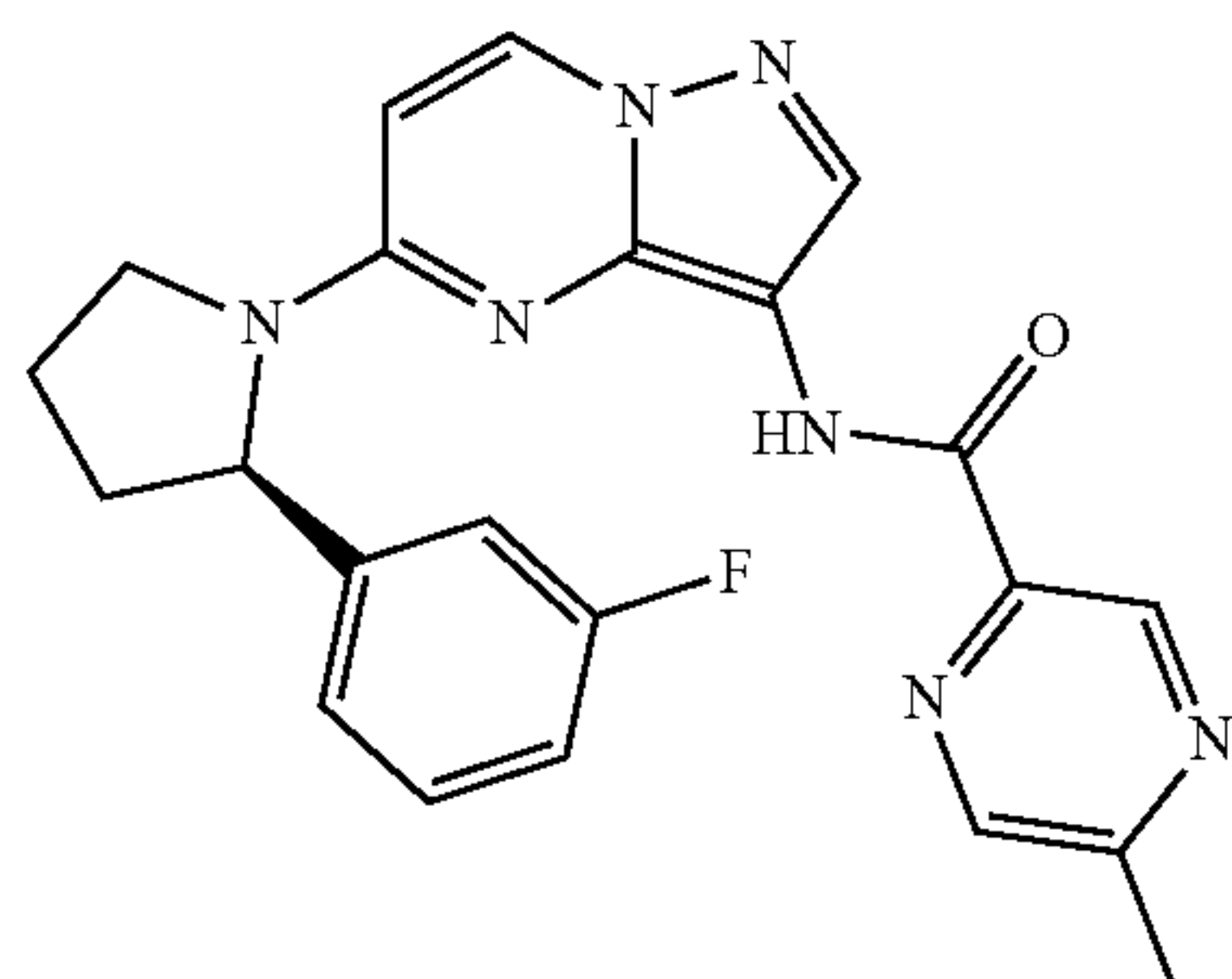
(R)—N-(5-(2-(3-fluorophenyl)pyrrolidin-1-yl)pyrazolo[1,5-a]pyrimidin-3-yl)-5-methylpyrazine-2-carboxamide
