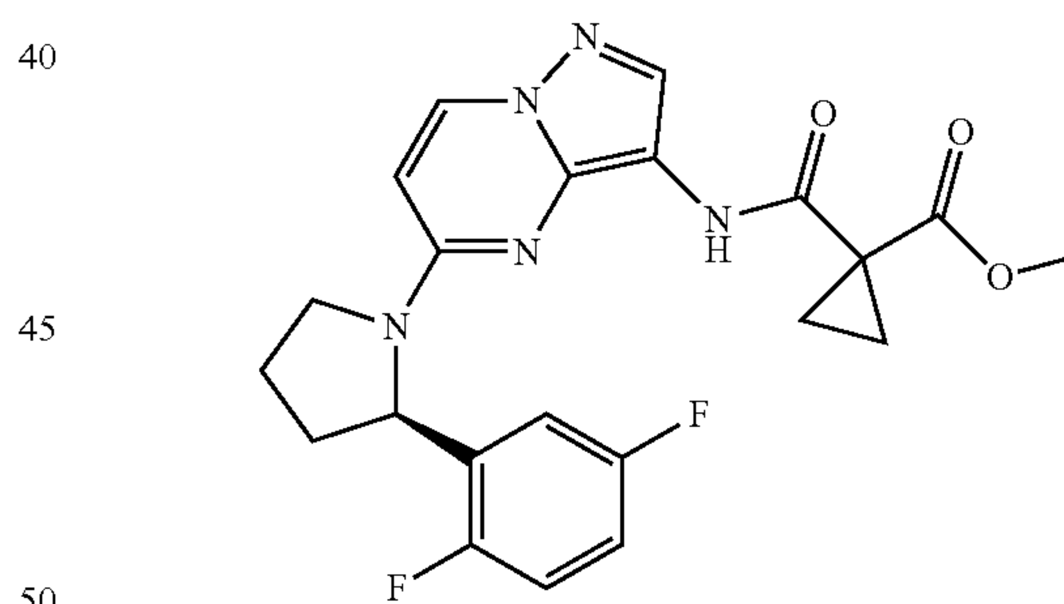
(R)-methyl 1-(5-(2-(2,5-difluorophenyl)pyrrolidin-1-yl)pyrazolo[1,5-a]pyrimidin-3-ylcarbamoyl)cyclopropanecarboxylate
