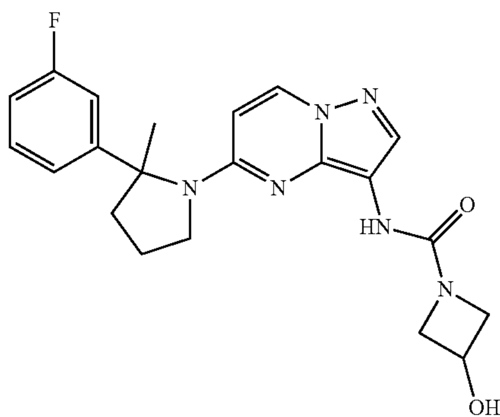
N-(5-(2-(3-fluorophenyl)-2-methylpyrrolidin-1-yl)pyrazolo[1,5-a]pyrimidin-3-yl)-3-hydroxyazetidine-1-carboxamide
