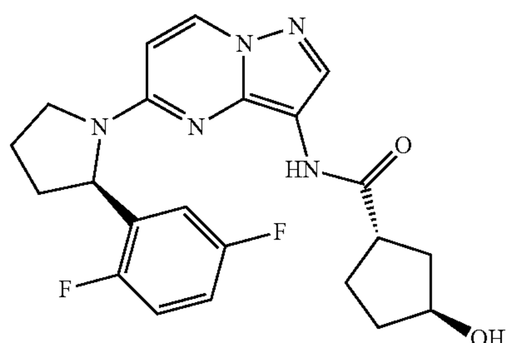
(1S,3S)-N-(5-((R)-2-(2,5-difluorophenyl)pyrrolidin-1-yl)pyrazolo[1,5-a]pyrimidin-3-yl)-3-hydroxycyclopentanecarboxamide
