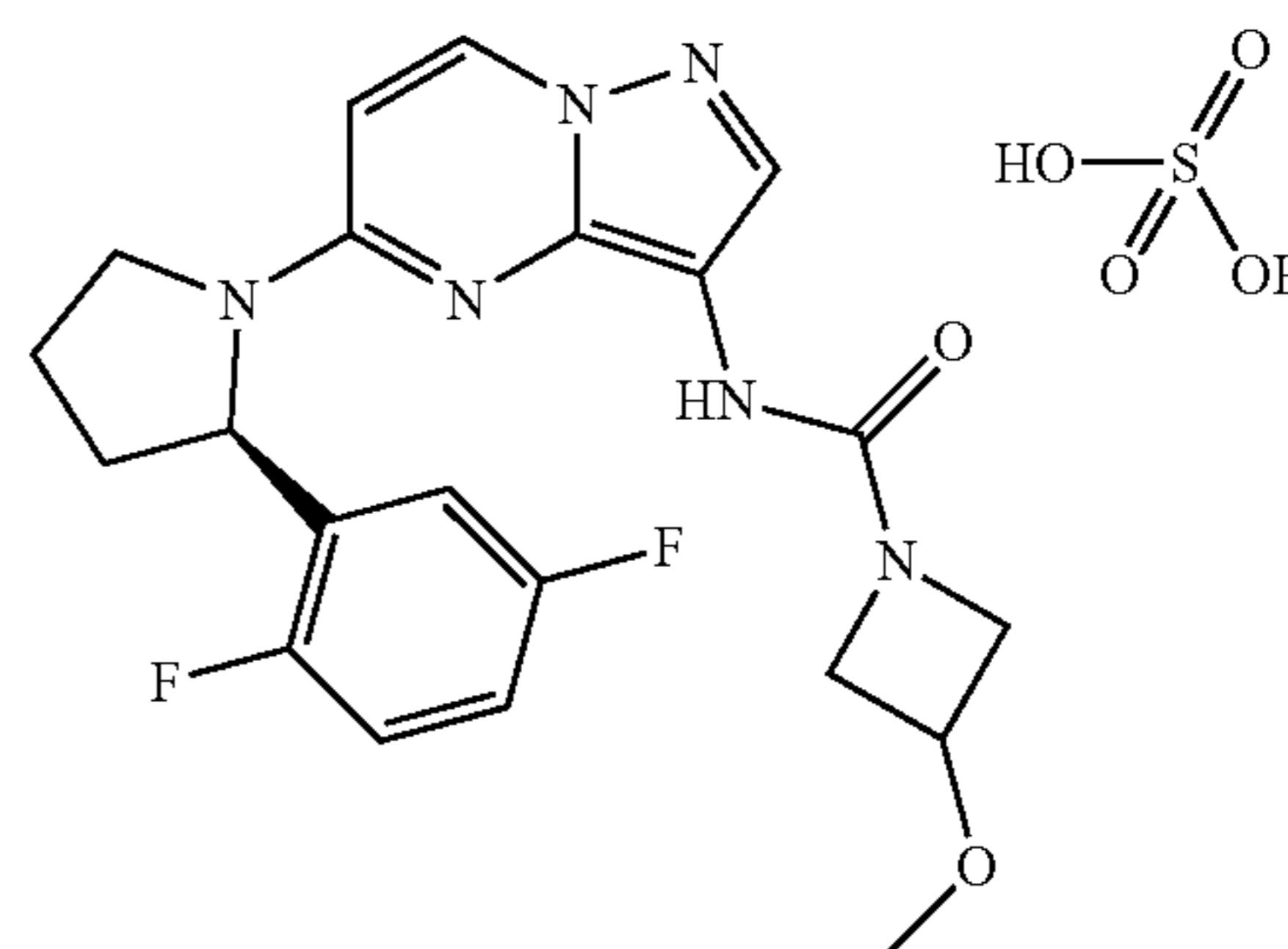
(R)—N-(5-(2-(2,5-difluorophenyl)pyrrolidin-1-yl)pyrazolo[1,5-a]pyrimidin-3-yl)-3-methoxyazetidene-1-carboxamide sulfate
