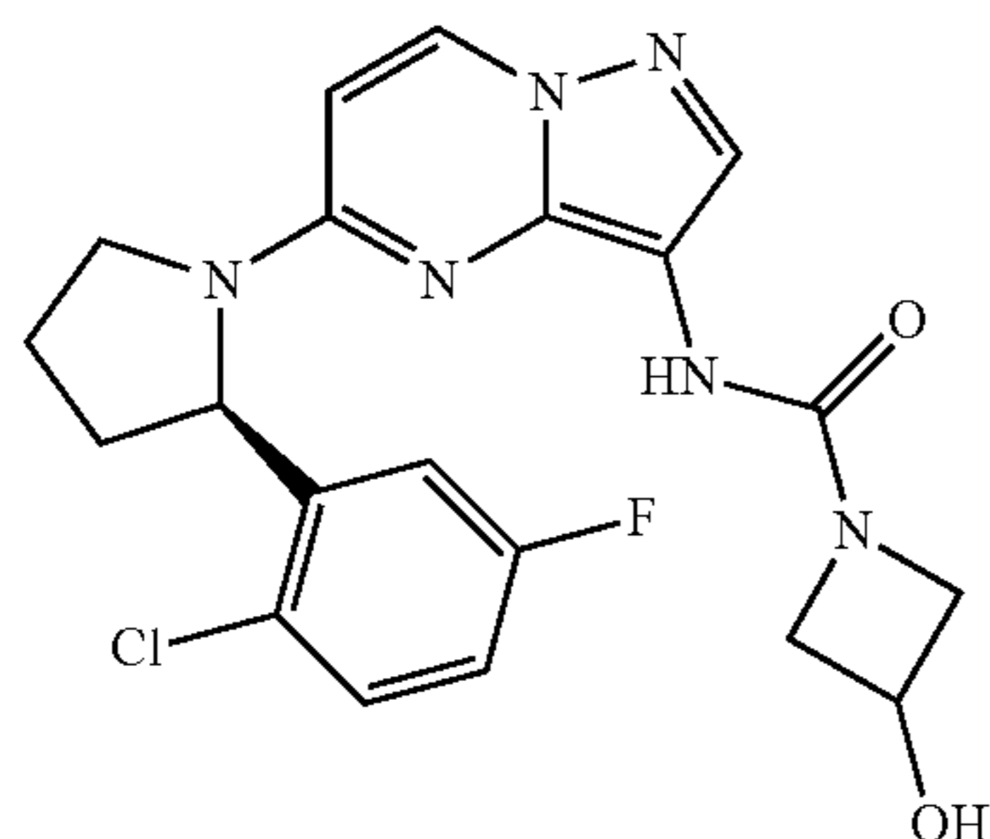
(R)-N-(5-(2-(2-chloro-5-fluorophenyl)pyrrolidin-1-yl)pyrazolo[1,5-a]pyrimidin-3-yl)-3-hydroxyazetidine-1-carboxamide
