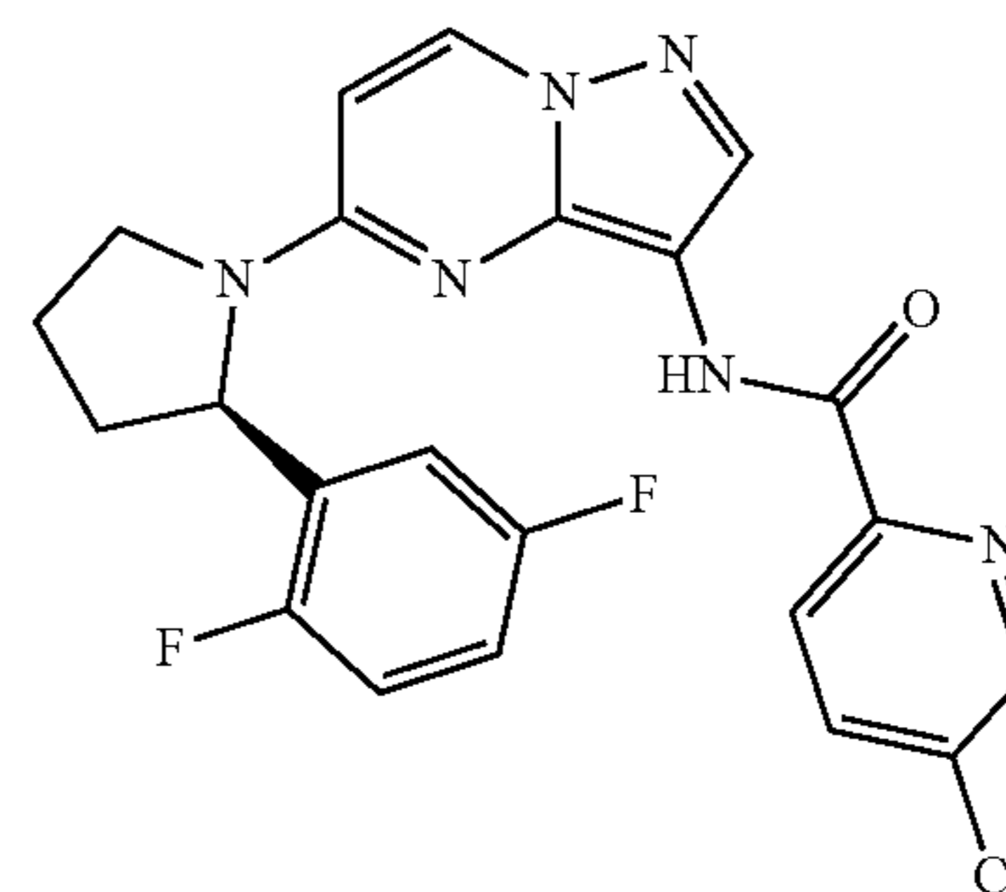
(R)-5-chloro-N-(5-(2-(2,5-difluorophenyl)pyrrolidin-1-yl)pyrazolo[1,5-a]pyrimidin-3-yl)picolinamide
