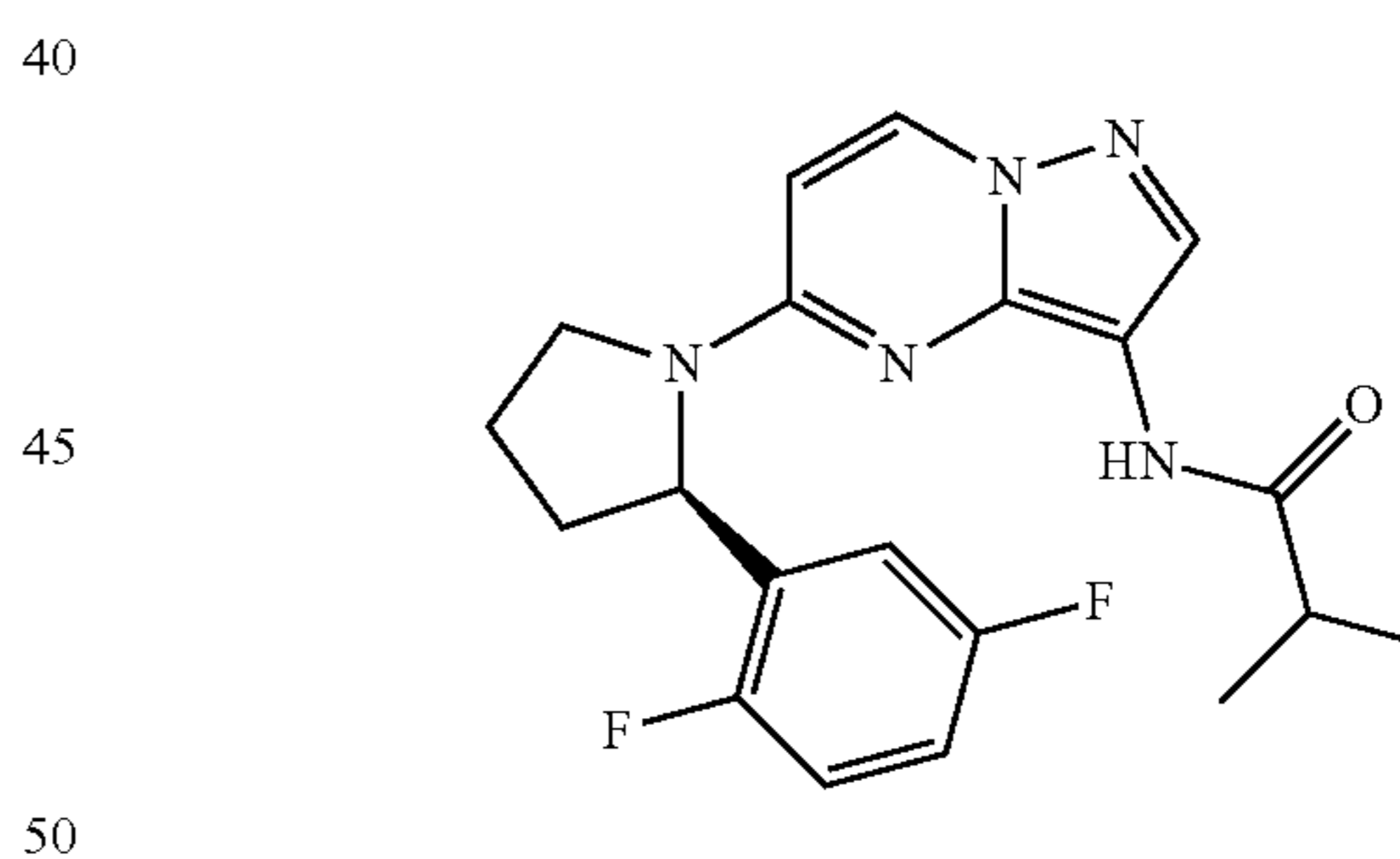
(R)-N-(5-(2-(2,5-difluorophenyl)pyrrolidin-1-yl)pyrazolo[1,5-a]pyrimidin-3-yl)isobutyramide
