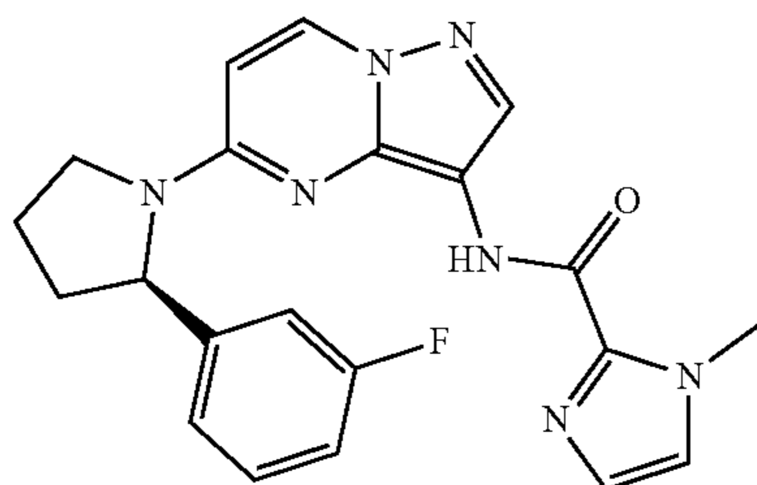
(R)—N-(5-(2-(3-fluorophenyl)pyrrolidin-1-yl)pyrazolo[1,5-a]pyrimidin-3-yl)-1-methyl-1H-imidazole-2-carboxamide
