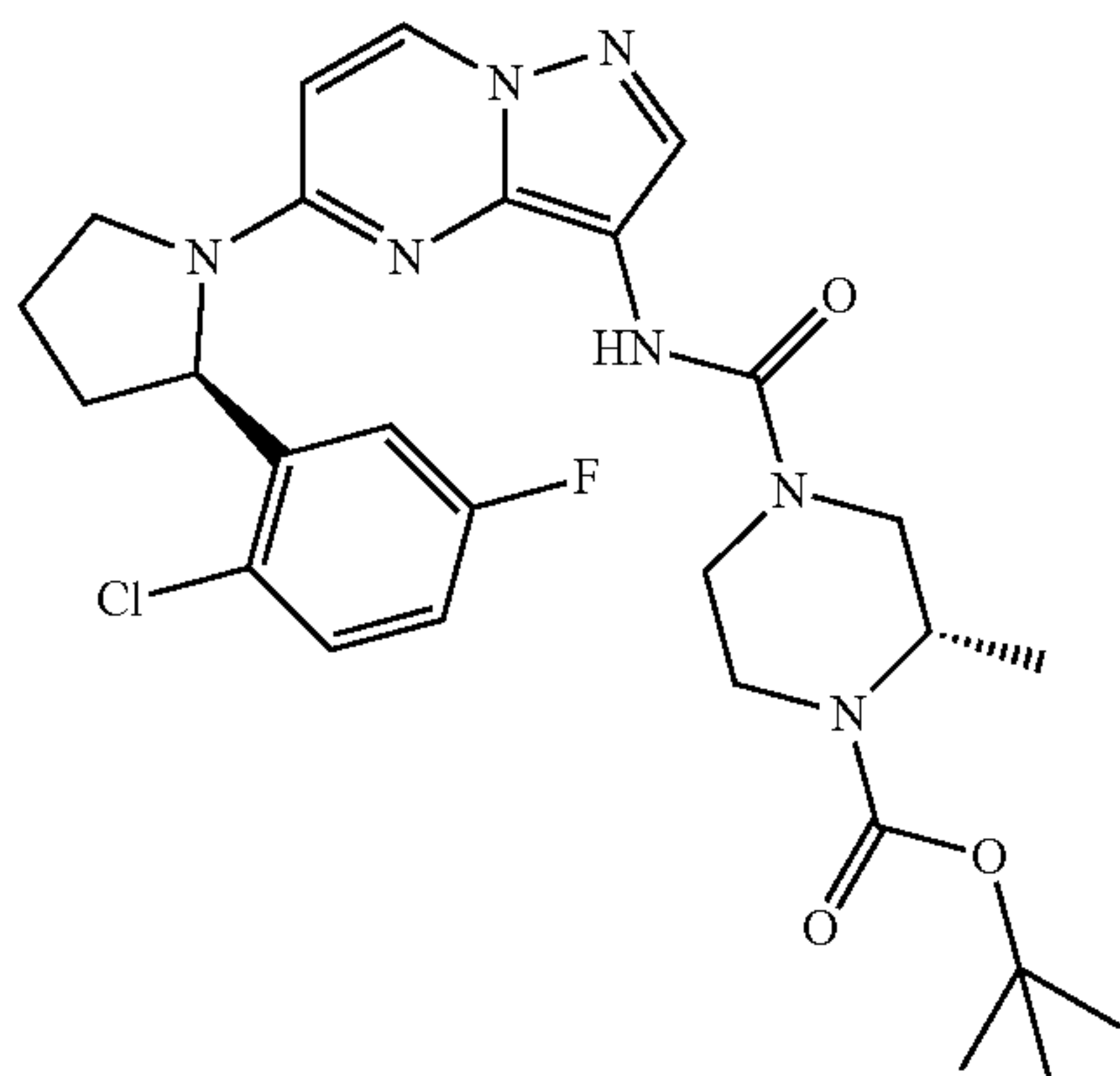
(S)-tert-butyl 4-(5-((R)-2-(2-chloro-5-fluorophenyl)pyrrolidin-1-yl)pyrazolo[1,5-a]pyrimidin-3-ylcarbamoyl)-2-methylpiperazine-1-carboxylate
