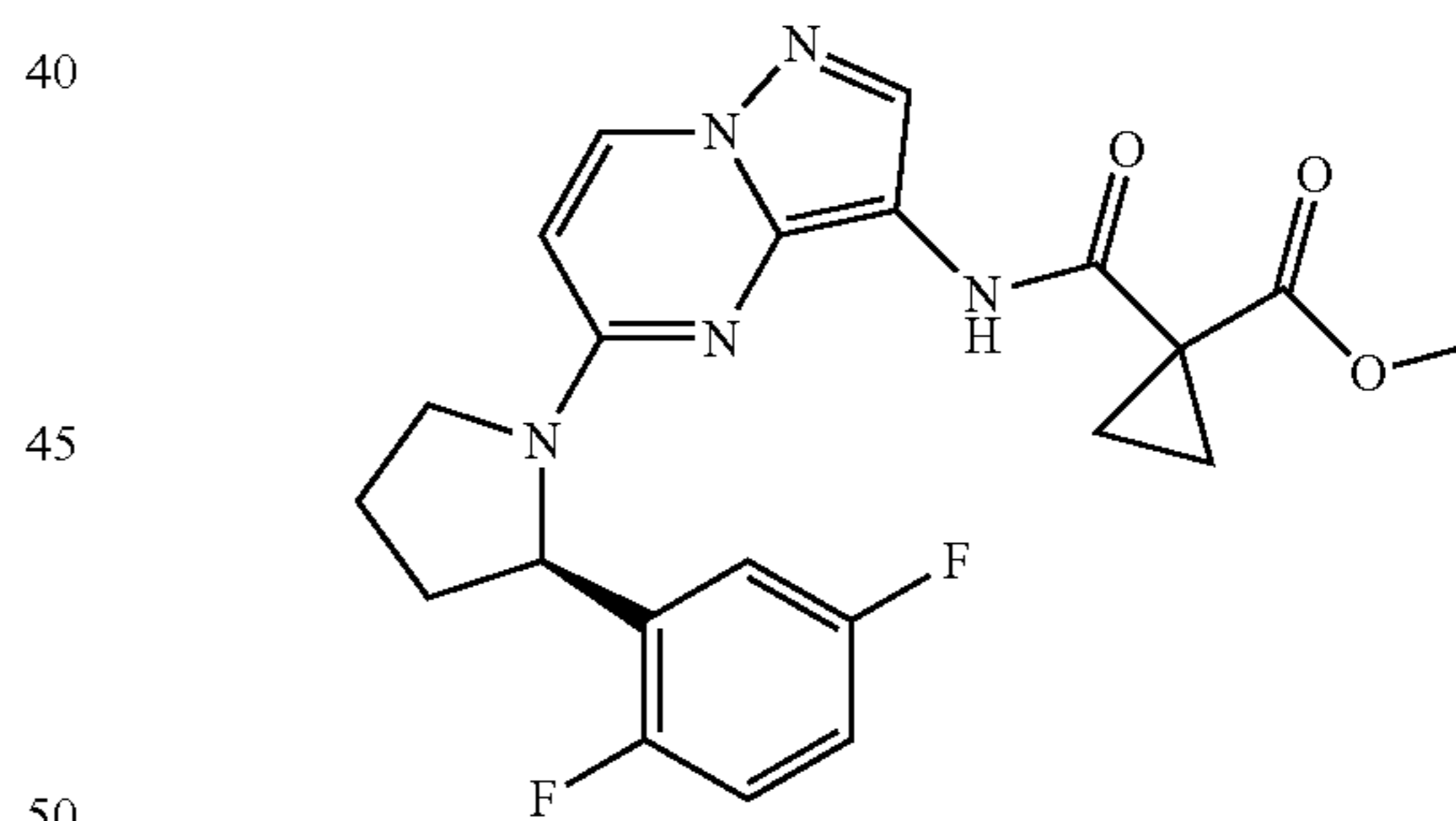
(R)-methyl 1-(5-(2-(2,5-difluorophenyl)pyrrolidin-1-yl)pyrazolo[1,5-a]pyrimidin-3-ylcarbamoyl)cyclopropanecarboxylate
