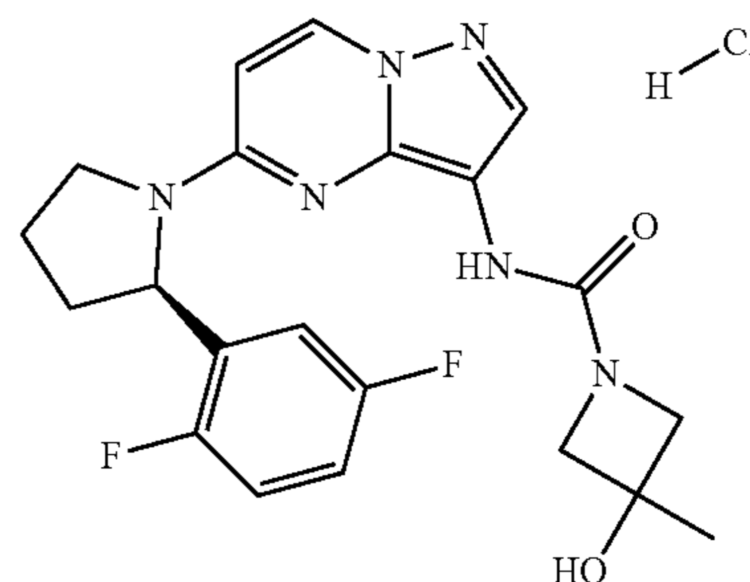
(R)—N-(5-(2-(2,5-difluorophenyl)pyrrolidin-1-yl)pyrazolo[1,5-a]pyrimidin-3-yl)-3-hydroxy-3-methylazetidide-1-carboxamide hydrochloride
