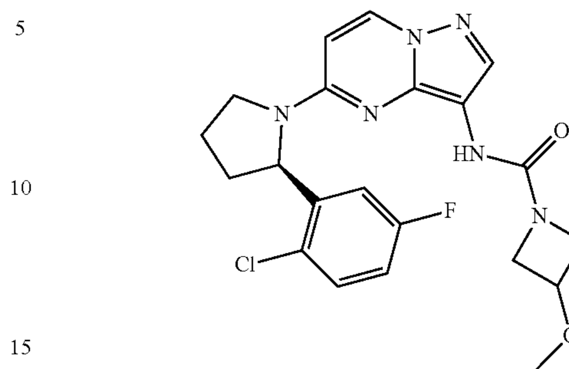
(R)-N-(5-(2-(2-chloro-5-fluorophenyl)pyrrolidin-1-yl)pyrazolo[1,5-a]pyrimidin-3-yl)-3-methoxyazetidine-1-carboxamide
