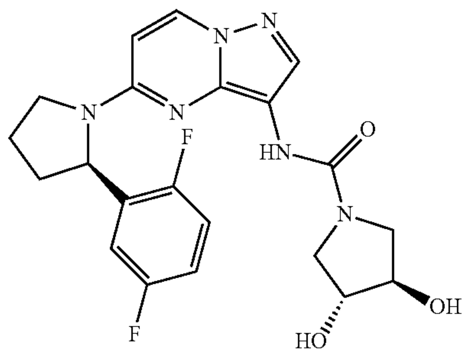
(3R,4R)—N-(5-((R)-2-(2,5-difluorophenyl)pyrrolidin-1-yl)pyrazolo[1,5-a]pyrimidin-3-yl)-3,4-dihydroxypyrrolidine-1-carboxamide
