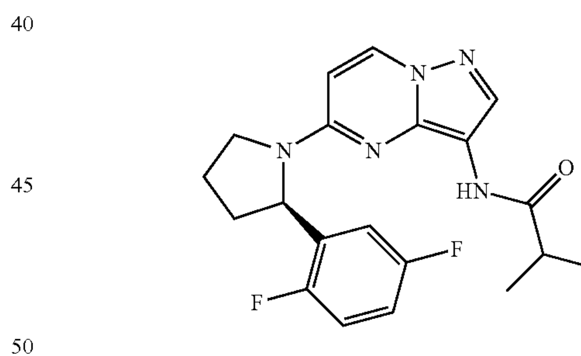
(R)-N-(5-(2-(2,5-difluorophenyl)pyrrolidin-1-yl)pyrazolo[1,5-a]pyrimidin-3-yl)isobutyramide
