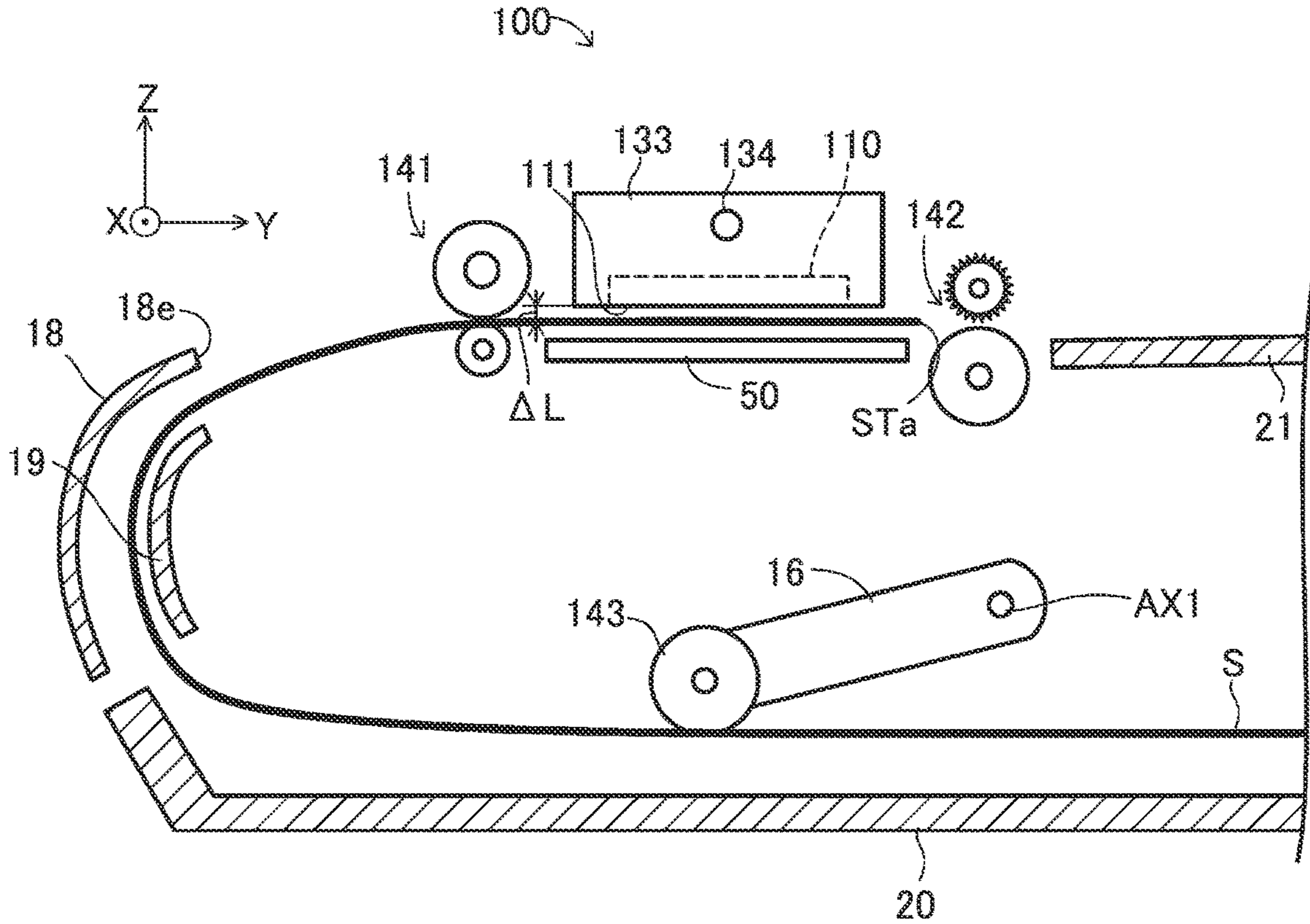
FIG. 4B FIRST HOLDING STATE S1
