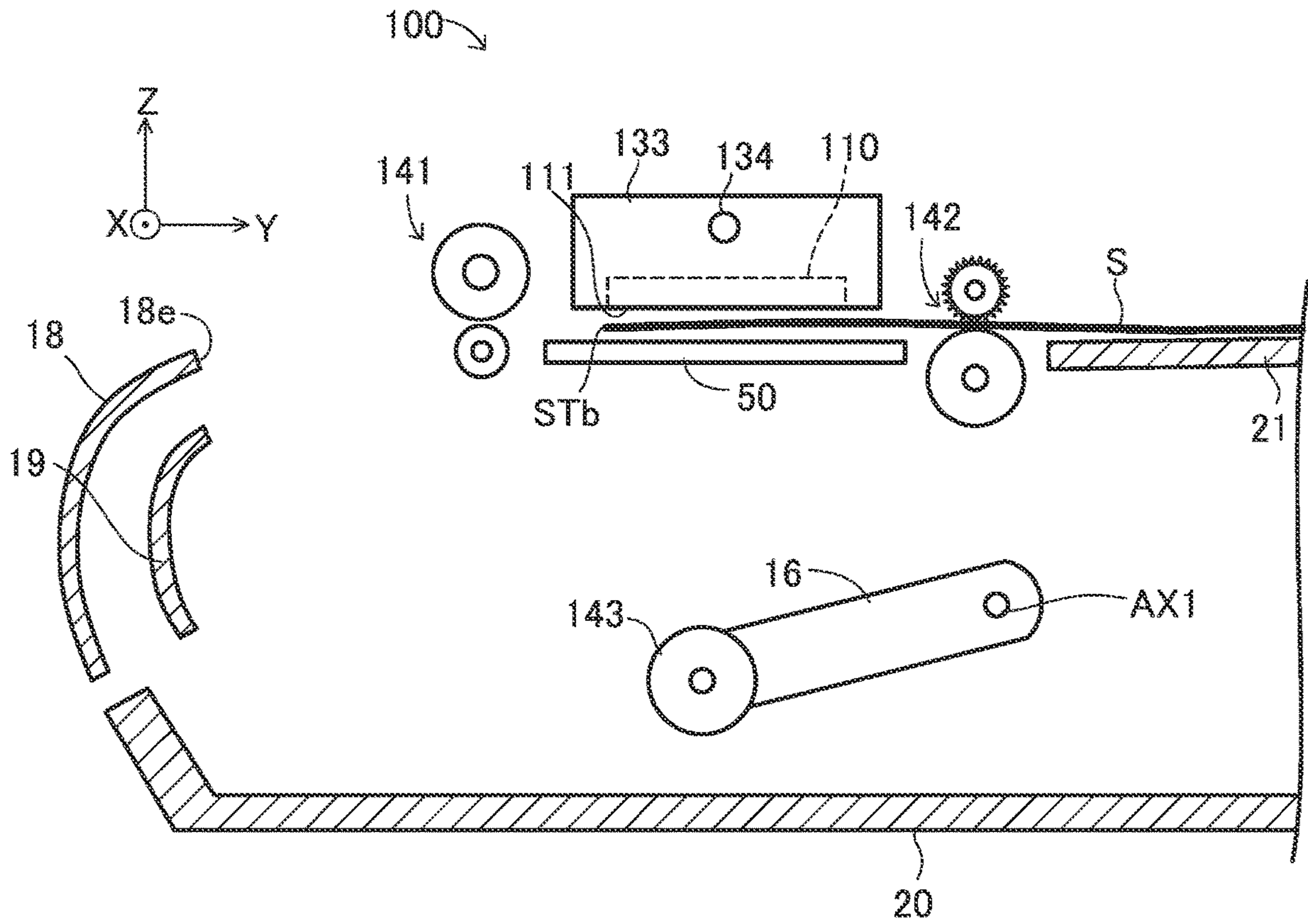
FIG. 6 FOURTH HOLDING STATE S1
