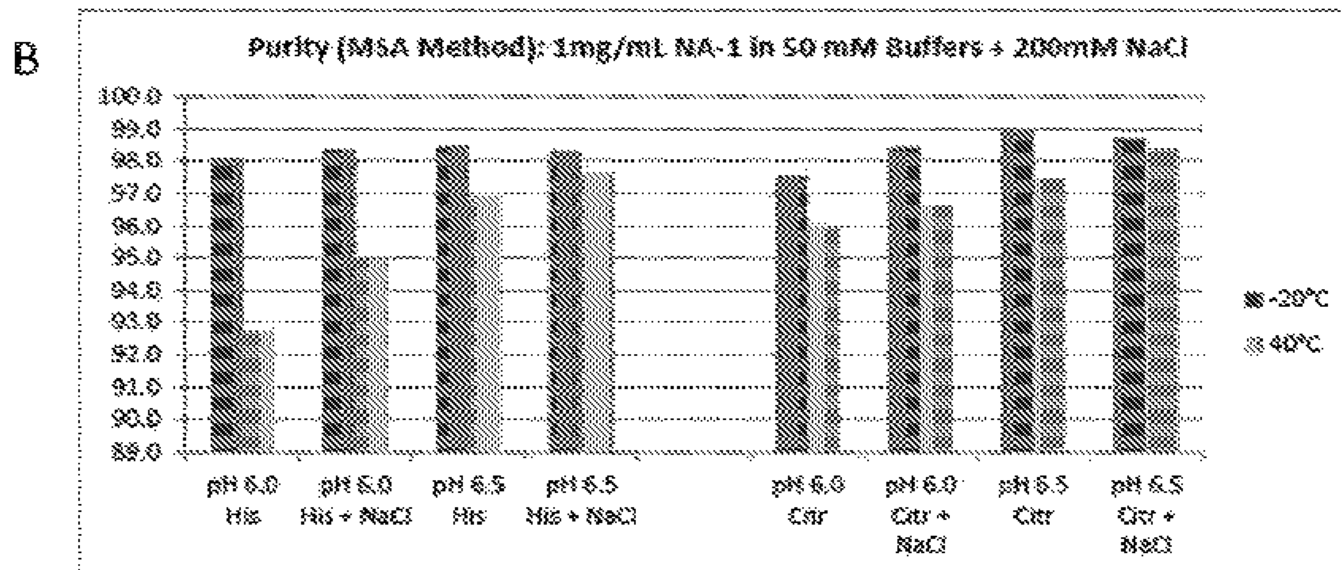
Figure II. Plot of Purity Results, MSA Method (Ordered by pH)
