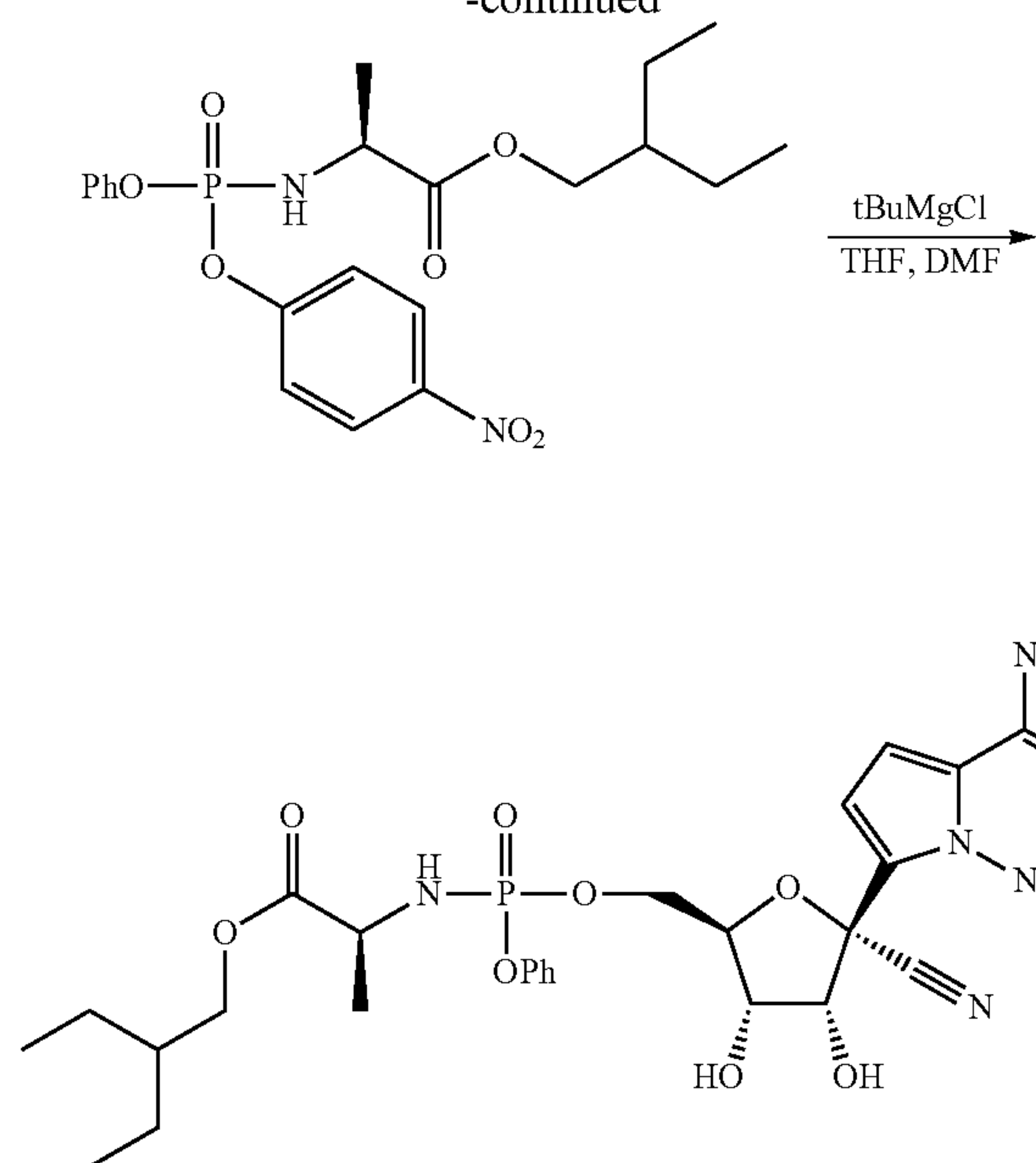
(2S)-2-ethylbutyl 2-((((2R,3S,4R,5R)-5-(4-aminopyrrolo[2,1-f][1,2,4]triazin-7-yl)-5-cyano-3,4-dihydroxytetrahydrofuran-2-yl)methoxy)(phenoxy)phosphoryl)amino) propanoate
