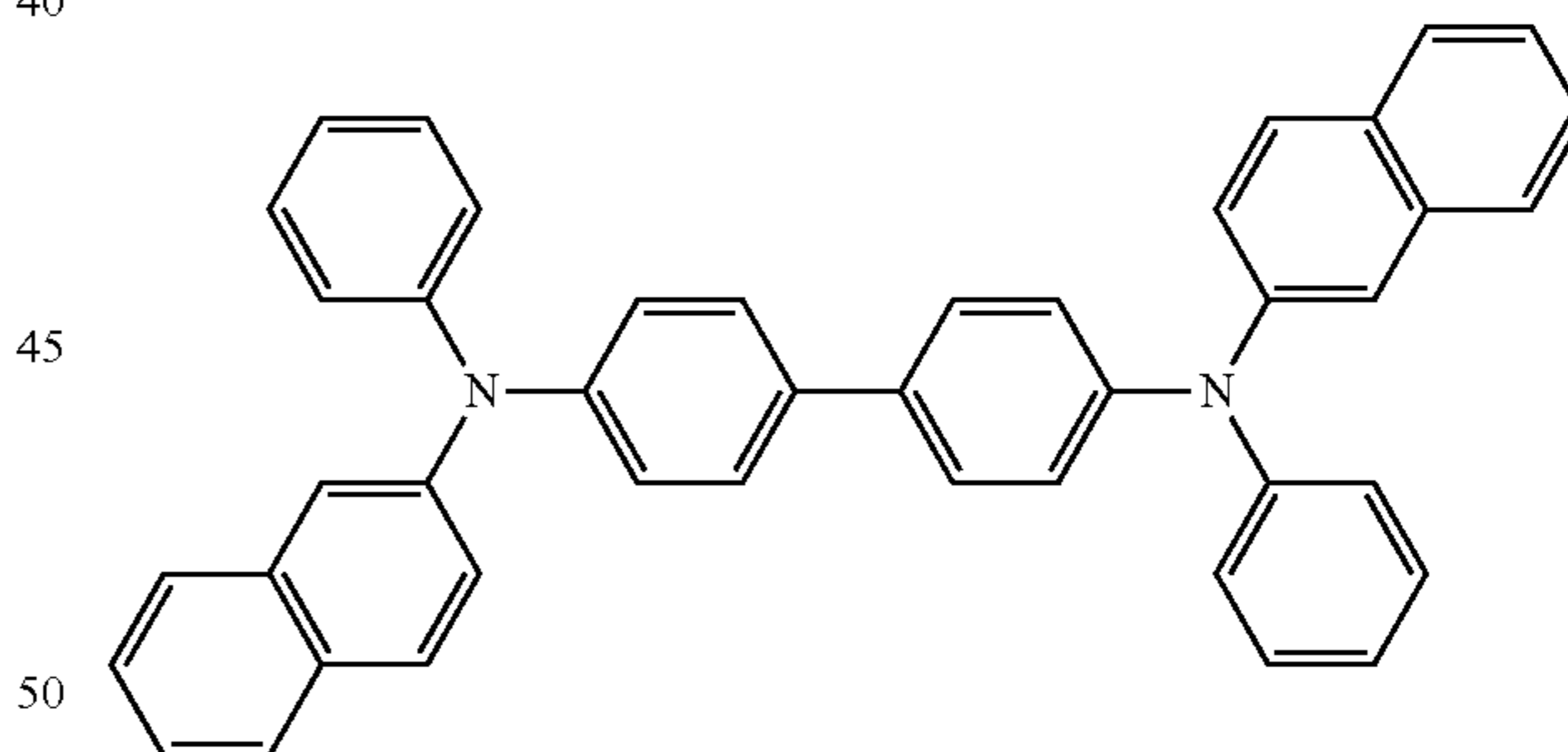
\beta -NPB
