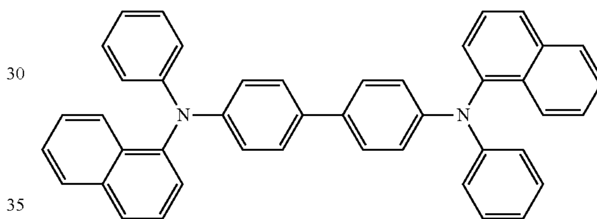
NPB
