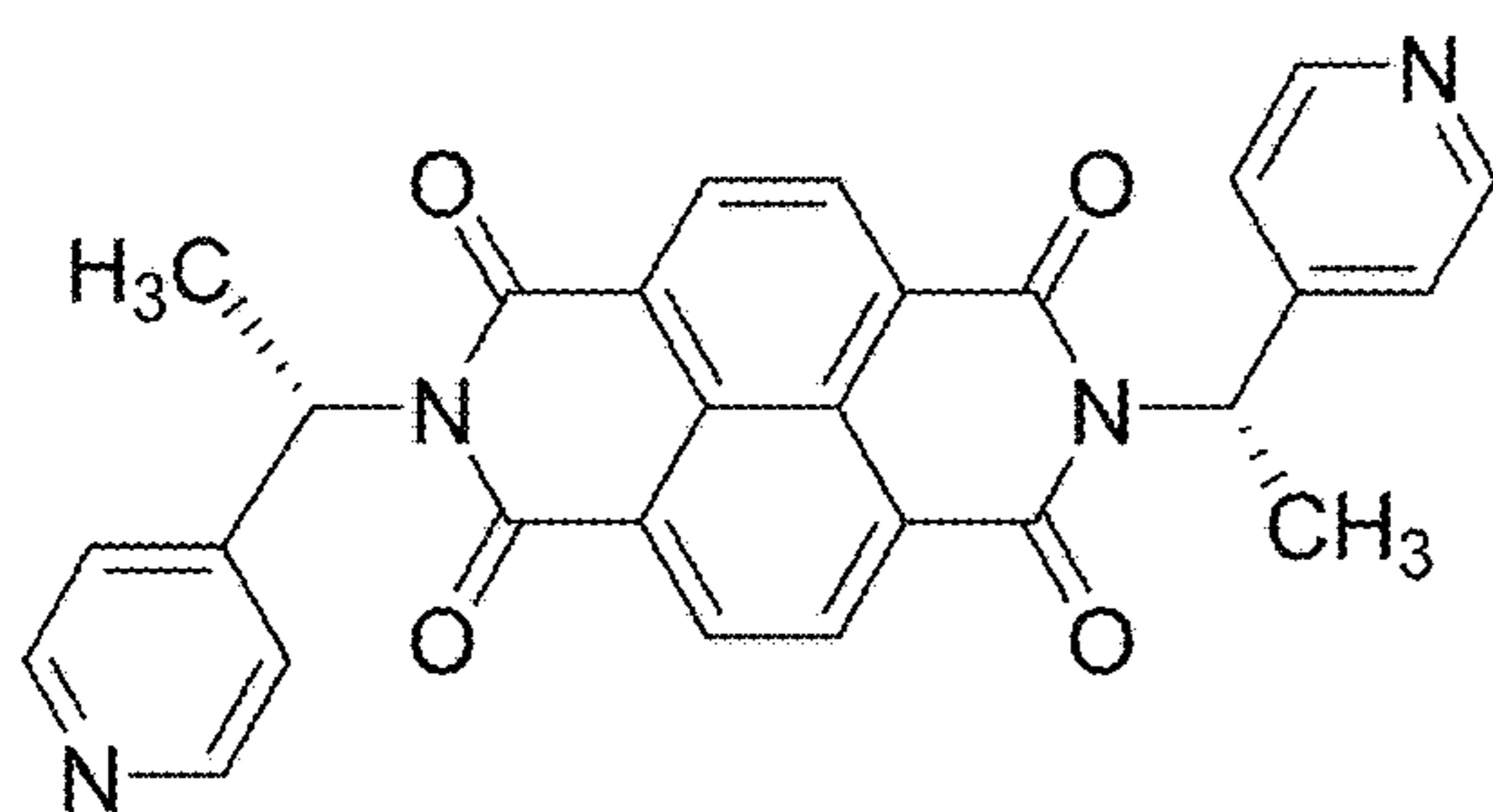
(S)-4-PyENDI
