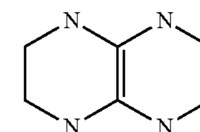
pyrazino[2,3-b]pyrazine 1,2,3,4,5,6,7,8-octahydropyrazino[2,3-b]pyrazine
