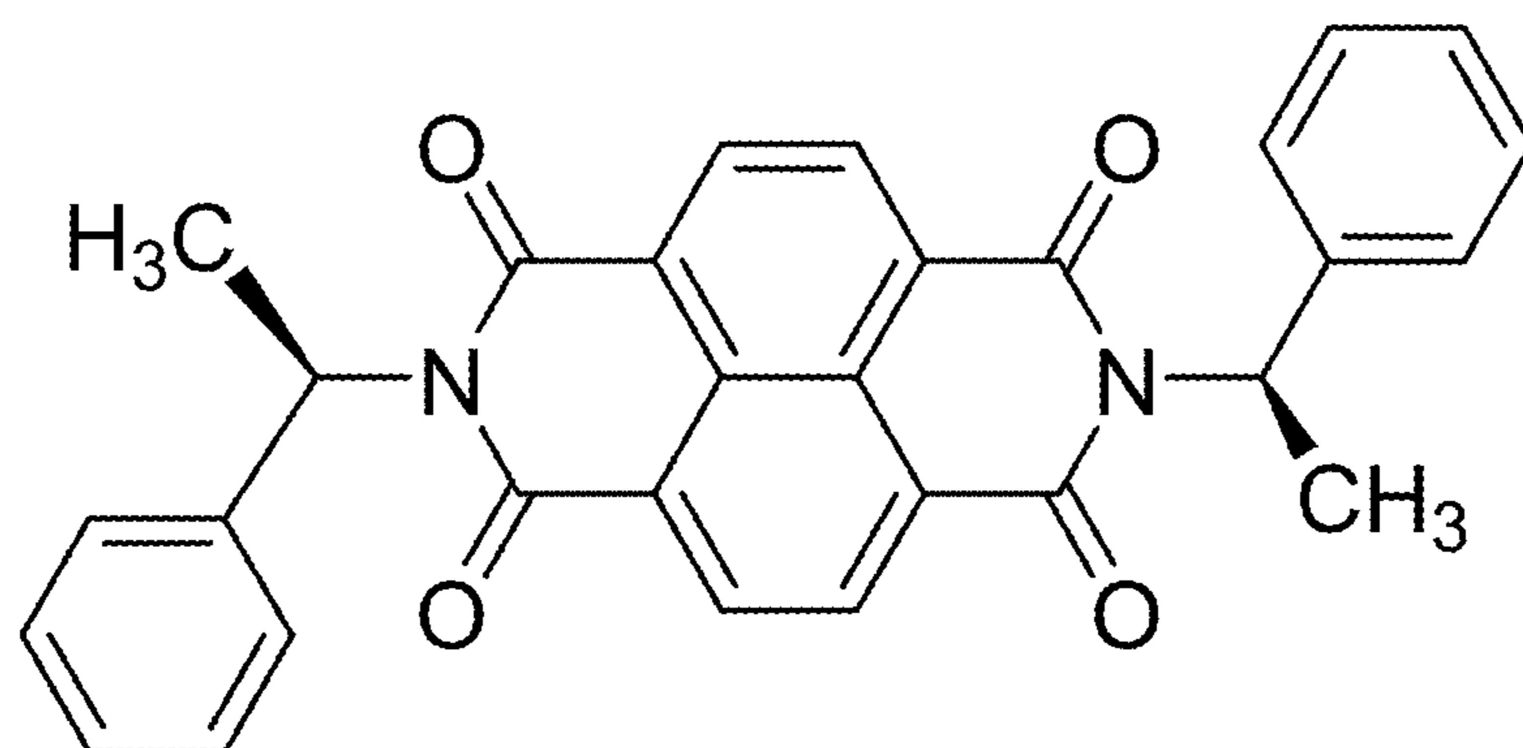
(R)-PhENDI
