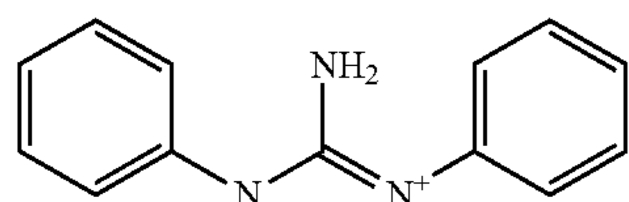
[Amino(anilino)methylene]-phenyl-ammonium
