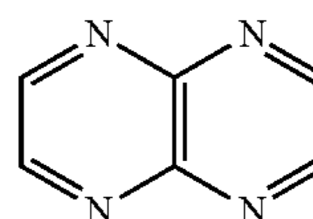
pyrazino[2,3-b]pyrazine 1,2,3,4,5,6,7,8-octahydropyrazino[2,3-b]pyrazine
