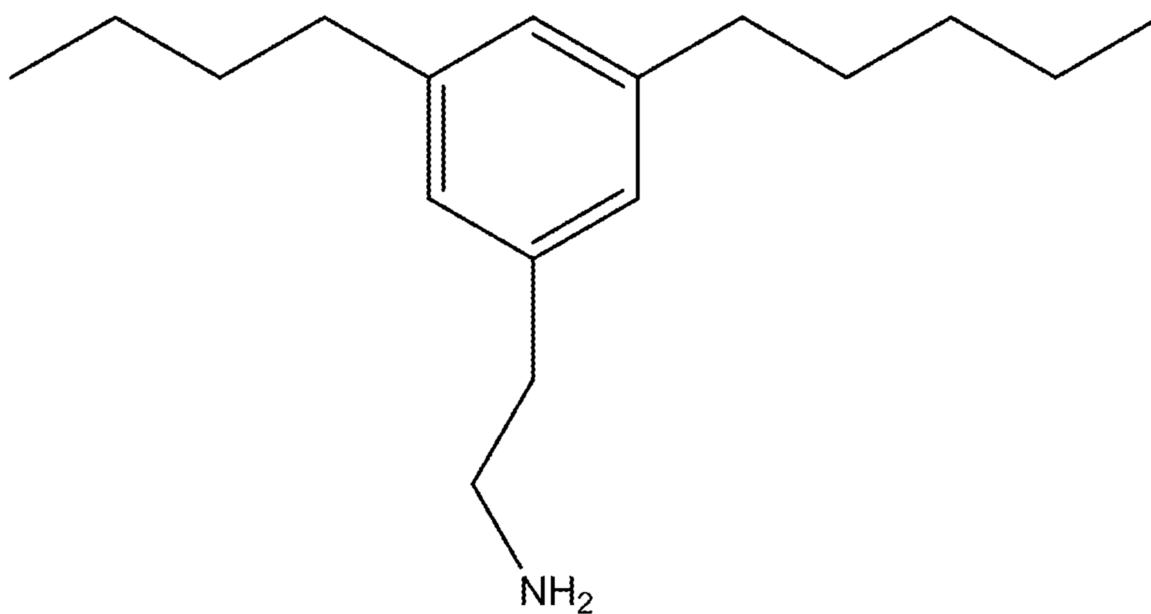
1-(3-Butyl-5-pentyl-2-phenyl)ethanamine
