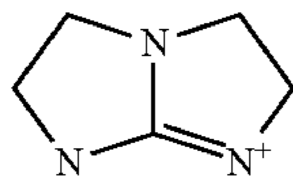
2,3,5,6-Tetrahydro-1H-imidazo[1,2-a]imidazol-7-ium
