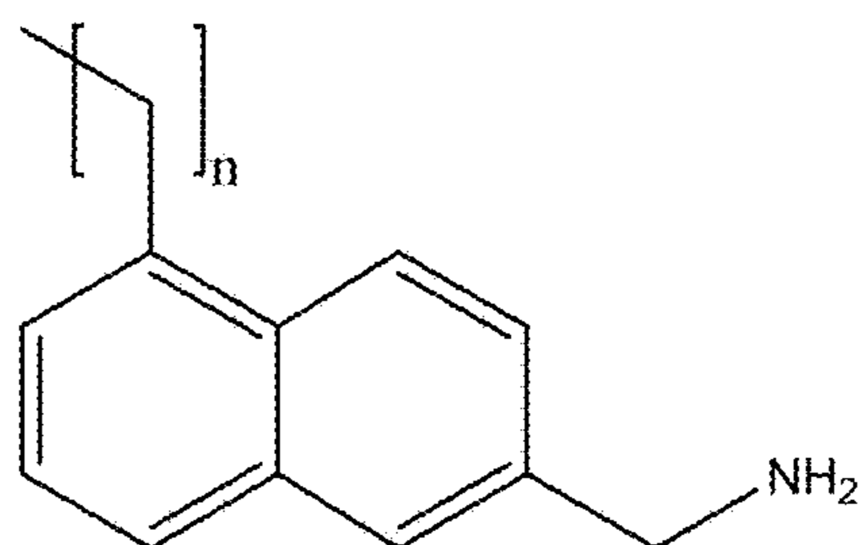
2-Methylamine-6-alkyl-Naphthalene
