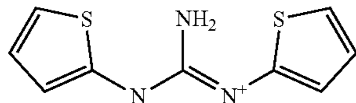
[Amino-(2-thienylamino)methylene]-(2-thienyl)ammonium
