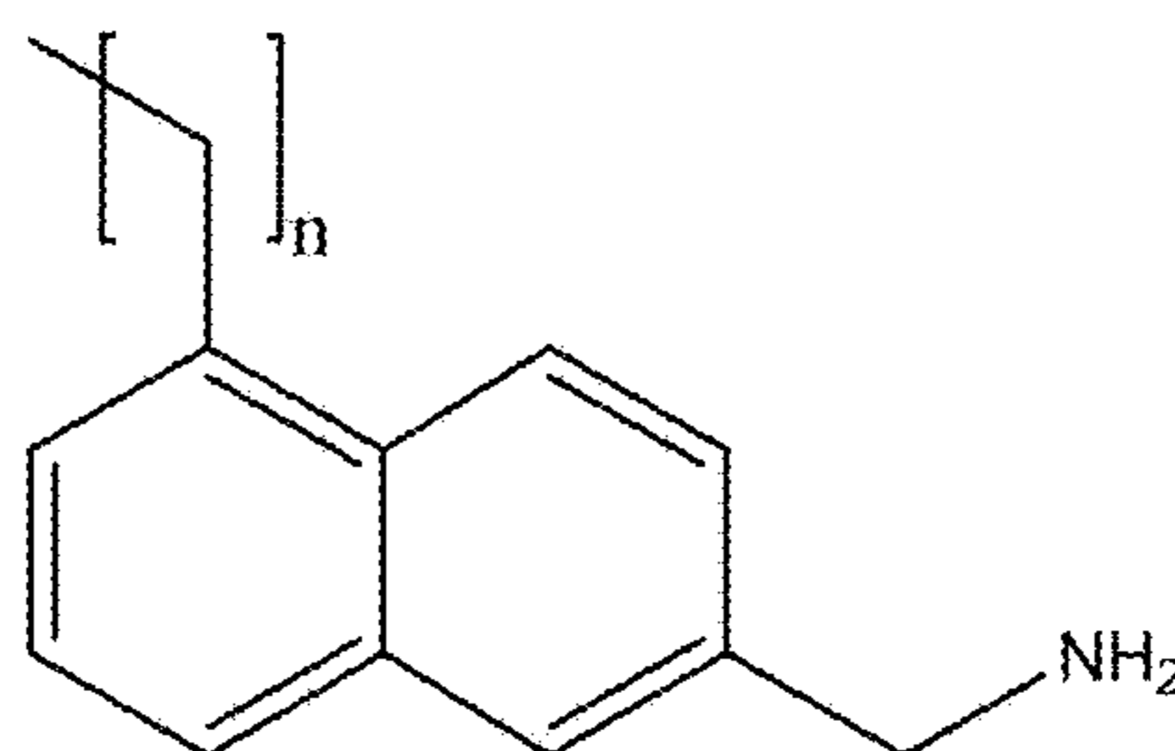
2-Methylamine-6-alkyl-Naphthalene
