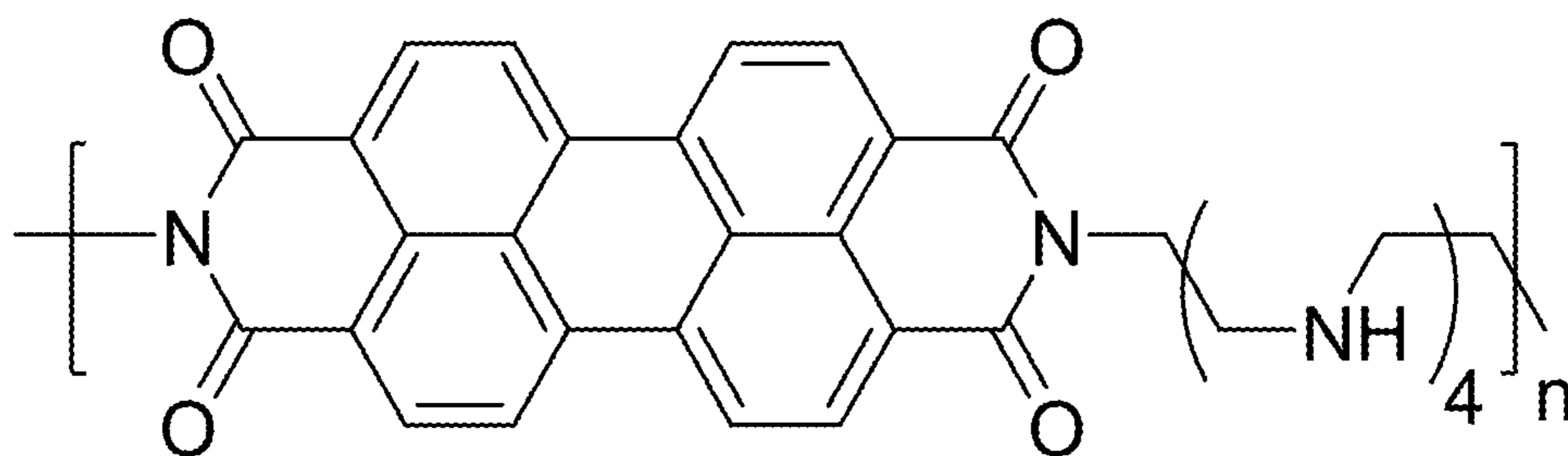
poly-PMHAPDI
