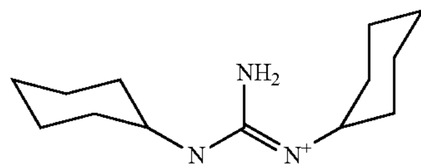
[Amino-(cyclohexylamino)methylene]-cyclohexyl-ammonium
