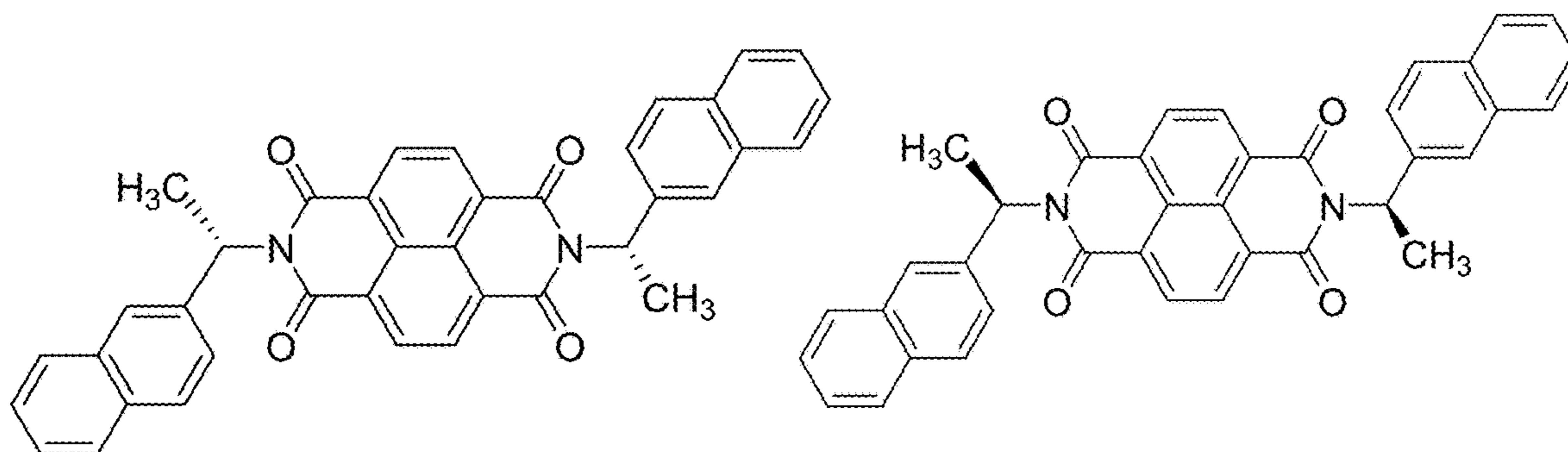
(R)-2-NaphENDI
