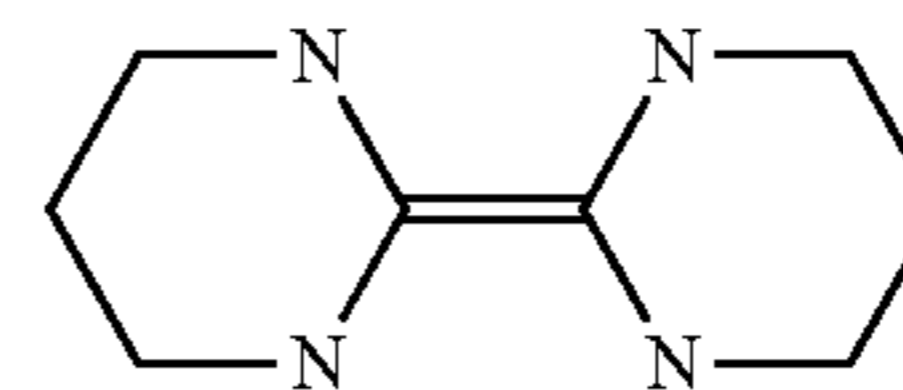
2-hexahydropyrimidin-2-ylidenehexahydropyrimidine
