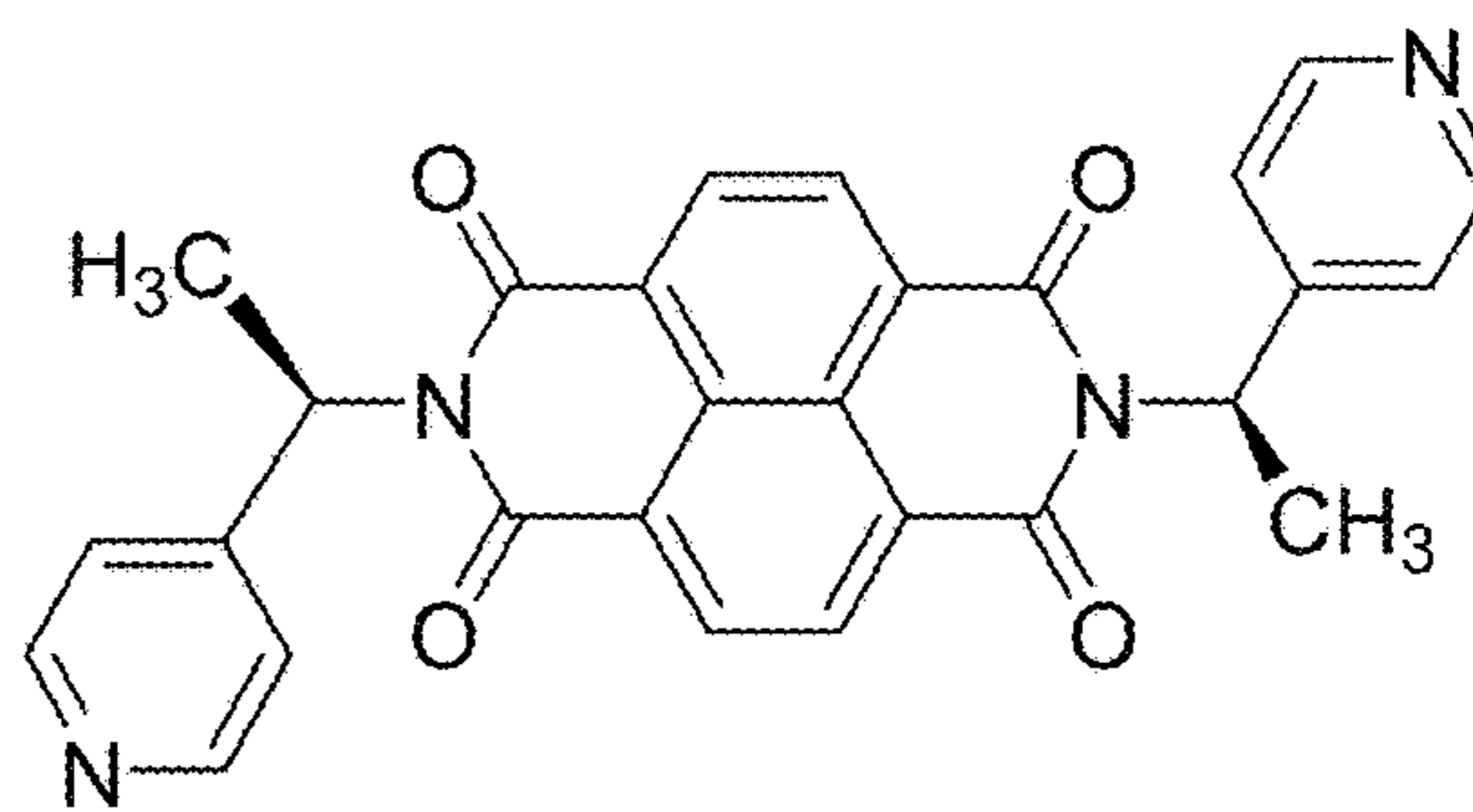
(R)-4-PyENDI
