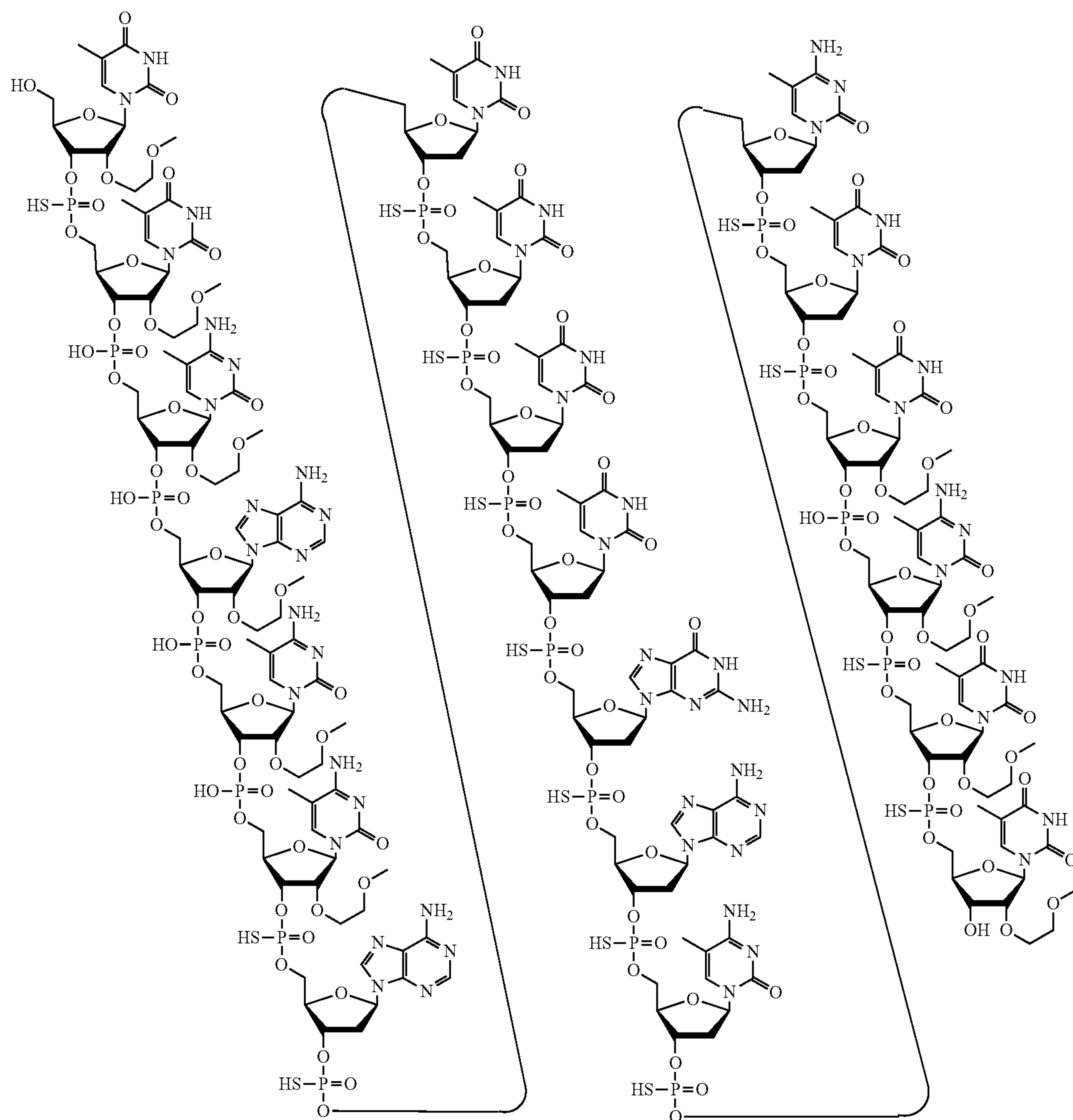
Structure 5. Compound No. 1263518
