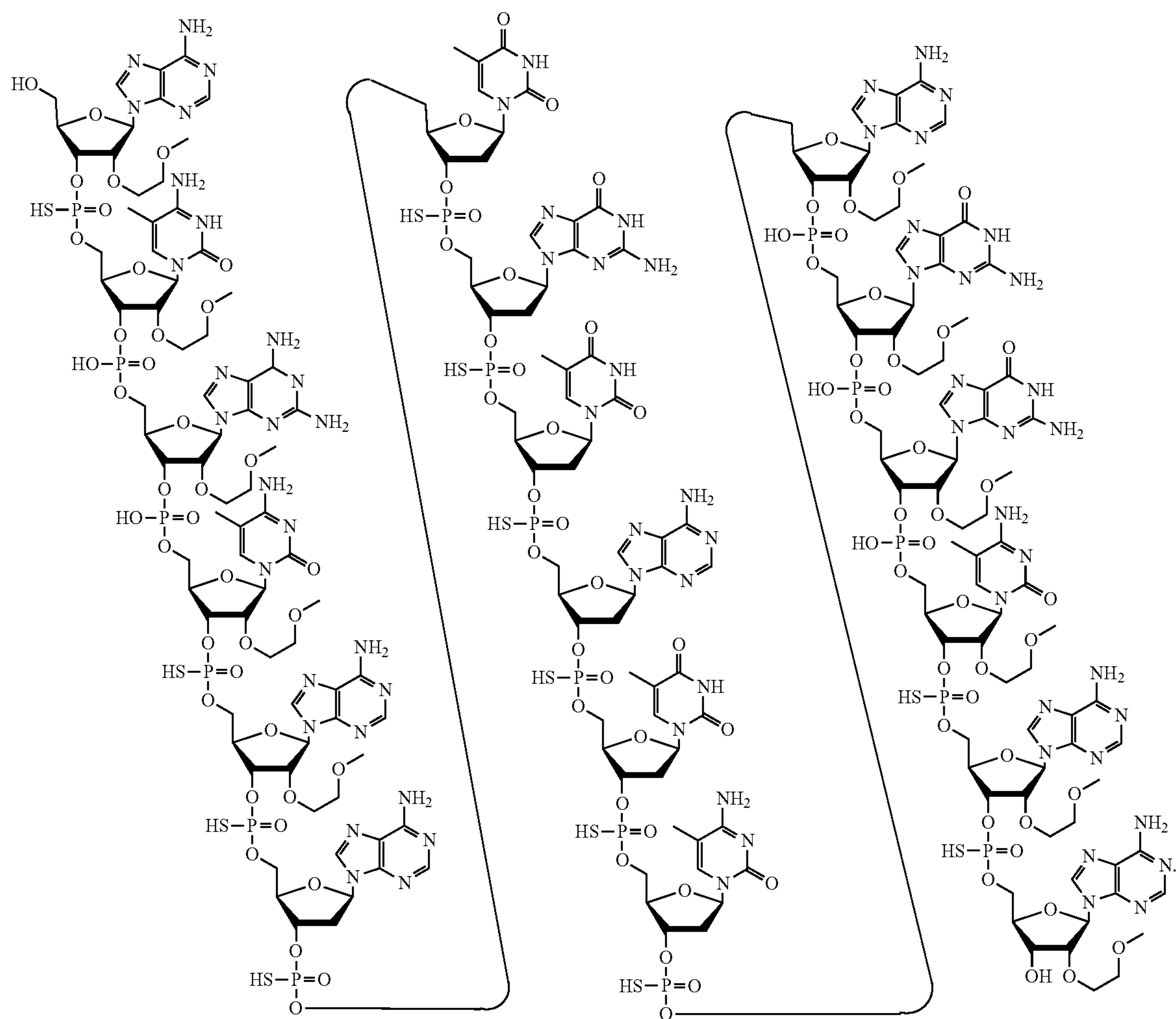
Structure 9. Compound No. 1273039
