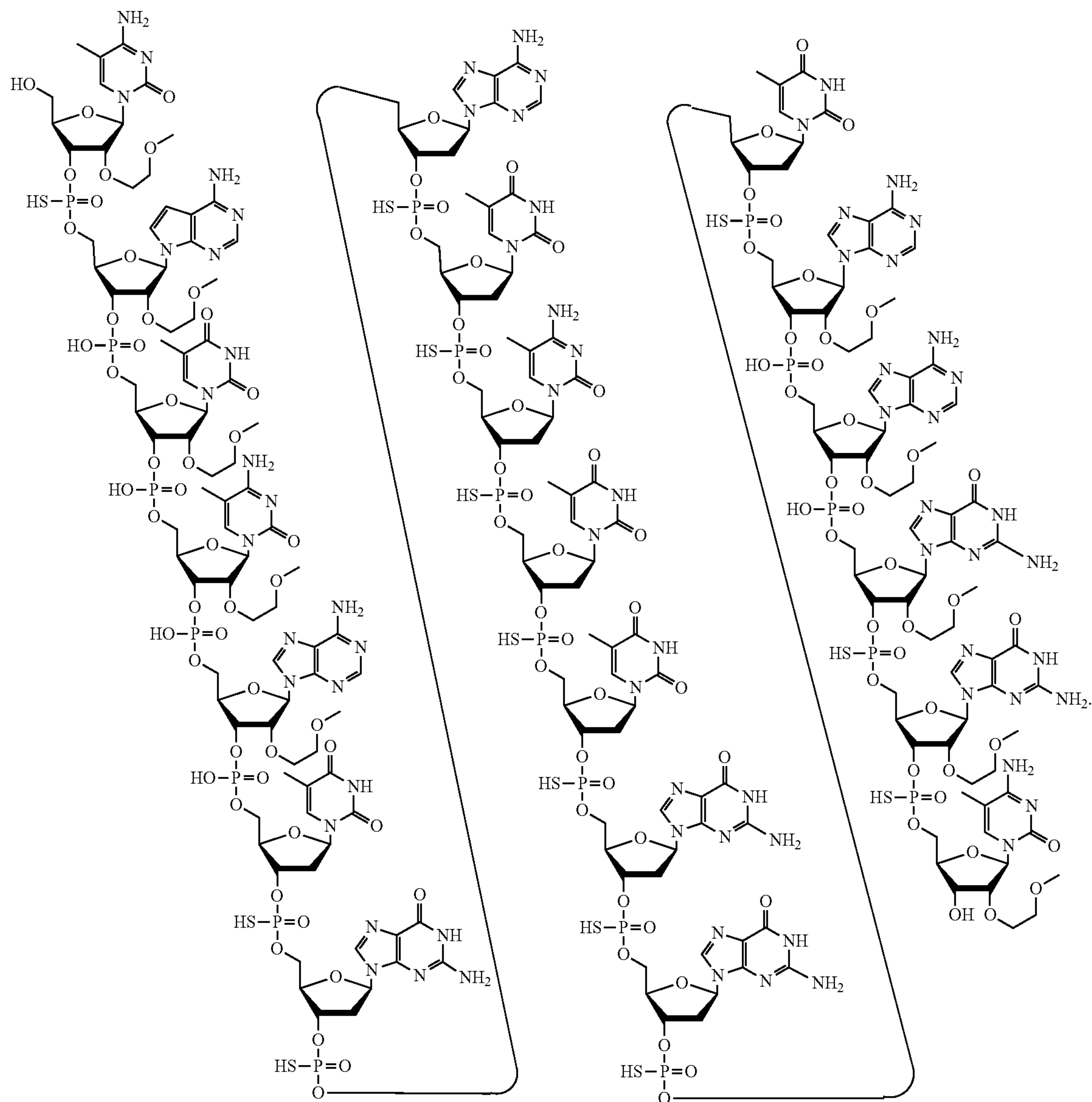
Structure 1. Compound No. 1065645
