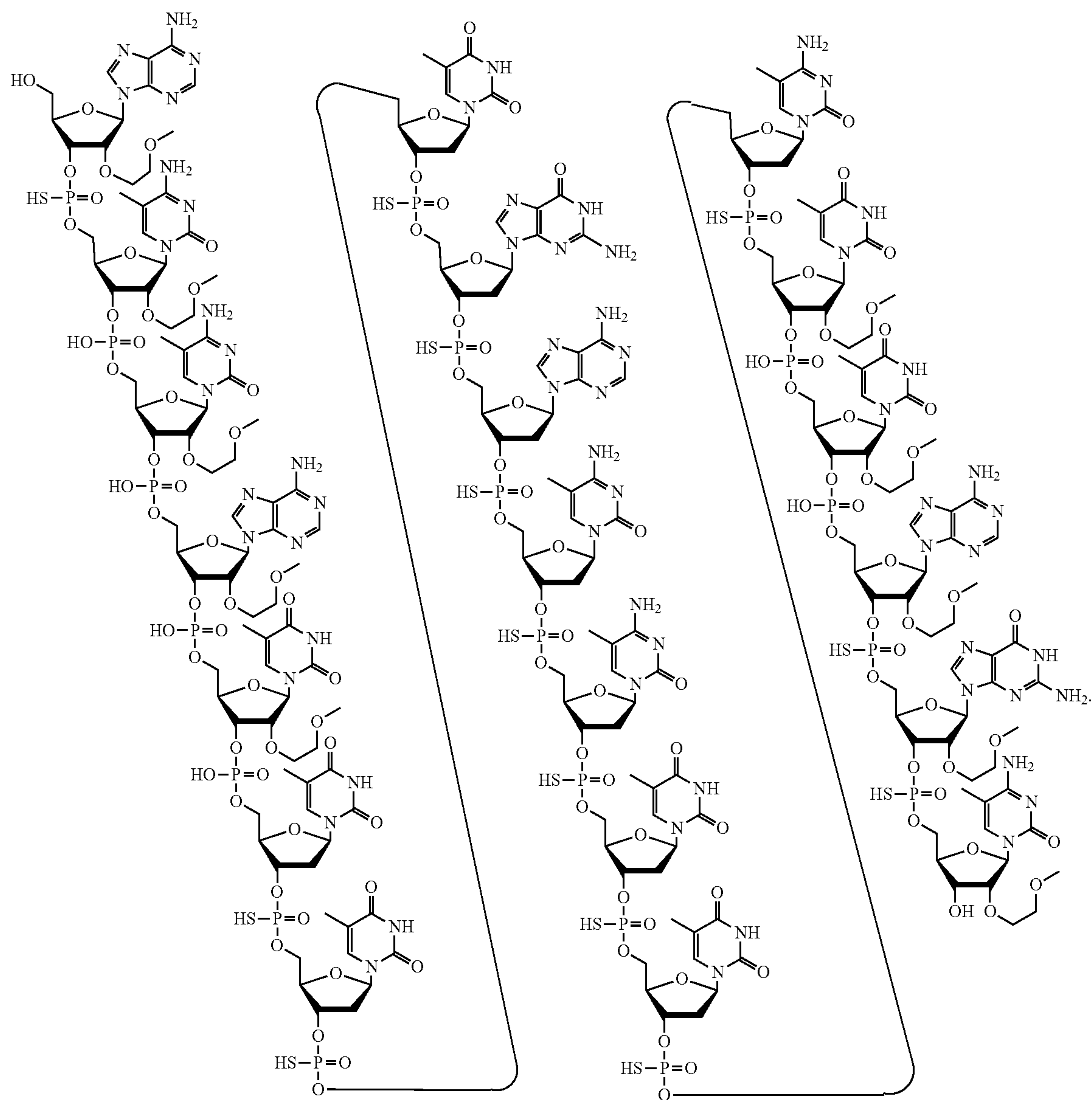
Structure 11. Compound No. 1273062
