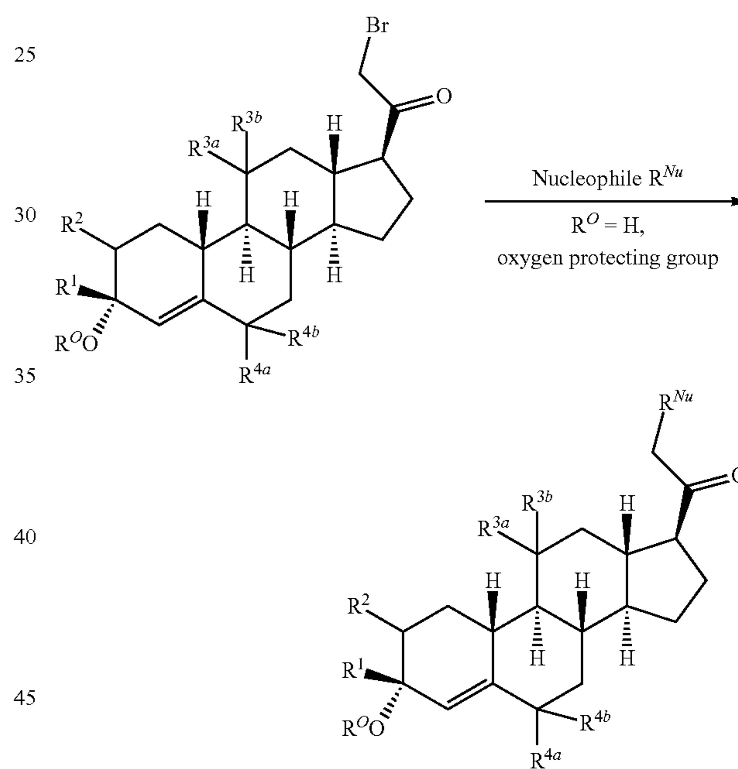
Scheme 3
