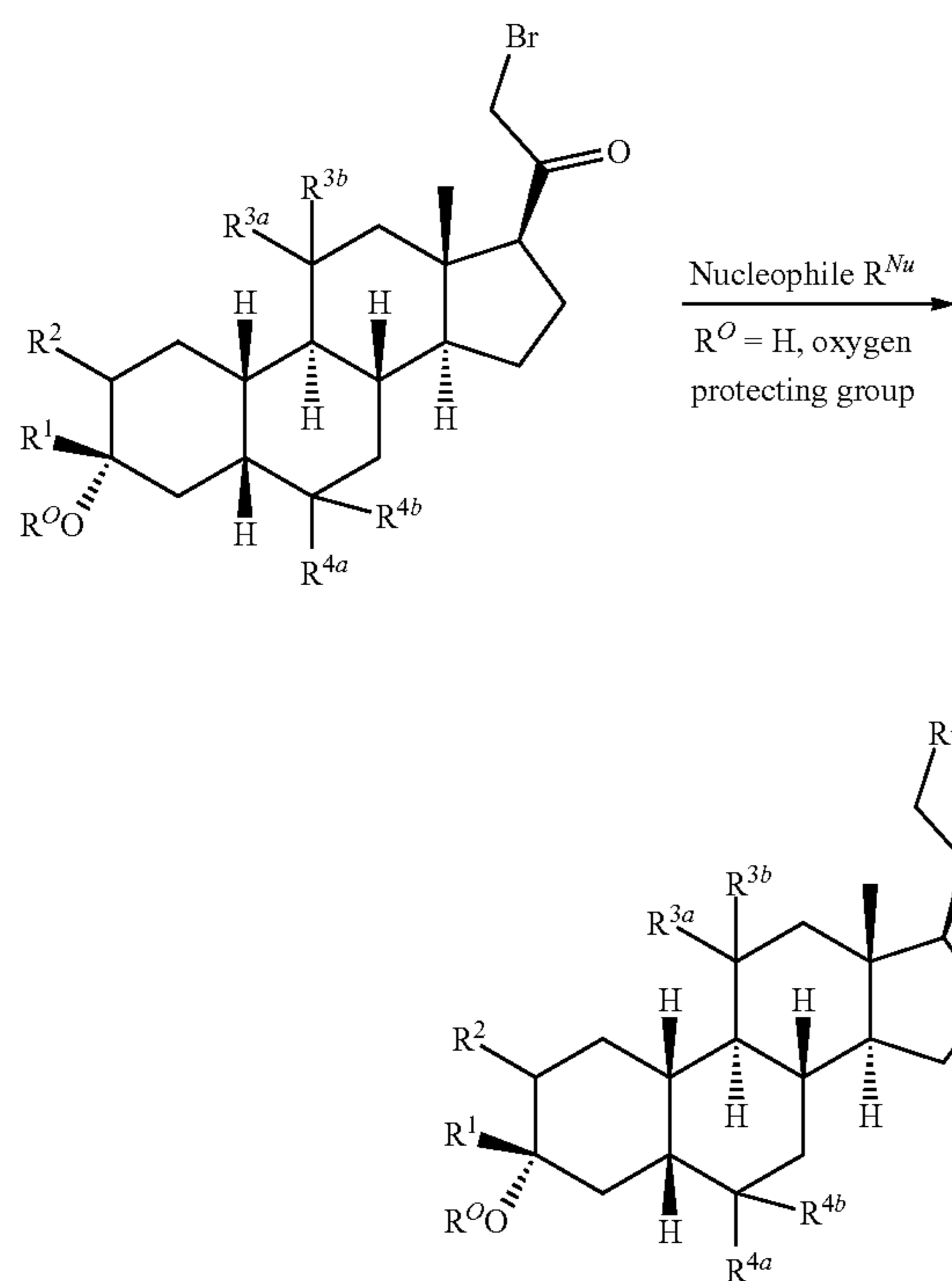
Scheme 1
