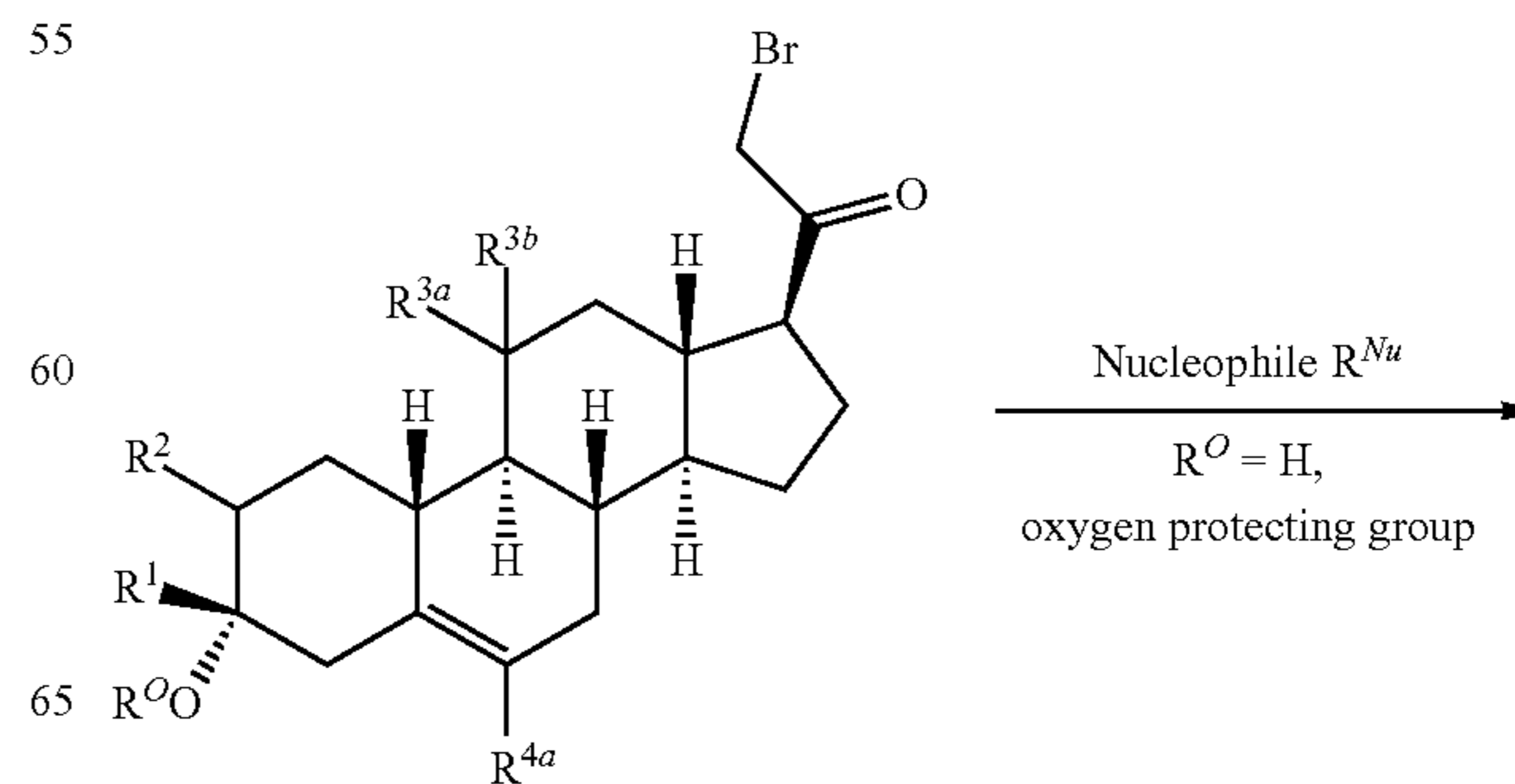
Scheme 4
