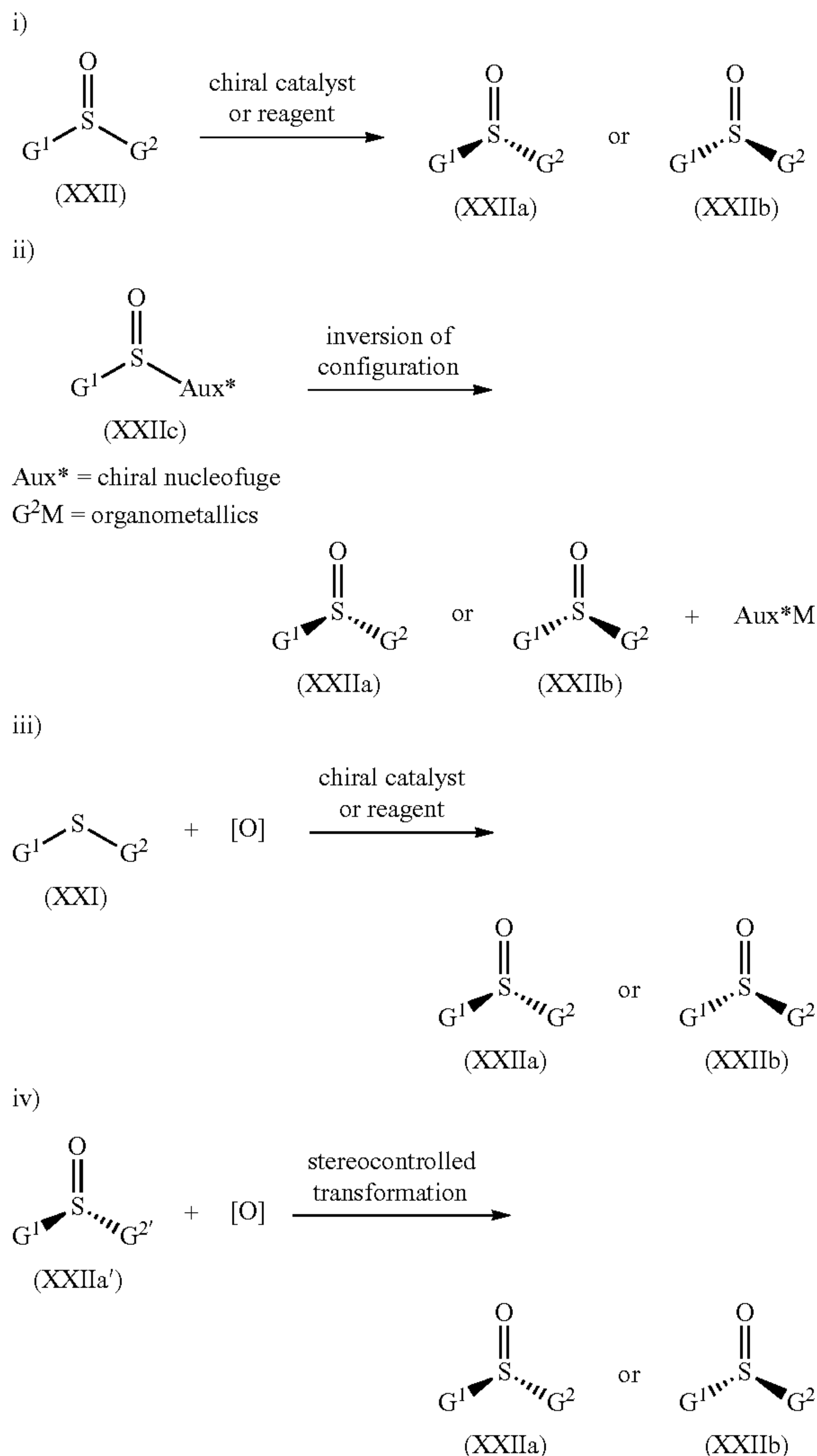
Scheme 12
