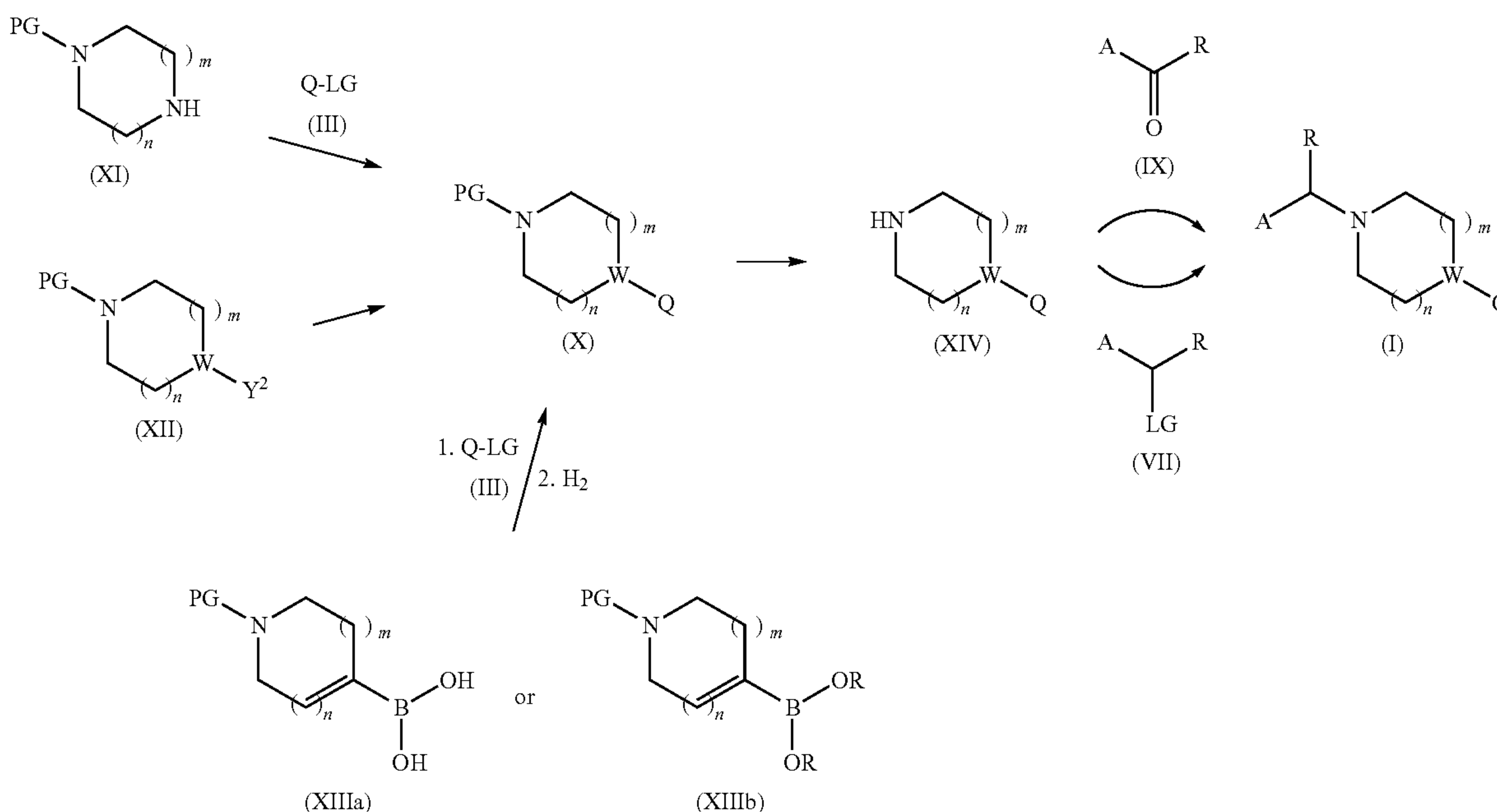
Scheme 5
