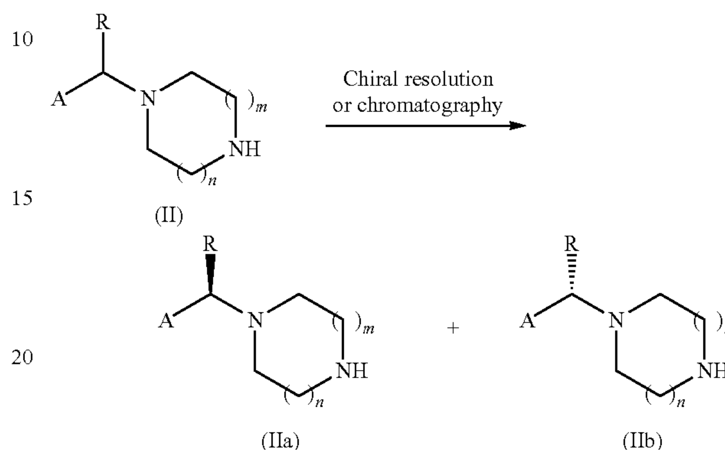
Scheme 6
