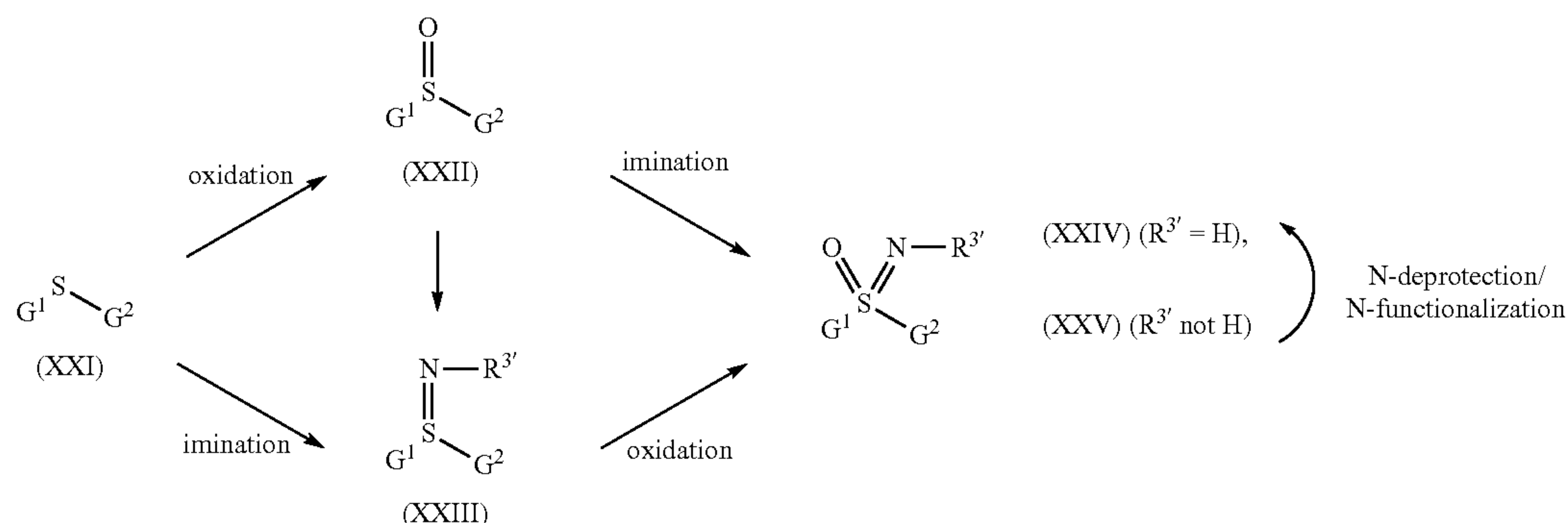
Scheme 10
