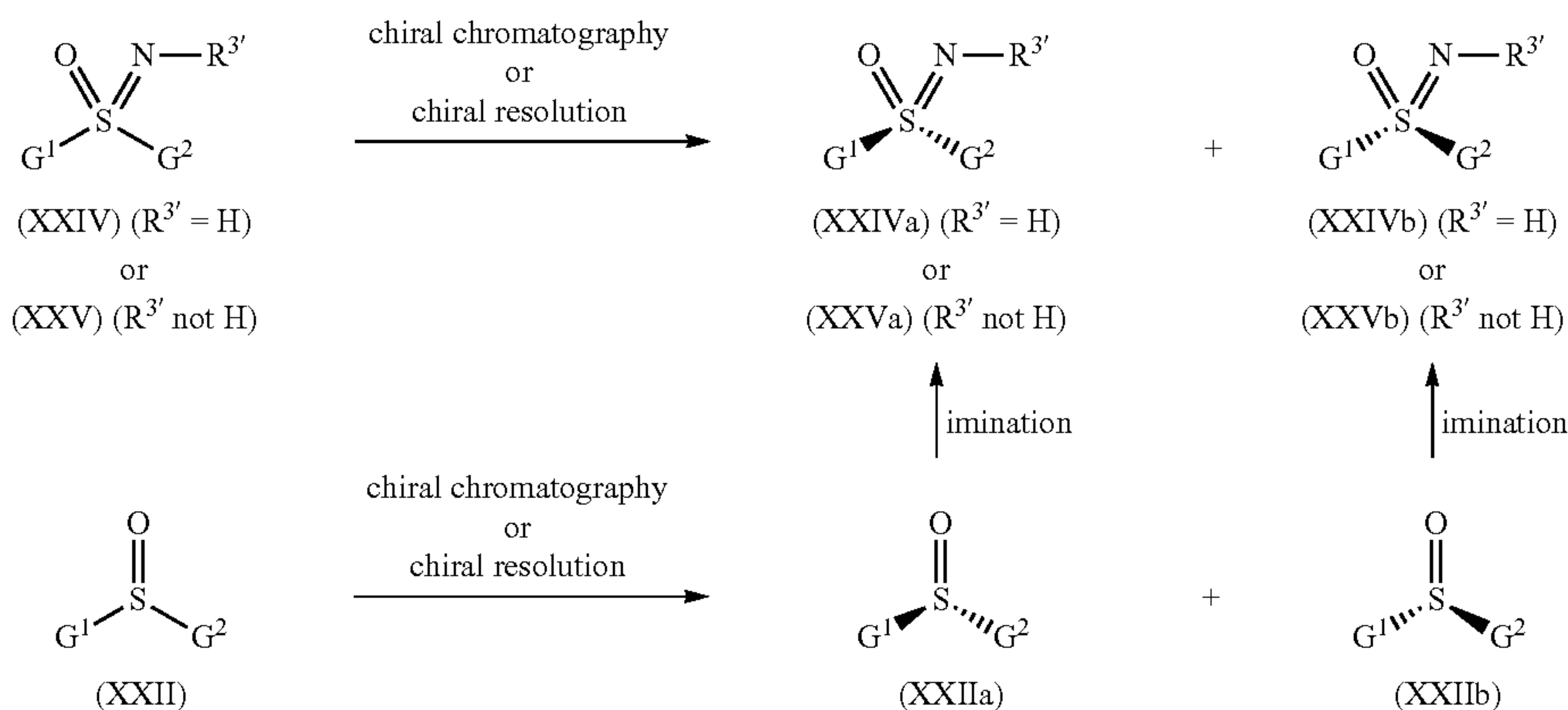
Scheme 11
