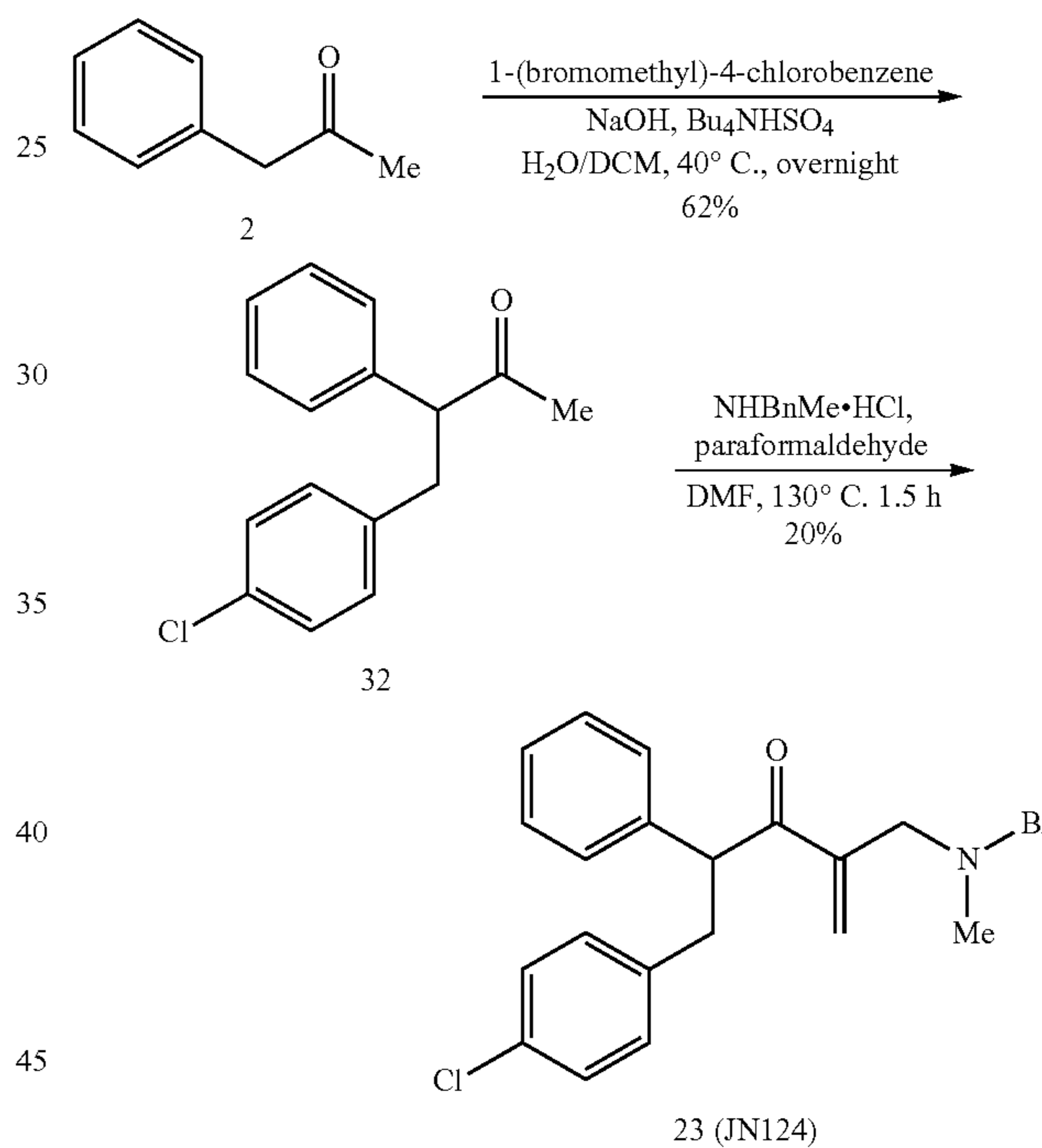
4-(4-Chlorophenyl)-3-phenylbutan-2-one (32)
