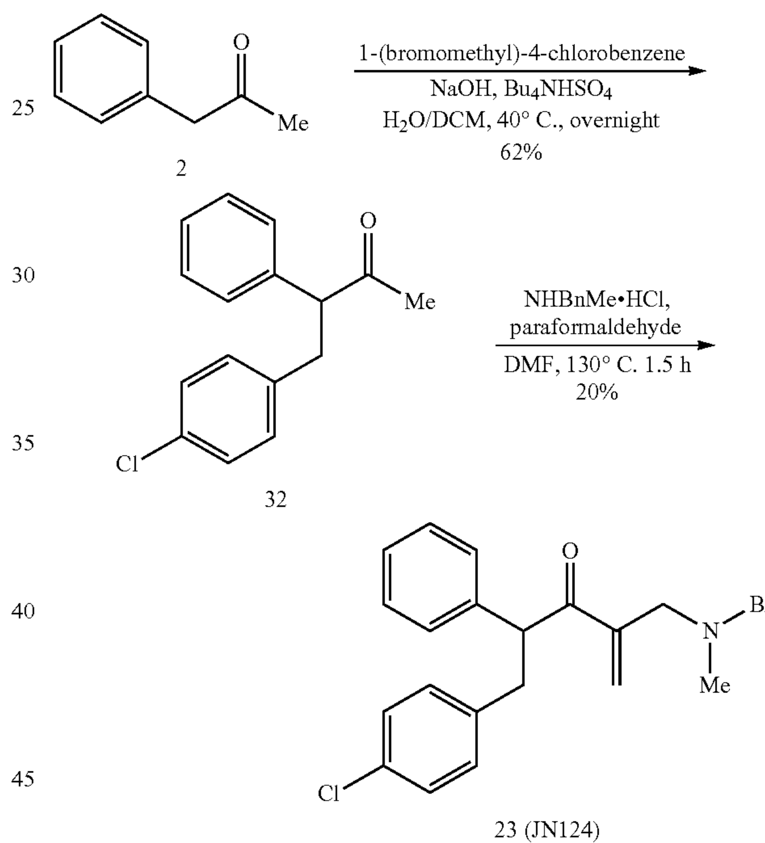
4-(4-Chlorophenyl)-3-phenylbutan-2-one (32)
