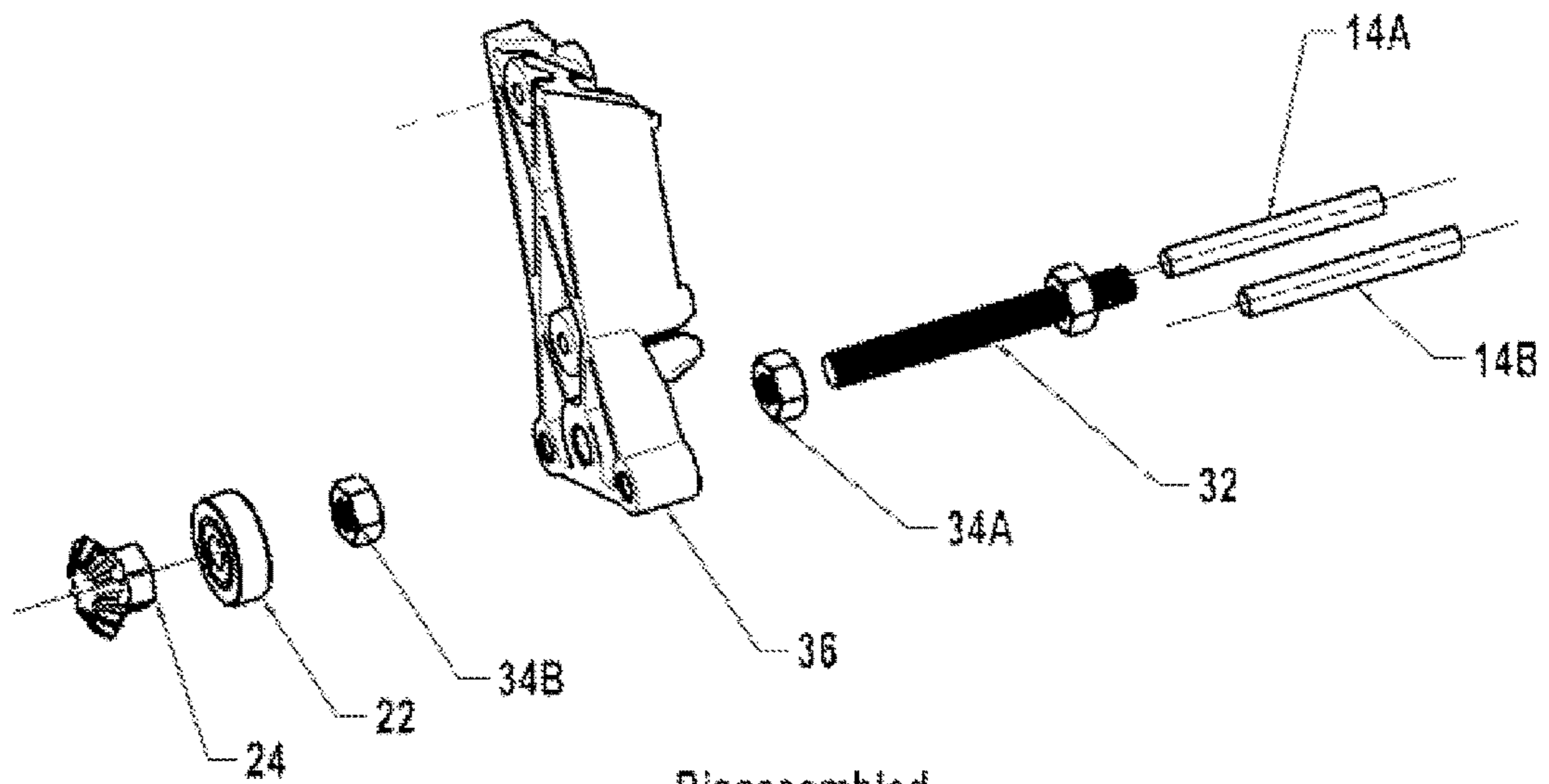
Disassembled
