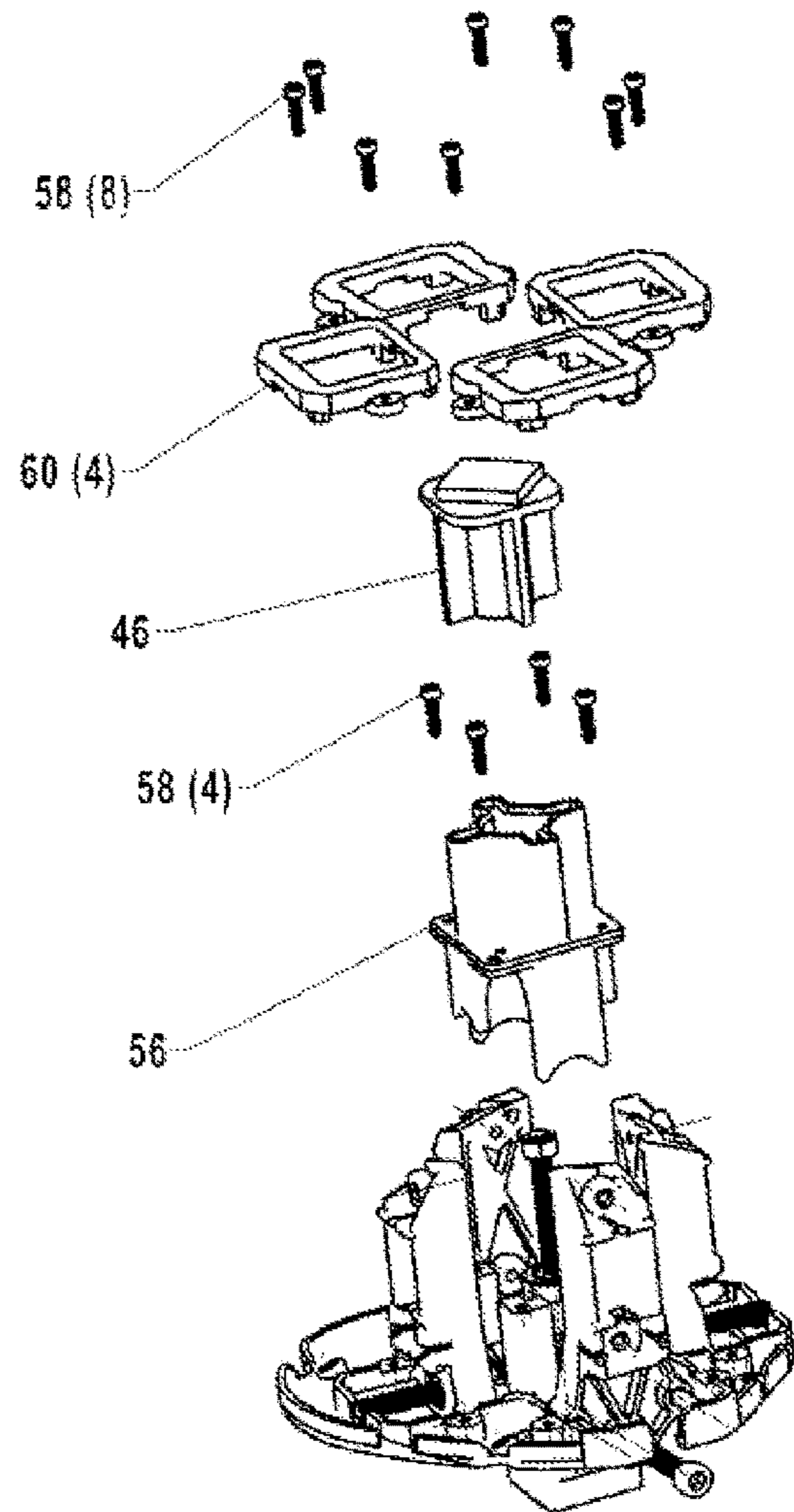
Disassembled
