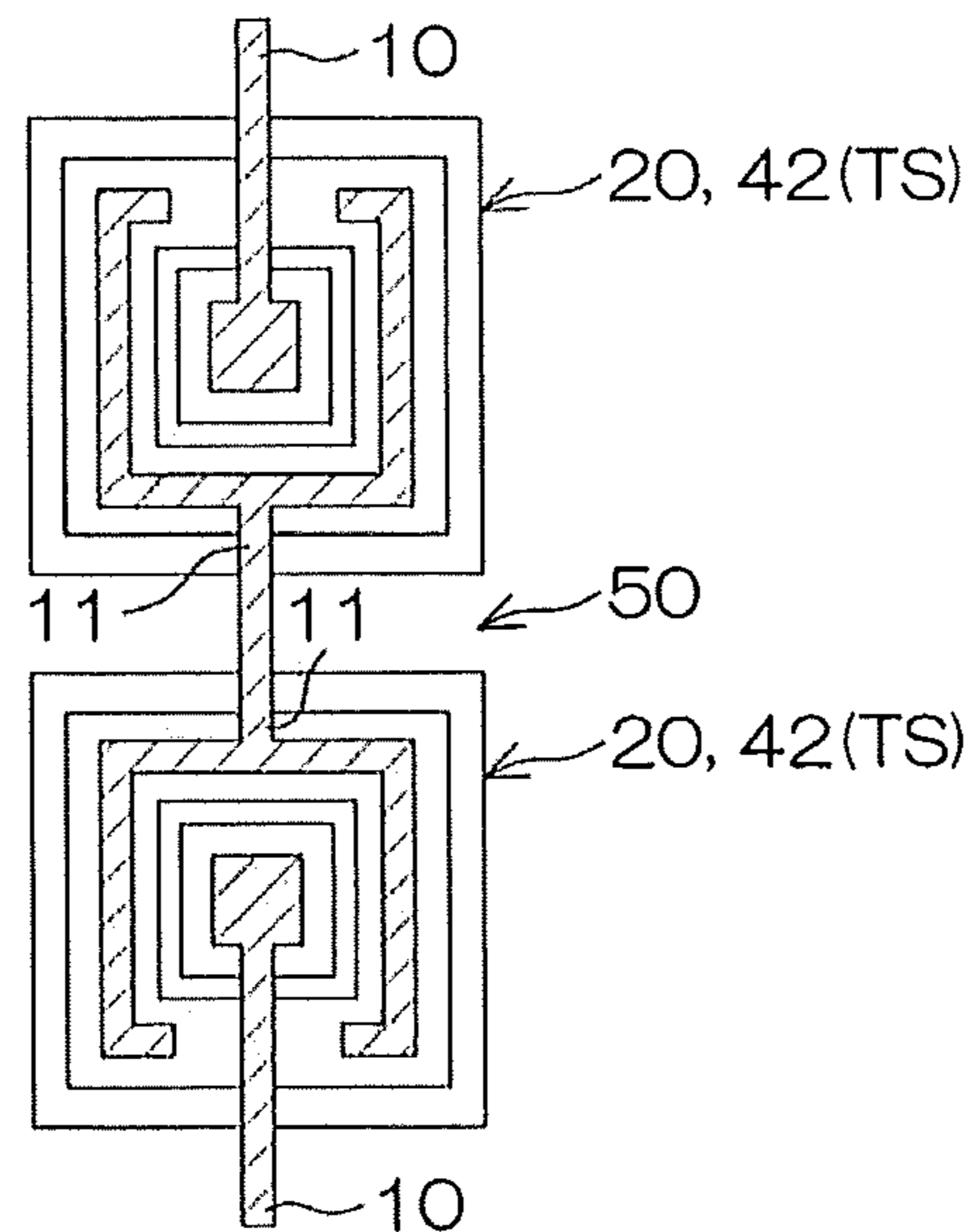
FIG. 12 (Reverse-series connection)
