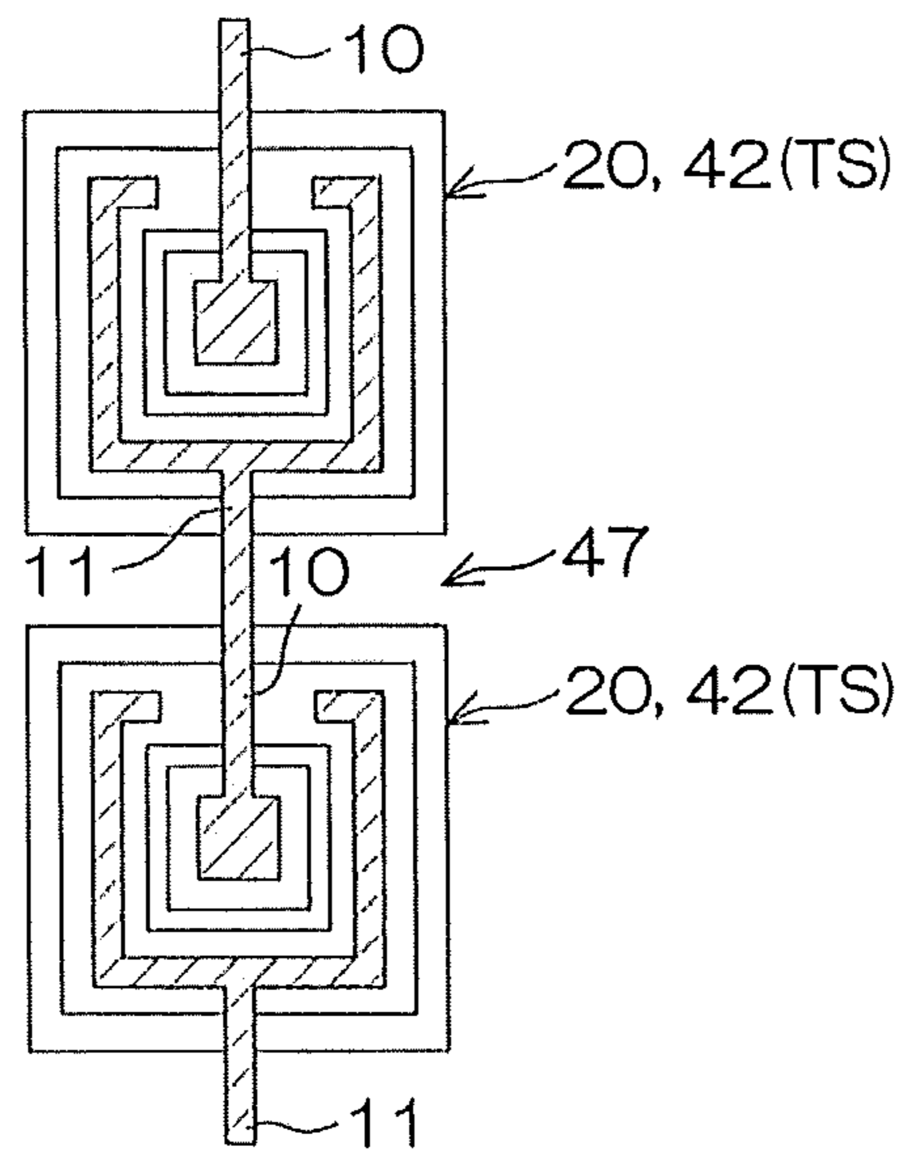
FIG. 10 (Serial connection)
