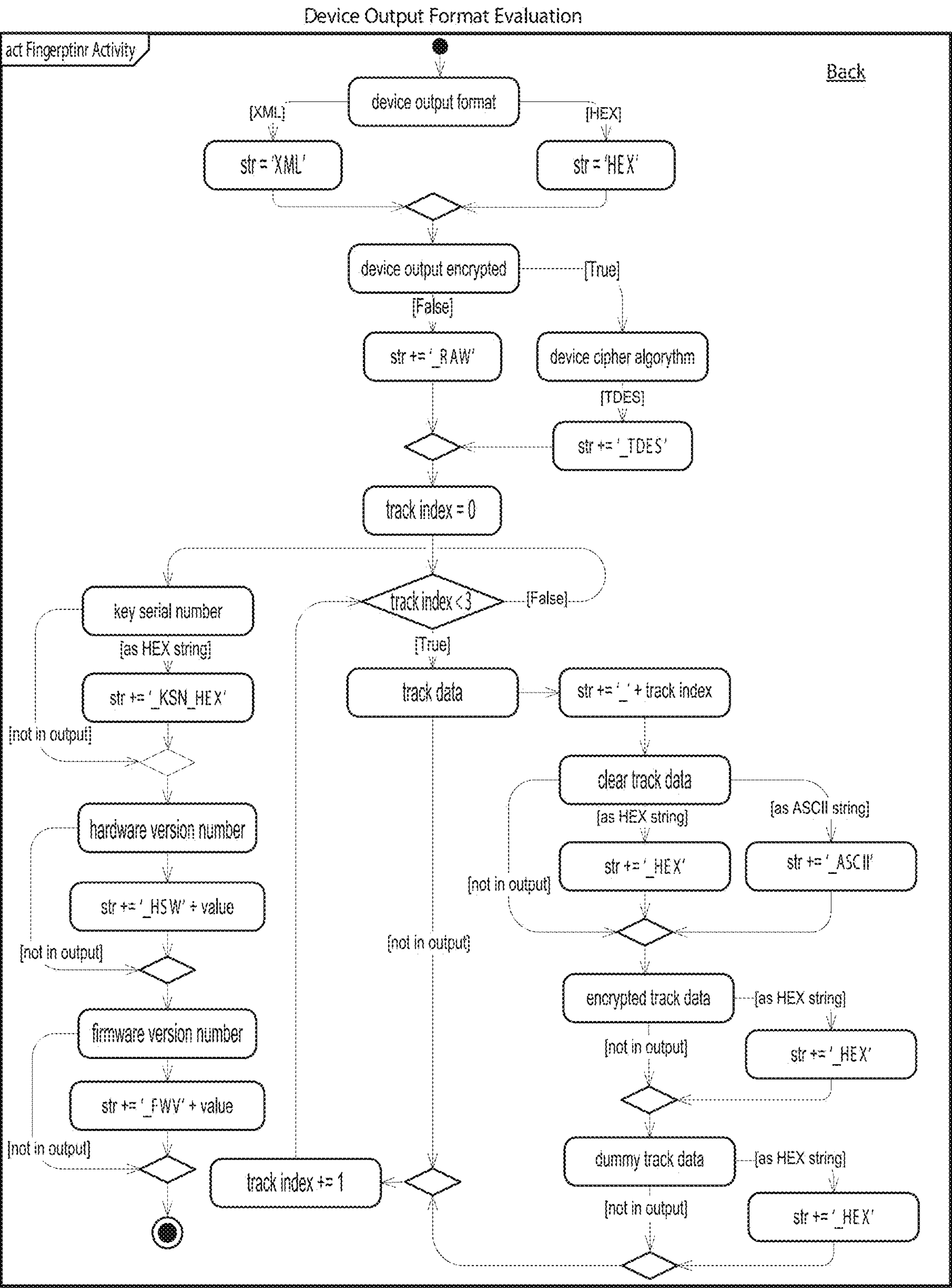
UML OF EXEMPLARY OUTPUT EVALUATION
