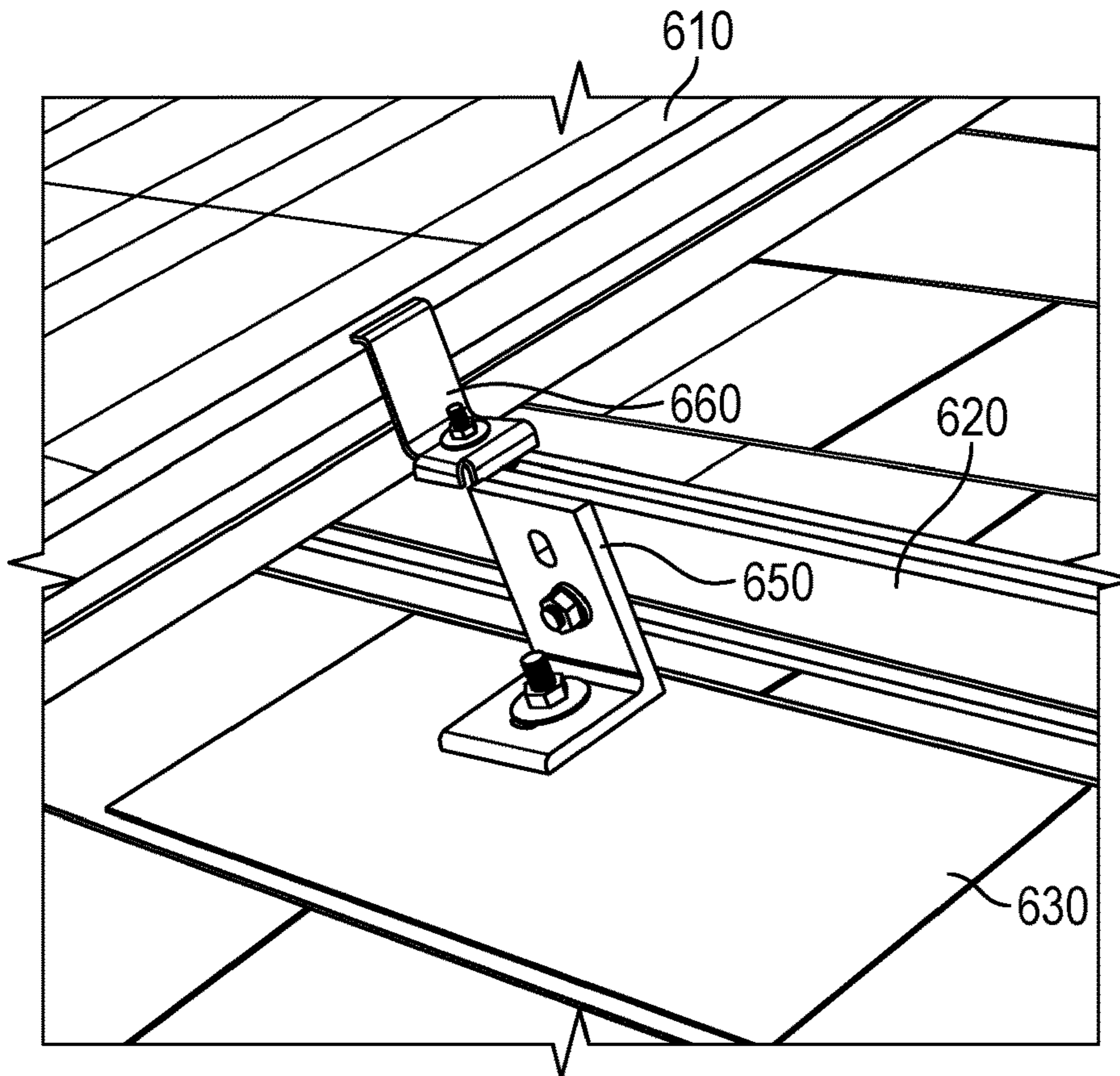
FIG. 2 PRIOR ART
