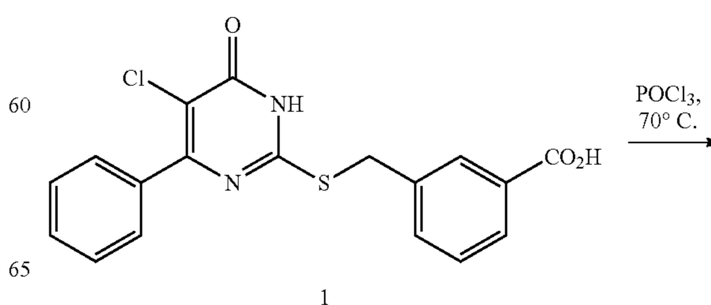
Scheme 22: Preparation of Compound 22
