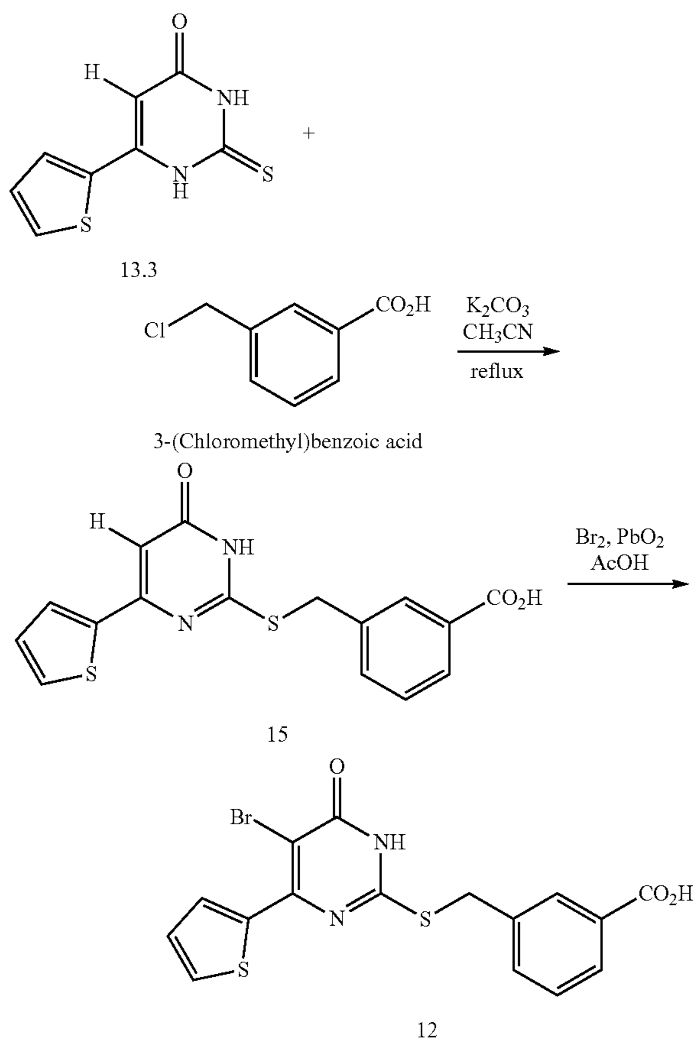
Scheme 20: Preparation of Compound 12
