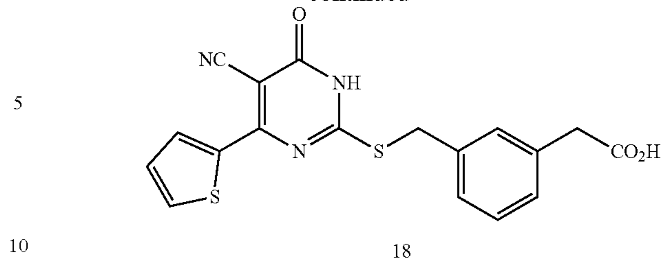
Example 26: Preparation of Compound 18
