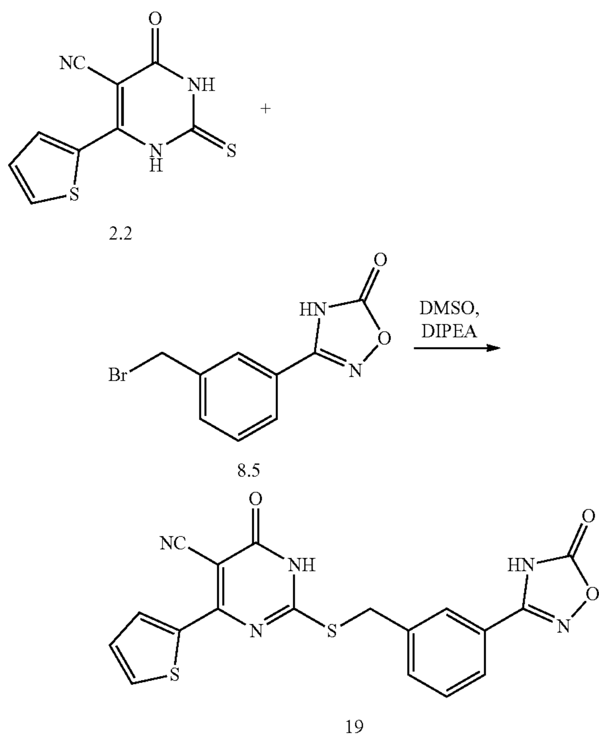
Scheme 25: Preparation of Compound 19
