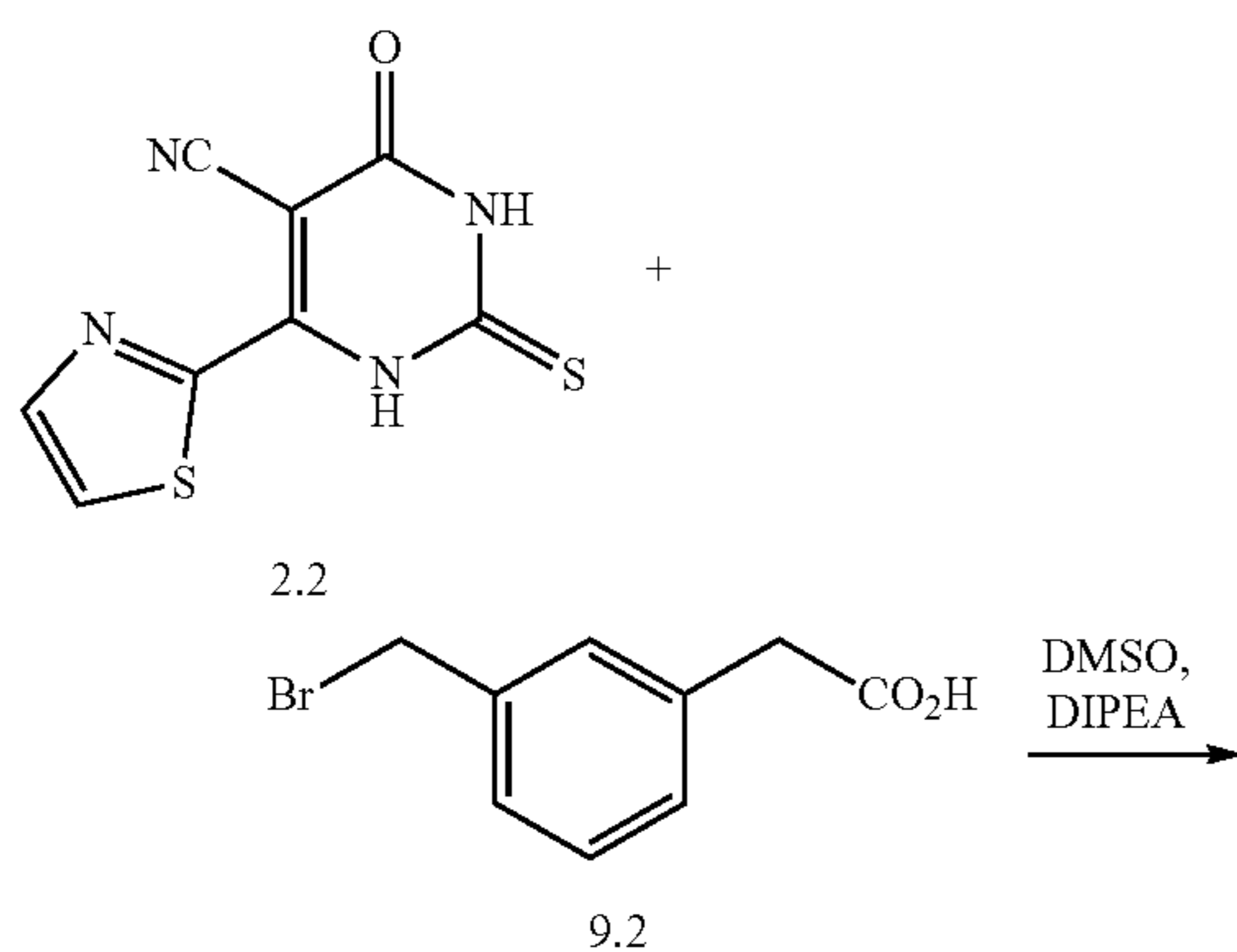
Scheme 26: Preparation of Compound 18
