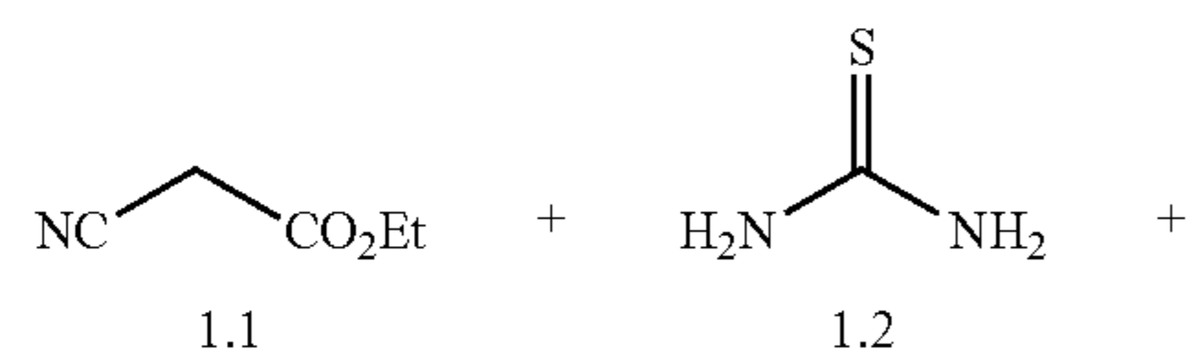
Scheme 1: Preparation of Intermediate 1.4
