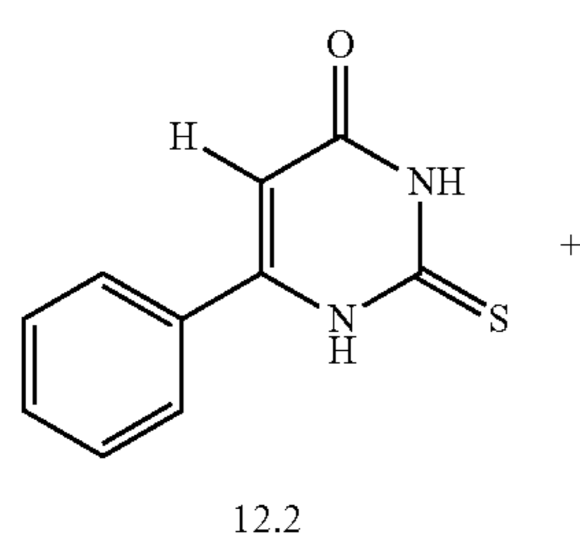
Scheme 19: Preparation of Compound 11
