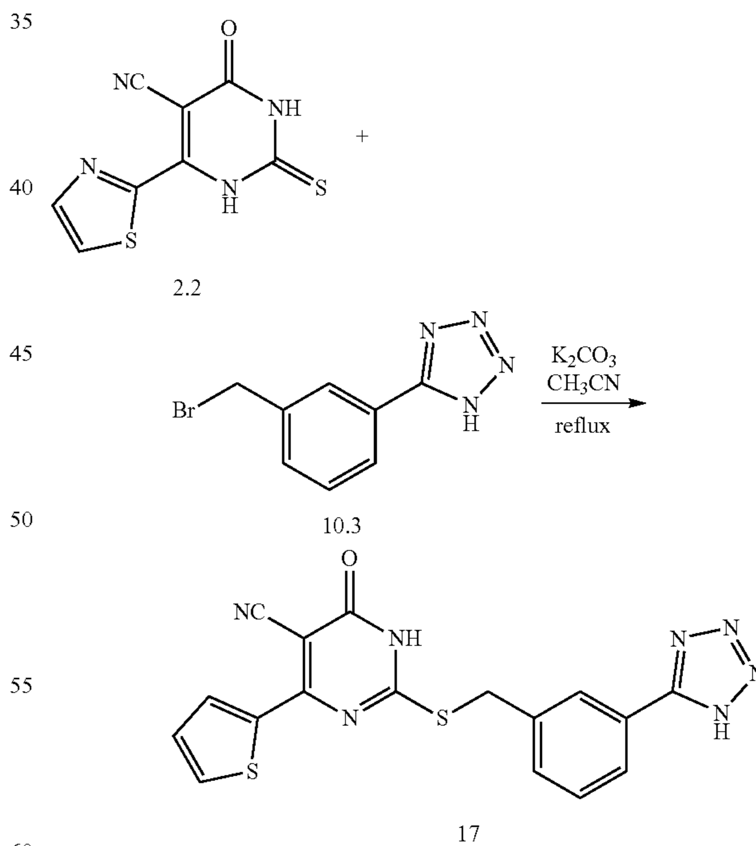
Scheme 27: Preparation of Compound 17
