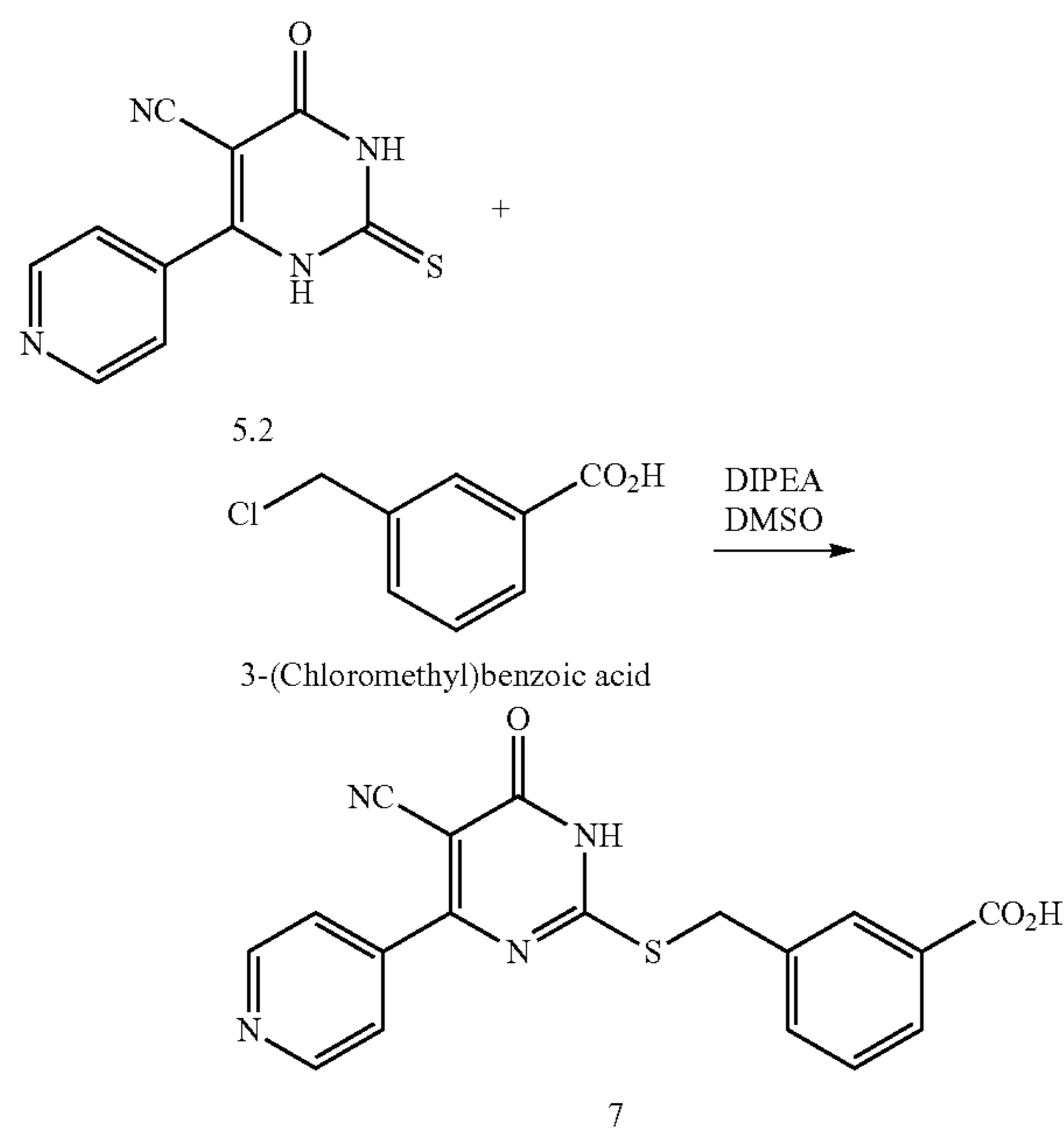
Scheme 18: Preparation of Compound 7
