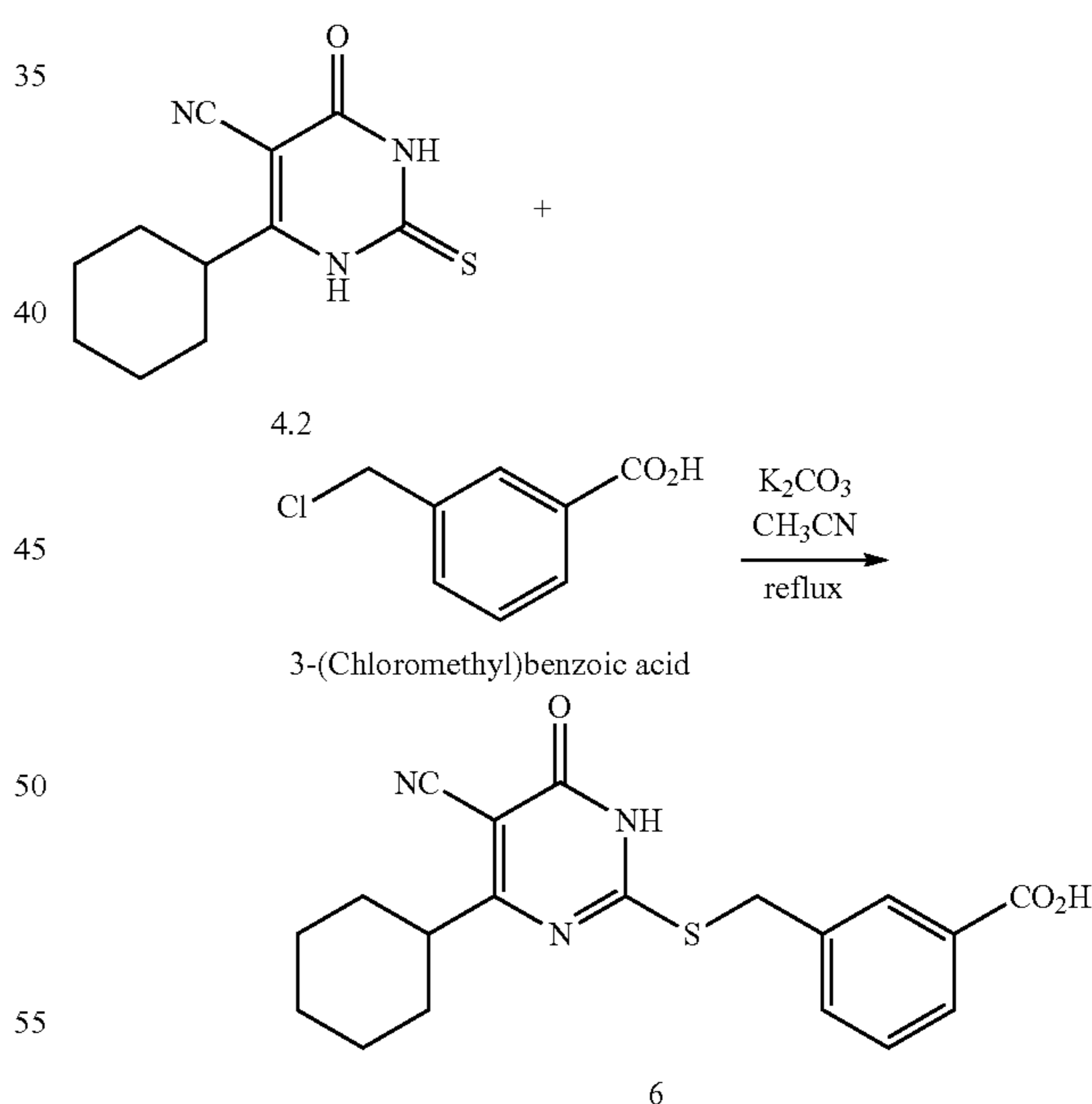
Scheme 17: Preparation of Compound 6
