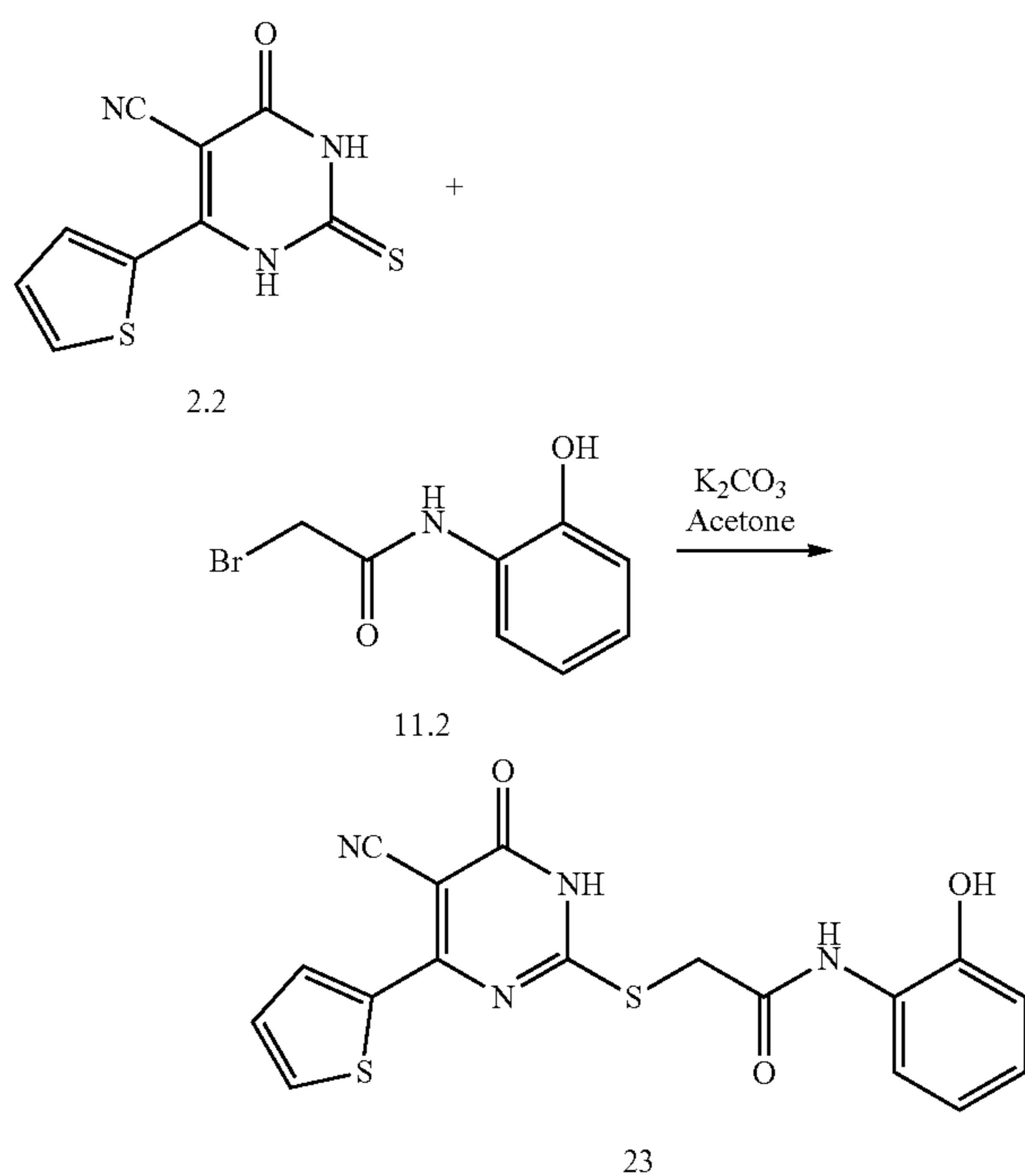
Scheme 28: Preparation of Compound 23
