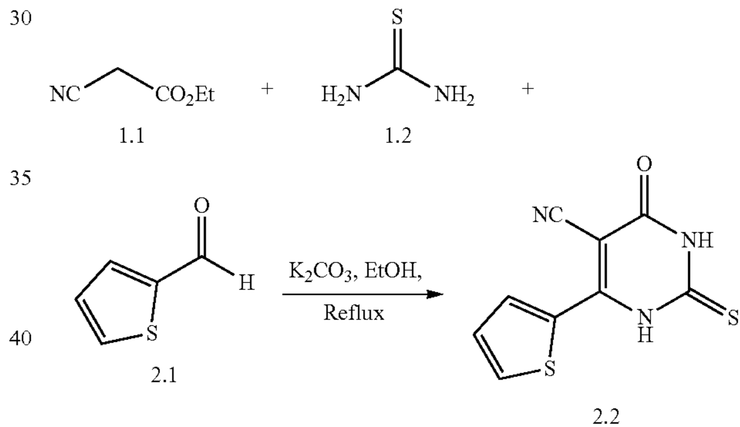
Scheme 2: Preparation of Intermediate 2.2
