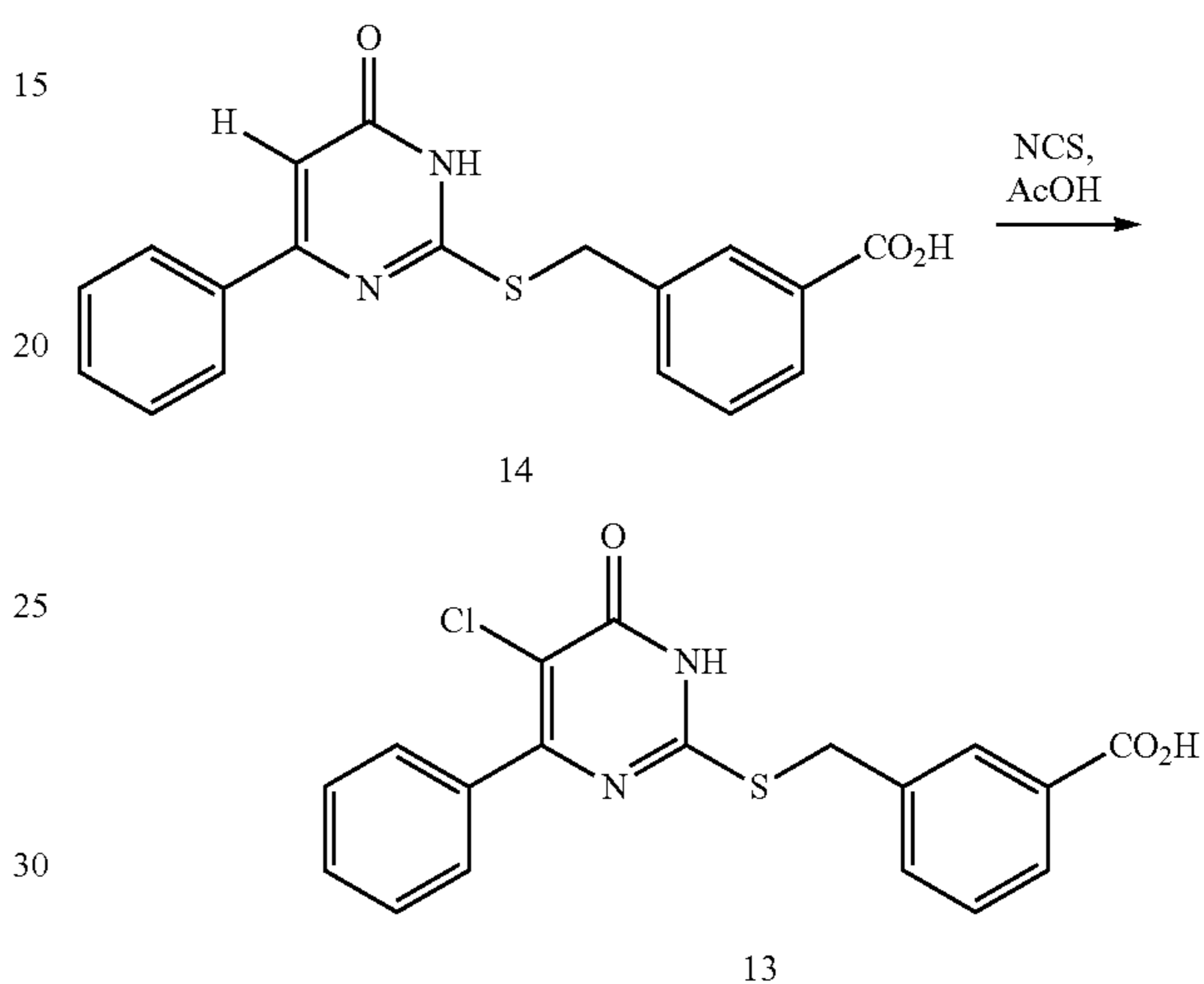
Scheme 21: Preparation of Compound 13
