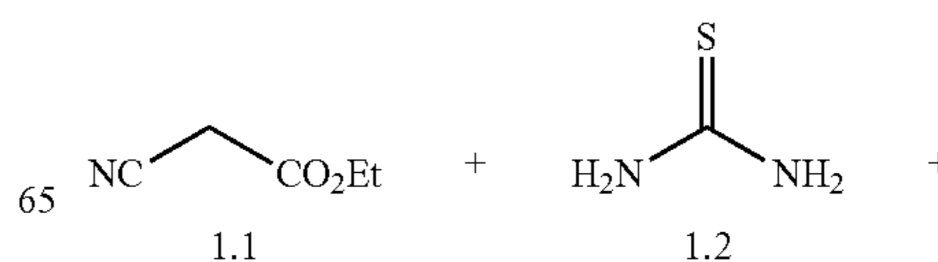
Scheme 3: Preparation of Intermediate 3.2
