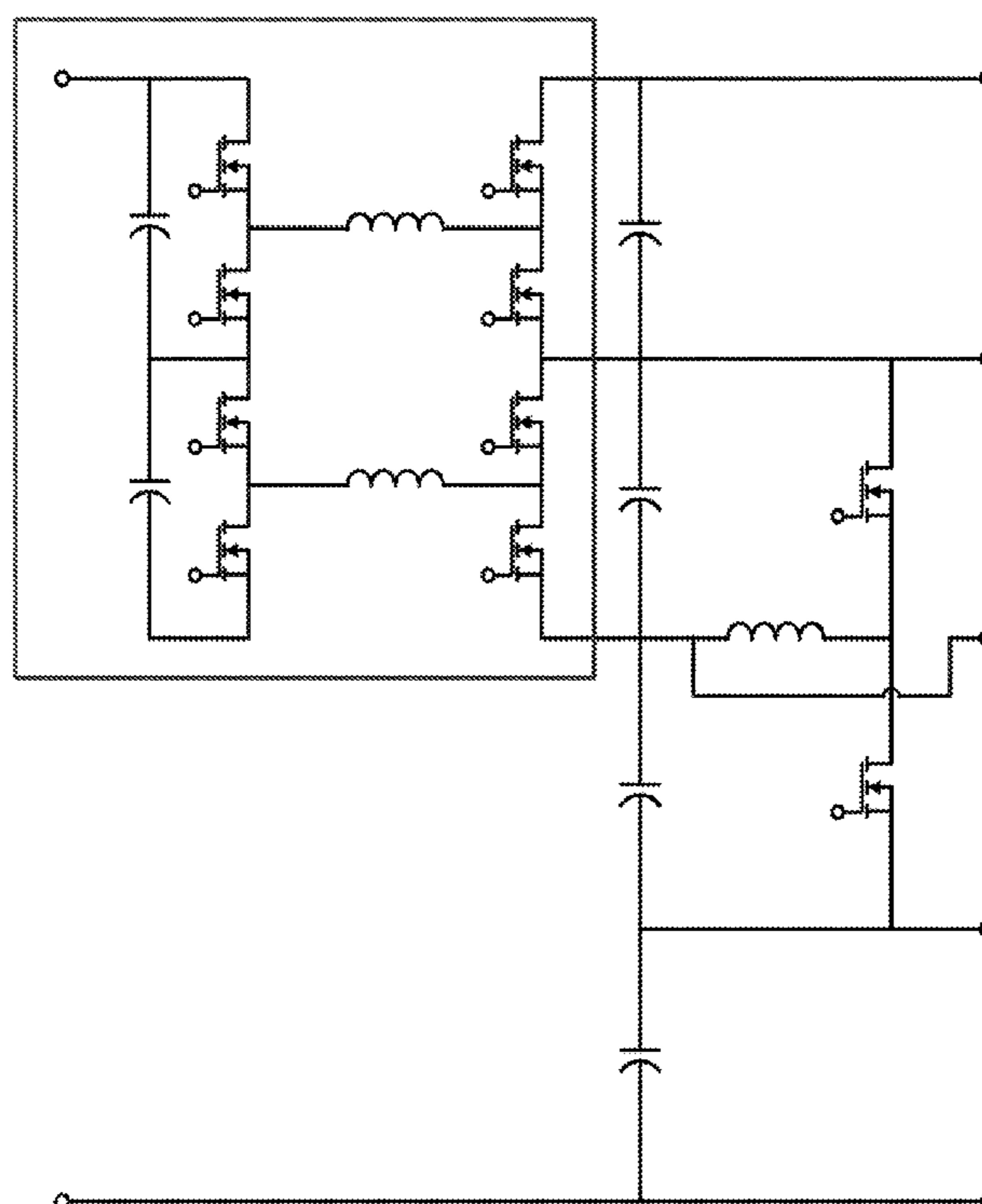
Buck-boost, can be paralleled
