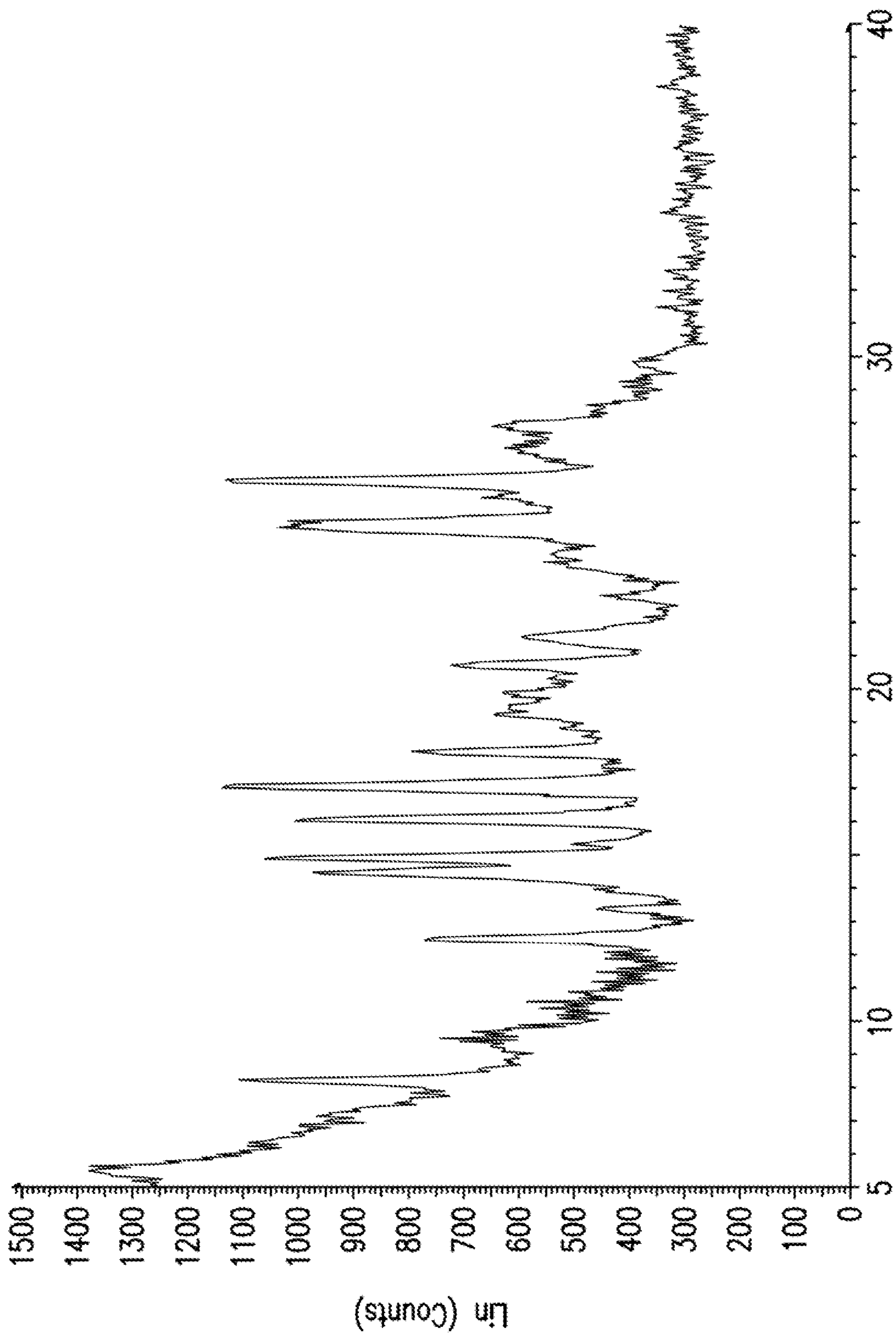
2-Theta - Scale
