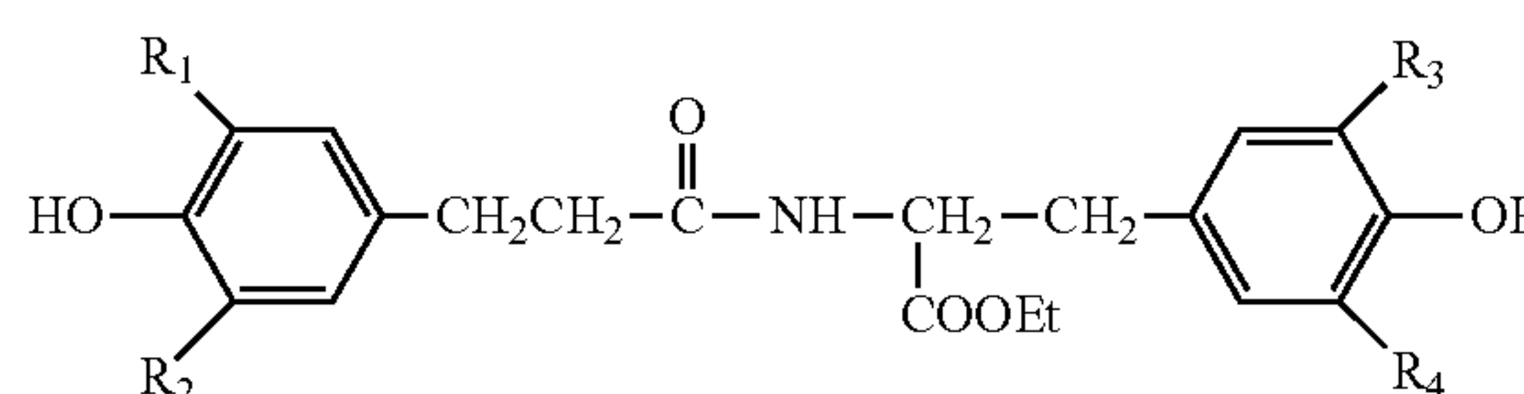
General Structure of iodinated DTE monomer
