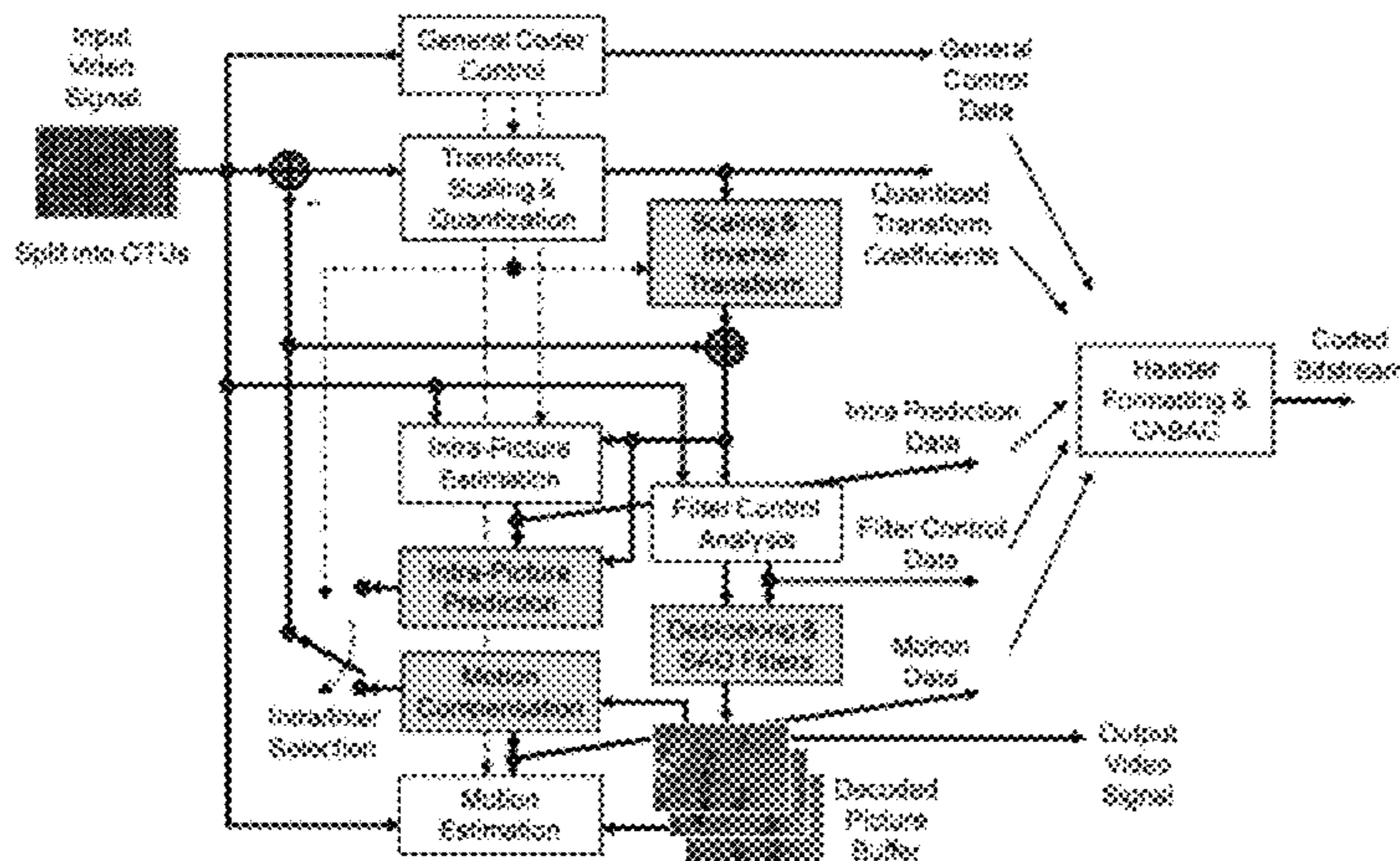
FIG. 1 is a block diagram of a video processing system according to an embodiment of the present disclosure.
