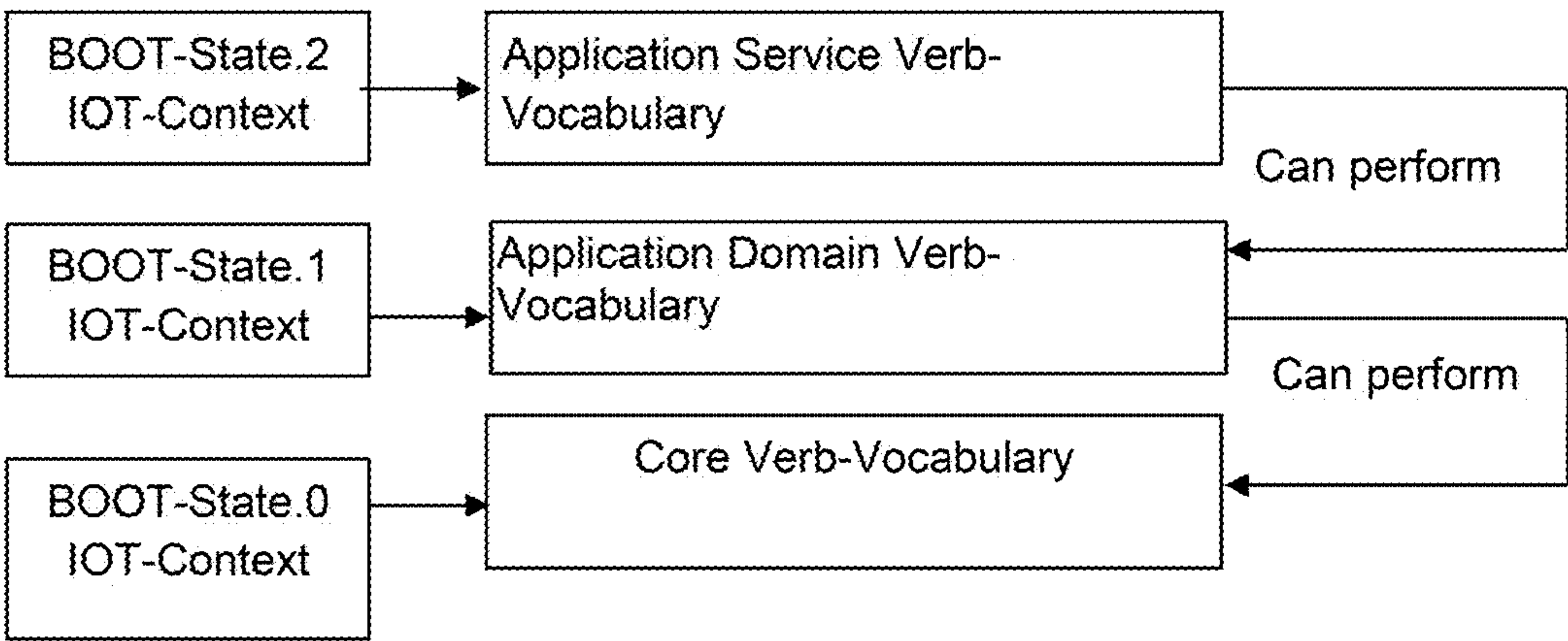
FIG. 55 Verb Vocabulary
