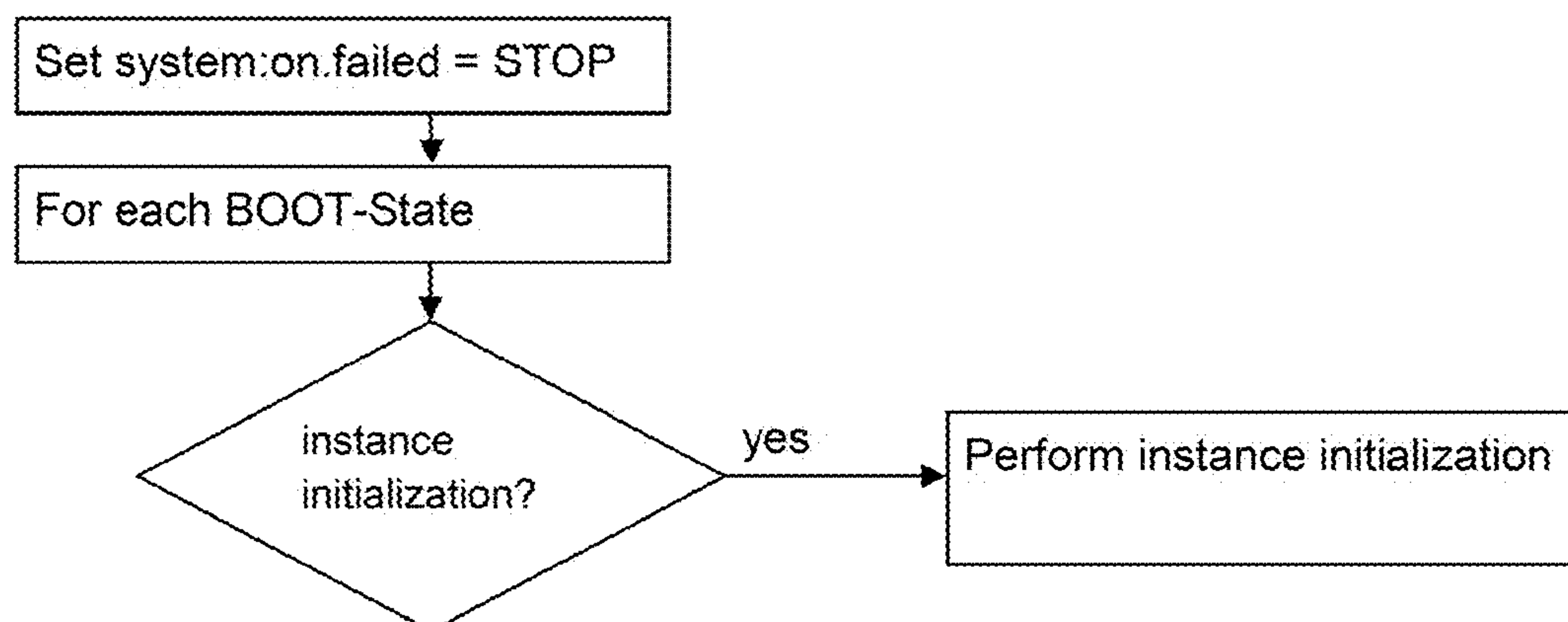
FIG. 19 ExecutiveStart (Boot-6)
