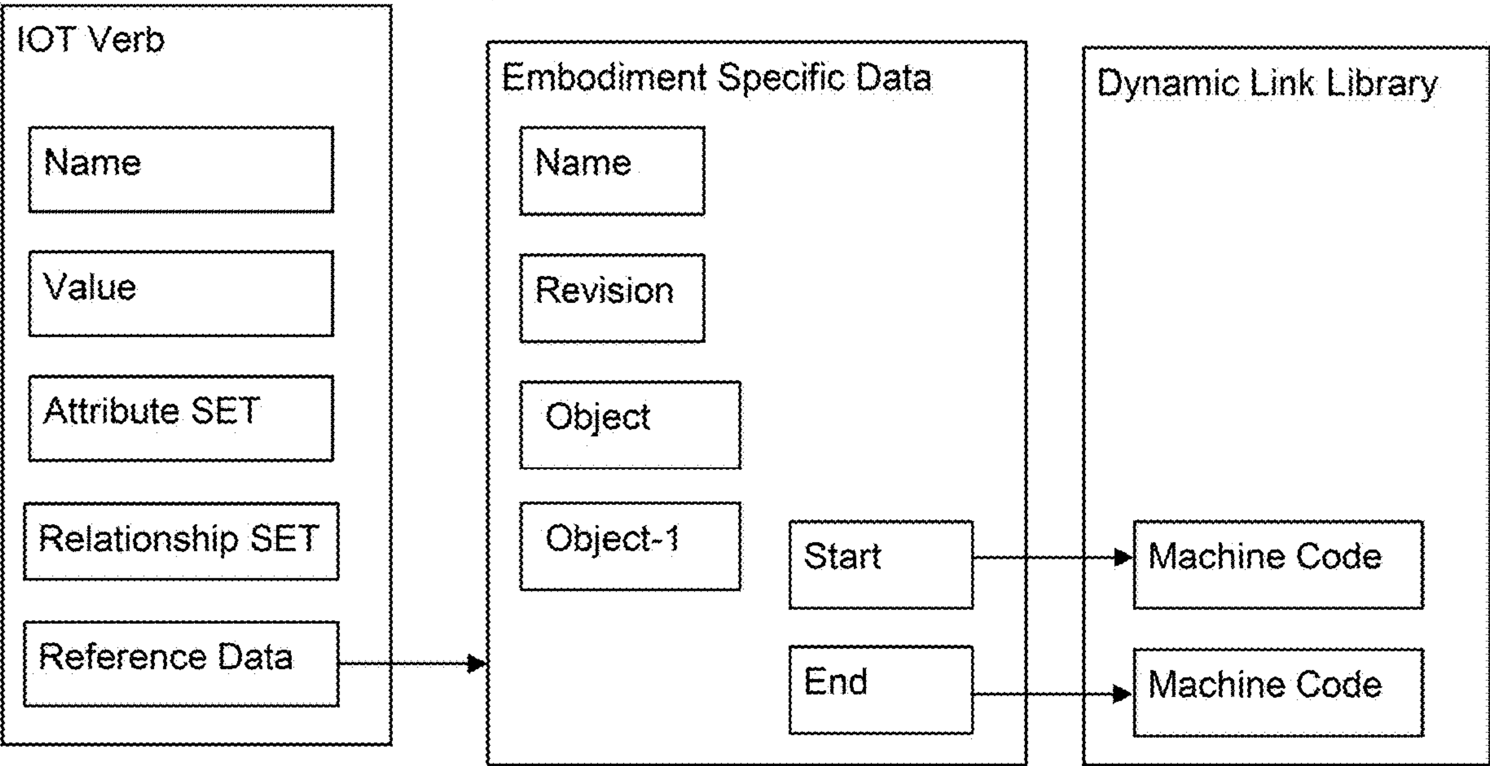
FIG. 8A Shared Library Embodiment Specific Data
