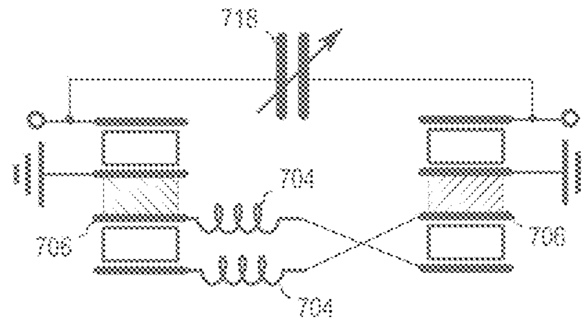
Bandpass Filter Fixed Tuned zero Fig. 12B
