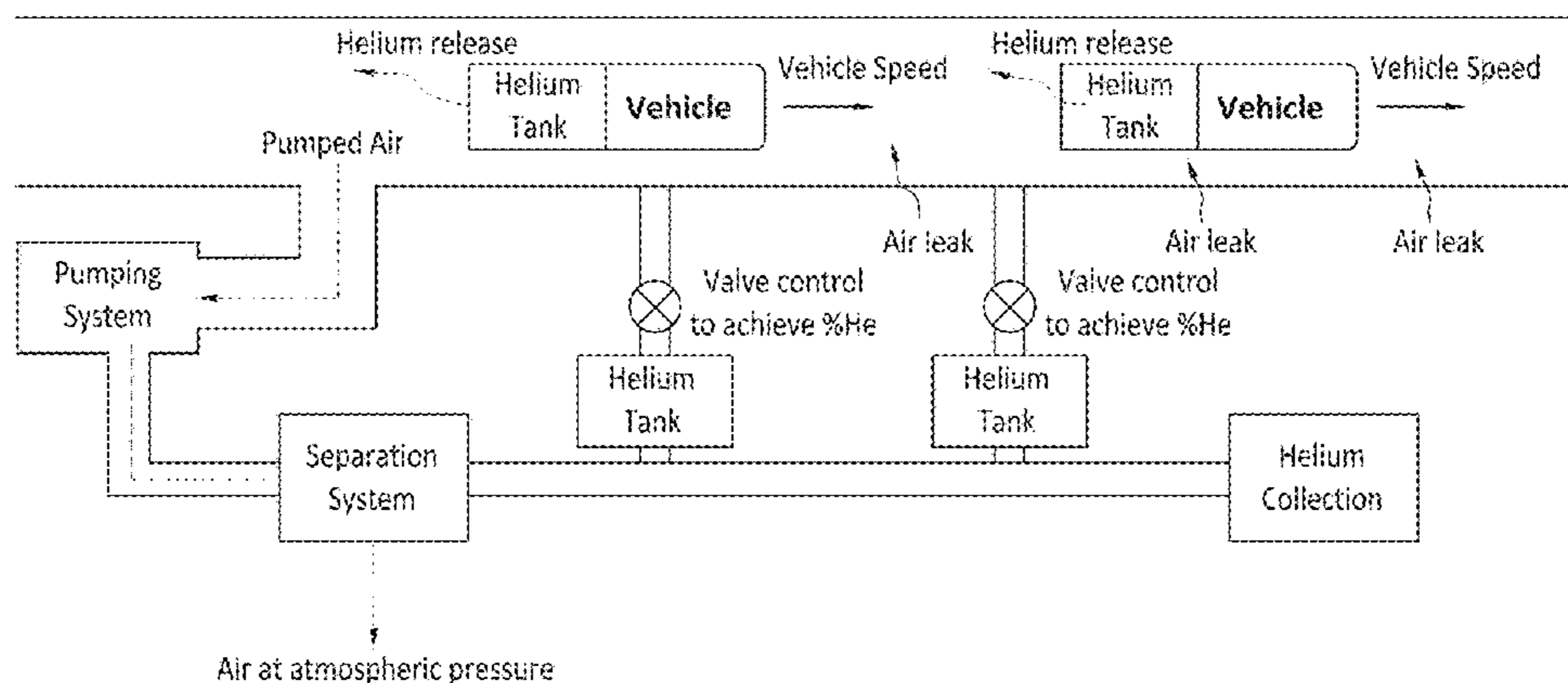
Tube Transportation with Helium mixture Tanks combined in Tube and Vehicles
