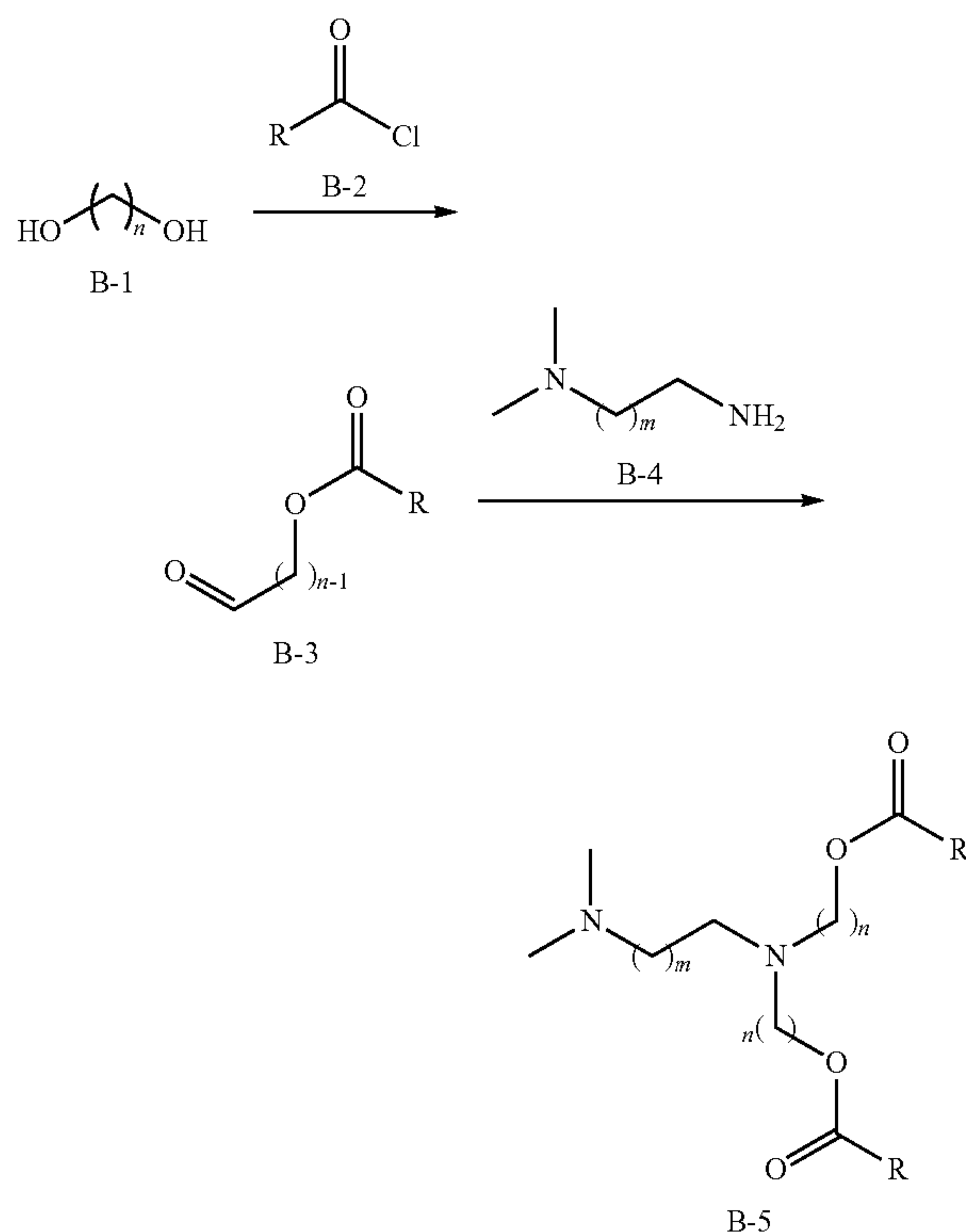
GENERAL REACTION SCHEME 2
