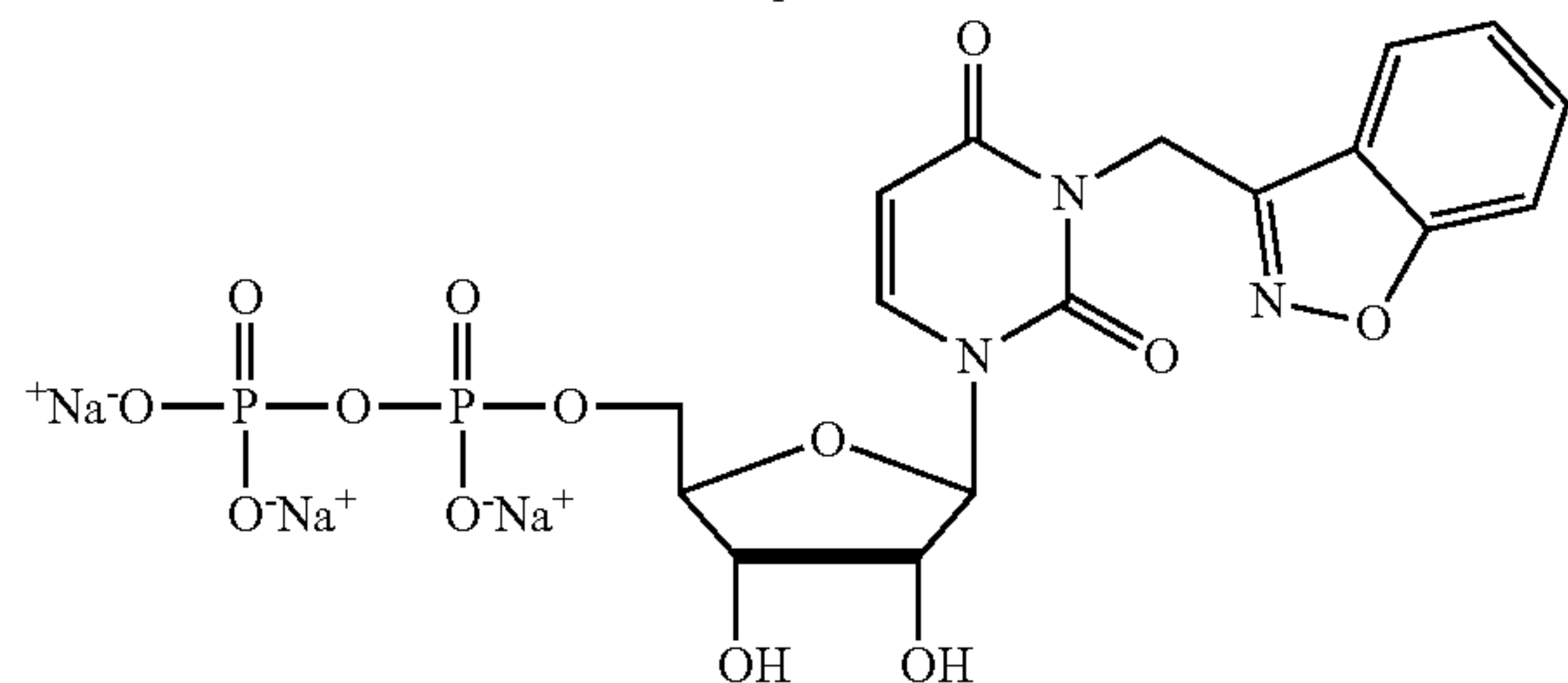
sodium salt of compound 5
