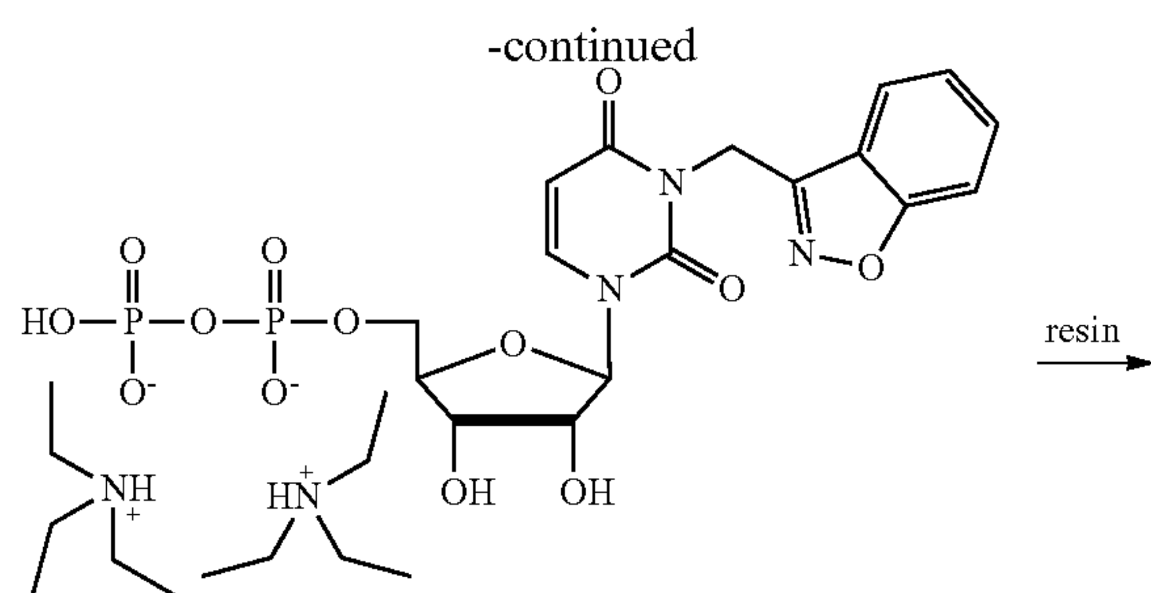
TEA salt of compound 5
