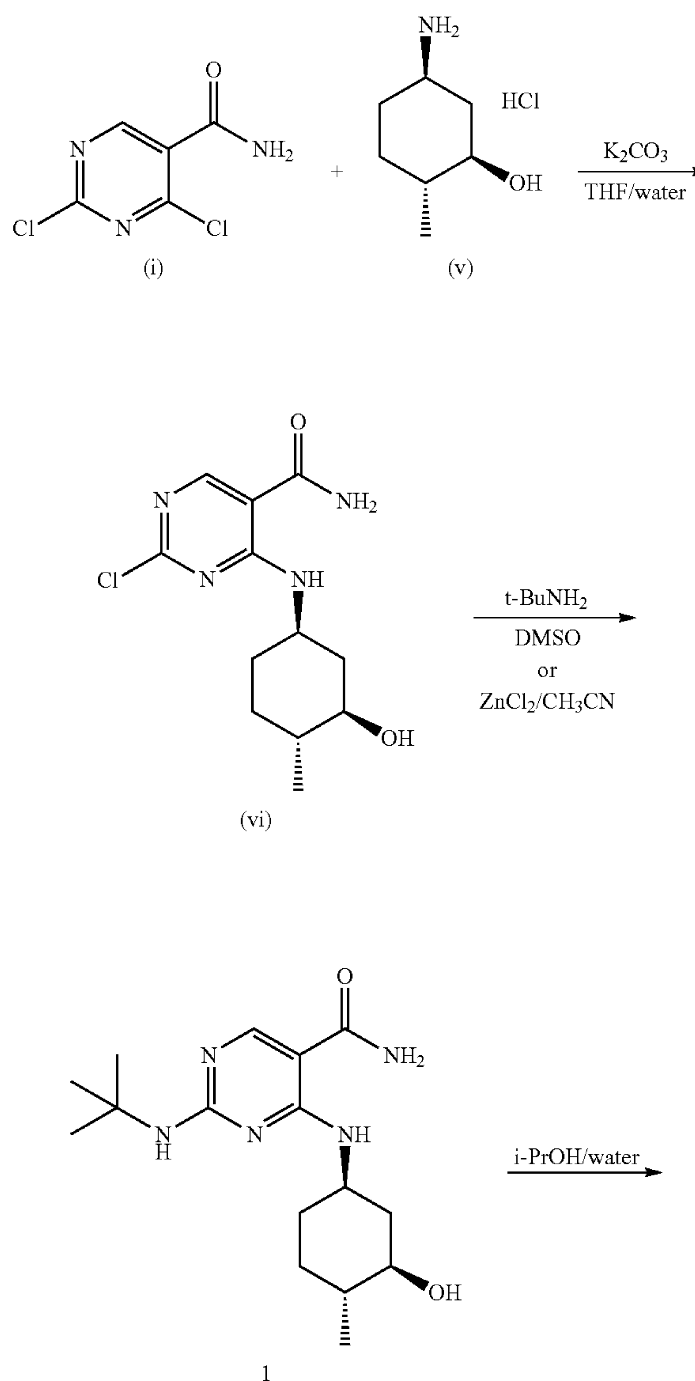
Scheme 2
