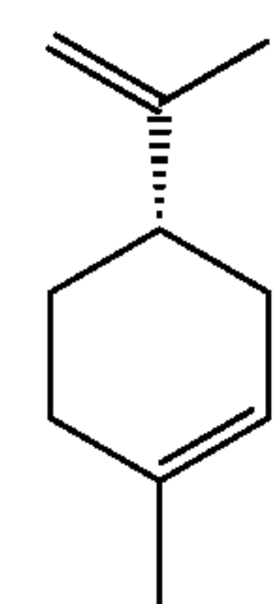
(-)-limonene
