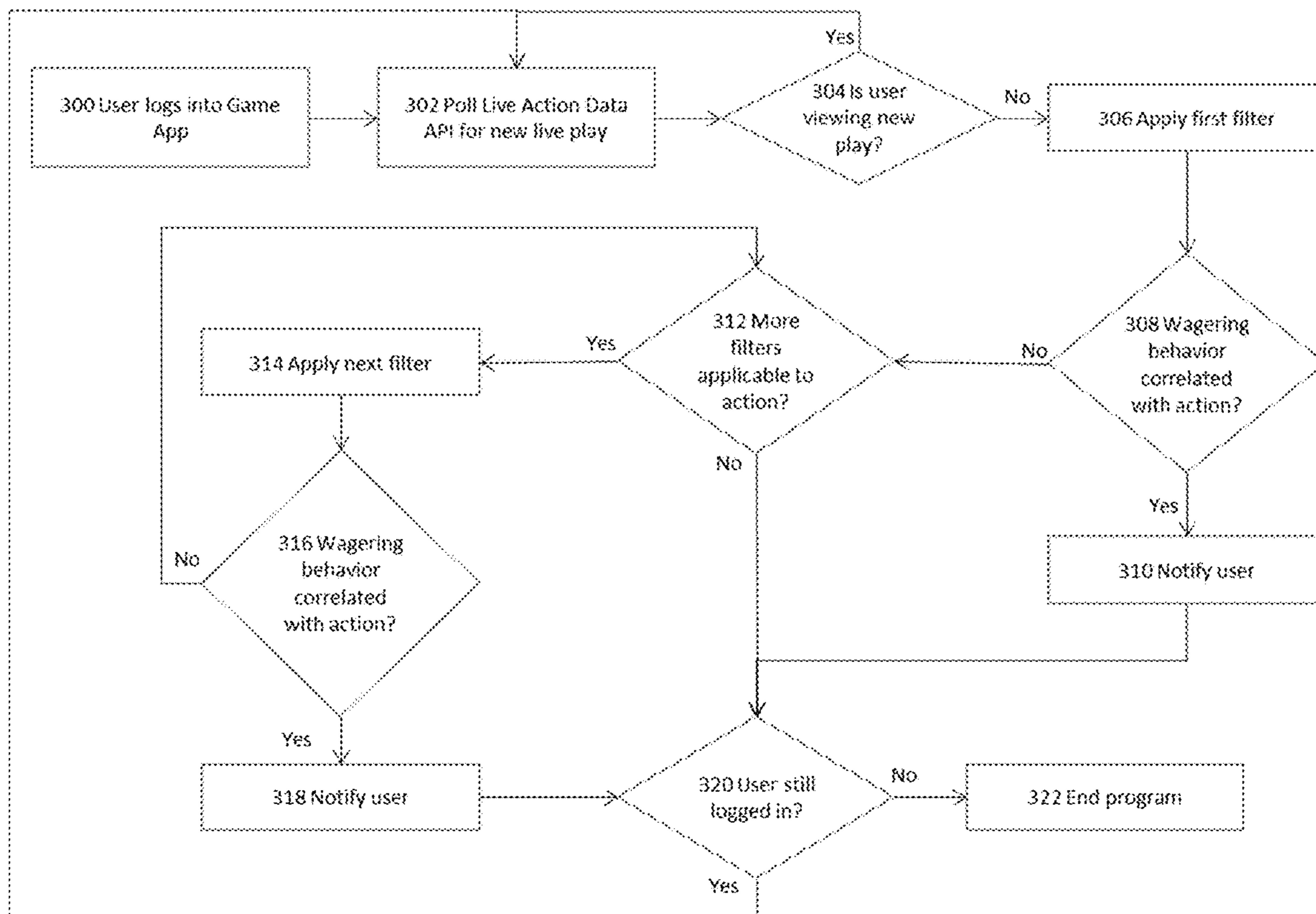
Fig. 3 Notification Module
