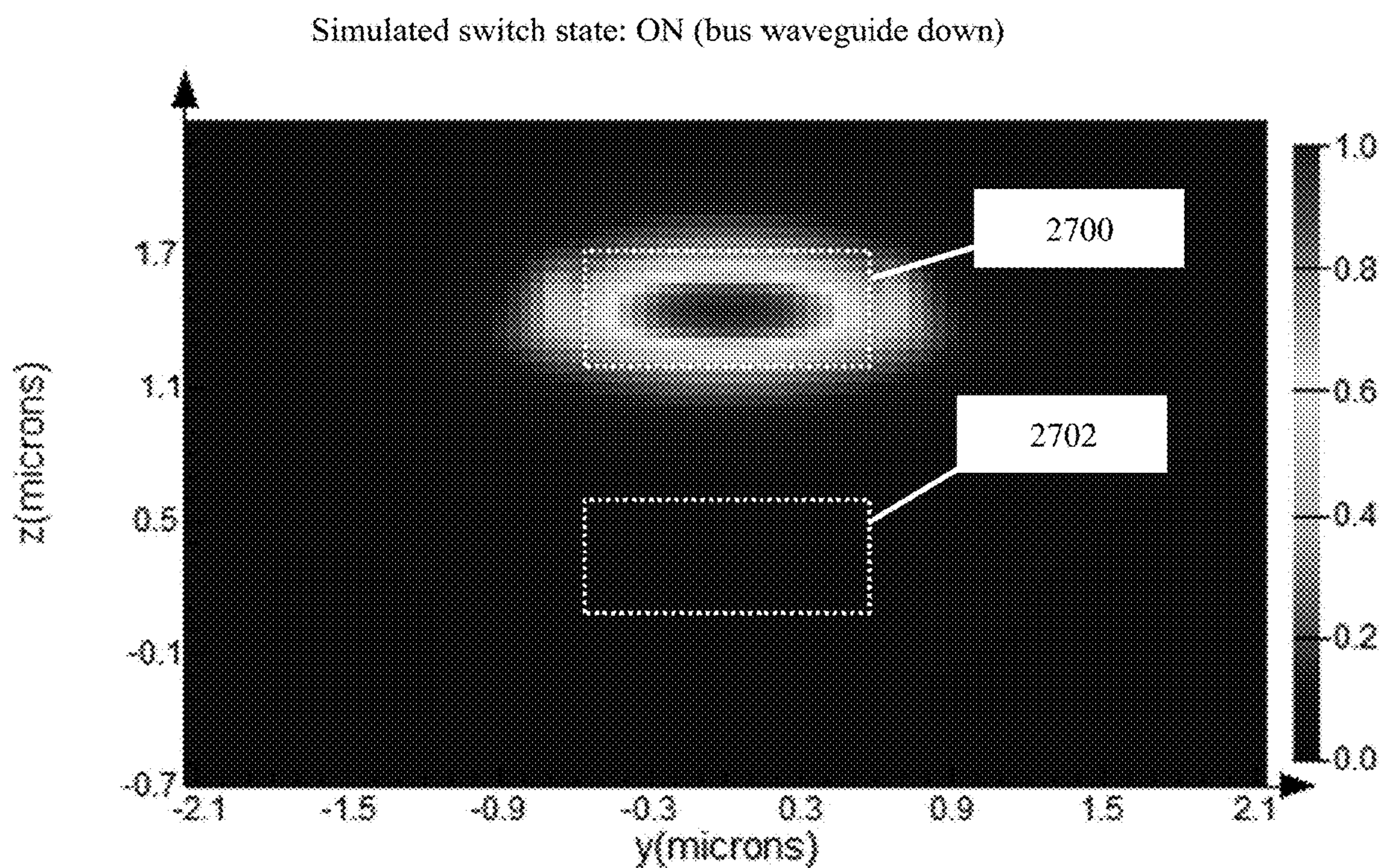
Propagating mode in top bus at start of adiabatic coupler
