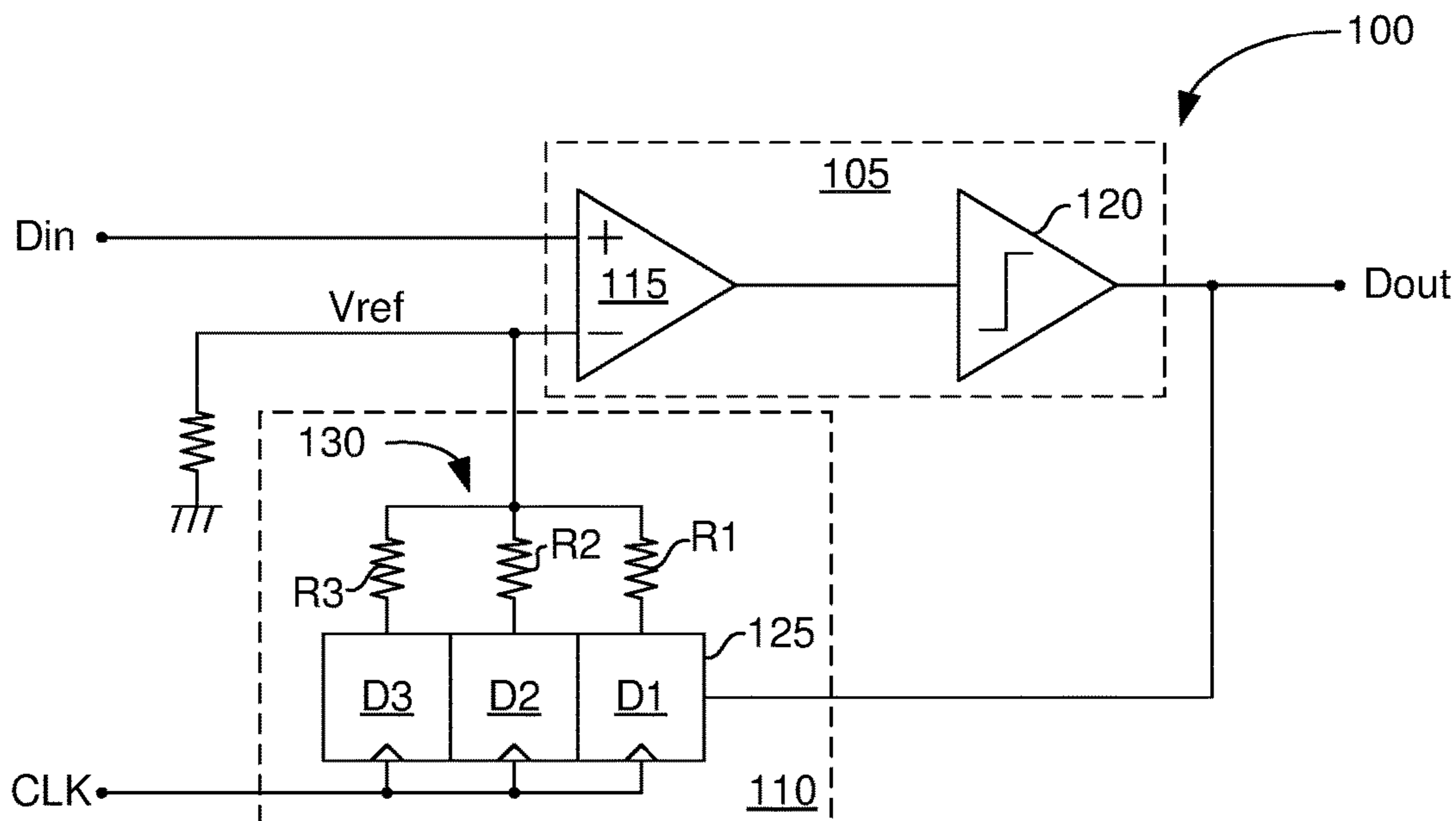
FIG. 1 (PRIOR ART)
