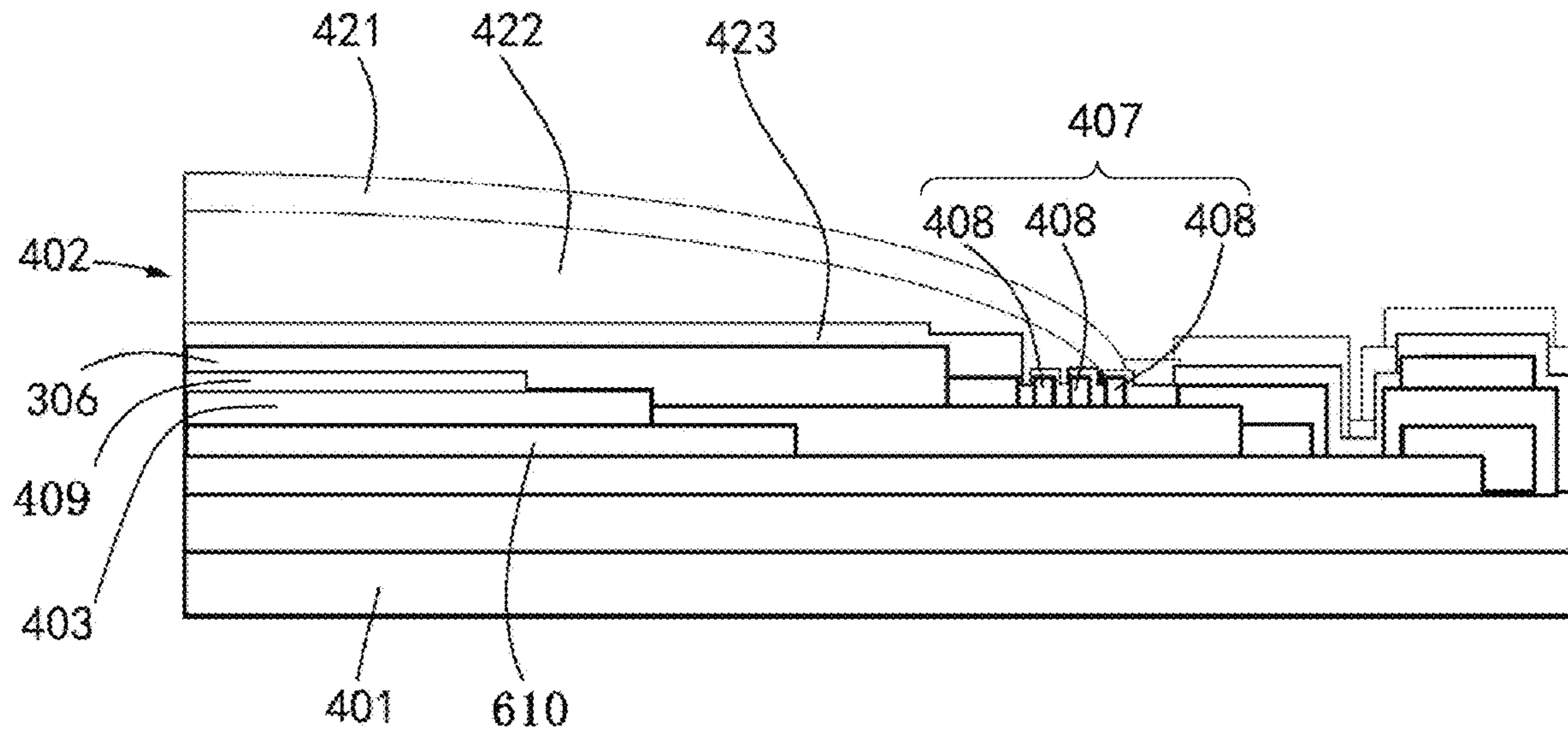
Fig. 4 (Related Art)
